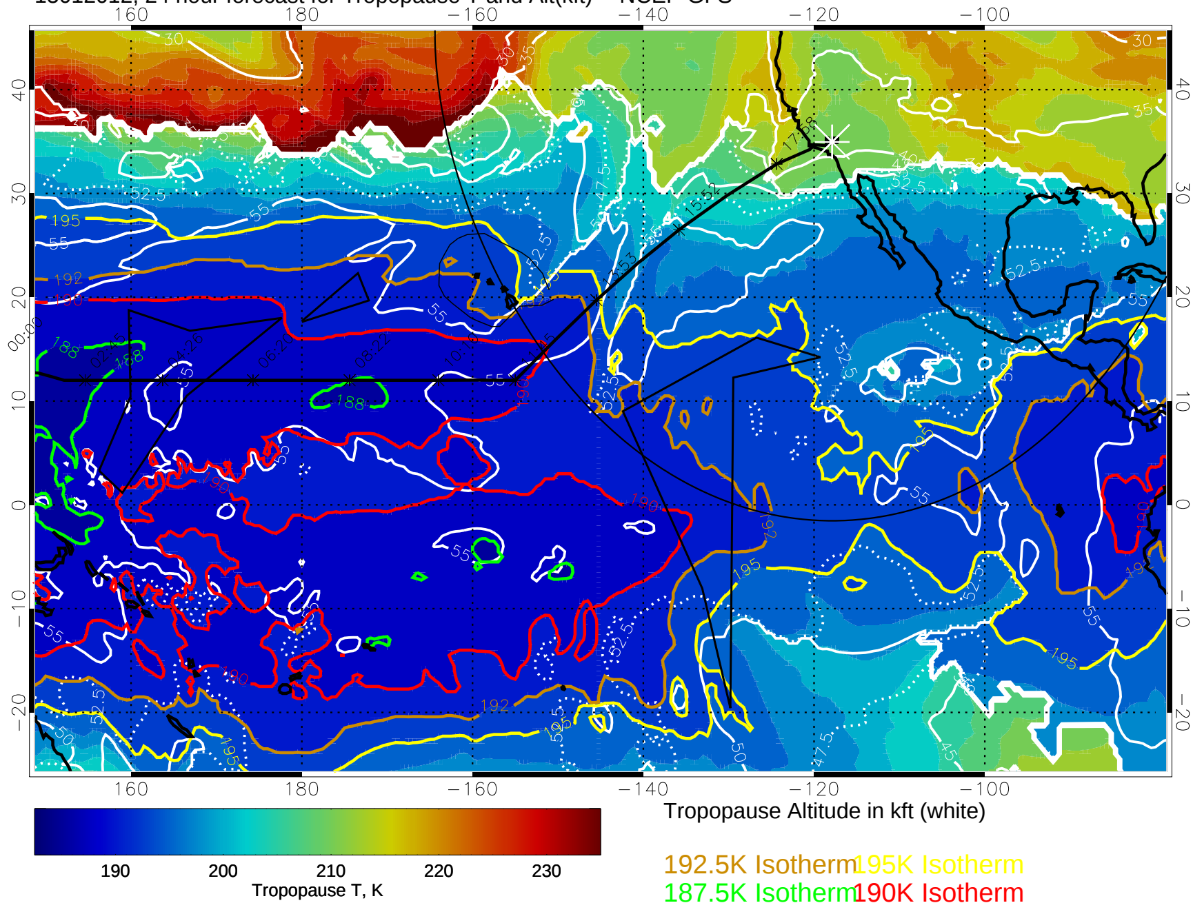
15012012, 24 hour forecast for Tropopause T and Alt(kft) -- NCEP GFS
