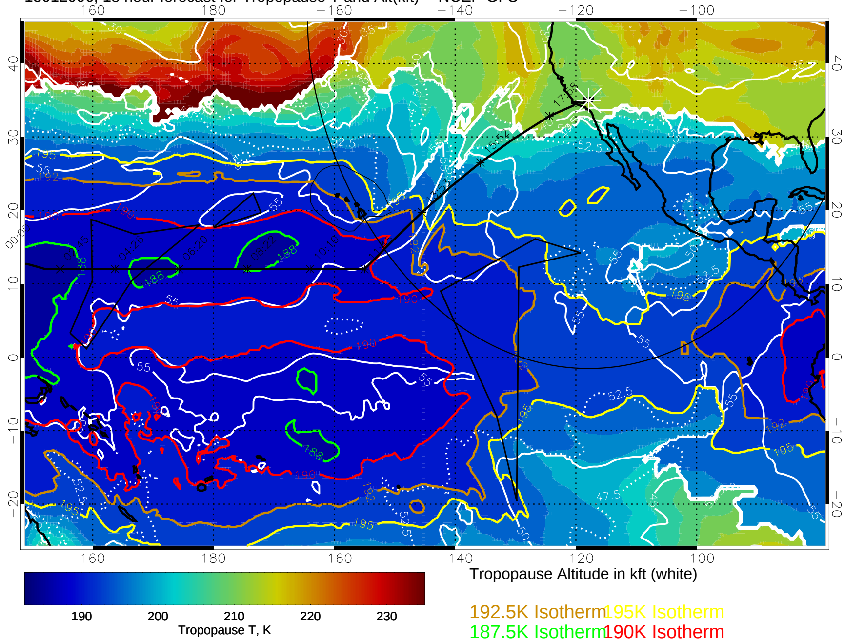
15012006, 18 hour forecast for Tropopause T and Alt(kft) -- NCEP GFS
