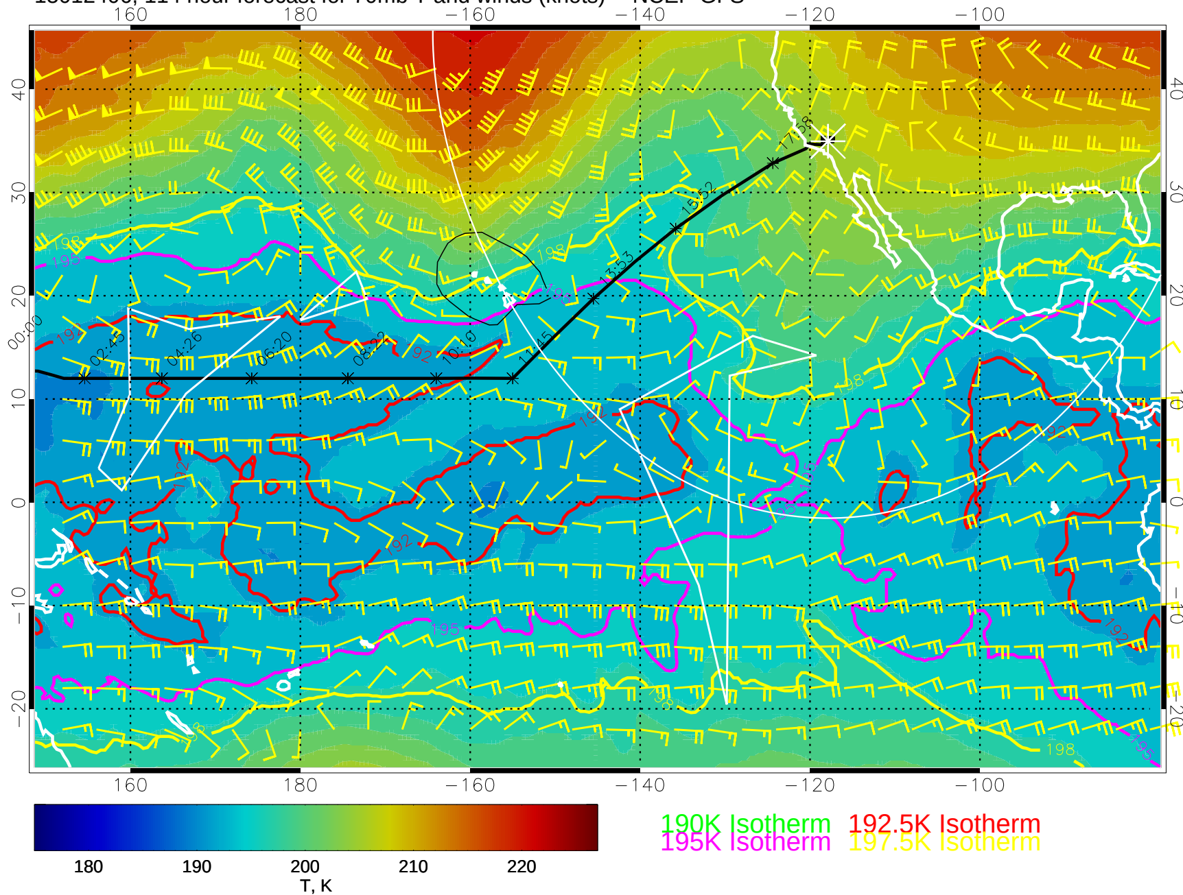
15012406, 114 hour forecast for 70mb T and winds (knots) -- NCEP GFS
