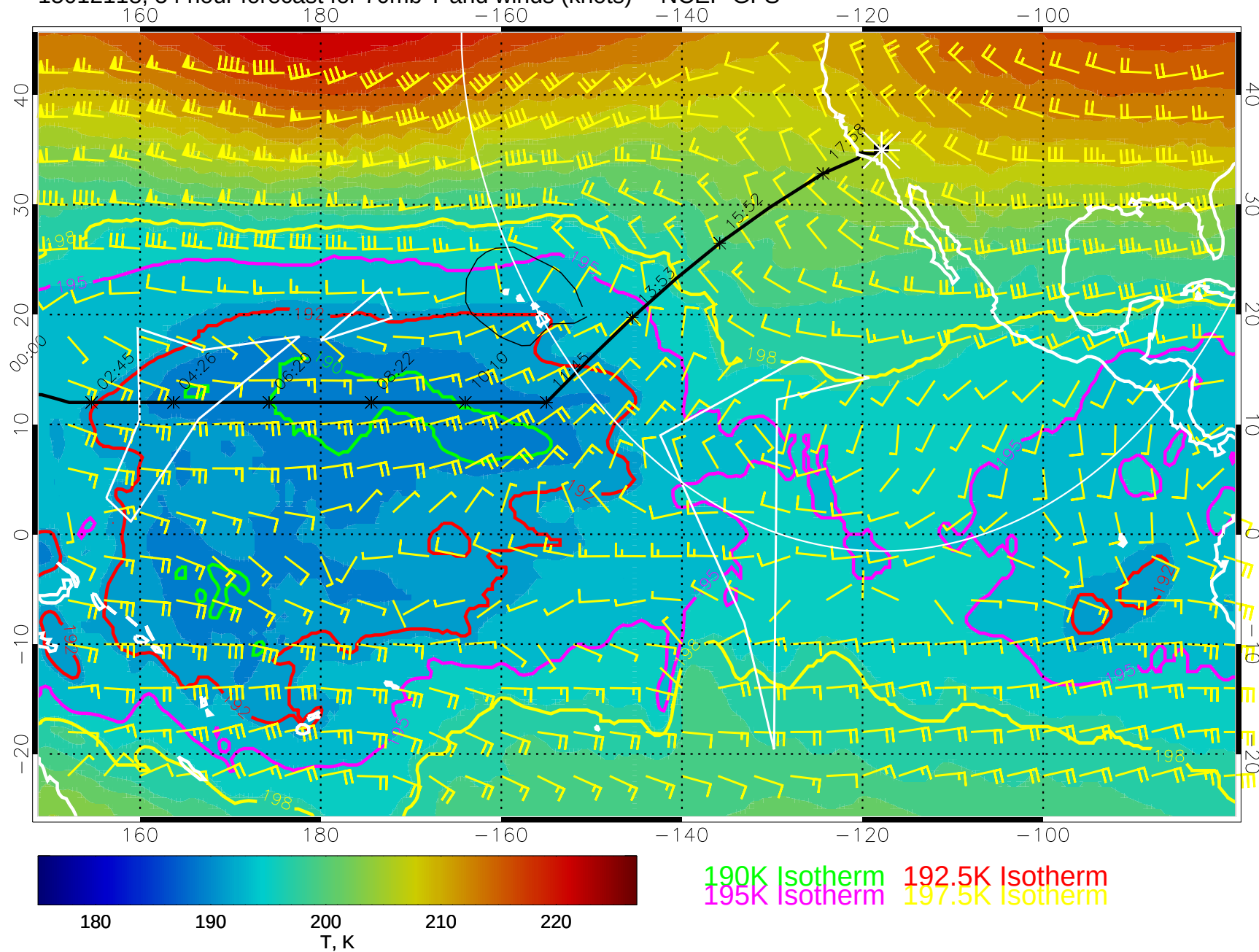
15012118, 54 hour forecast for 70mb T and winds (knots) -- NCEP GFS
