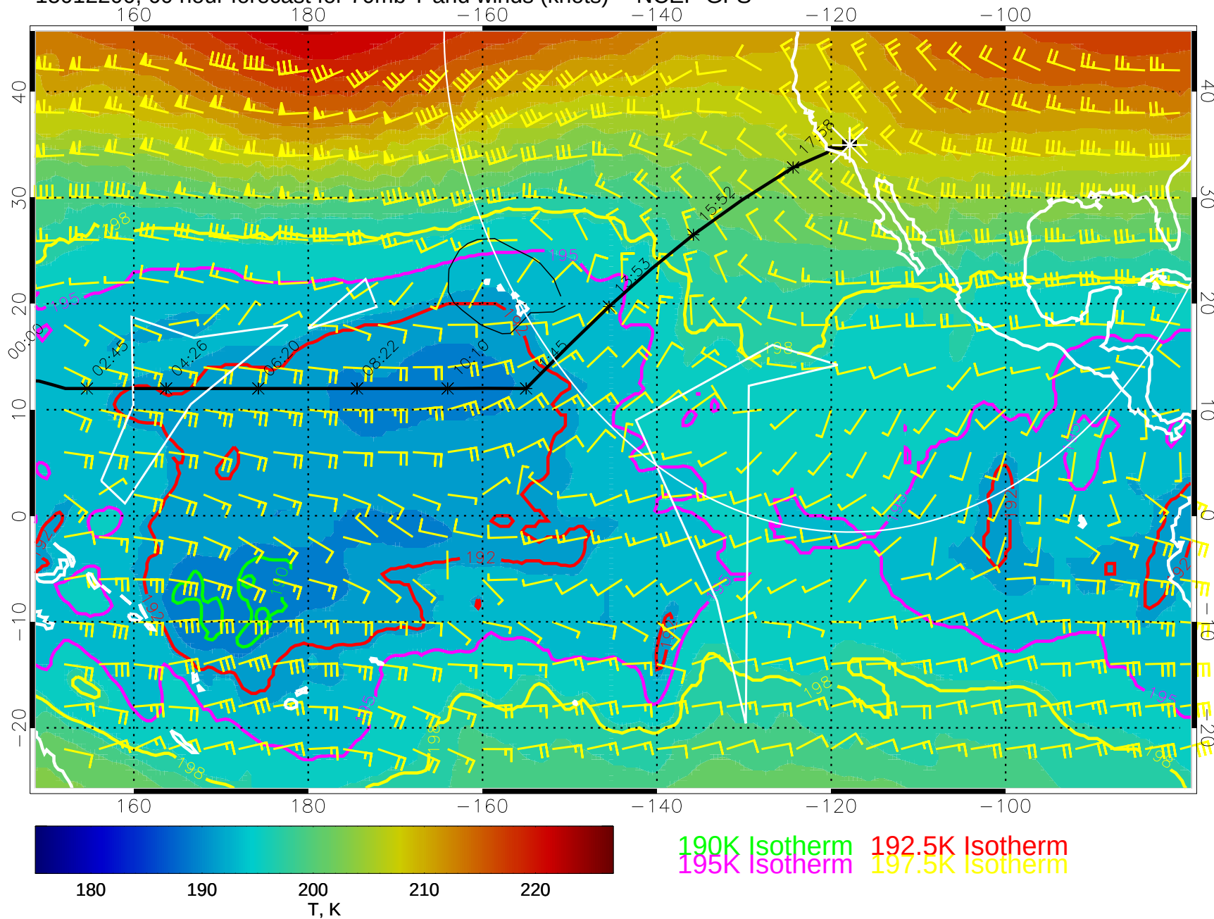
15012200, 60 hour forecast for 70mb T and winds (knots) -- NCEP GFS
