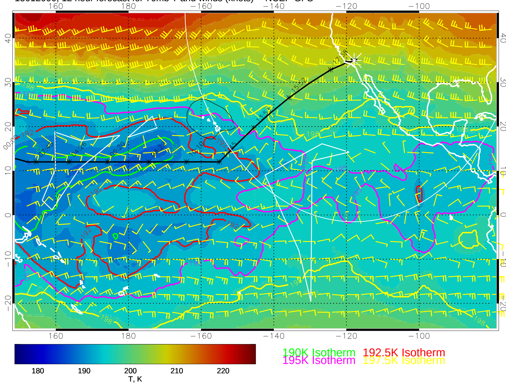
15012000, 12 hour forecast for 70mb T and winds (knots) -- NCEP GFS
