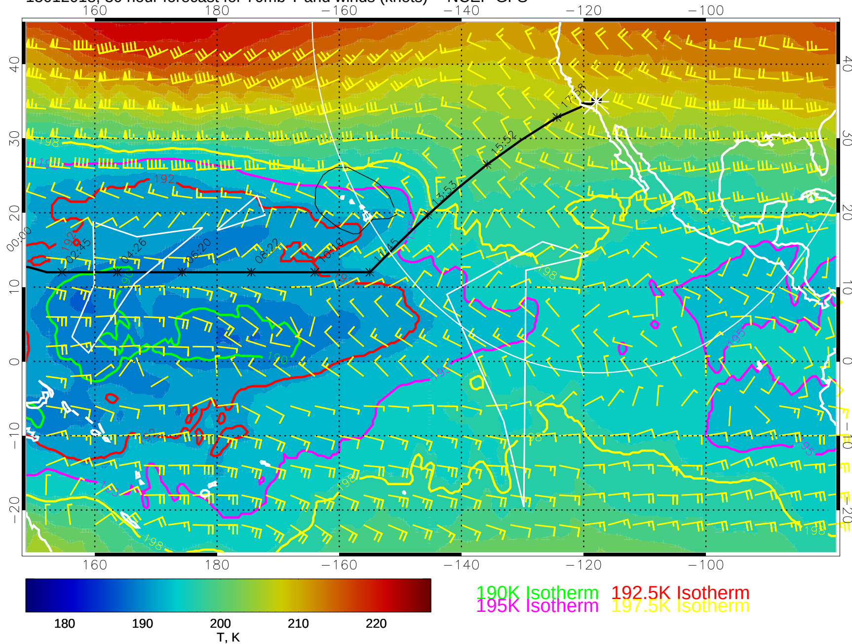
15012018, 30 hour forecast for 70mb T and winds (knots) -- NCEP GFS
