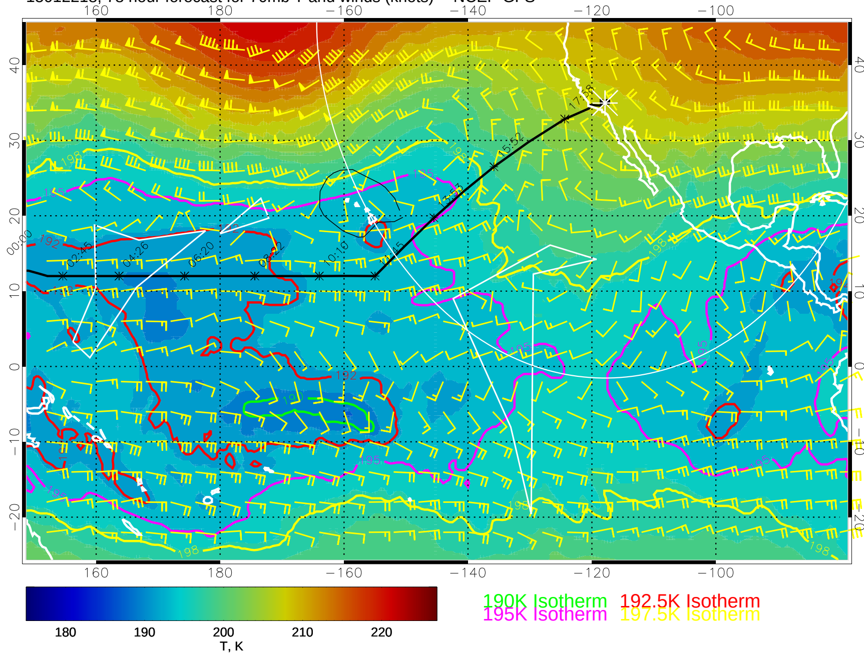
15012218, 78 hour forecast for 70mb T and winds (knots) -- NCEP GFS
