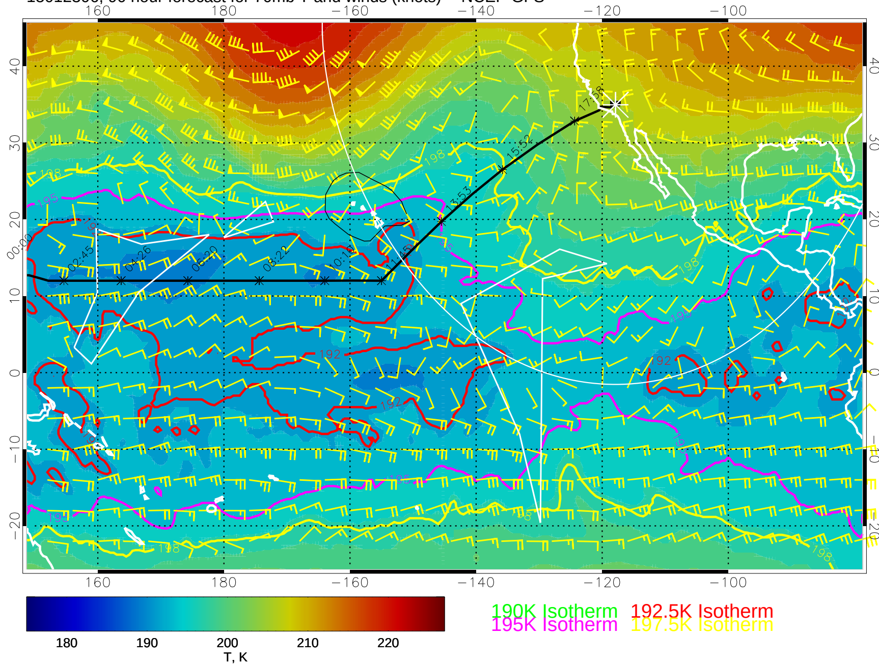
15012306, 90 hour forecast for 70mb T and winds (knots) -- NCEP GFS
