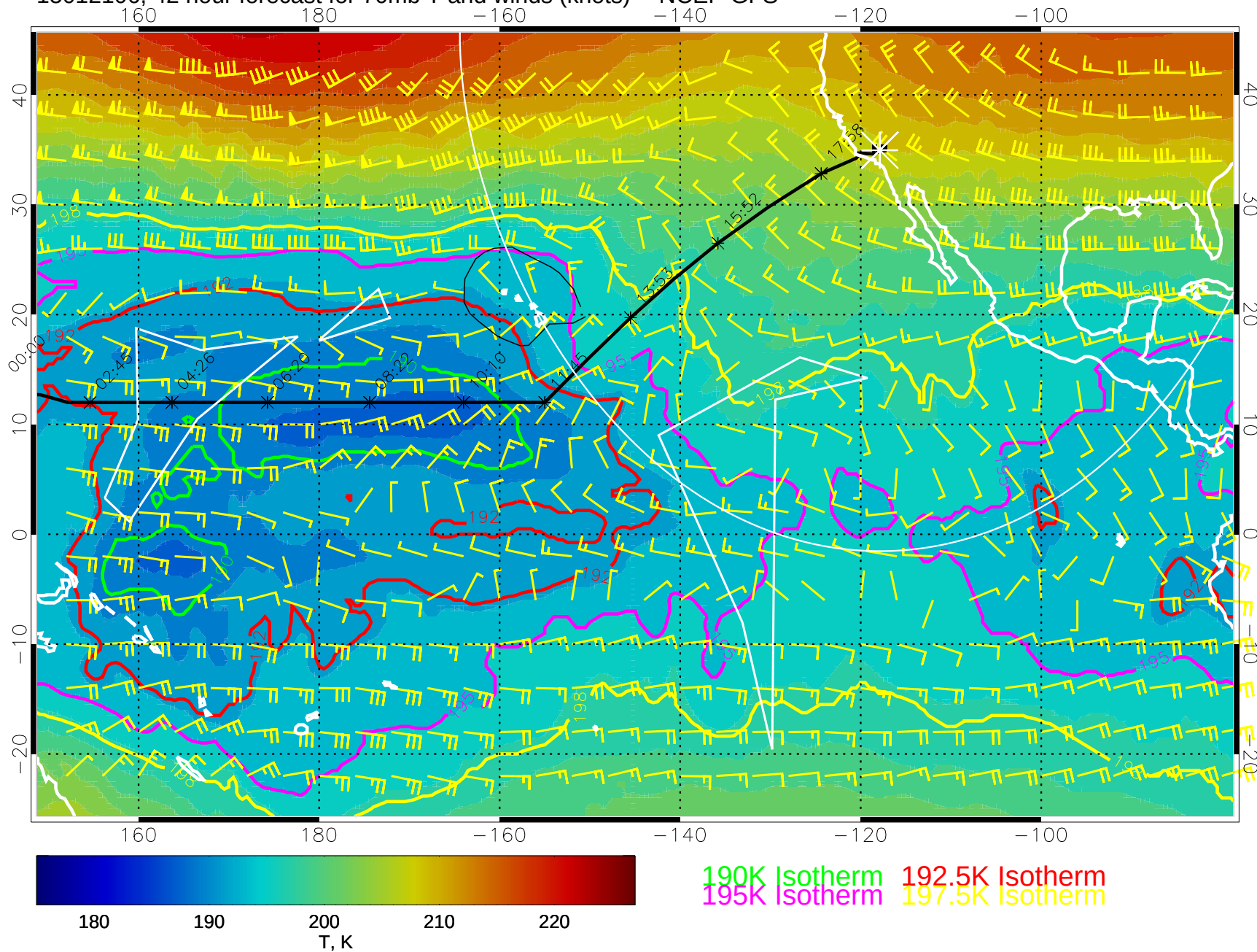
15012106, 42 hour forecast for 70mb T and winds (knots) -- NCEP GFS
