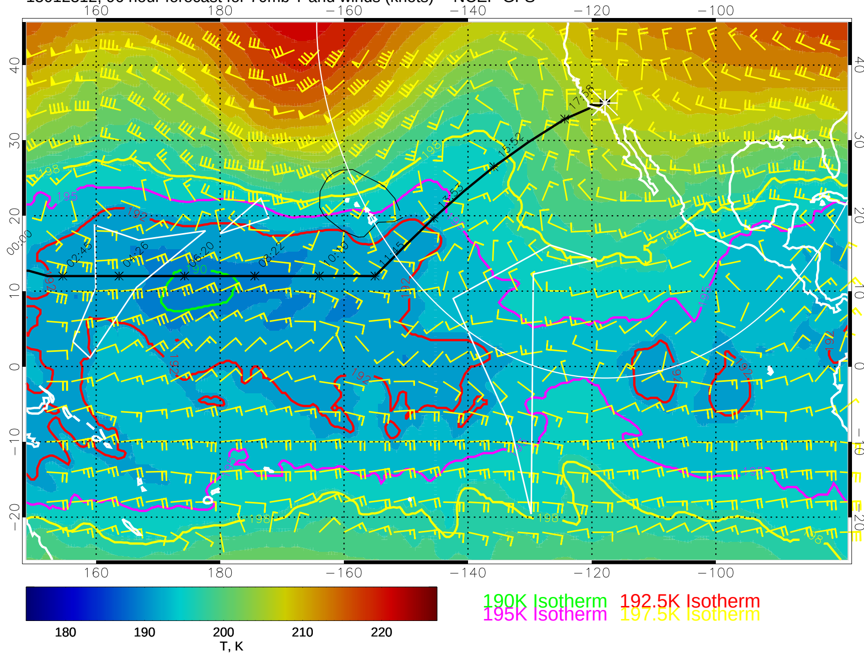
15012312, 96 hour forecast for 70mb T and winds (knots) -- NCEP GFS
