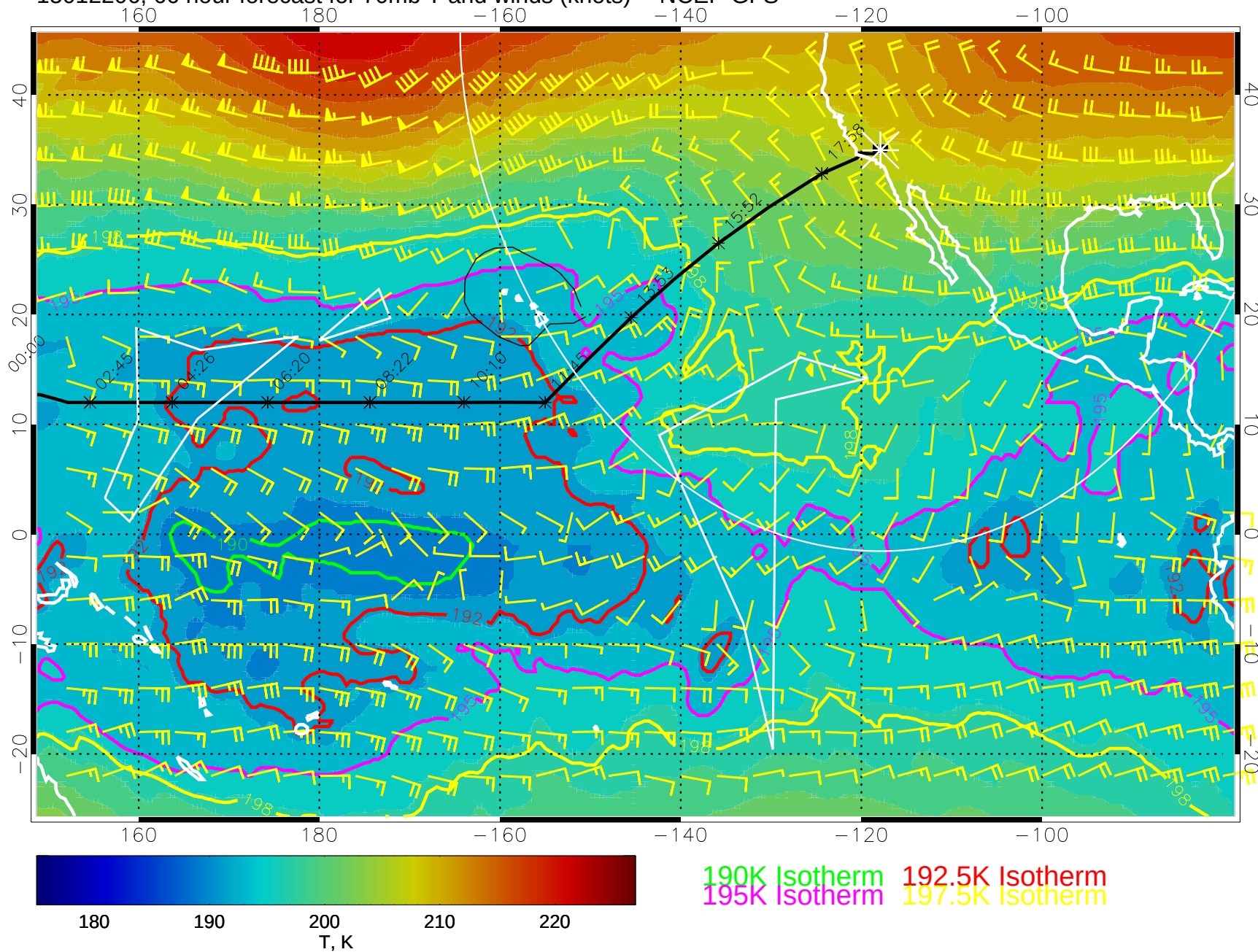
15012206, 66 hour forecast for 70mb T and winds (knots) -- NCEP GFS
