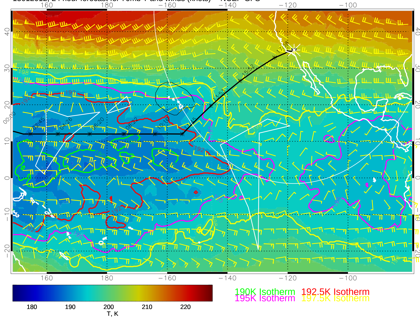
15012012, 24 hour forecast for 70mb T and winds (knots) -- NCEP GFS
