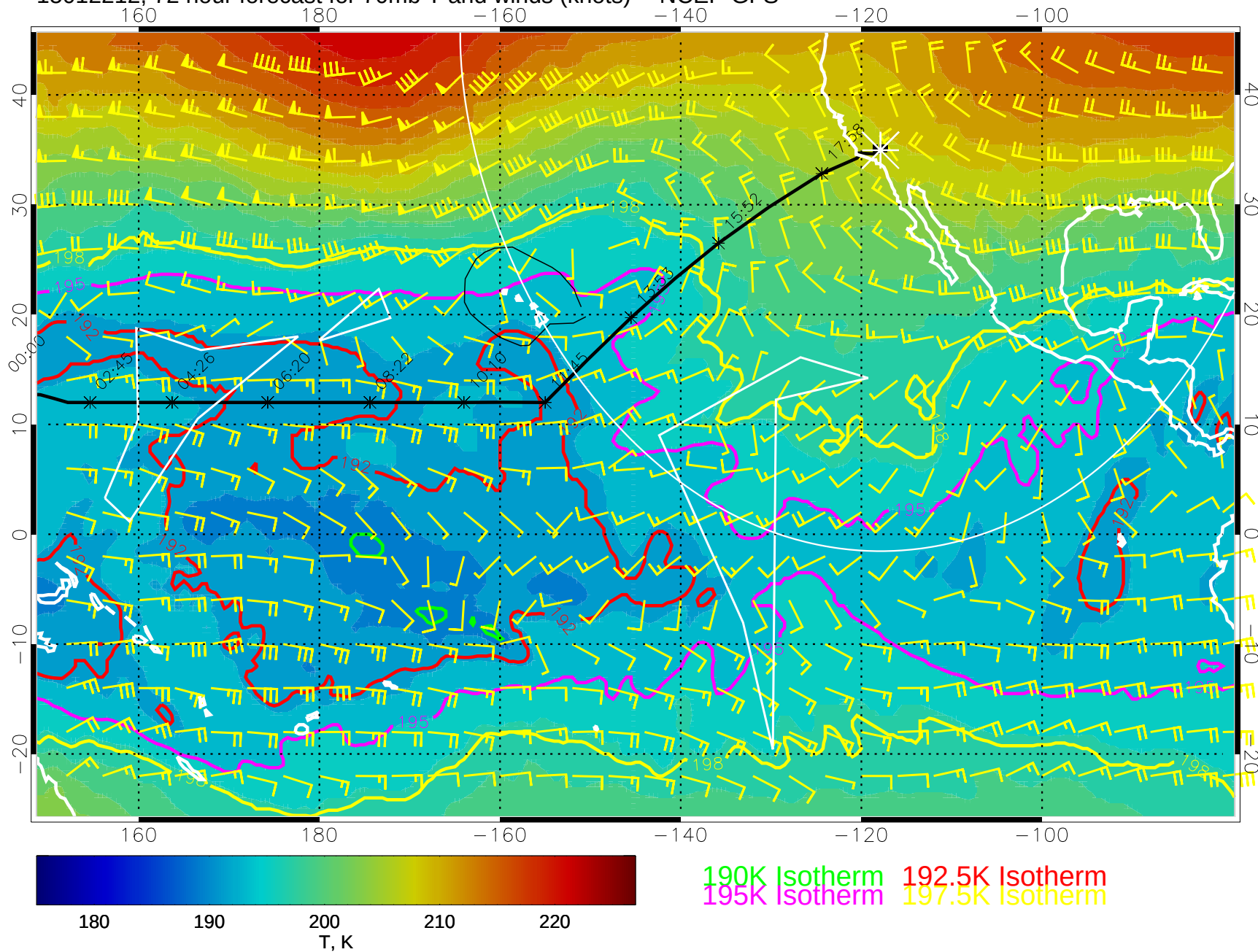
15012212, 72 hour forecast for 70mb T and winds (knots) -- NCEP GFS
