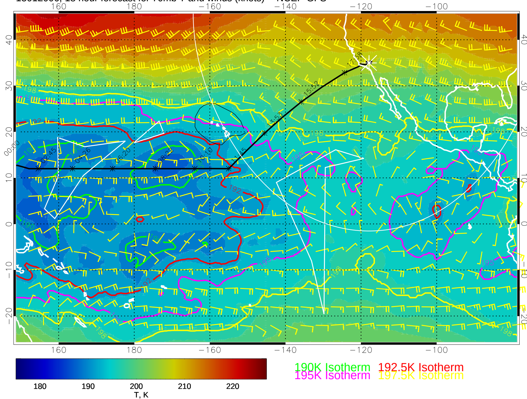
15012006, 18 hour forecast for 70mb T and winds (knots) -- NCEP GFS
