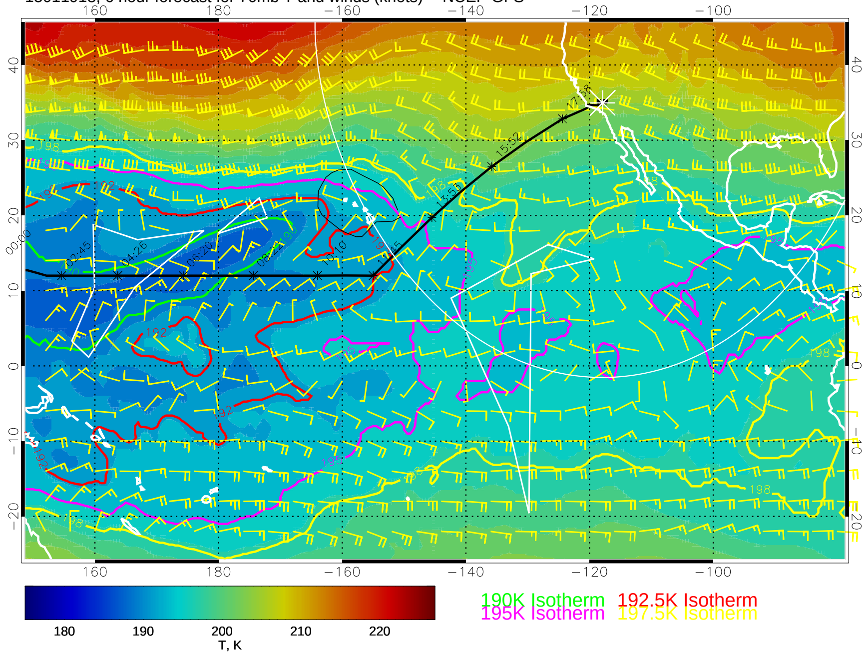
15011918, 6 hour forecast for 70mb T and winds (knots) -- NCEP GFS
