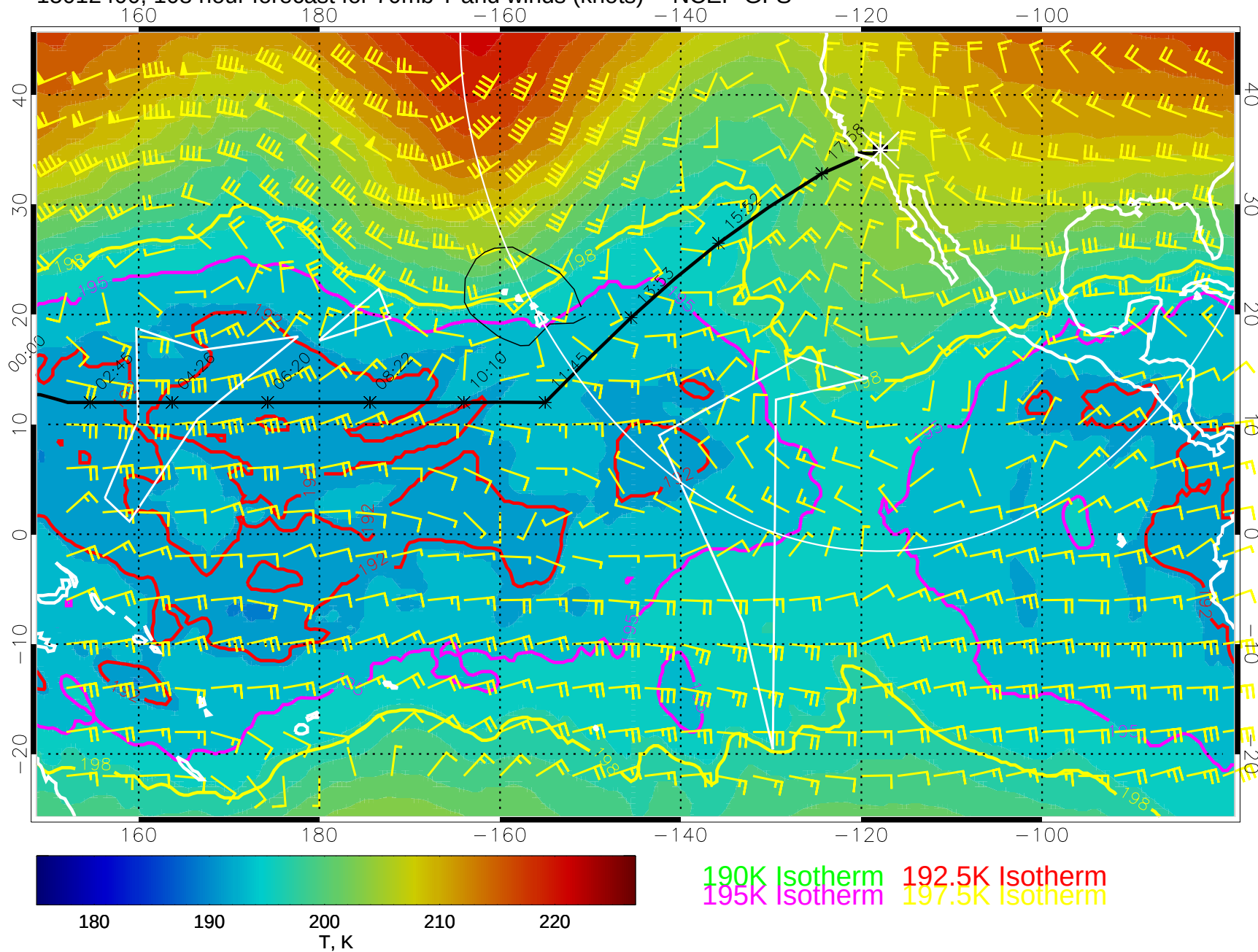
15012400, 108 hour forecast for 70mb T and winds (knots) -- NCEP GFS
