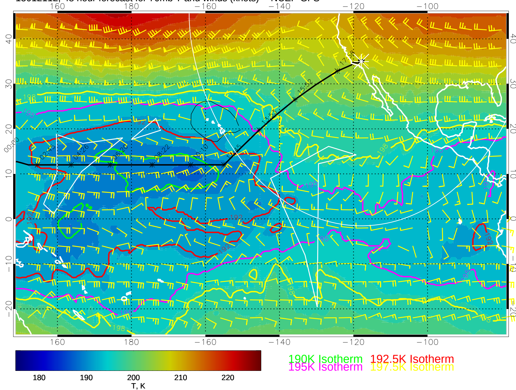
15012112, 48 hour forecast for 70mb T and winds (knots) -- NCEP GFS
