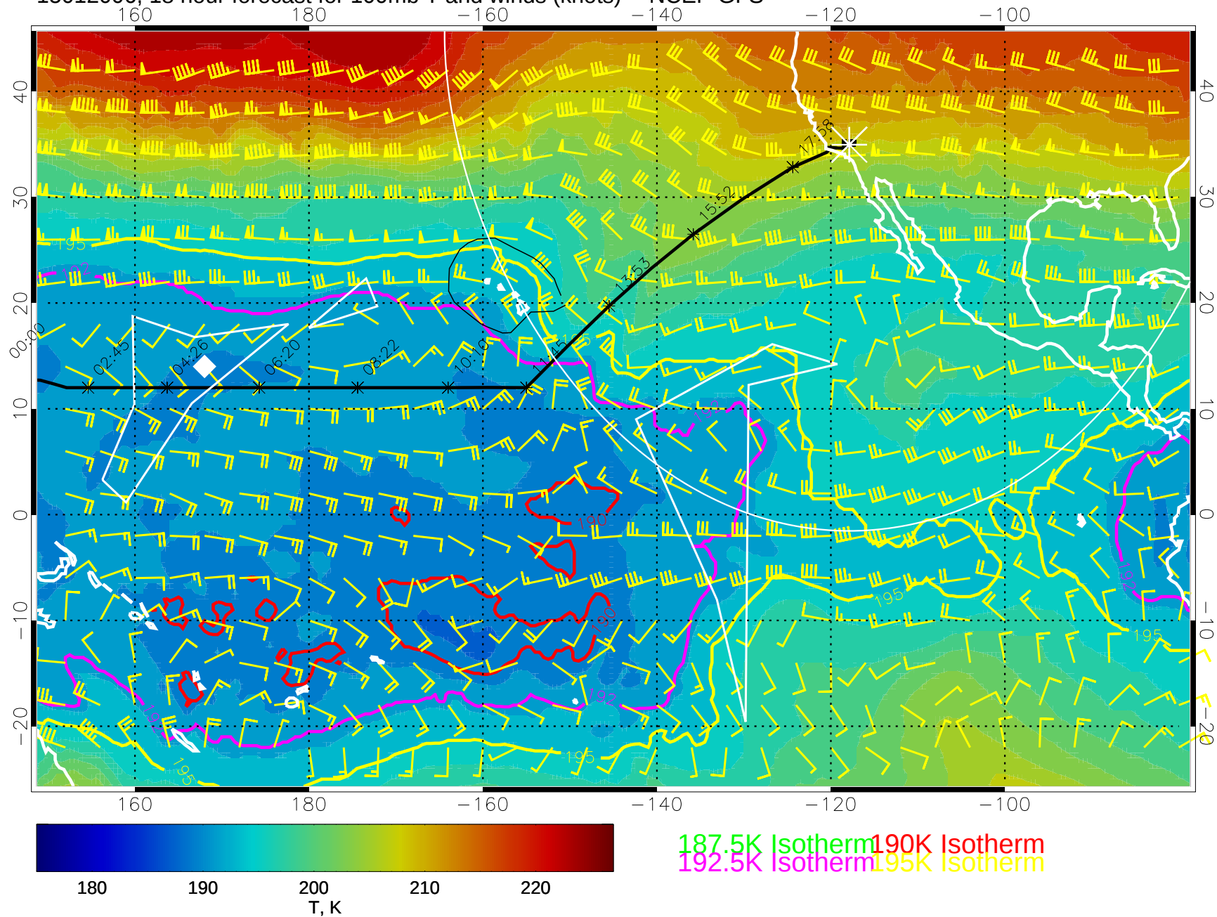
15012006, 18 hour forecast for 100mb T and winds (knots) -- NCEP GFS
