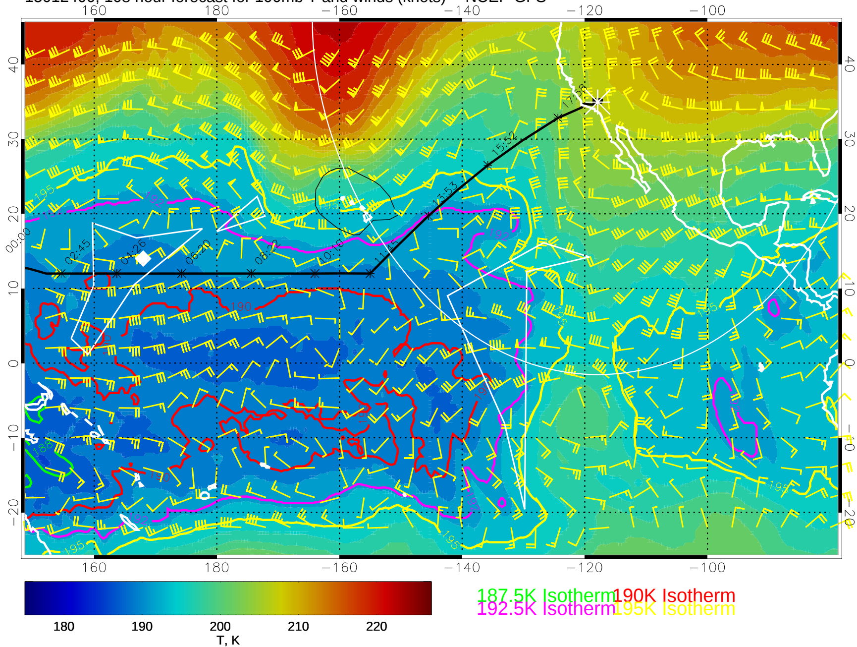
15012400, 108 hour forecast for 100mb T and winds (knots) -- NCEP GFS
