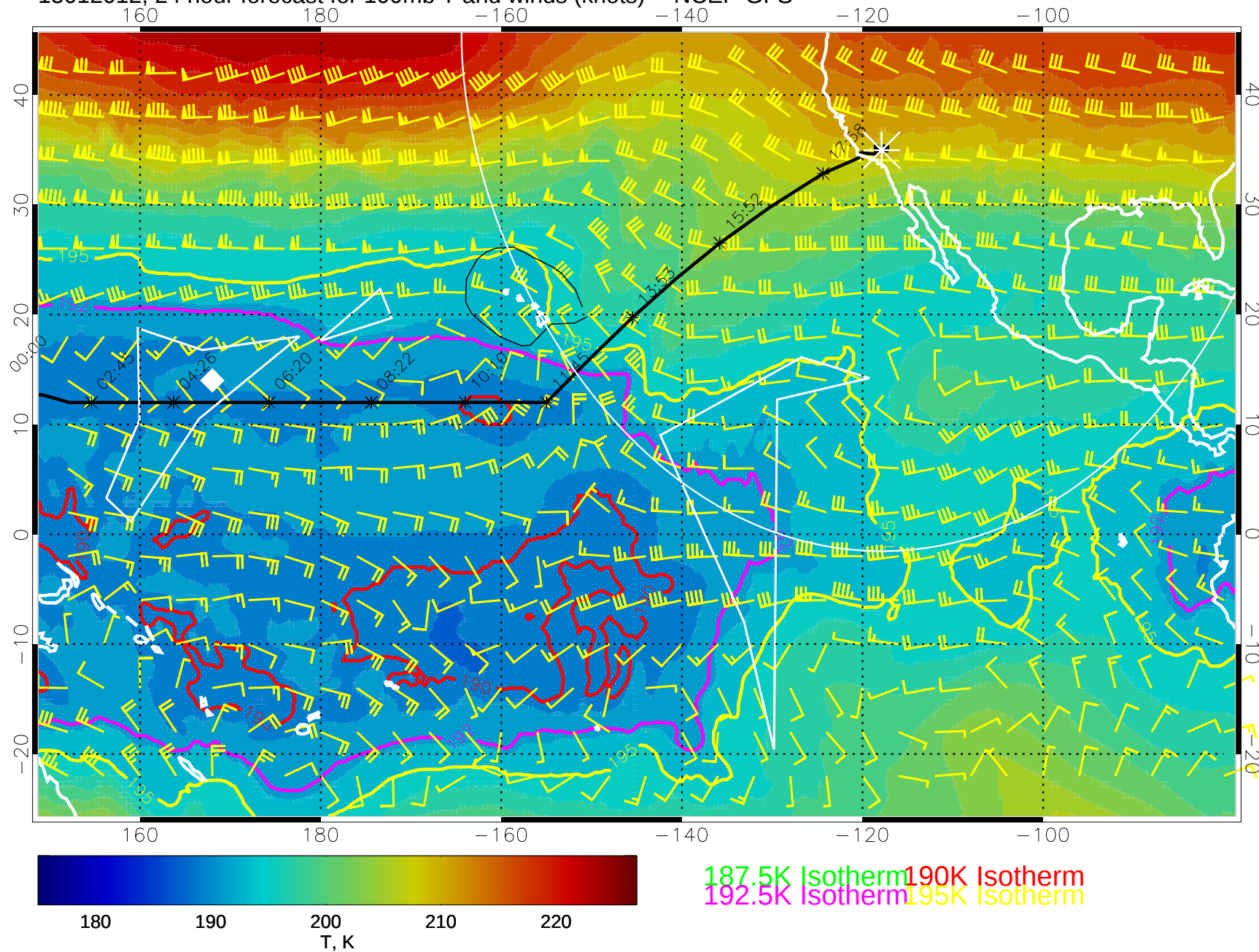
15012012, 24 hour forecast for 100mb T and winds (knots) -- NCEP GFS
