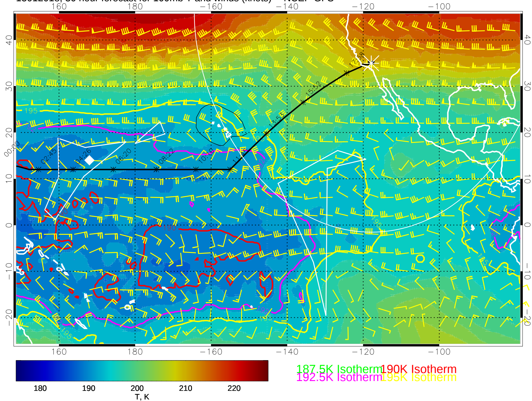
15012018, 30 hour forecast for 100mb T and winds (knots) -- NCEP GFS
