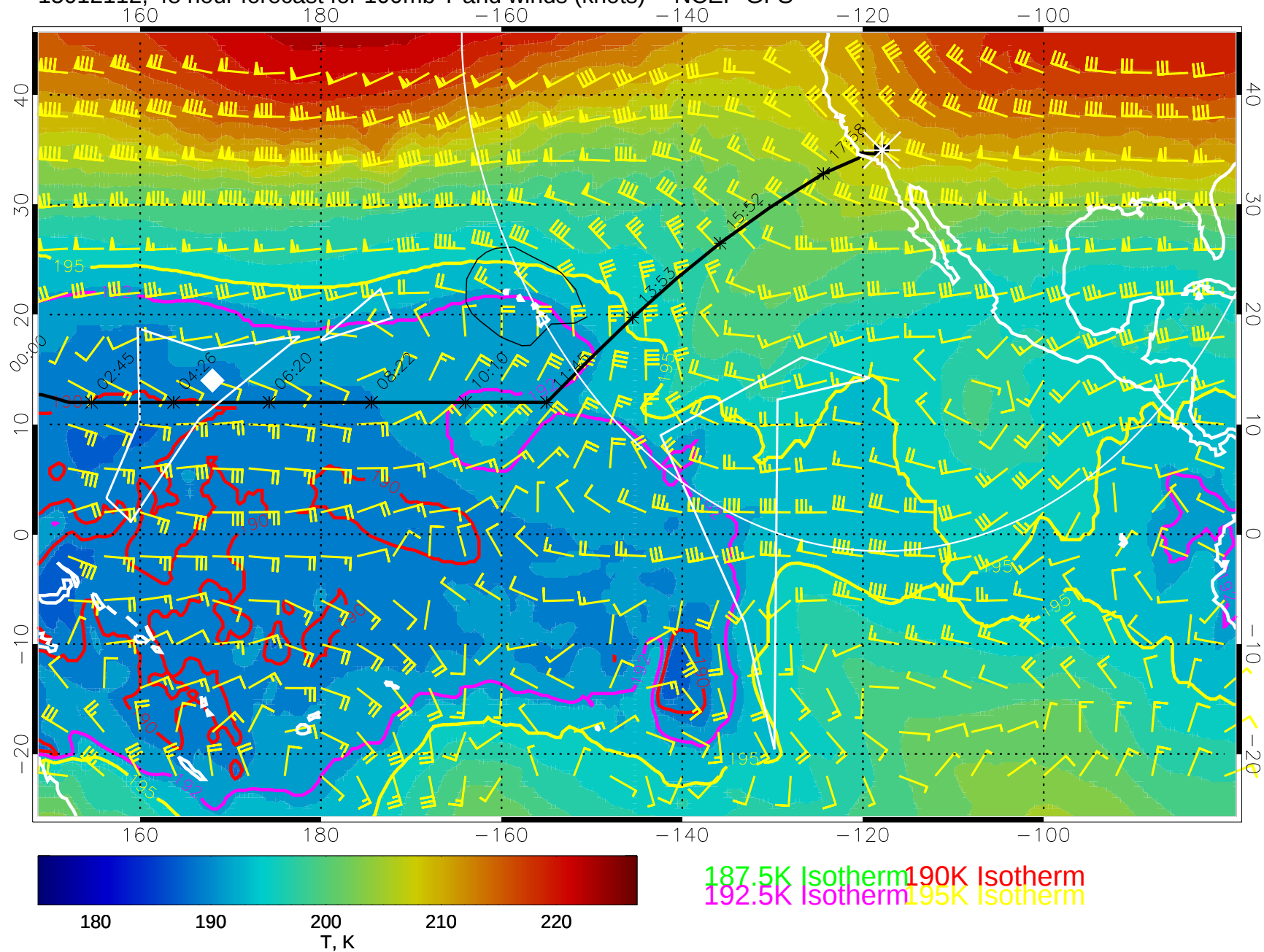
15012112, 48 hour forecast for 100mb T and winds (knots) -- NCEP GFS
