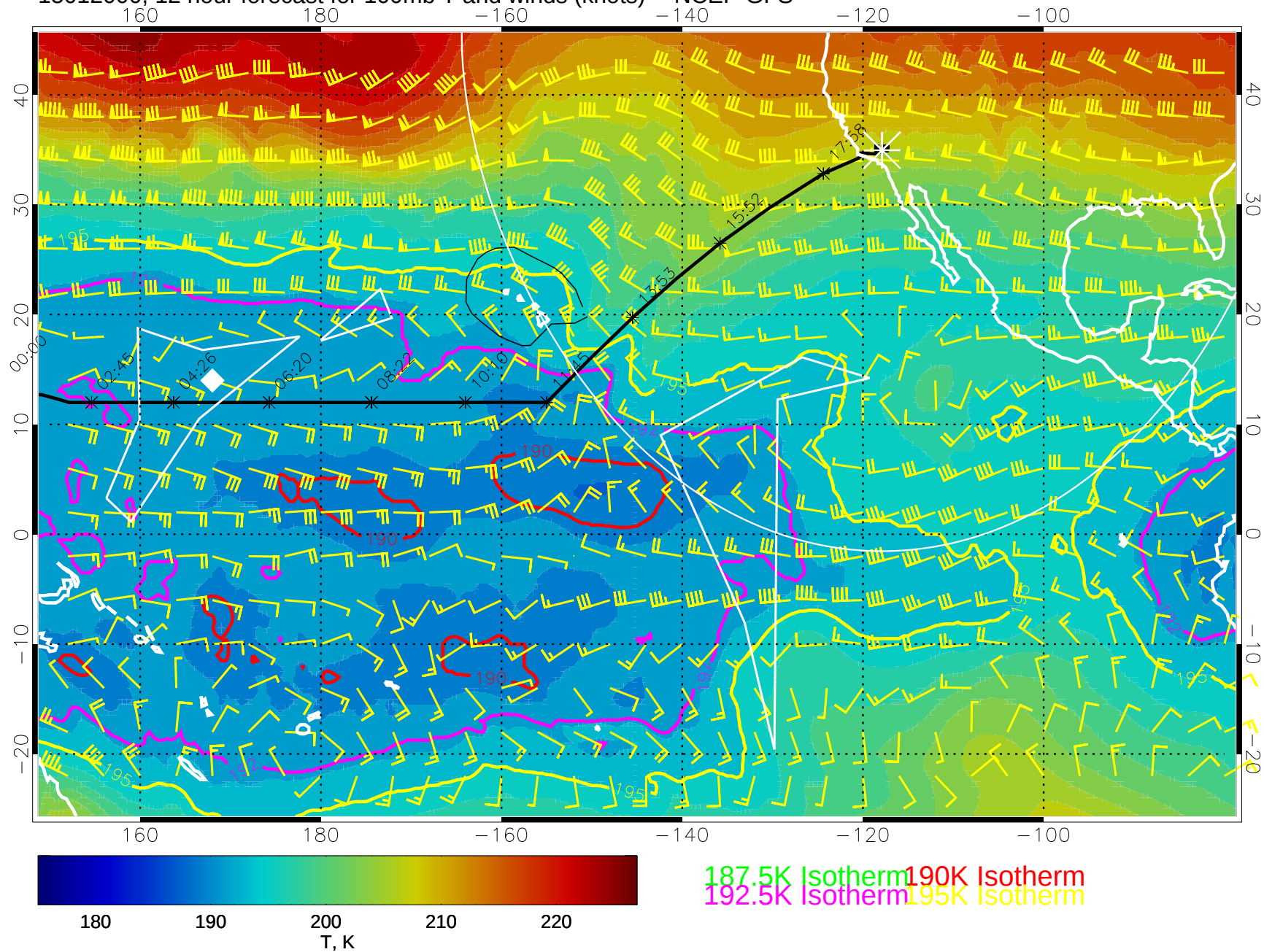
15012000, 12 hour forecast for 100mb T and winds (knots) -- NCEP GFS
