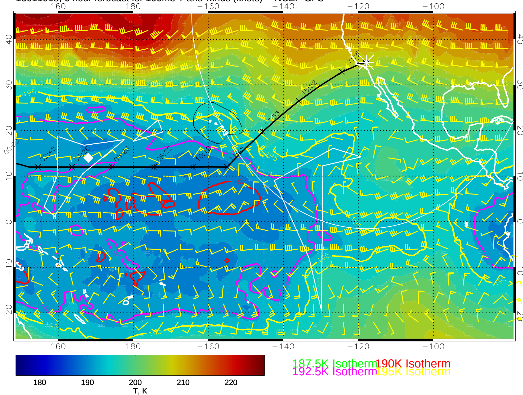
15011918, 6 hour forecast for 100mb T and winds (knots) -- NCEP GFS
