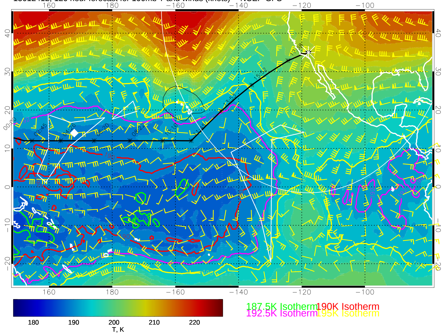
15012412, 120 hour forecast for 100mb T and winds (knots) -- NCEP GFS
