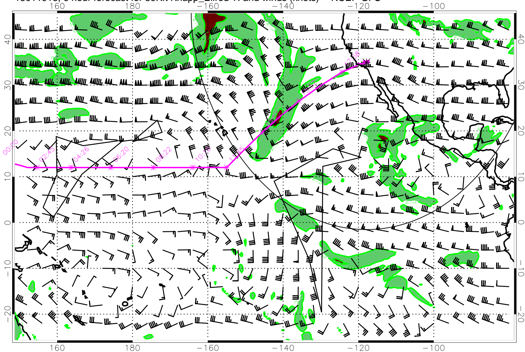
15011918, 6 hour forecast for 39Kft Knapp_Ellrod TI and winds (knots) -- NCEP GFS
