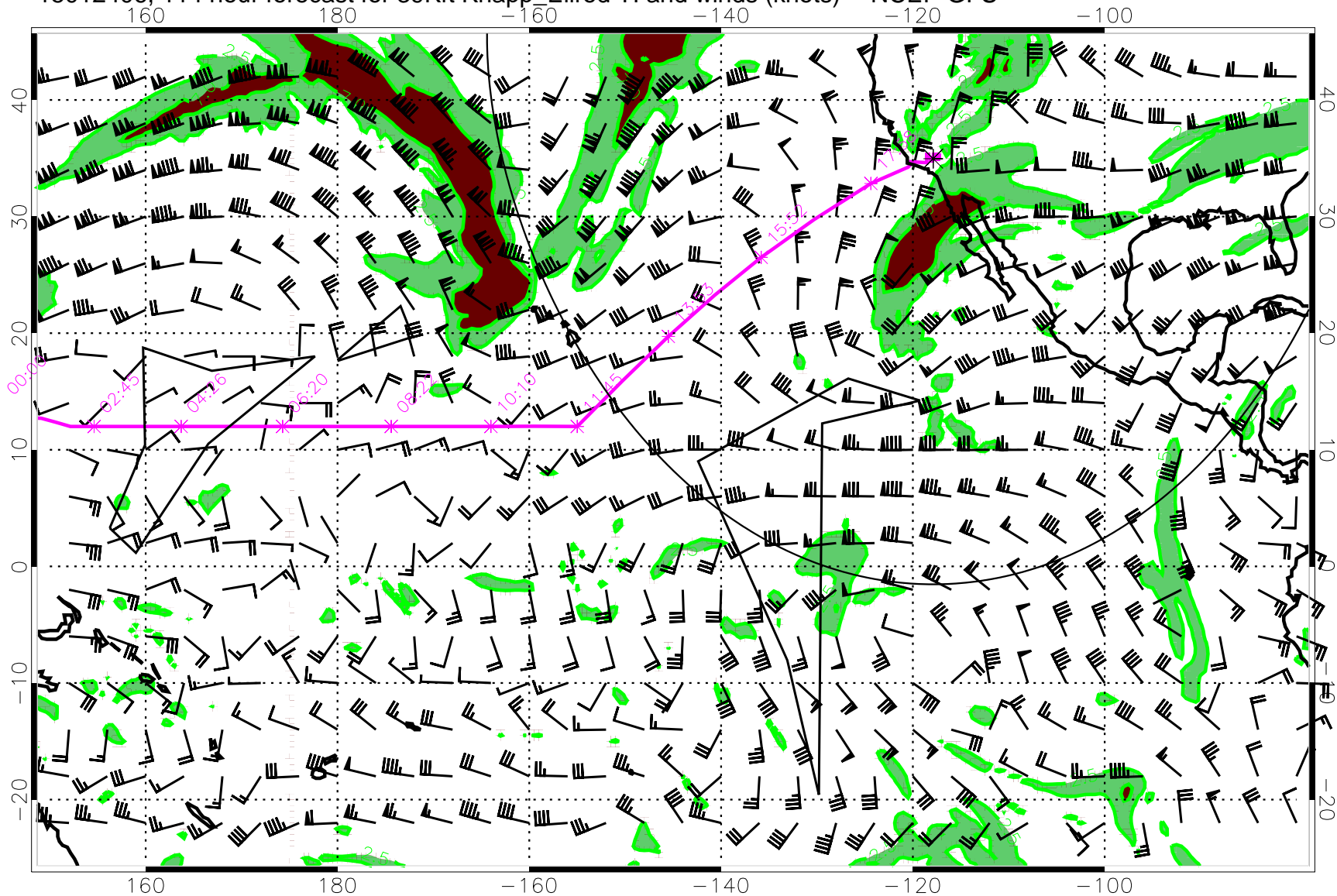
15012406, 114 hour forecast for 39Kft Knapp_Ellrod TI and winds (knots) -- NCEP GFS
