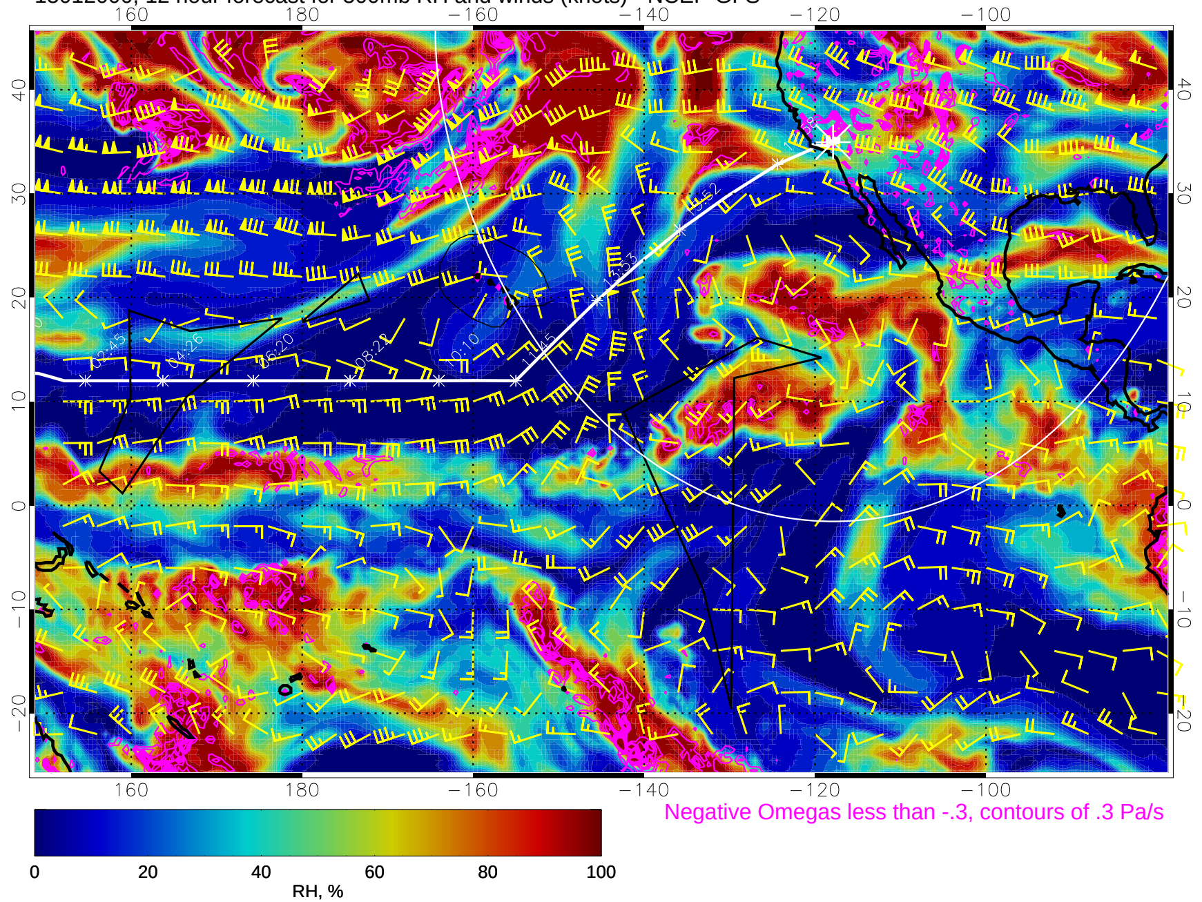
15012000, 12 hour forecast for 500mb RH and winds (knots) - NCEP GFS
