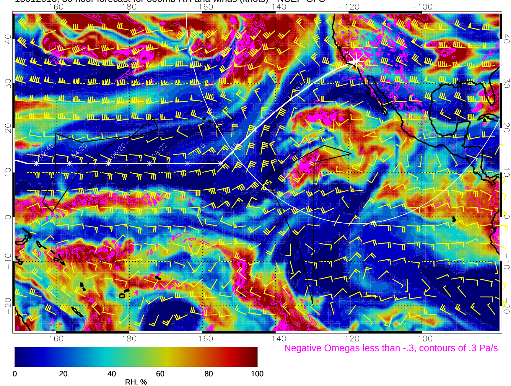
15012018, 30 hour forecast for 500mb RH and winds (knots) - NCEP GFS
