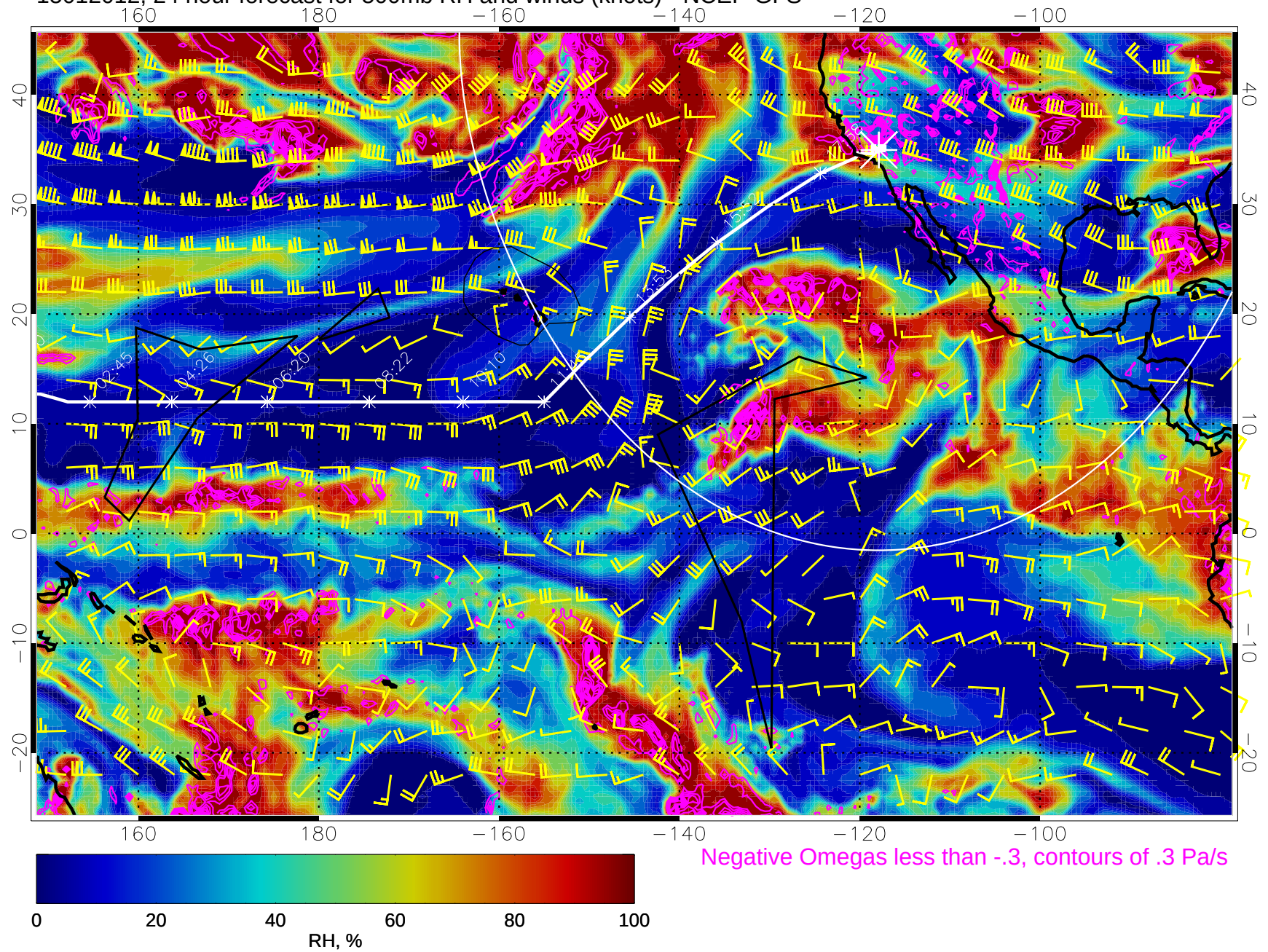
15012012, 24 hour forecast for 500mb RH and winds (knots) - NCEP GFS
