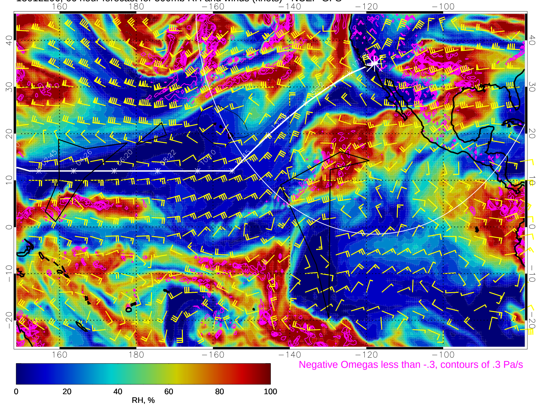
15012206, 66 hour forecast for 500mb RH and winds (knots) - NCEP GFS
