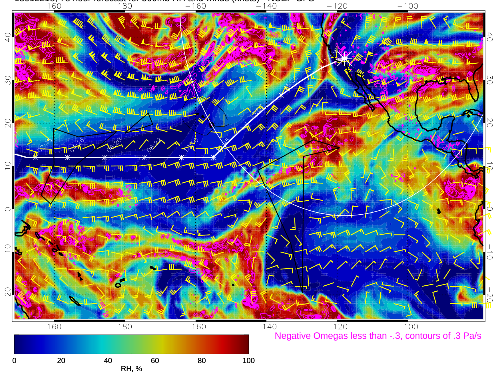
15012218, 78 hour forecast for 500mb RH and winds (knots) - NCEP GFS
