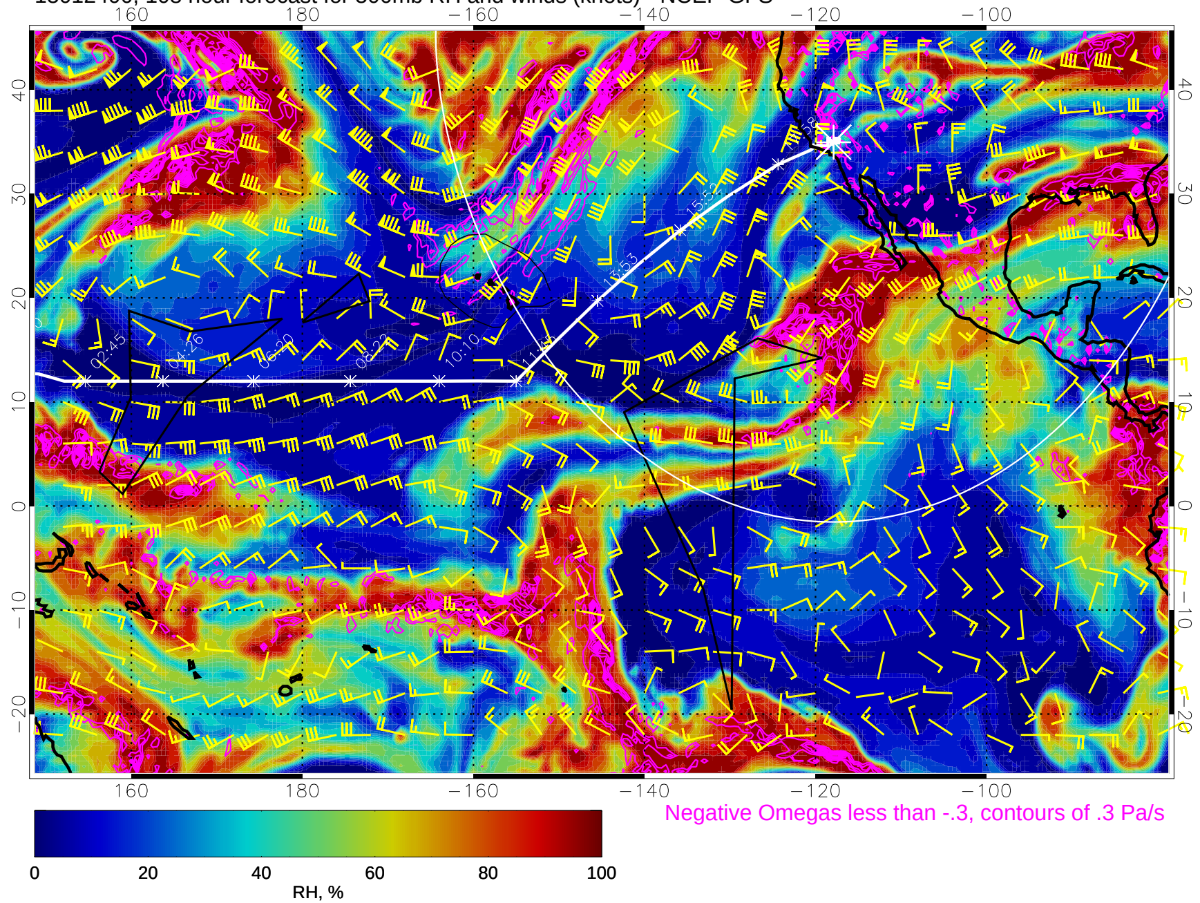
15012400, 108 hour forecast for 500mb RH and winds (knots) - NCEP GFS
