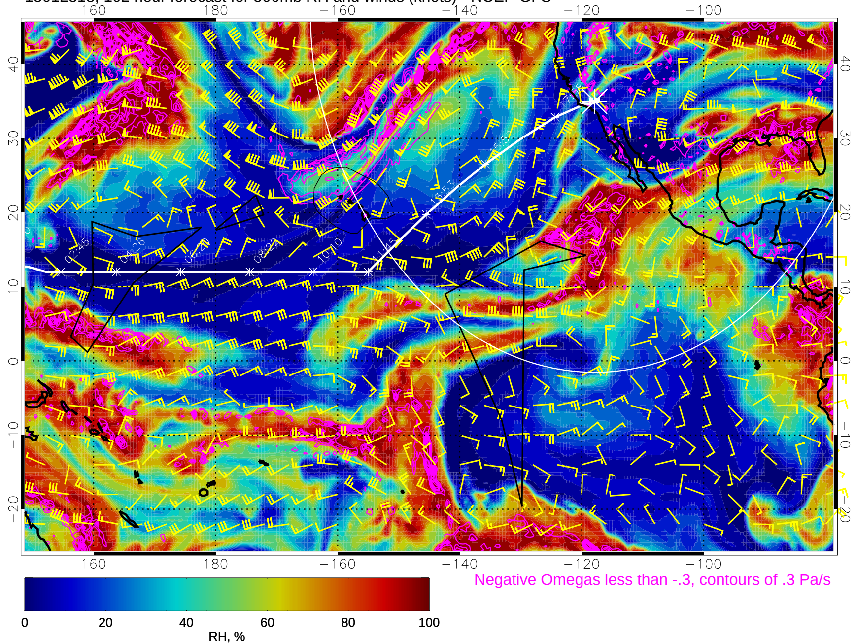
15012318, 102 hour forecast for 500mb RH and winds (knots) - NCEP GFS
