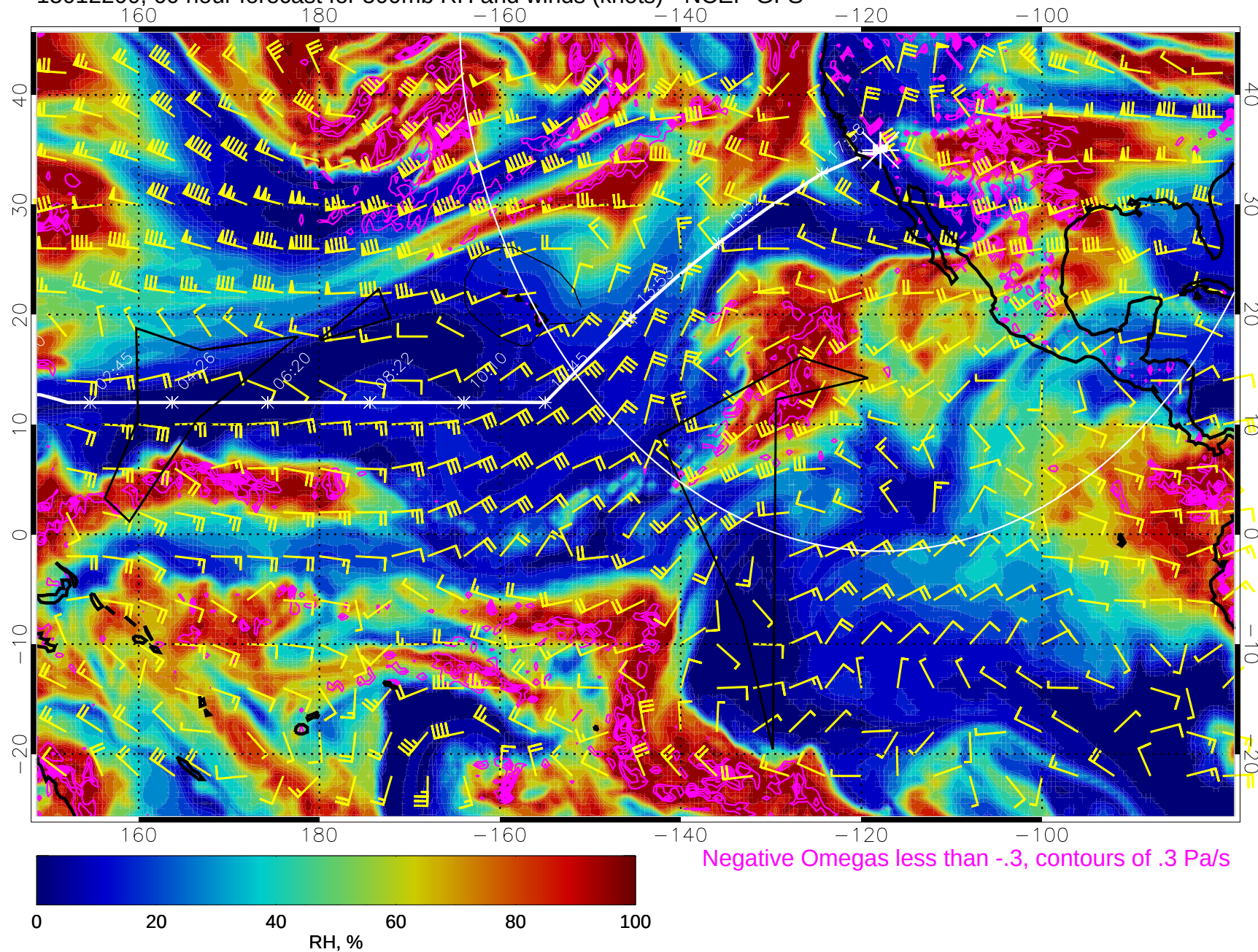
15012200, 60 hour forecast for 500mb RH and winds (knots) - NCEP GFS
