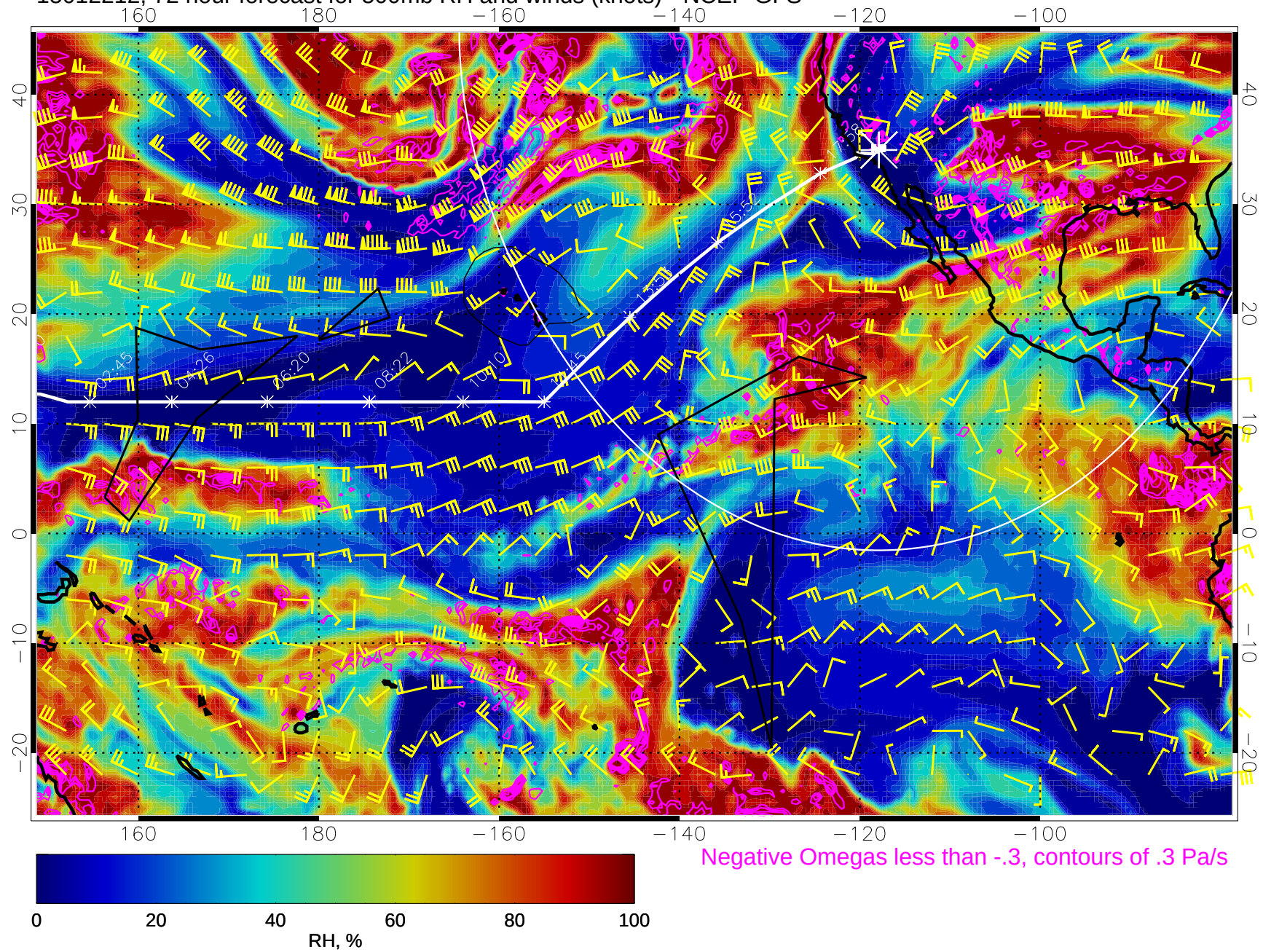
15012212, 72 hour forecast for 500mb RH and winds (knots) - NCEP GFS
