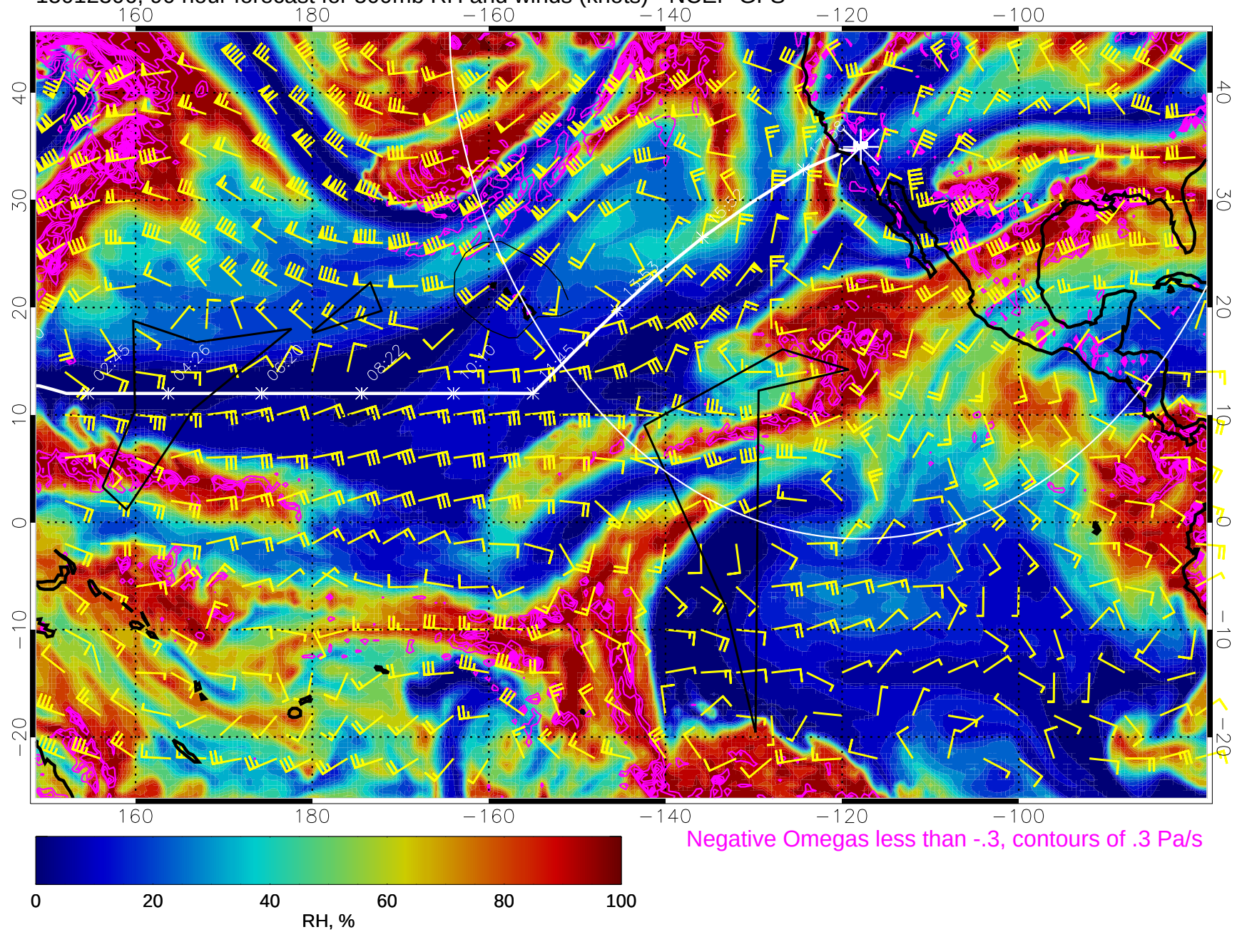
15012306, 90 hour forecast for 500mb RH and winds (knots) - NCEP GFS
