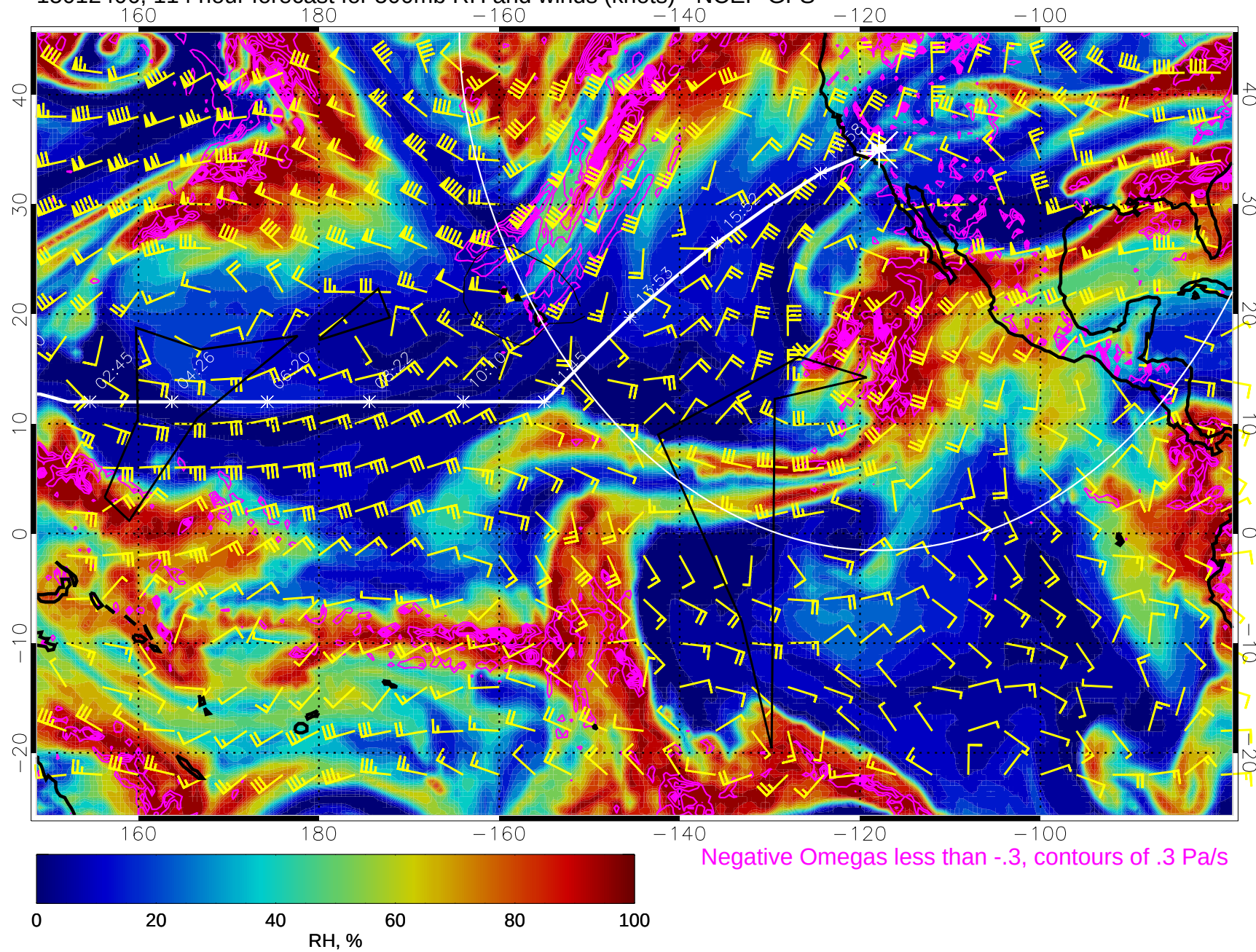
15012406, 114 hour forecast for 500mb RH and winds (knots) - NCEP GFS
