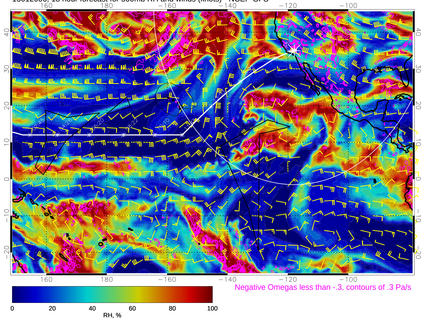
15012006, 18 hour forecast for 500mb RH and winds (knots) - NCEP GFS
