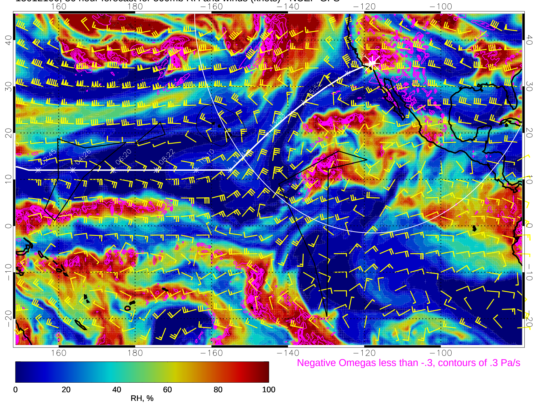
15012100, 36 hour forecast for 500mb RH and winds (knots) - NCEP GFS
