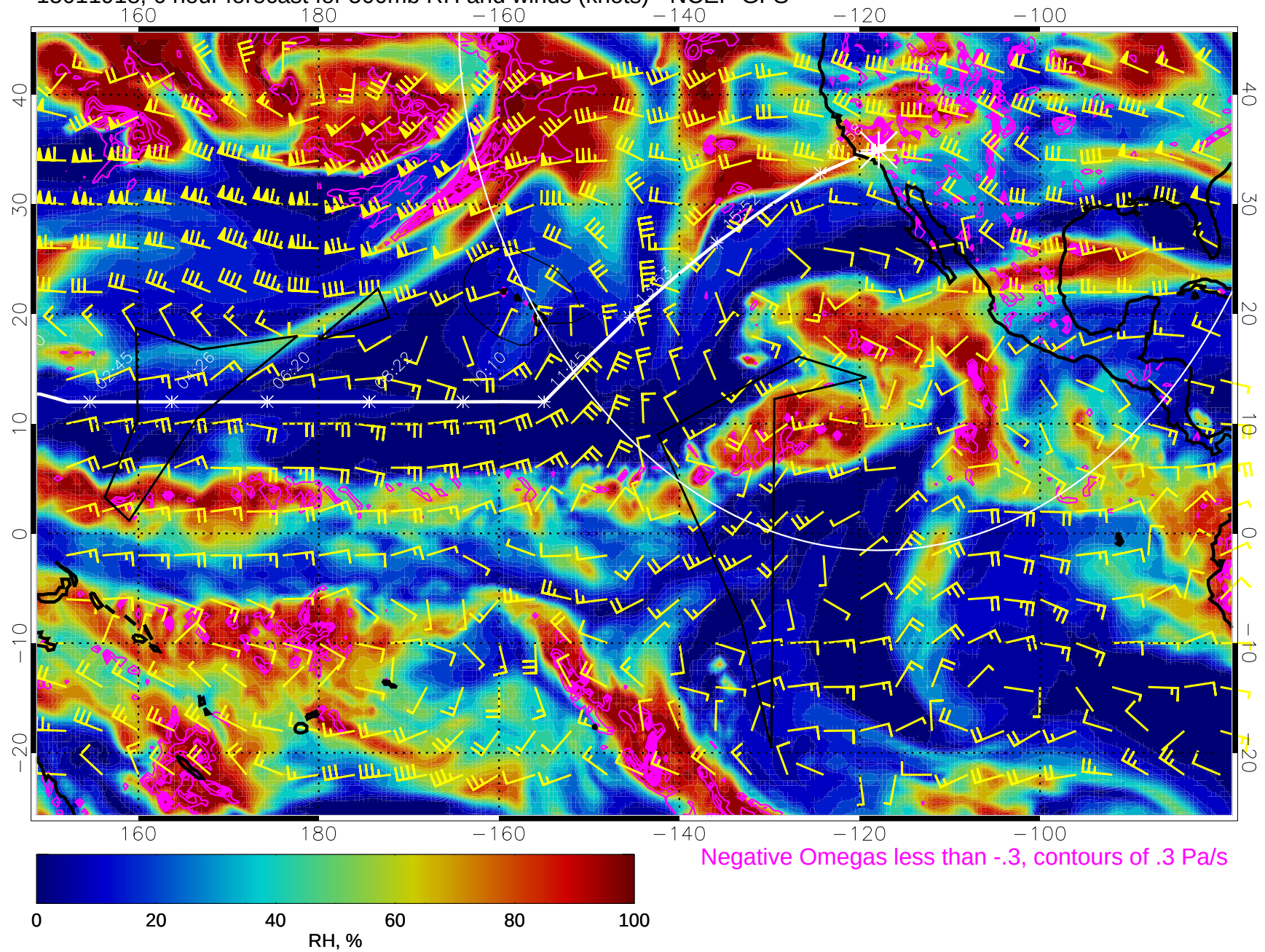
15011918, 6 hour forecast for 500mb RH and winds (knots) - NCEP GFS
