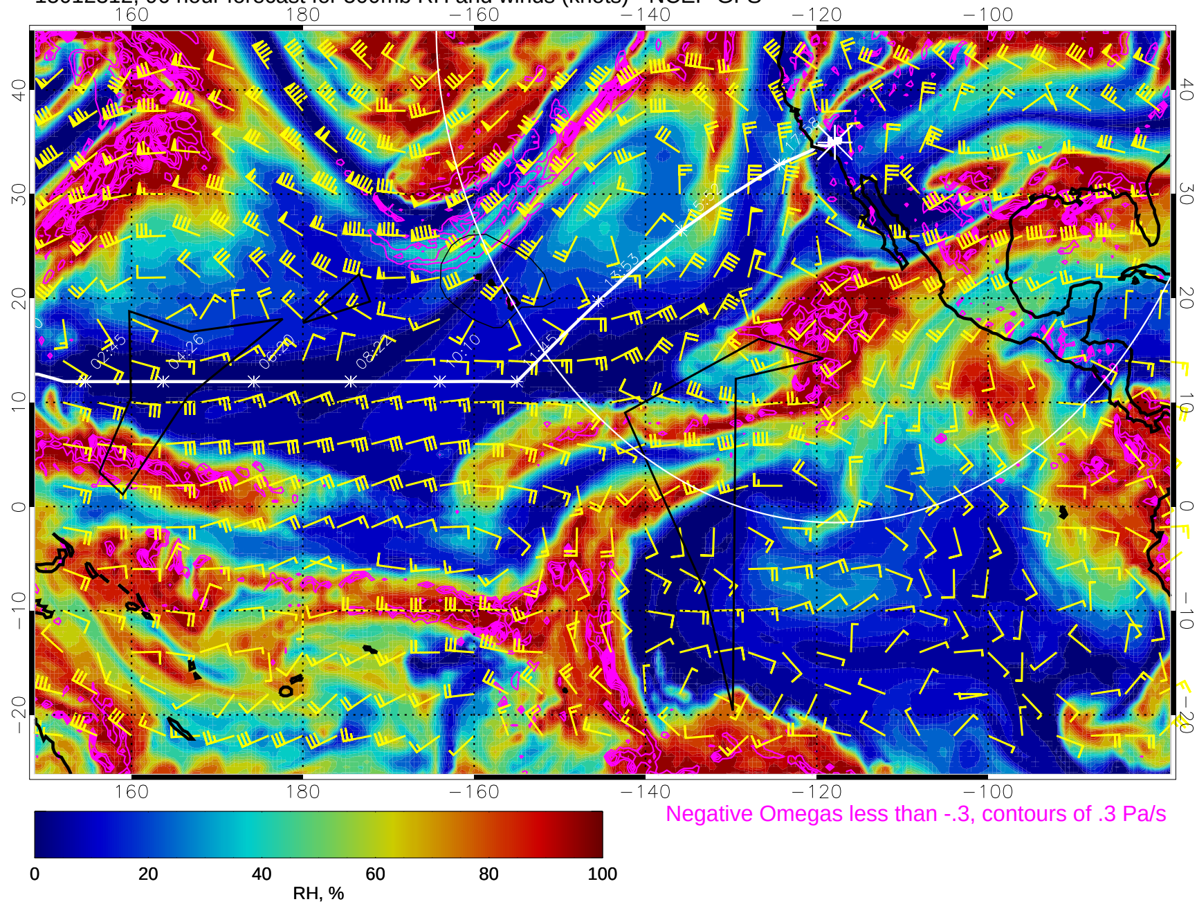
15012312, 96 hour forecast for 500mb RH and winds (knots) - NCEP GFS
