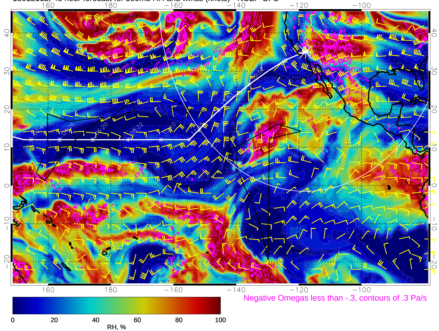
15012112, 48 hour forecast for 500mb RH and winds (knots) - NCEP GFS
