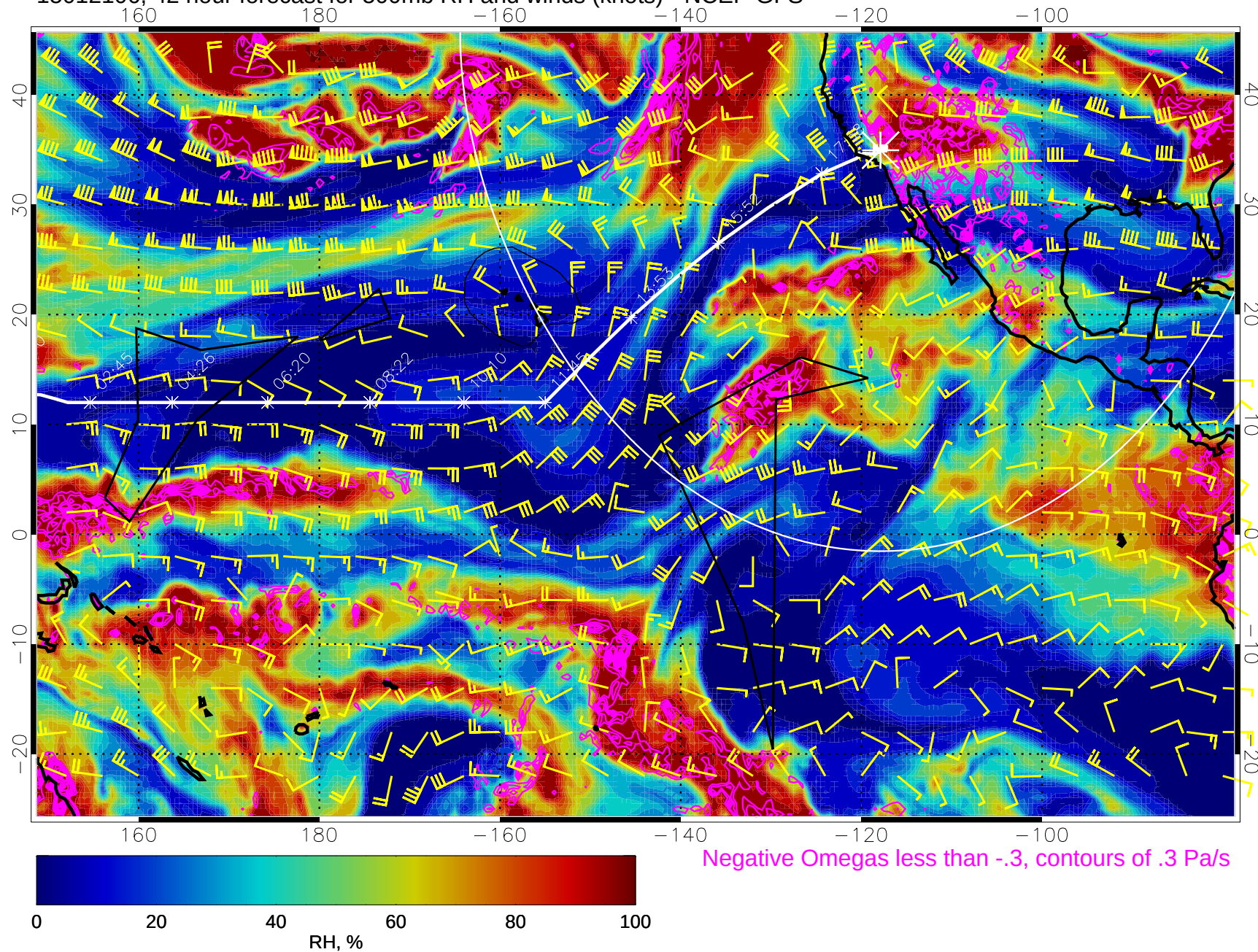
15012106, 42 hour forecast for 500mb RH and winds (knots) - NCEP GFS
