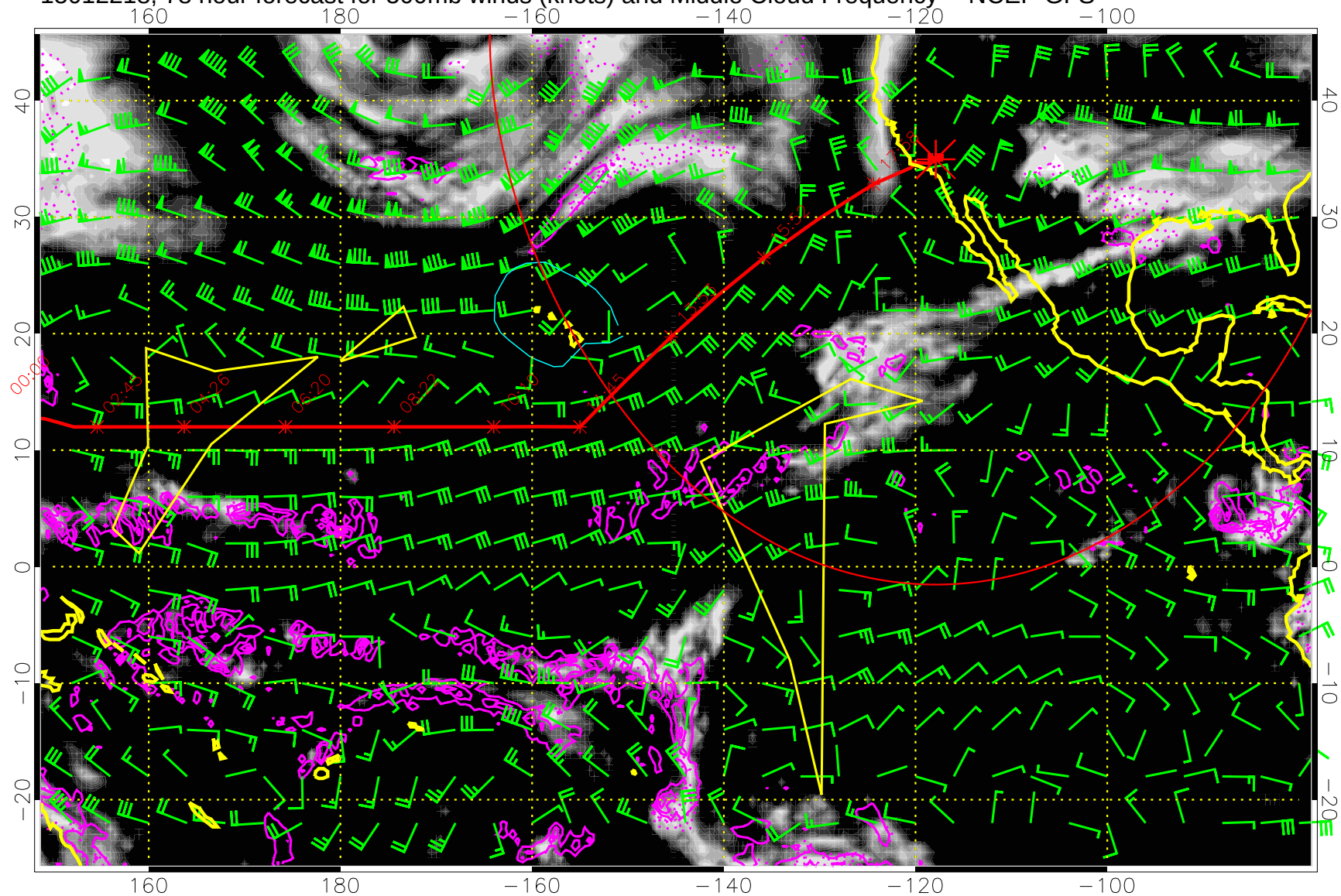
15012218, 78 hour forecast for 500mb winds (knots) and Middle Cloud Frequency -- NCEP GFS
