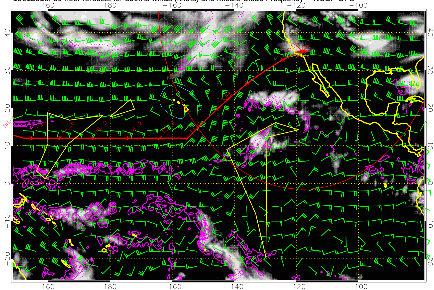
15012018, 30 hour forecast for 500mb winds (knots) and Middle Cloud Frequency -- NCEP GFS
