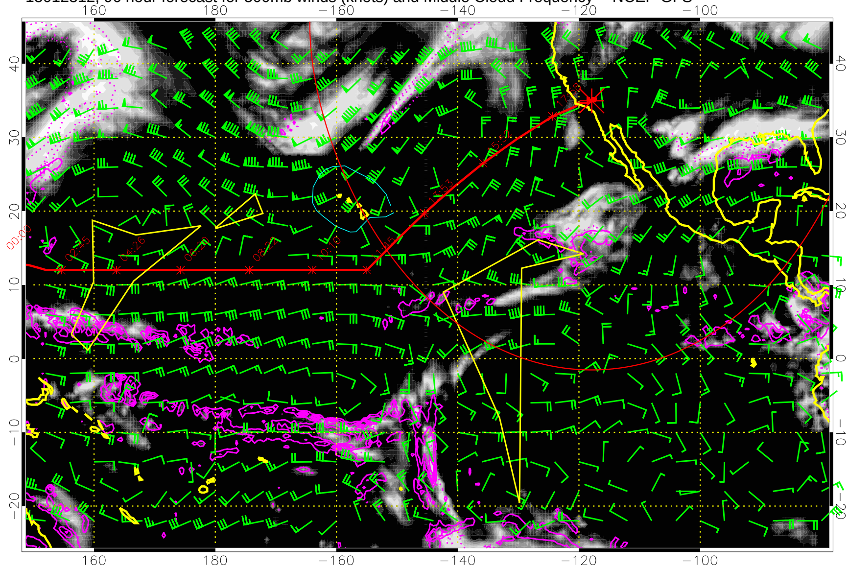
15012312, 96 hour forecast for 500mb winds (knots) and Middle Cloud Frequency -- NCEP GFS
