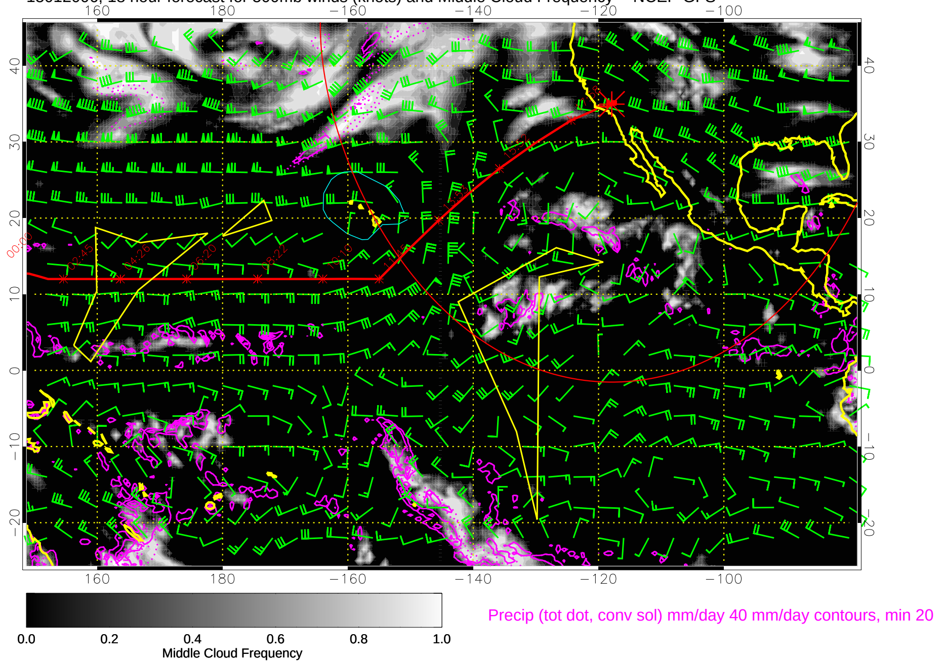
15012006, 18 hour forecast for 500mb winds (knots) and Middle Cloud Frequency -- NCEP GFS
