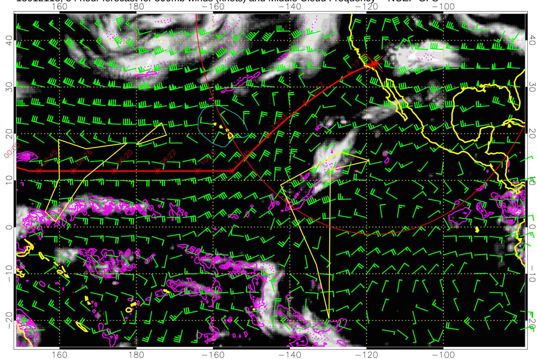
15012118, 54 hour forecast for 500mb winds (knots) and Middle Cloud Frequency -- NCEP GFS
