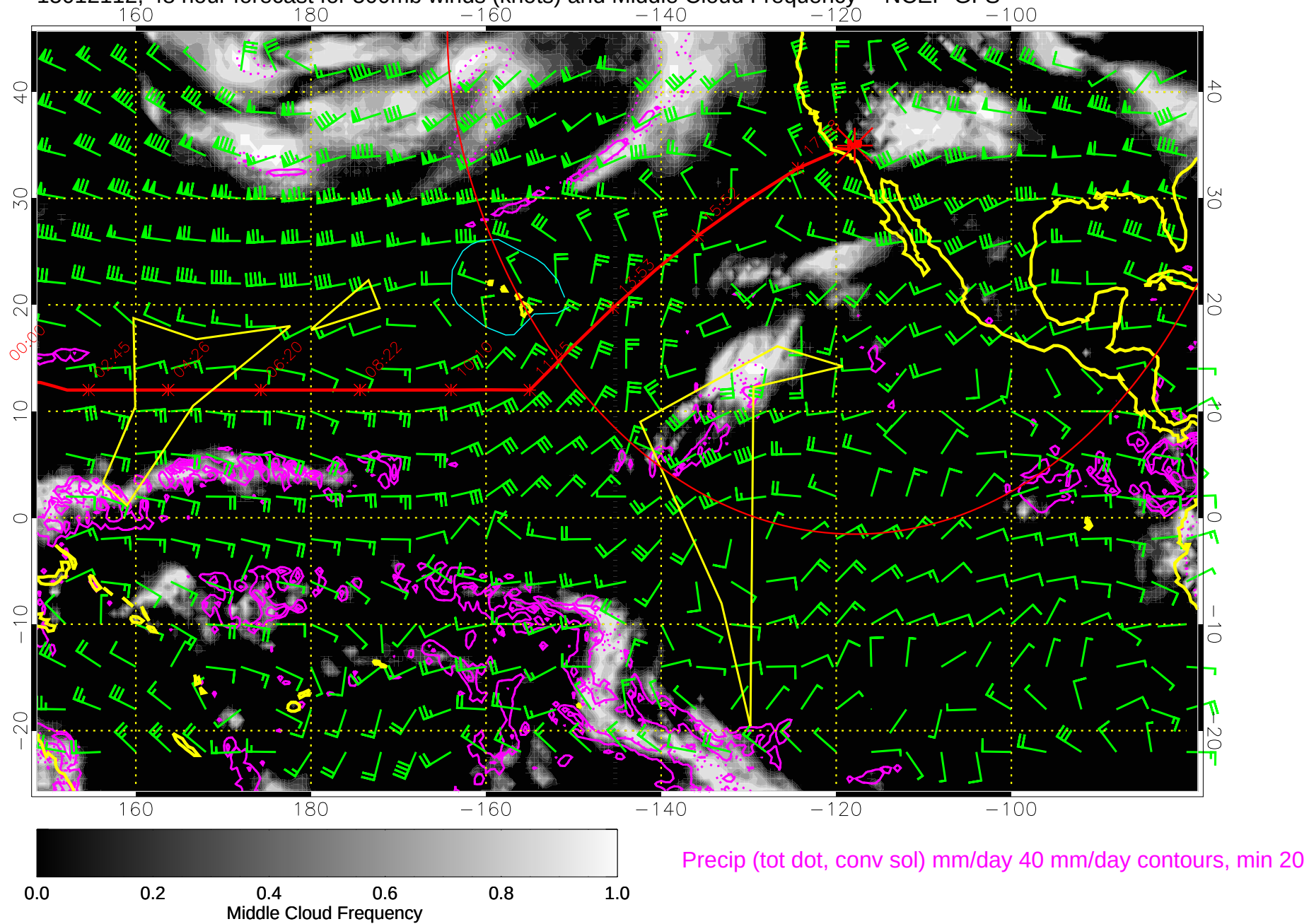
15012112, 48 hour forecast for 500mb winds (knots) and Middle Cloud Frequency -- NCEP GFS
