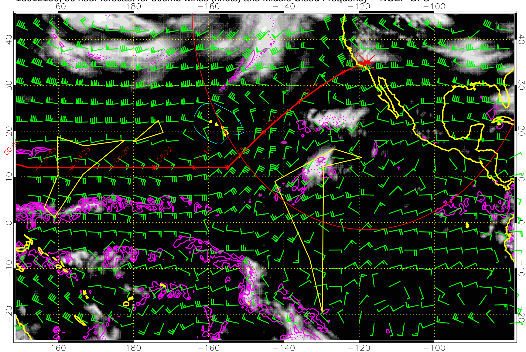
15012100, 36 hour forecast for 500mb winds (knots) and Middle Cloud Frequency -- NCEP GFS
