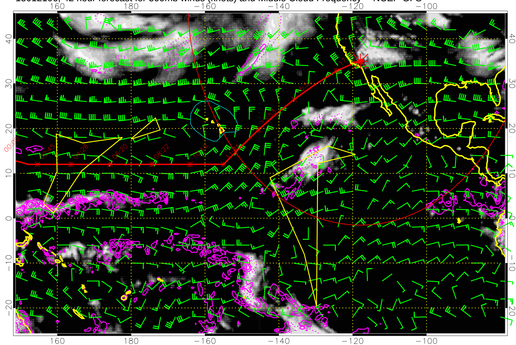
15012106, 42 hour forecast for 500mb winds (knots) and Middle Cloud Frequency -- NCEP GFS
