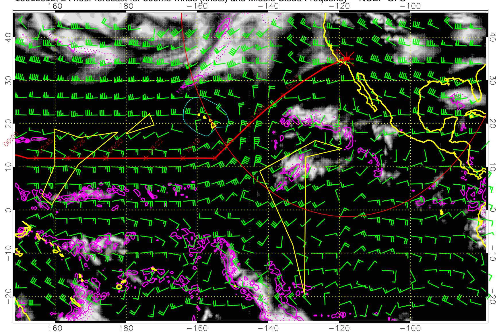
15012012, 24 hour forecast for 500mb winds (knots) and Middle Cloud Frequency -- NCEP GFS
