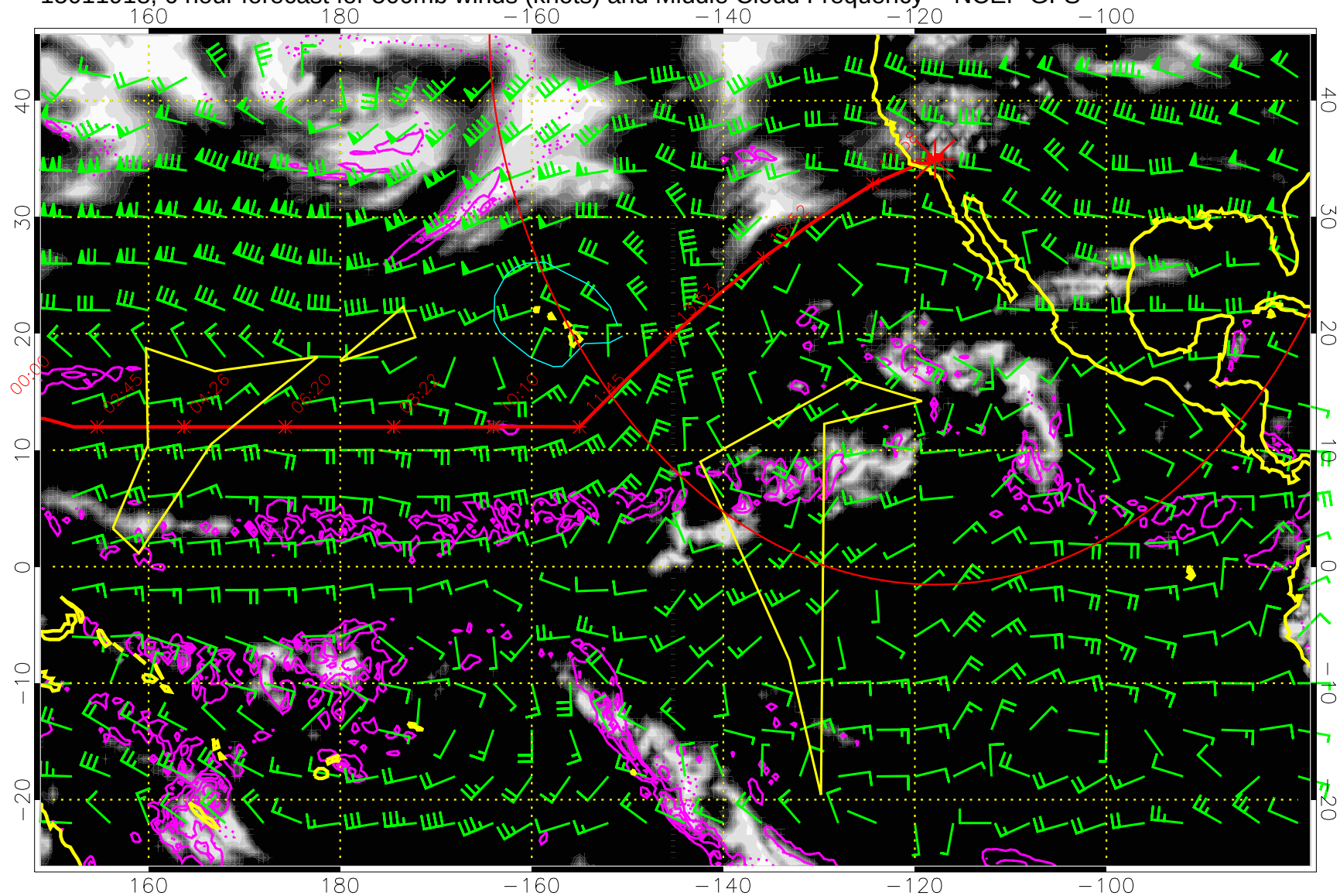
15011918, 6 hour forecast for 500mb winds (knots) and Middle Cloud Frequency -- NCEP GFS
