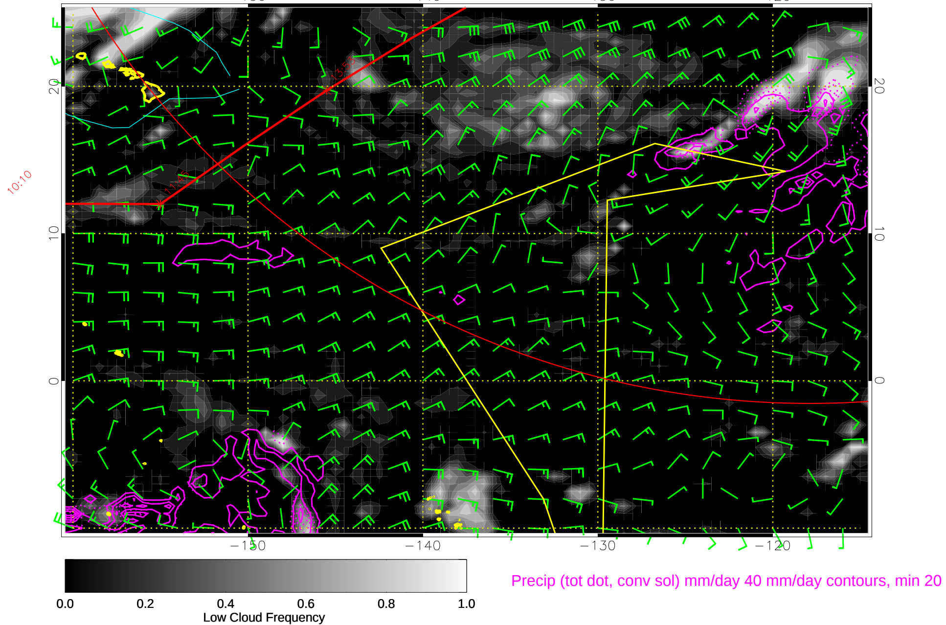
15012412, 120 hour forecast for 850mb winds (knots) and Low Cloud Frequency -- NCEP GFS
