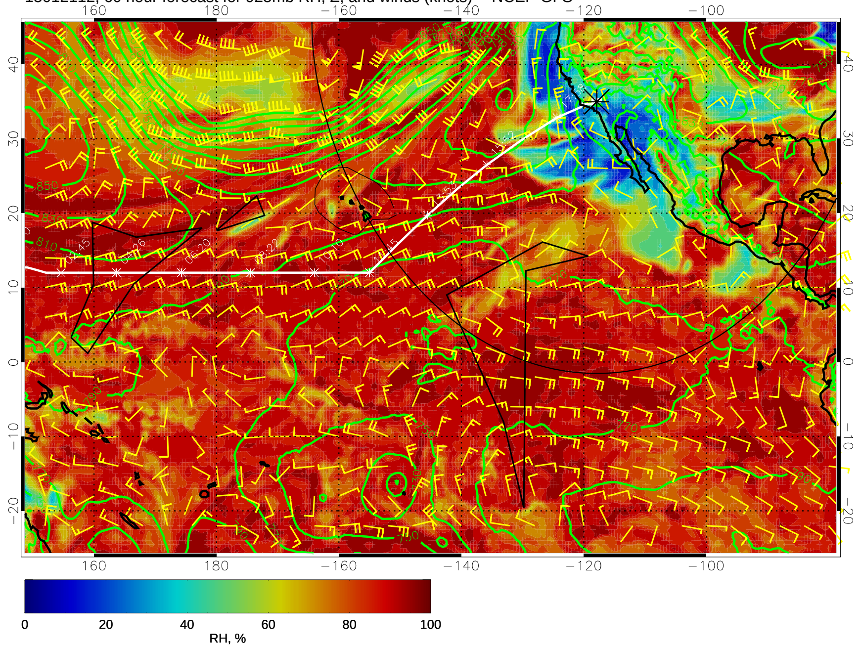
15012112, 60 hour forecast for 925mb RH, Z, and winds (knots) -- NCEP GFS
