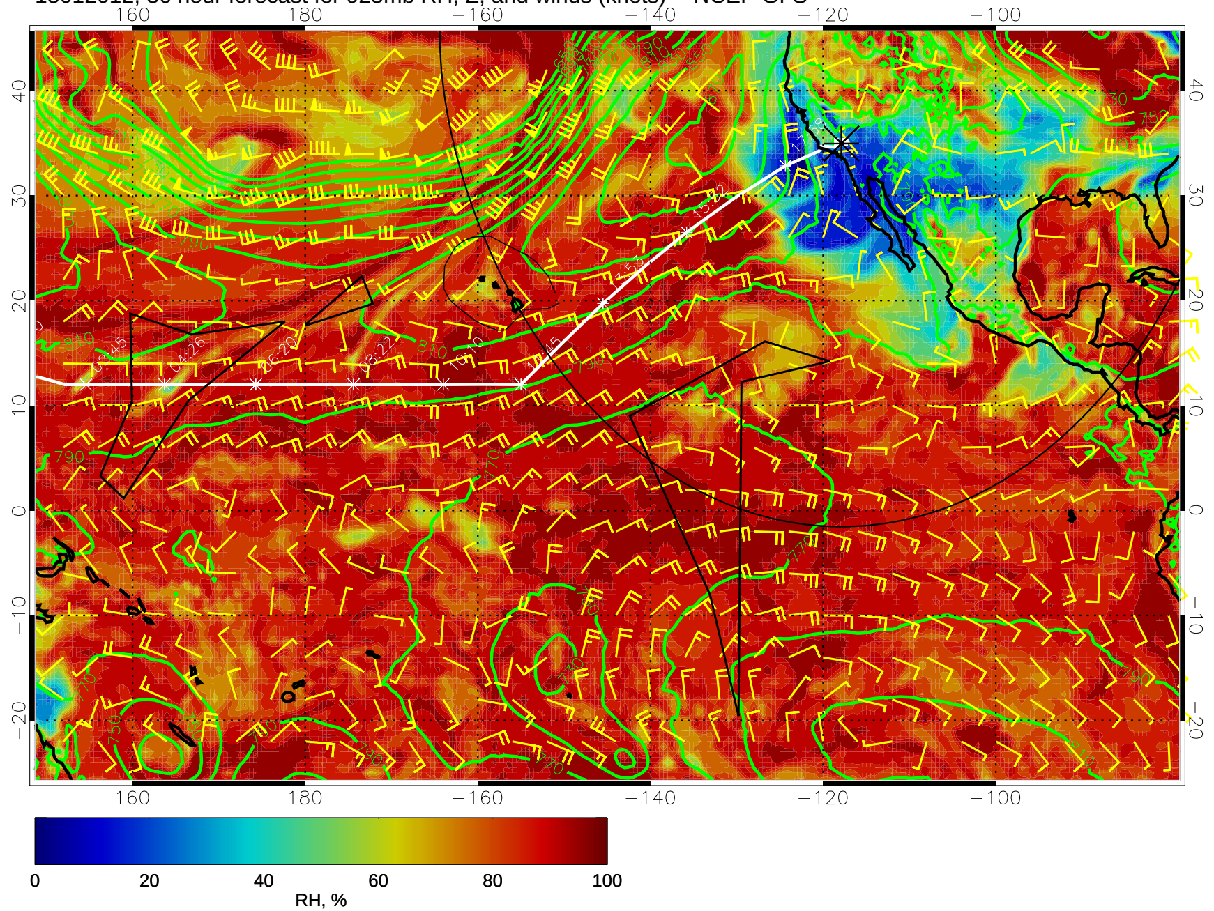
15012012, 36 hour forecast for 925mb RH, Z, and winds (knots) -- NCEP GFS
