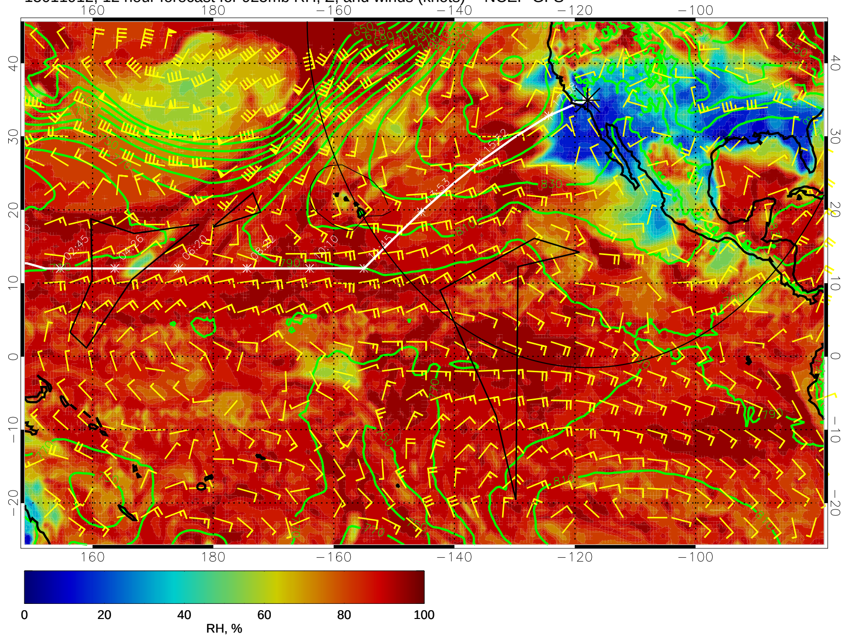
15011912, 12 hour forecast for 925mb RH, Z, and winds (knots) -- NCEP GFS
