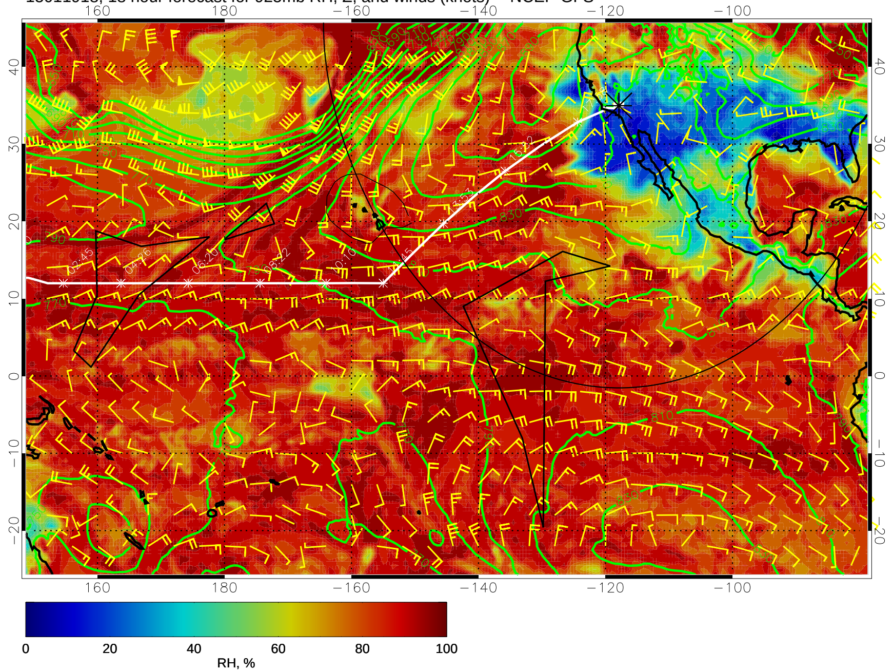
15011918, 18 hour forecast for 925mb RH, Z, and winds (knots) -- NCEP GFS
