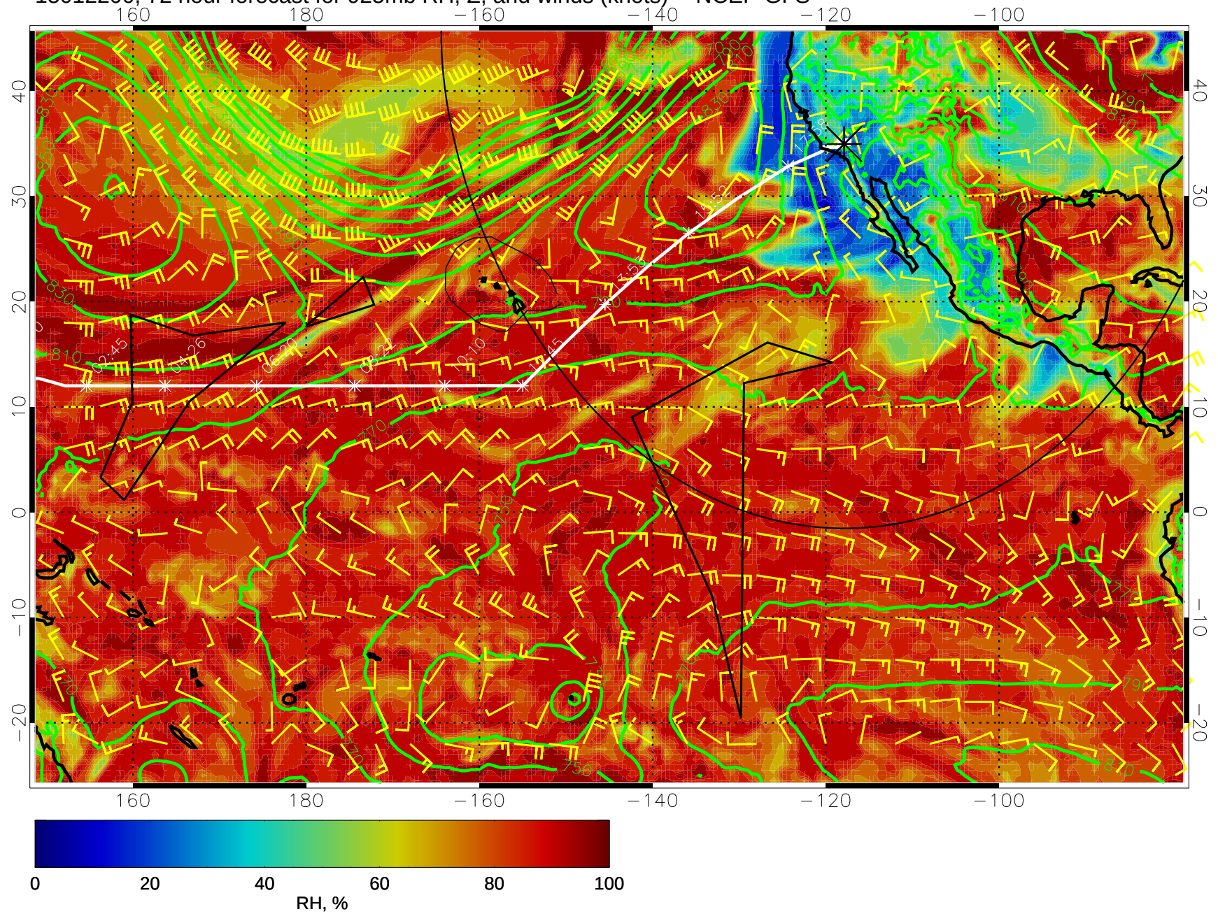
15012200, 72 hour forecast for 925mb RH, Z, and winds (knots) -- NCEP GFS
