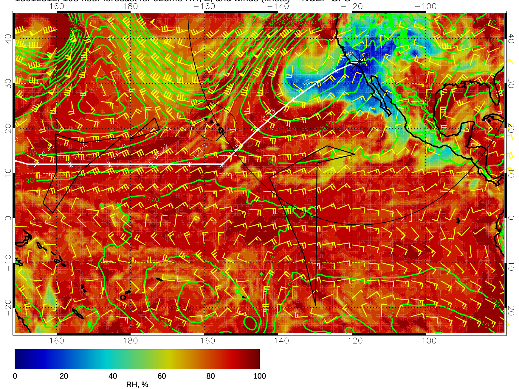
15012312, 108 hour forecast for 925mb RH, Z, and winds (knots) -- NCEP GFS
