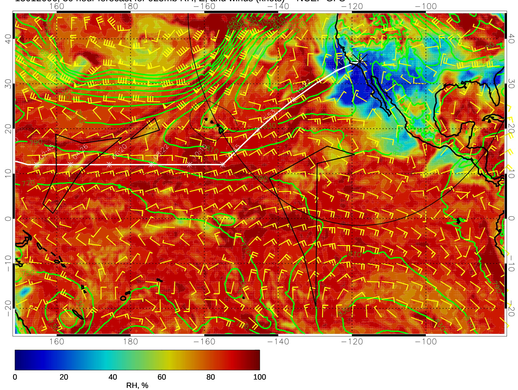
15012006, 30 hour forecast for 925mb RH, Z, and winds (knots) -- NCEP GFS
