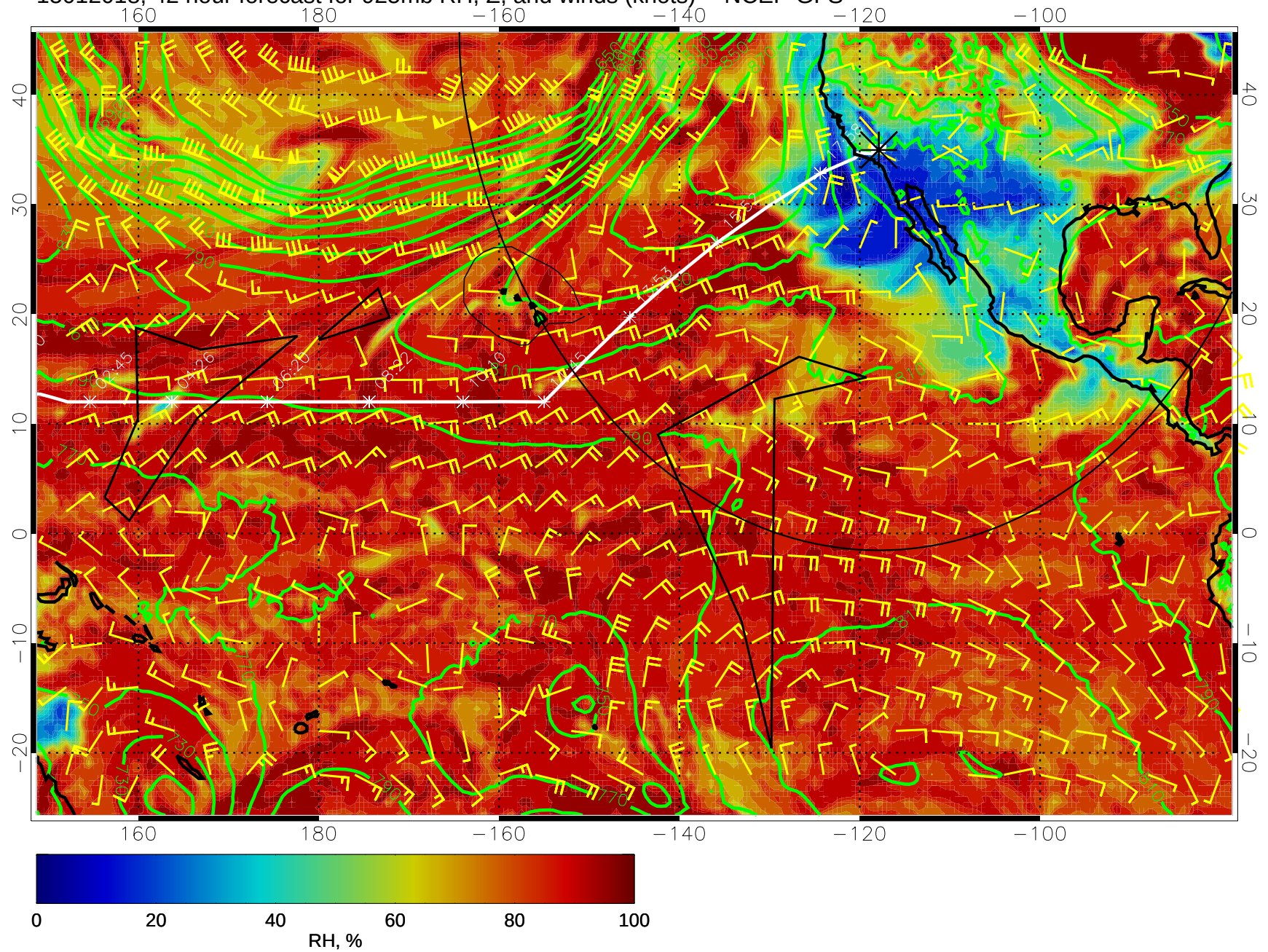
15012018, 42 hour forecast for 925mb RH, Z, and winds (knots) -- NCEP GFS
