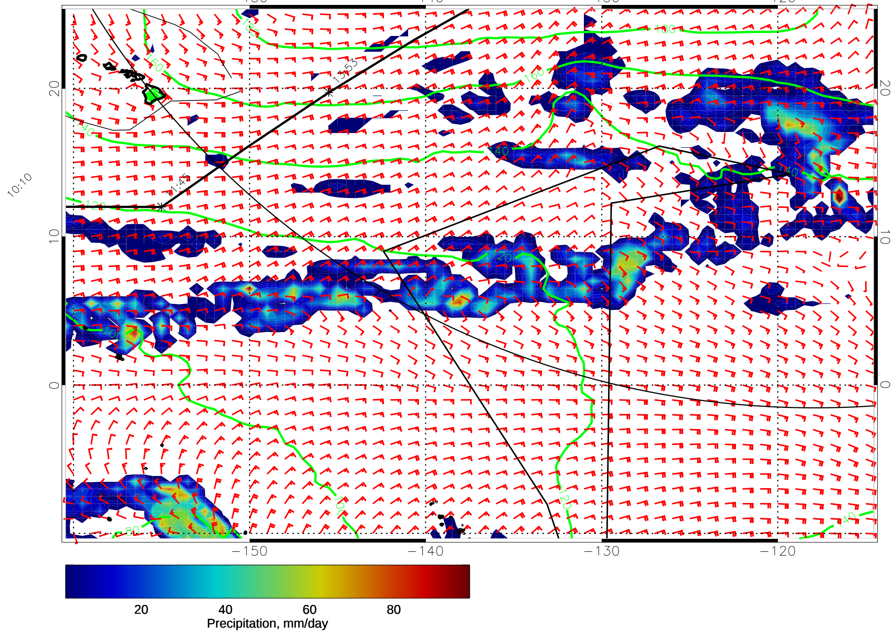
15011918, 18 hour forecast for precip, 1000mb Z, and winds (knots) -- NCEP GFS
