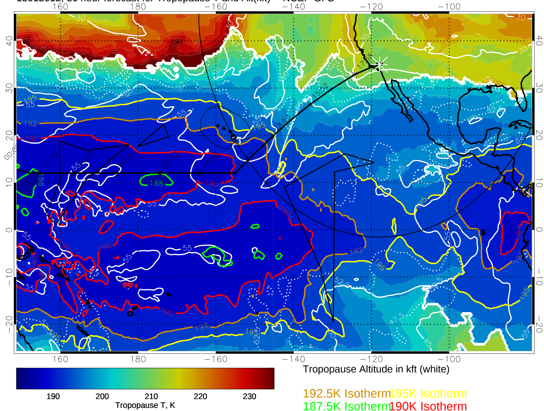
15012012, 36 hour forecast for Tropopause T and Alt(kft) -- NCEP GFS
