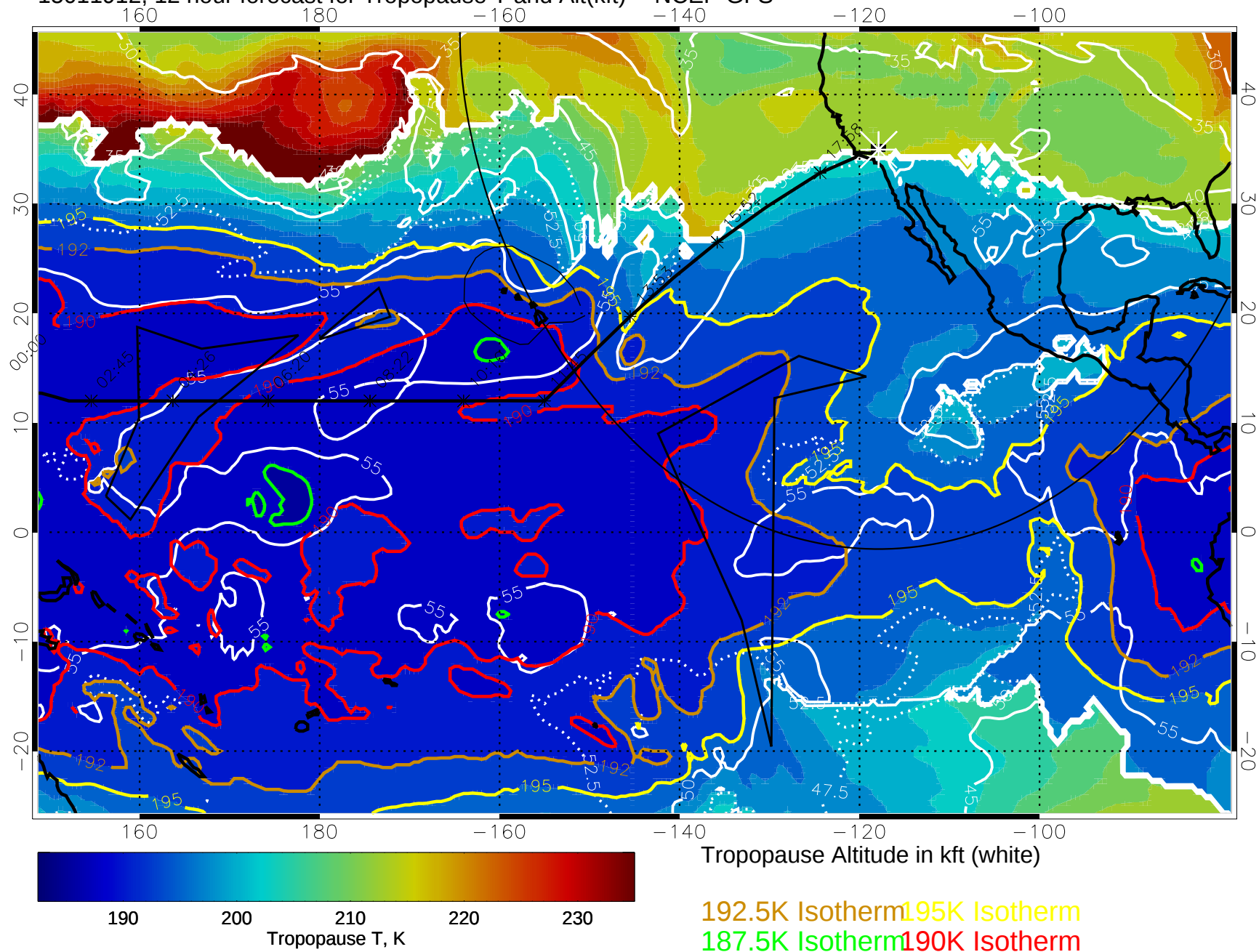
15011912, 12 hour forecast for Tropopause T and Alt(kft) -- NCEP GFS
