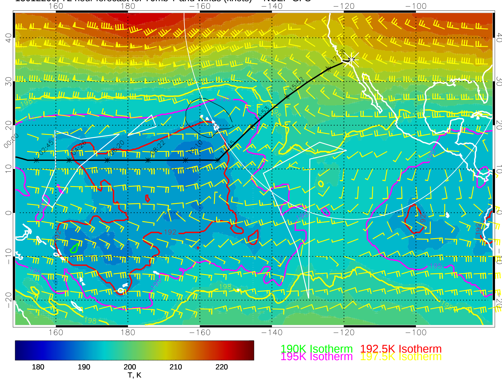
15012200, 72 hour forecast for 70mb T and winds (knots) -- NCEP GFS
