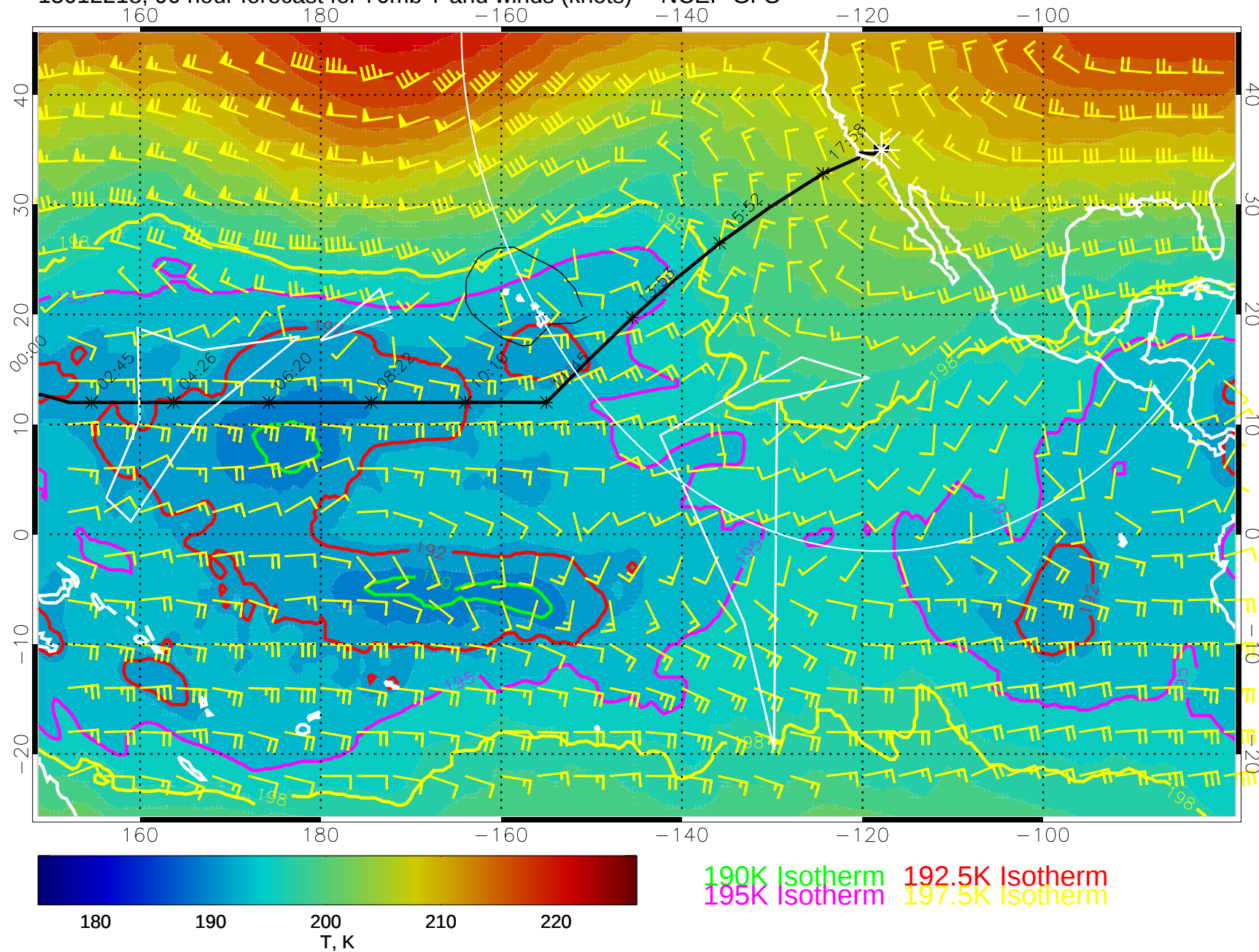
15012218, 90 hour forecast for 70mb T and winds (knots) -- NCEP GFS
