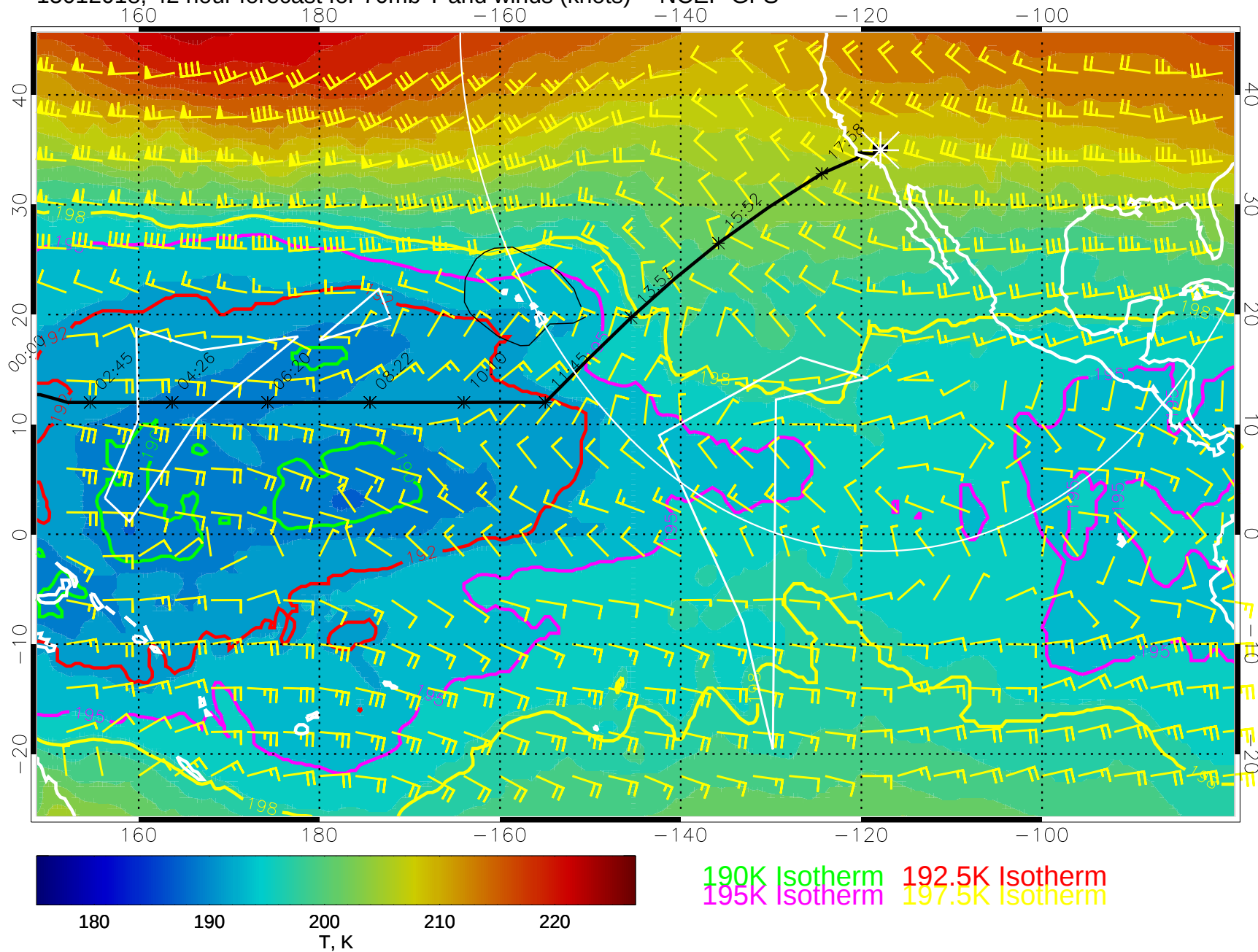
15012018, 42 hour forecast for 70mb T and winds (knots) -- NCEP GFS
