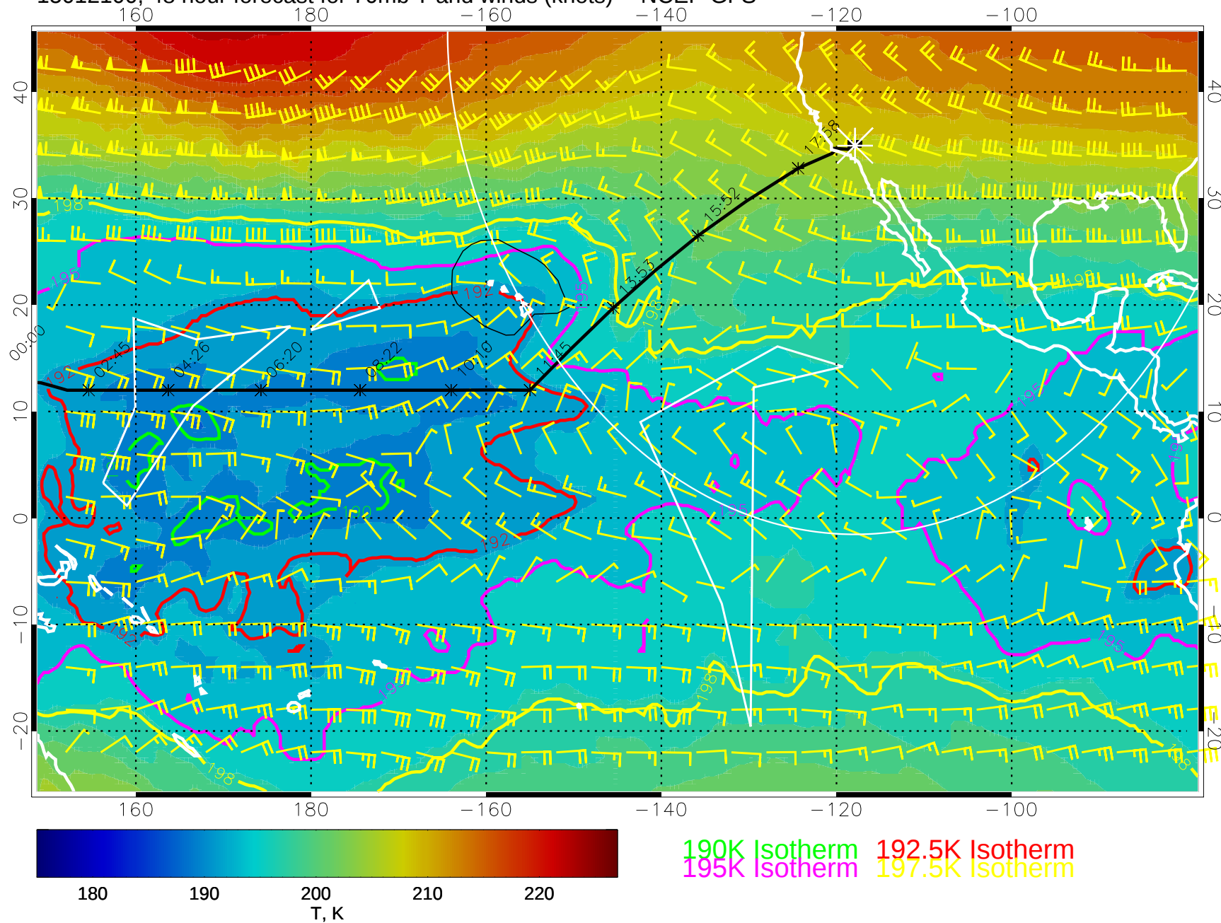
15012100, 48 hour forecast for 70mb T and winds (knots) -- NCEP GFS
