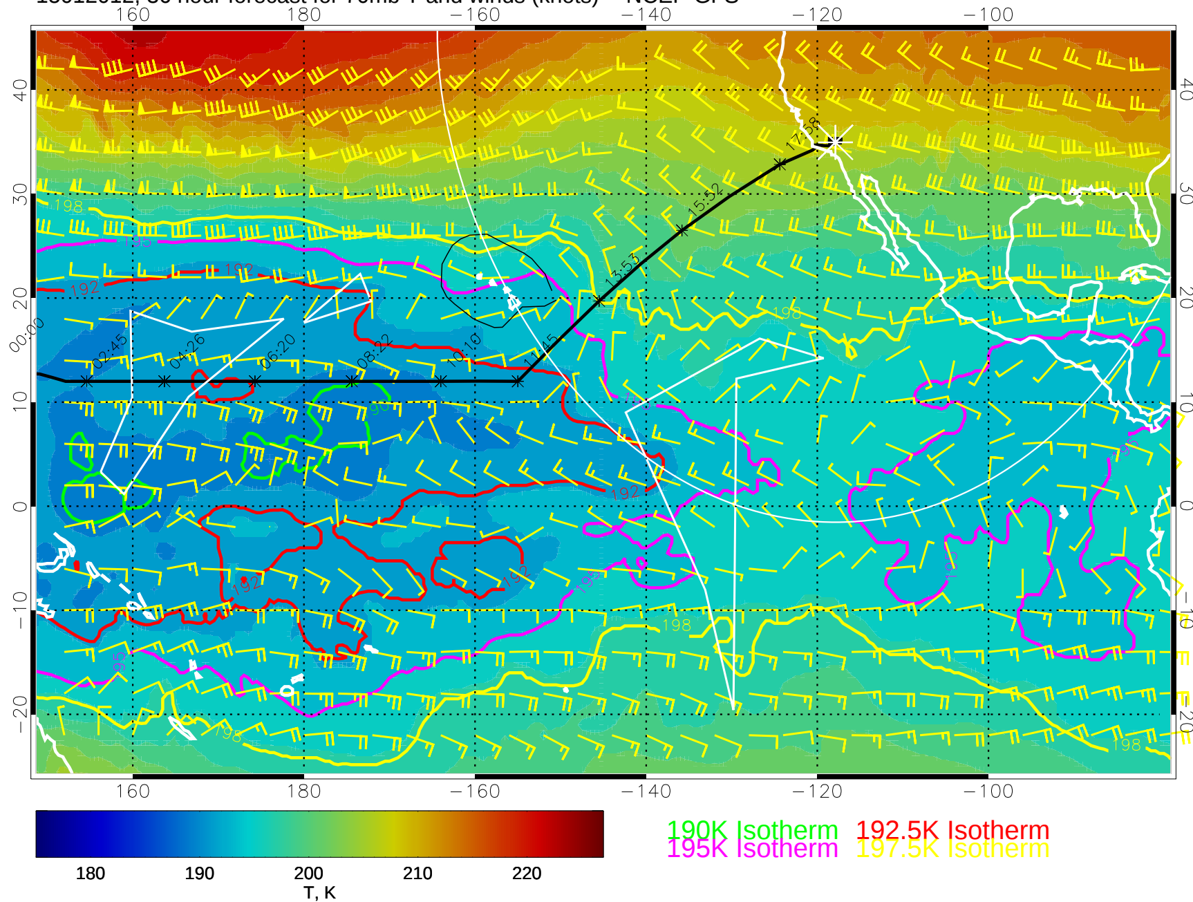
15012012, 36 hour forecast for 70mb T and winds (knots) -- NCEP GFS
