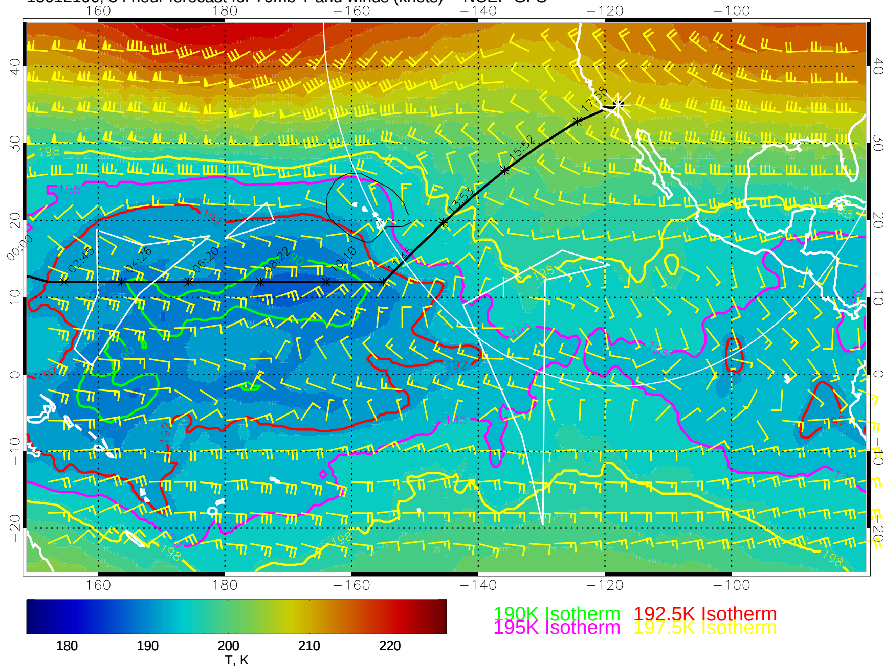
15012106, 54 hour forecast for 70mb T and winds (knots) -- NCEP GFS
