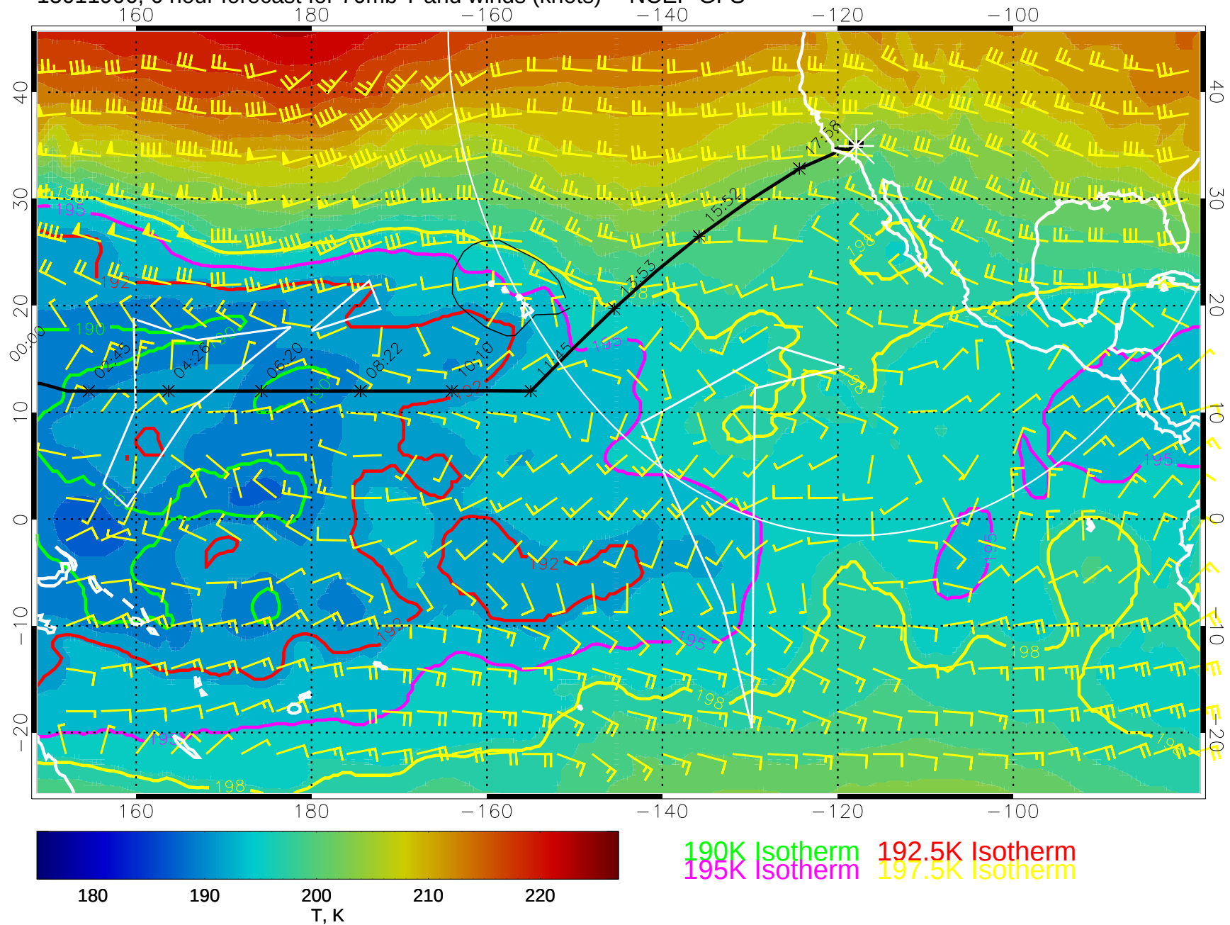
15011906, 6 hour forecast for 70mb T and winds (knots) -- NCEP GFS
