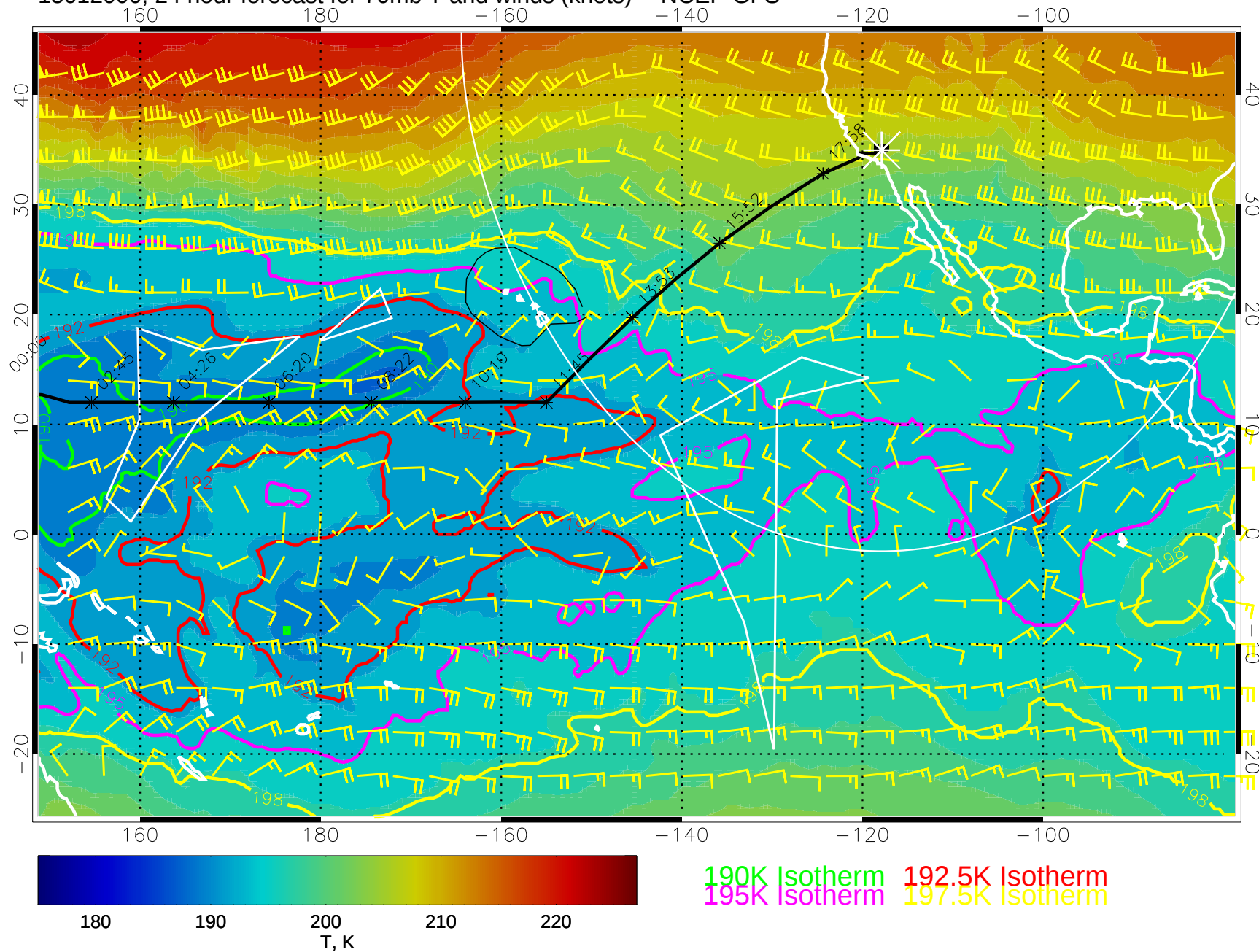
15012000, 24 hour forecast for 70mb T and winds (knots) -- NCEP GFS
