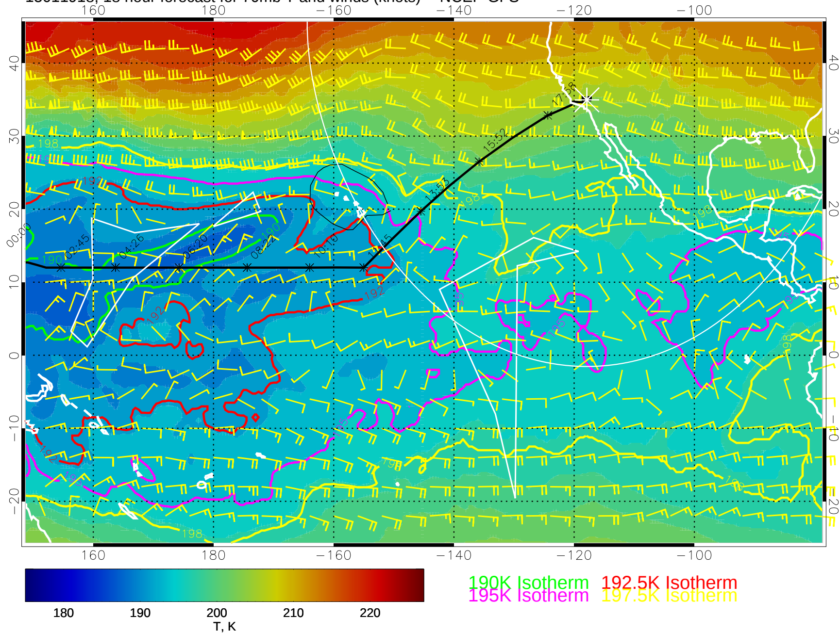
15011918, 18 hour forecast for 70mb T and winds (knots) -- NCEP GFS
