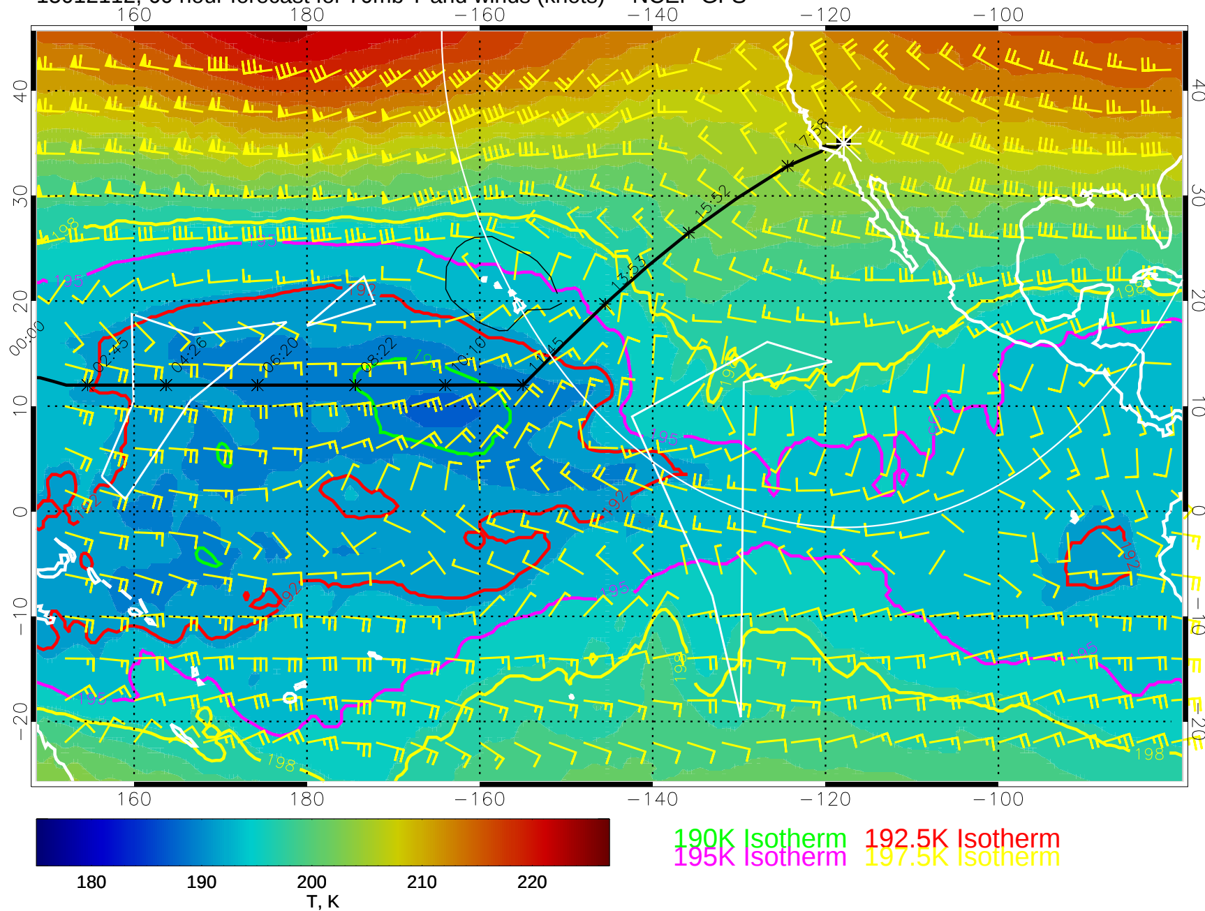
15012112, 60 hour forecast for 70mb T and winds (knots) -- NCEP GFS
