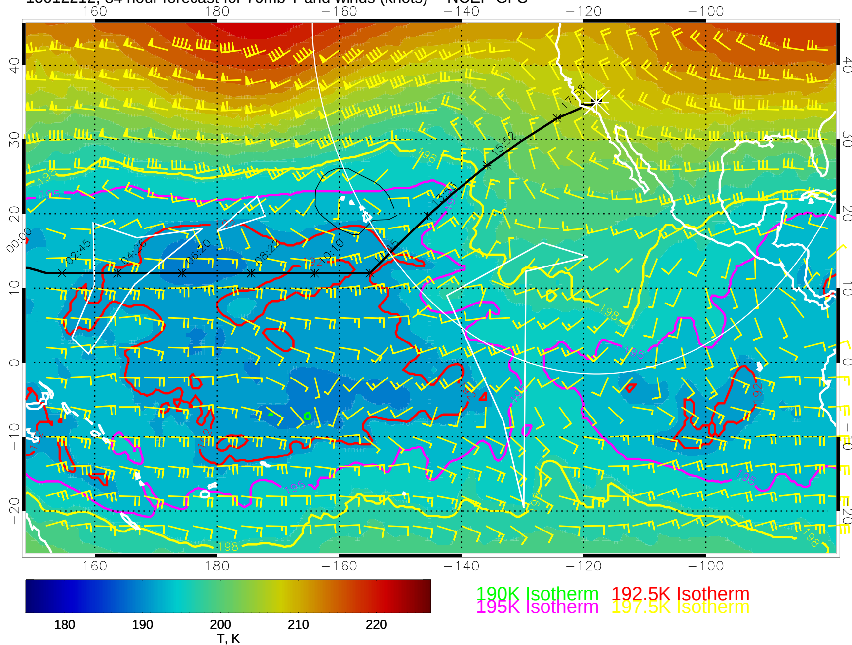
15012212, 84 hour forecast for 70mb T and winds (knots) -- NCEP GFS
