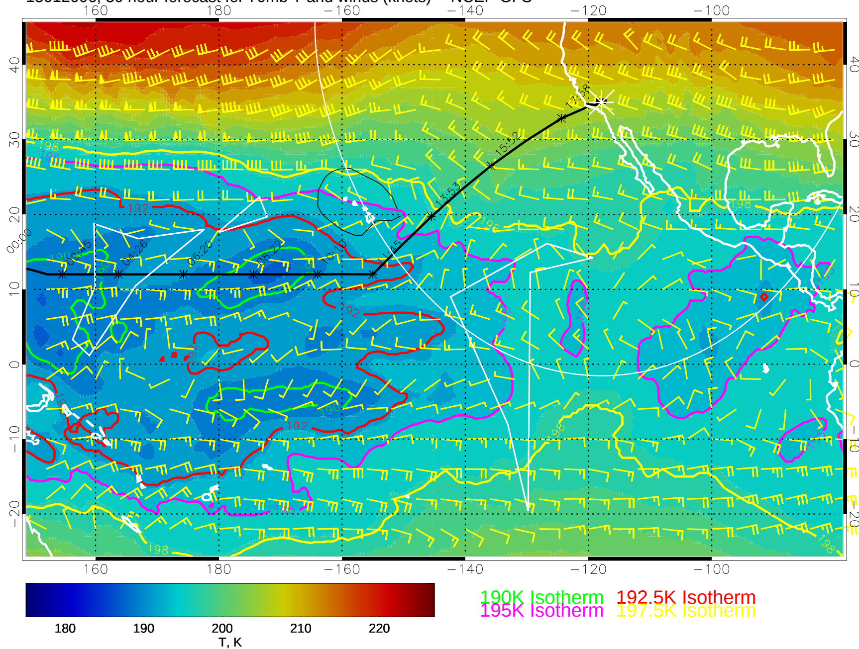
15012006, 30 hour forecast for 70mb T and winds (knots) -- NCEP GFS
