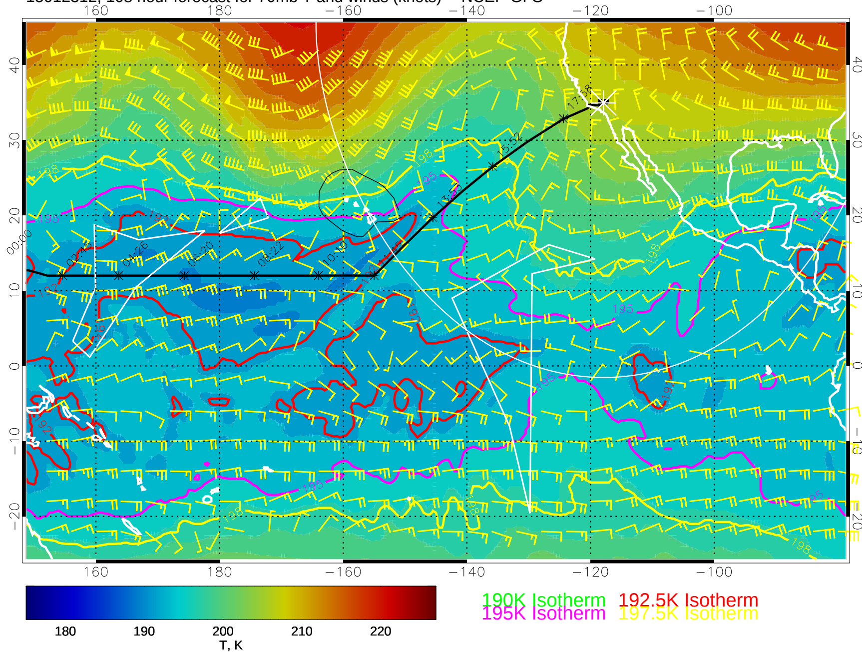
15012312, 108 hour forecast for 70mb T and winds (knots) -- NCEP GFS
