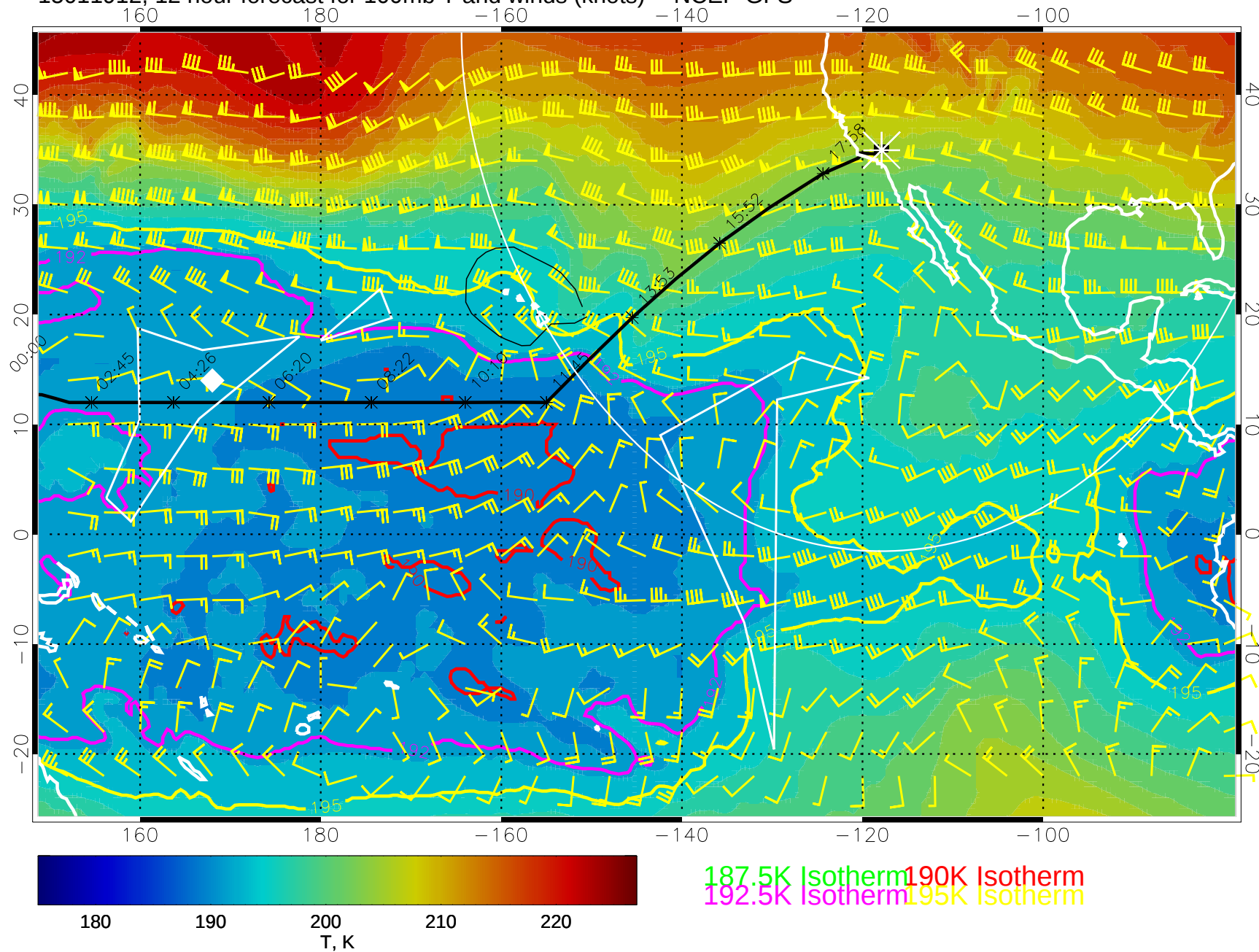
15011912, 12 hour forecast for 100mb T and winds (knots) -- NCEP GFS
