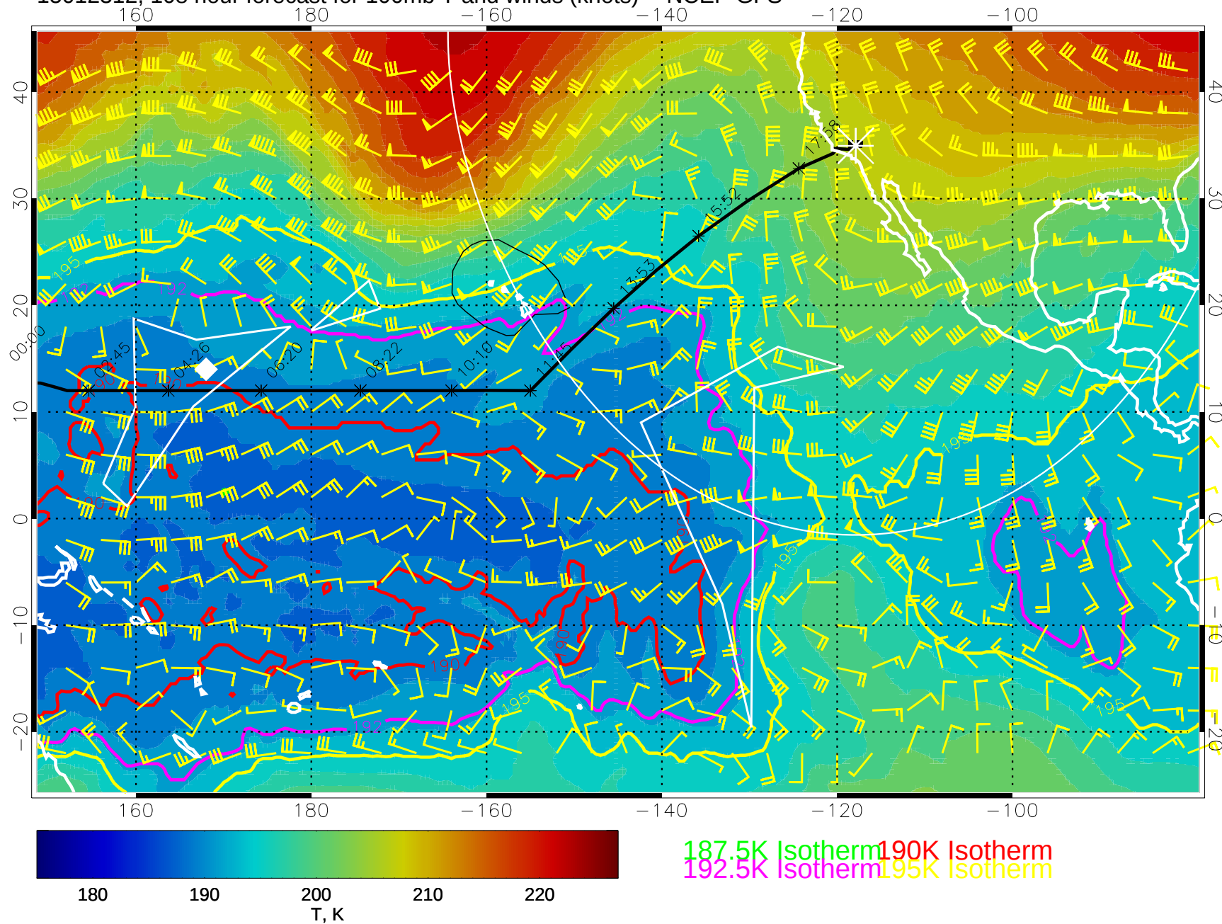
15012312, 108 hour forecast for 100mb T and winds (knots) -- NCEP GFS
