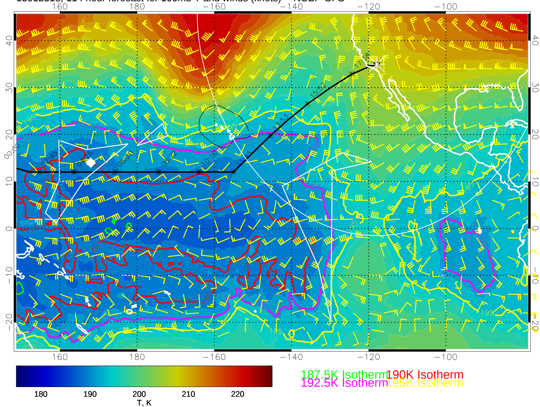
15012318, 114 hour forecast for 100mb T and winds (knots) -- NCEP GFS
