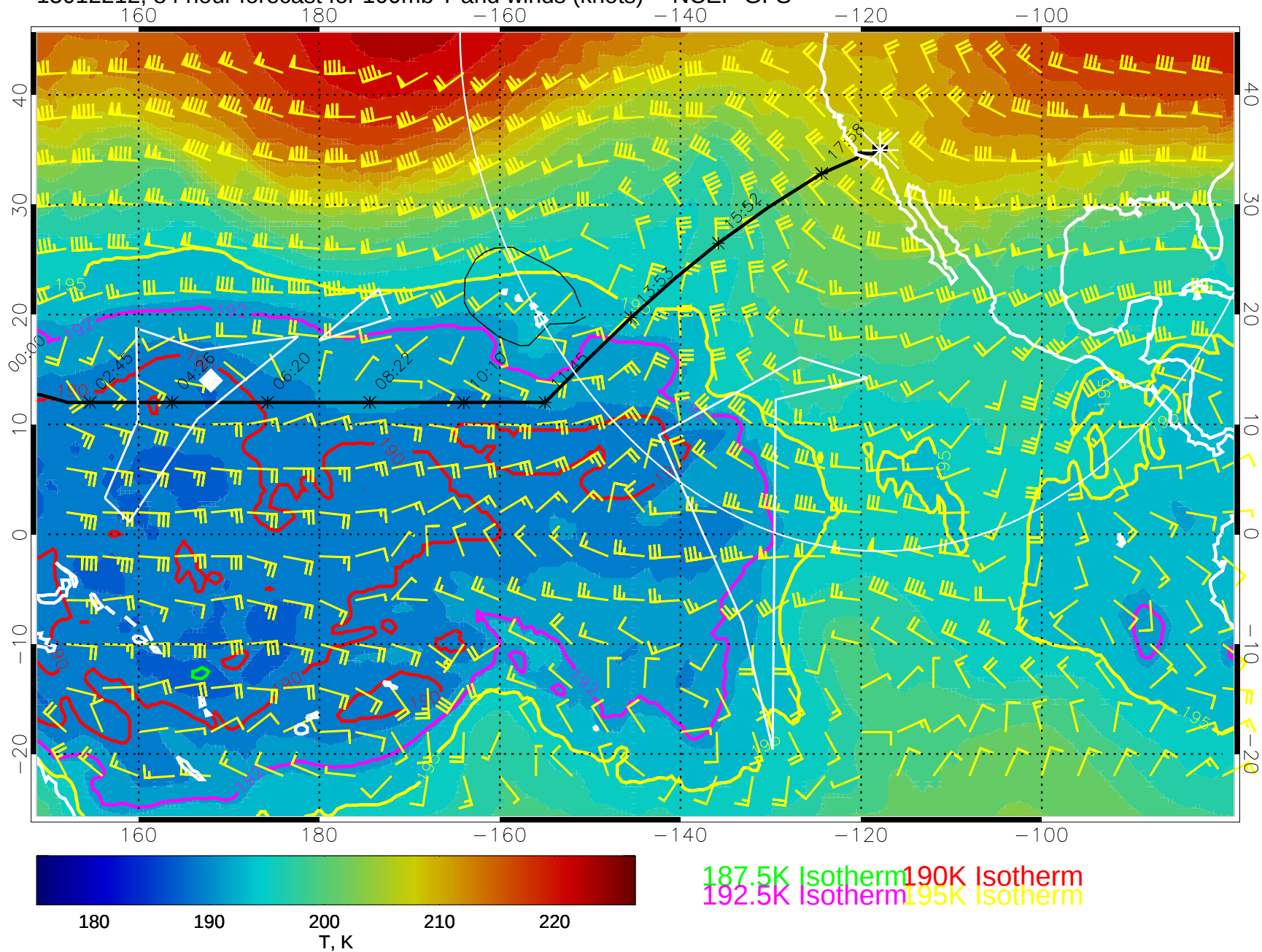
15012212, 84 hour forecast for 100mb T and winds (knots) -- NCEP GFS
