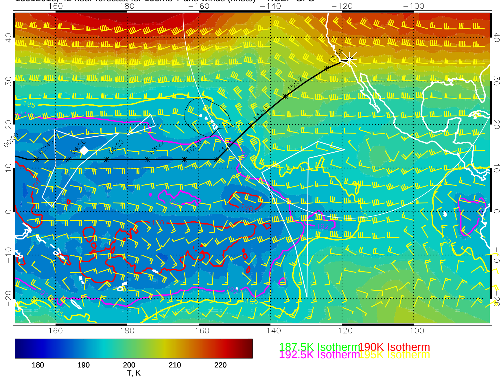
15012018, 42 hour forecast for 100mb T and winds (knots) -- NCEP GFS
