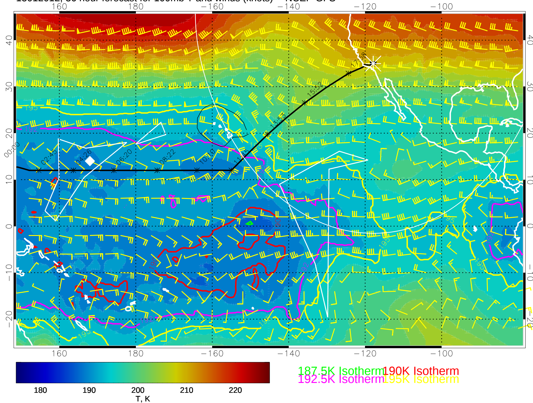
15012012, 36 hour forecast for 100mb T and winds (knots) -- NCEP GFS
