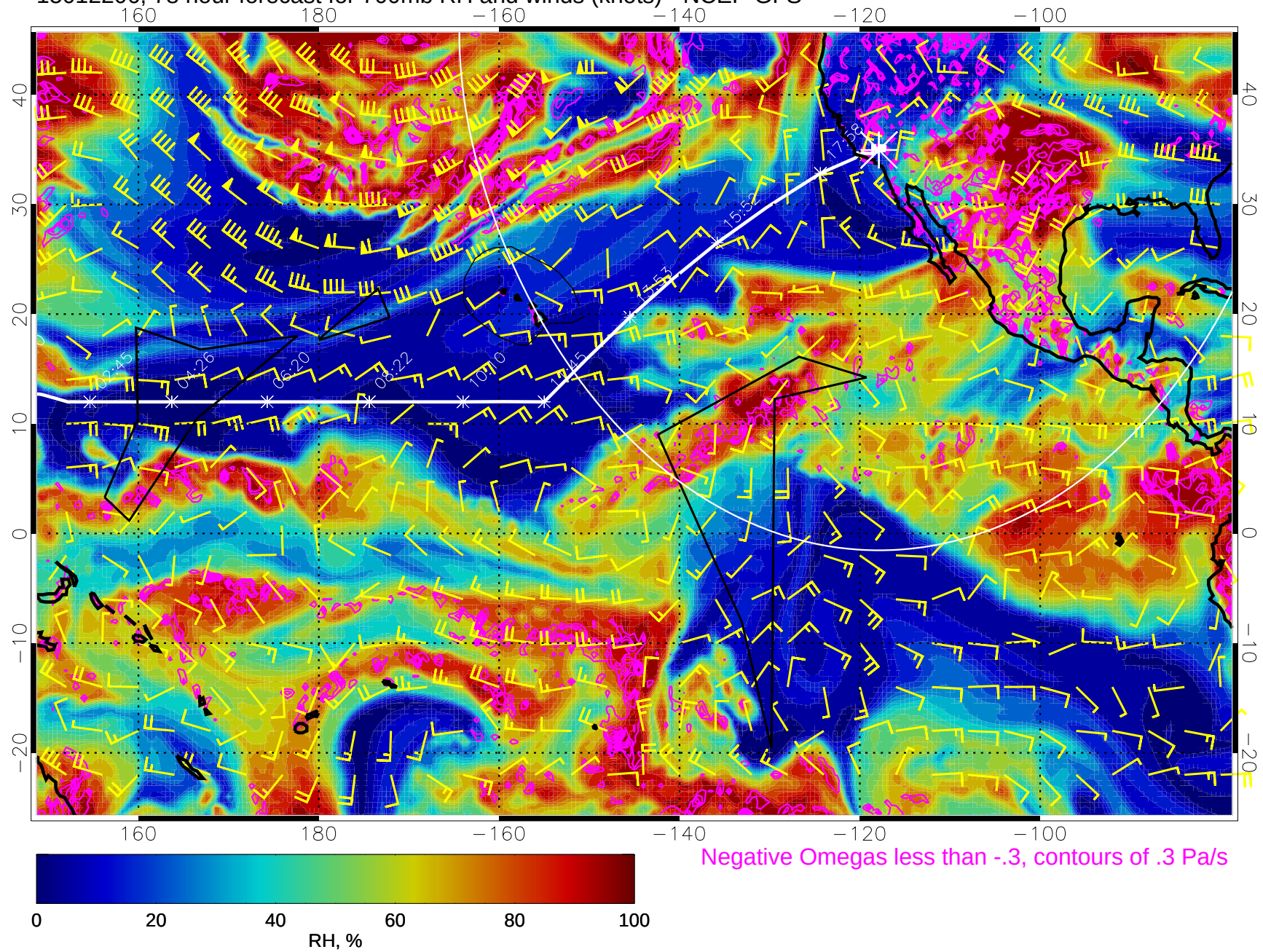
15012206, 78 hour forecast for 700mb RH and winds (knots) - NCEP GFS
