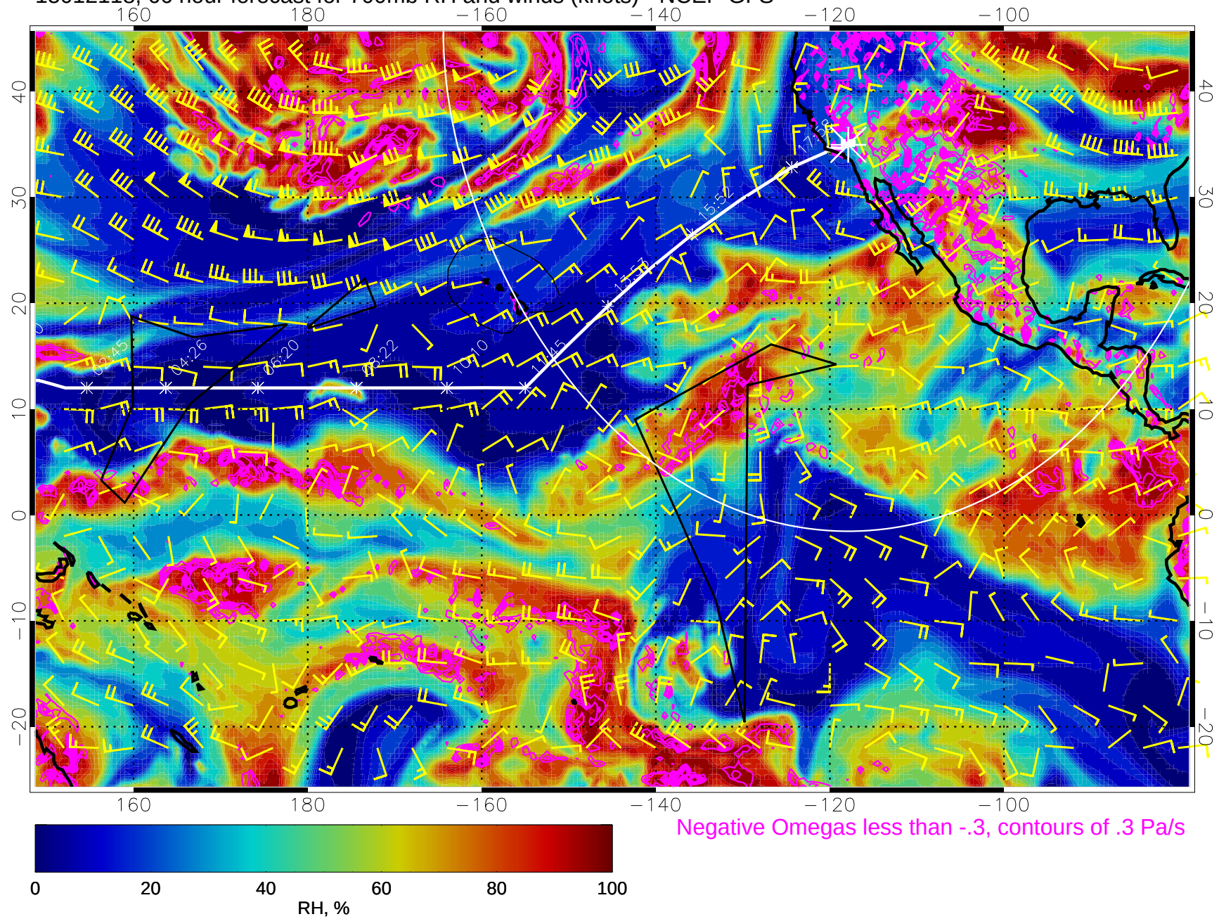
15012118, 66 hour forecast for 700mb RH and winds (knots) - NCEP GFS
