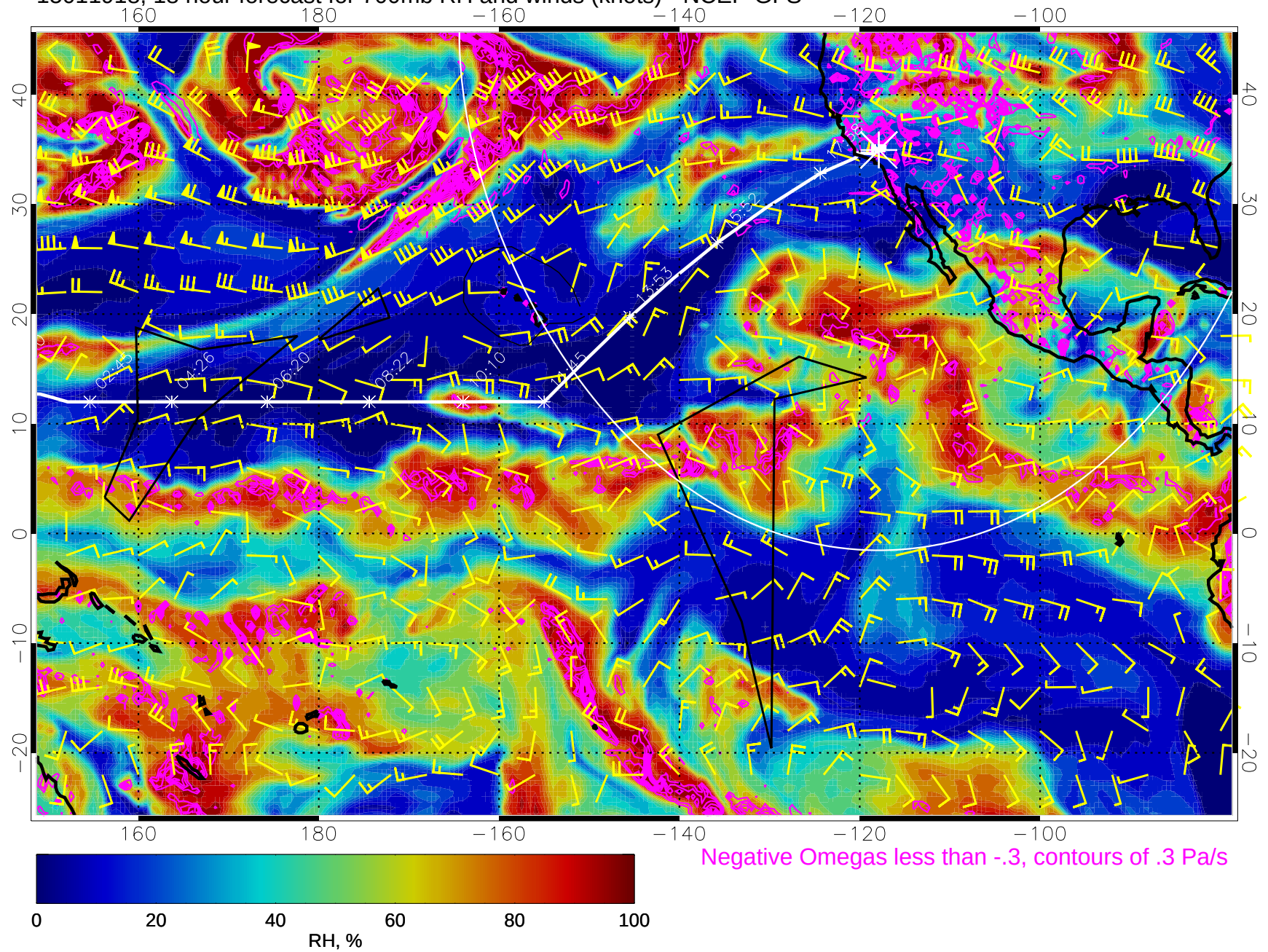
15011918, 18 hour forecast for 700mb RH and winds (knots) - NCEP GFS
