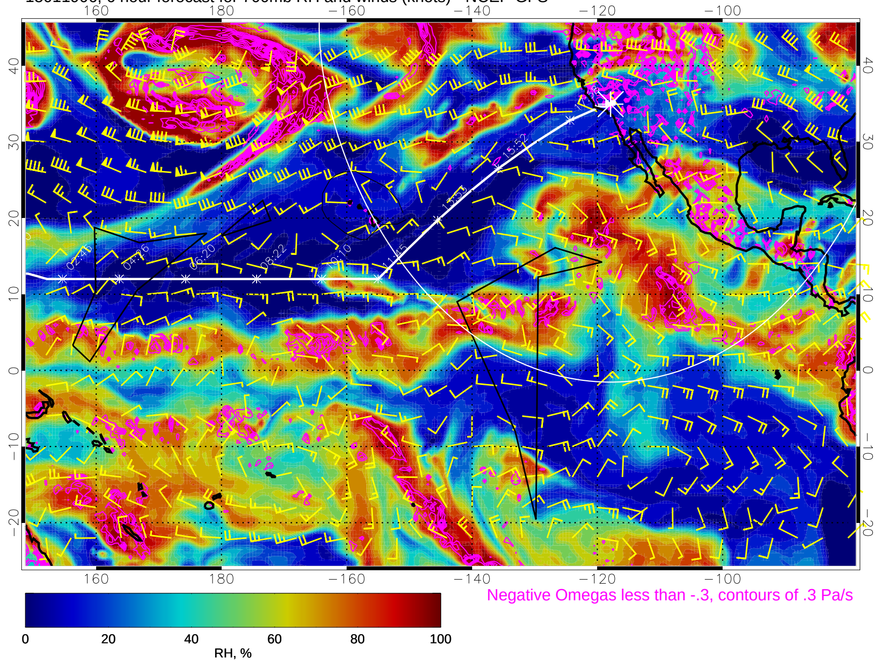
15011906, 6 hour forecast for 700mb RH and winds (knots) - NCEP GFS
