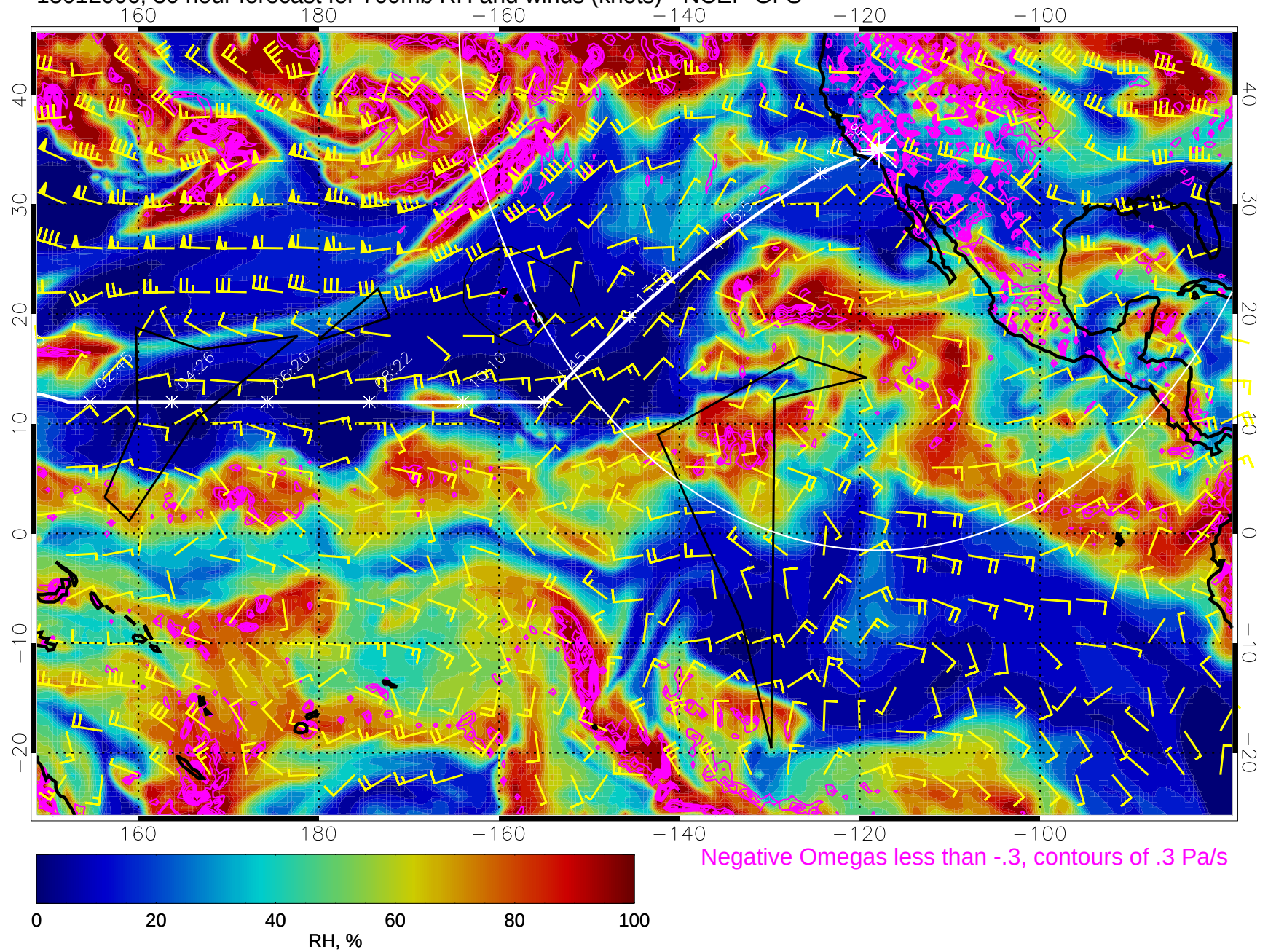
15012006, 30 hour forecast for 700mb RH and winds (knots) - NCEP GFS
