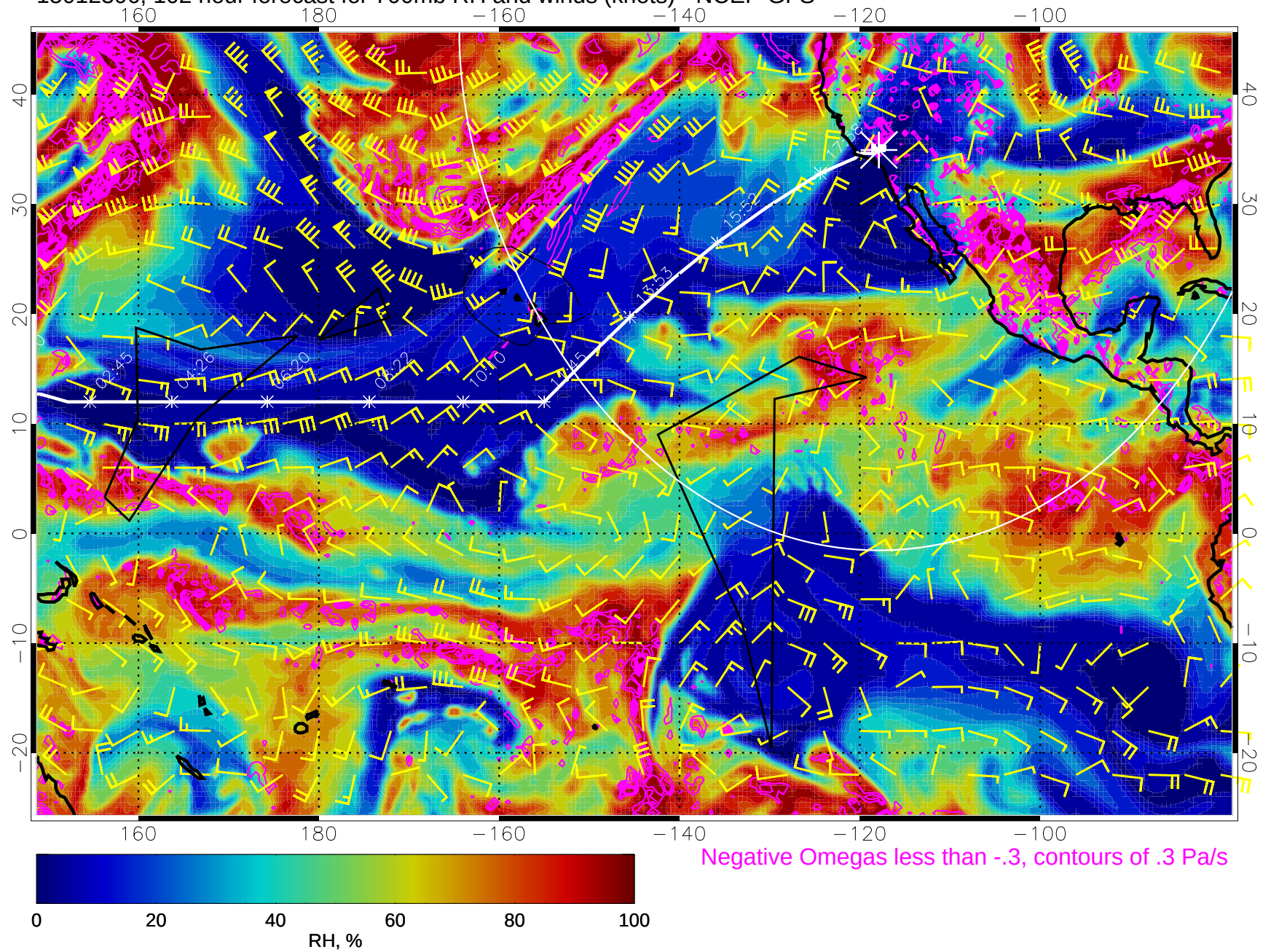
15012306, 102 hour forecast for 700mb RH and winds (knots) - NCEP GFS
