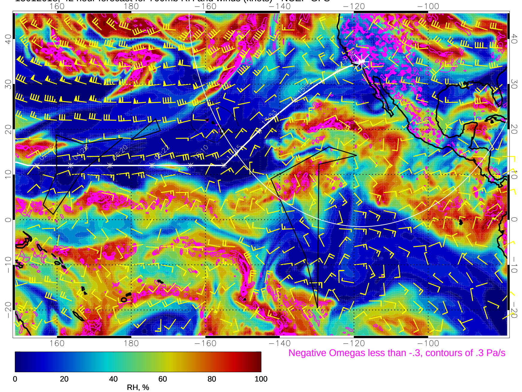
15012018, 42 hour forecast for 700mb RH and winds (knots) - NCEP GFS
