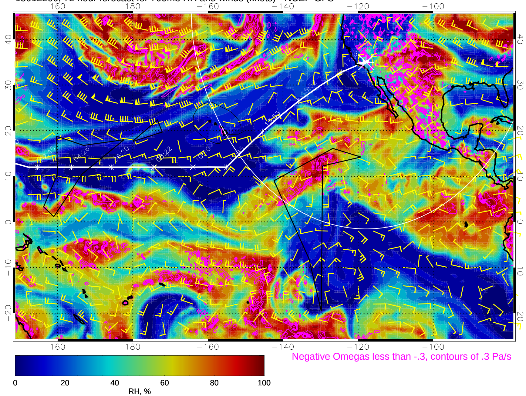
15012200, 72 hour forecast for 700mb RH and winds (knots) - NCEP GFS
