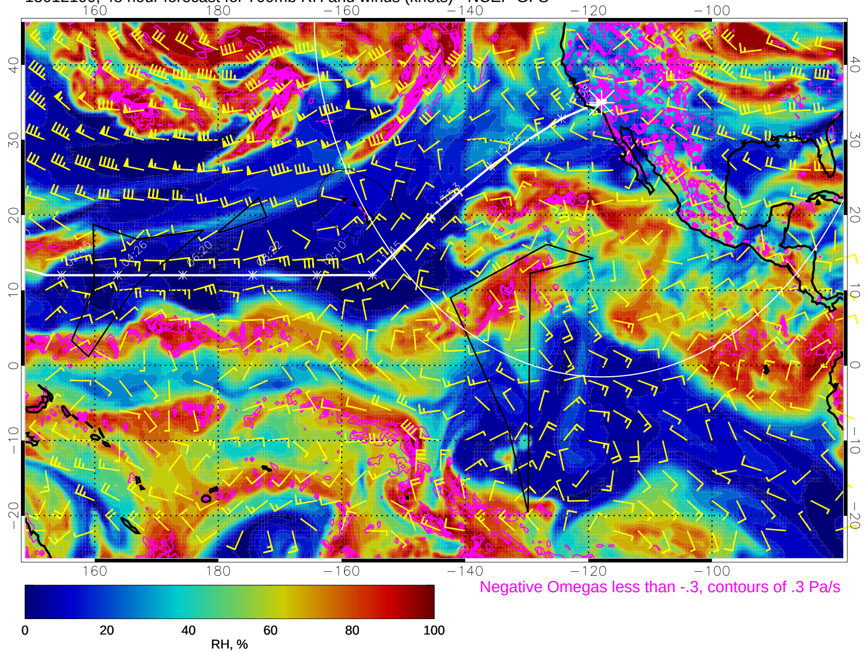
15012100, 48 hour forecast for 700mb RH and winds (knots) - NCEP GFS
