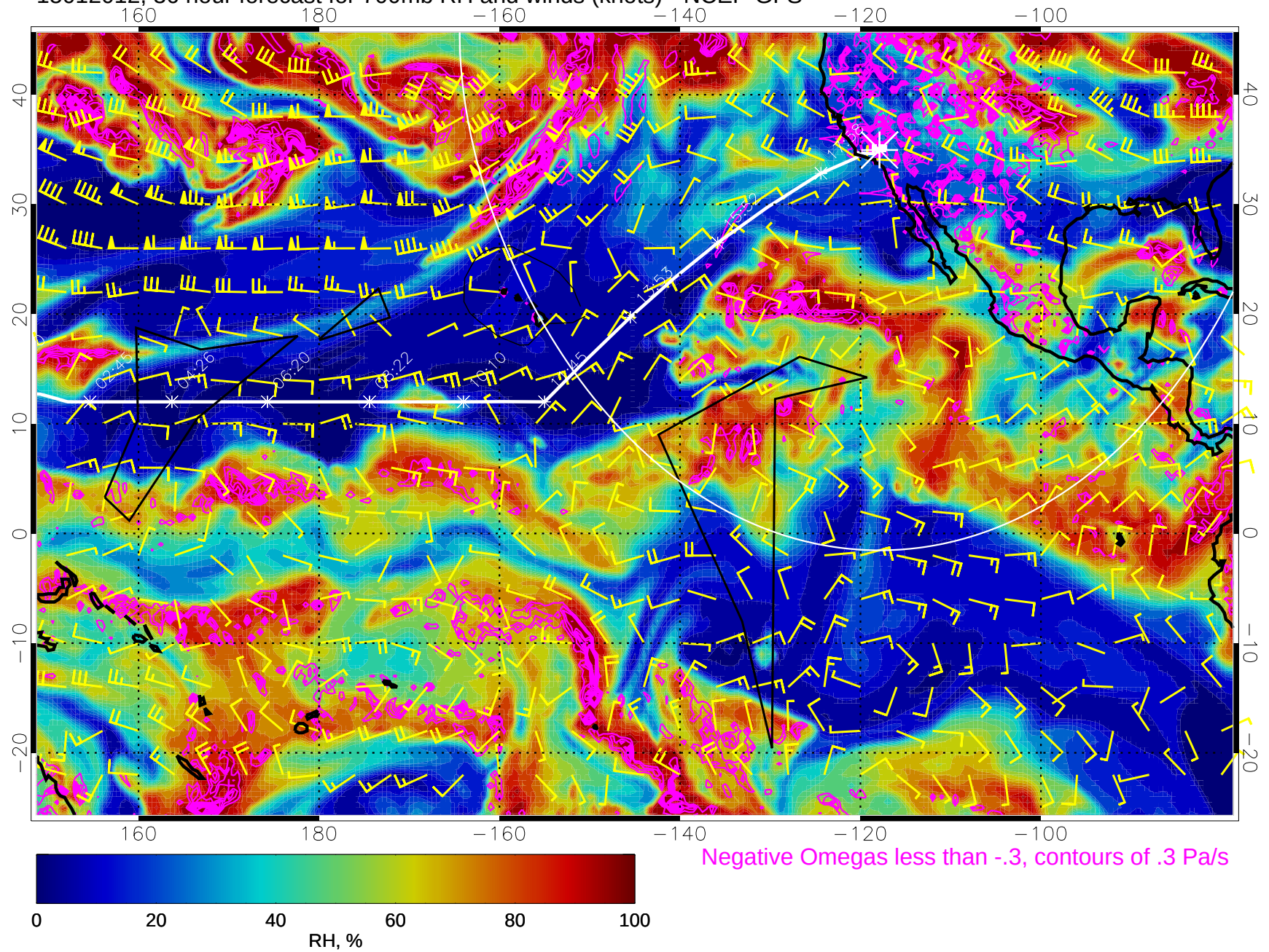
15012012, 36 hour forecast for 700mb RH and winds (knots) - NCEP GFS
