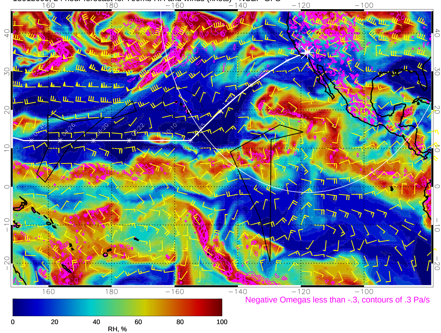
15012000, 24 hour forecast for 700mb RH and winds (knots) - NCEP GFS
