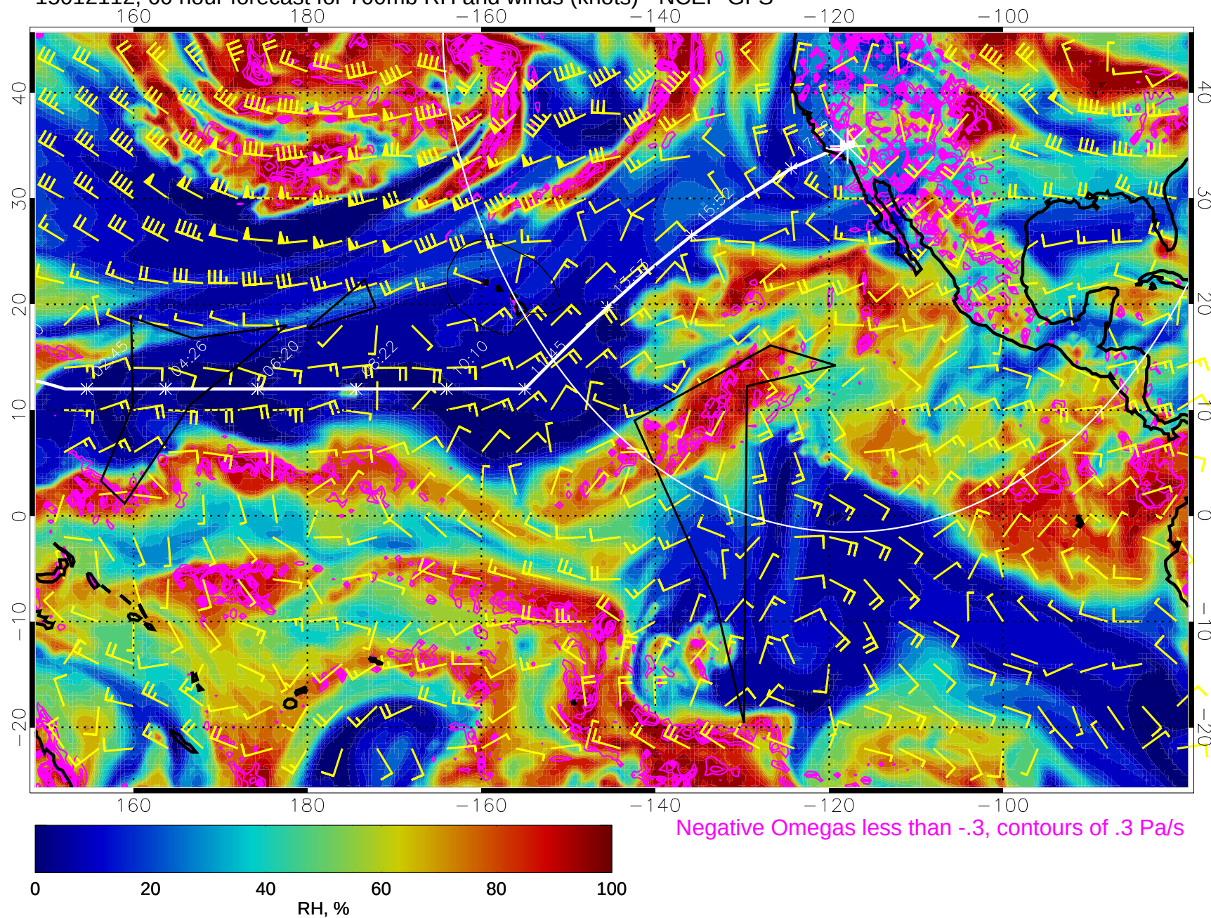
15012112, 60 hour forecast for 700mb RH and winds (knots) - NCEP GFS
