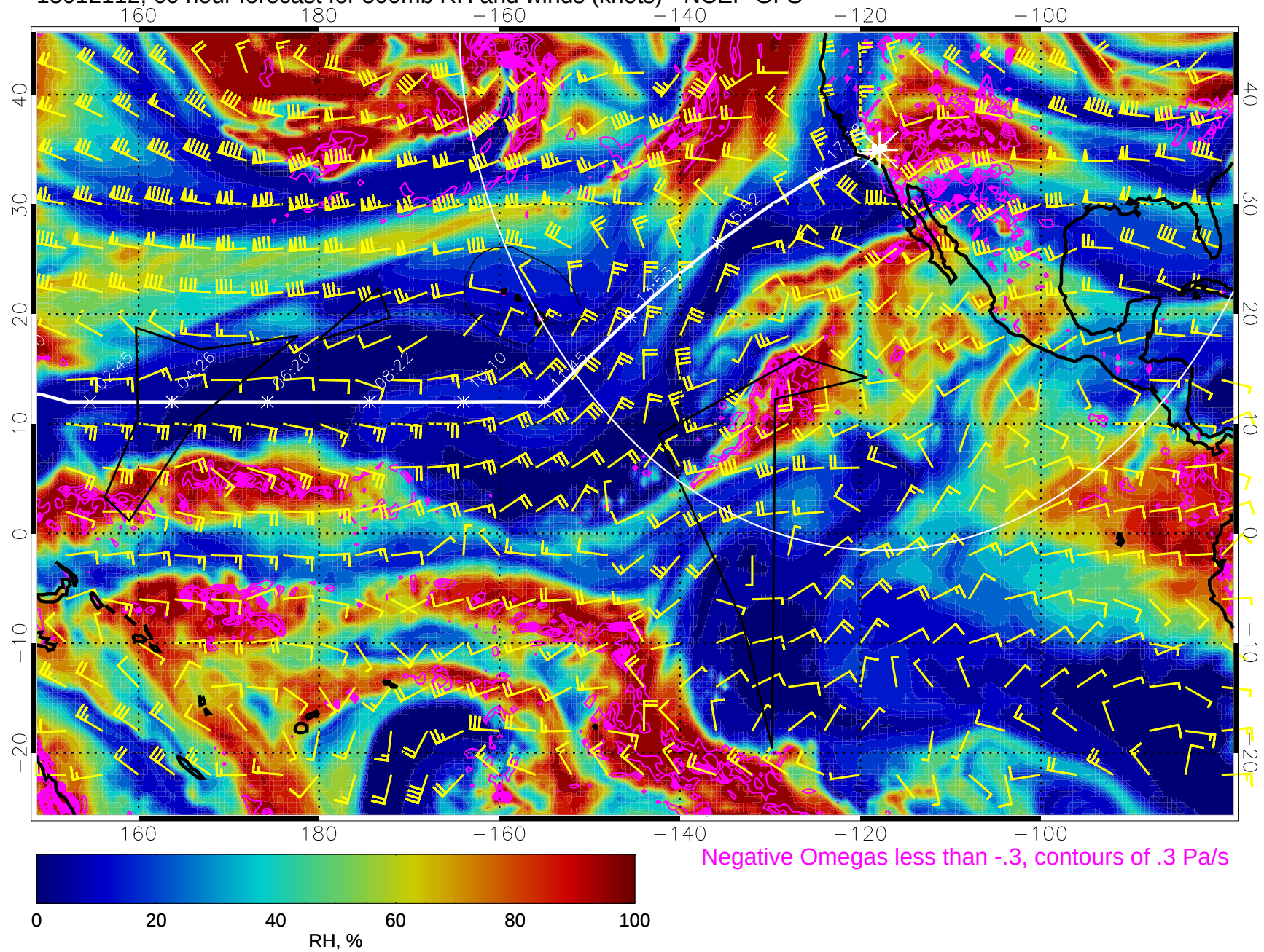
15012112, 60 hour forecast for 500mb RH and winds (knots) - NCEP GFS
