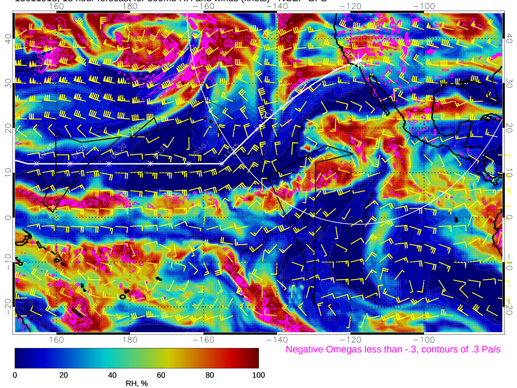
15011918, 18 hour forecast for 500mb RH and winds (knots) - NCEP GFS
