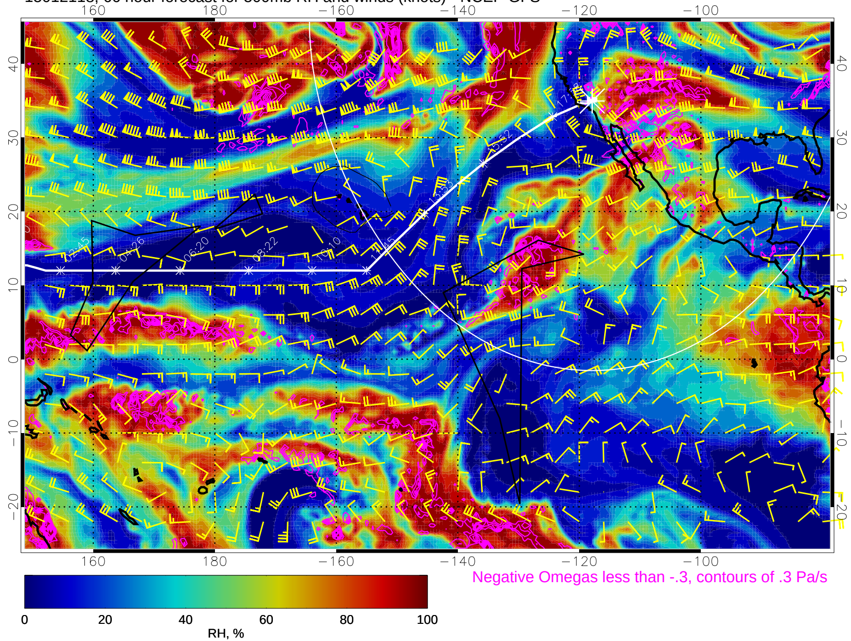
15012118, 66 hour forecast for 500mb RH and winds (knots) - NCEP GFS
