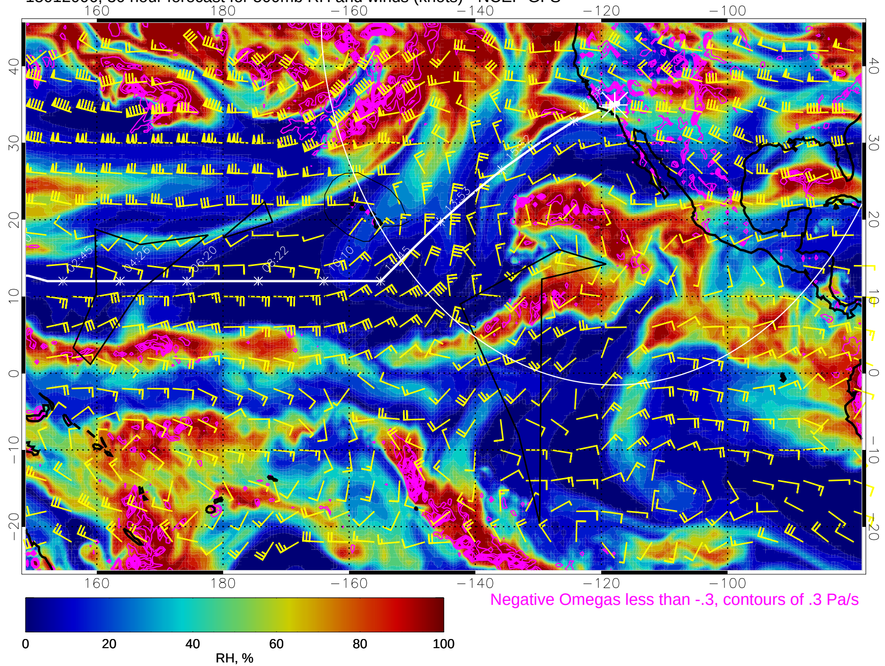
15012006, 30 hour forecast for 500mb RH and winds (knots) - NCEP GFS
