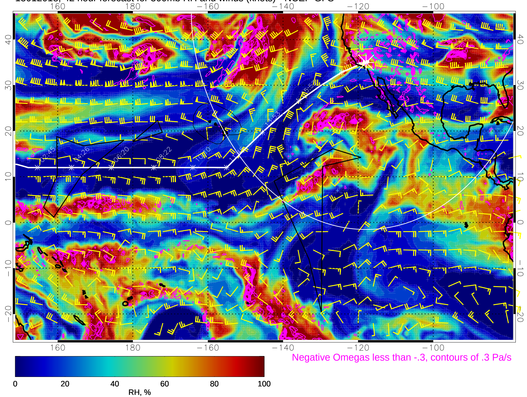
15012018, 42 hour forecast for 500mb RH and winds (knots) - NCEP GFS
