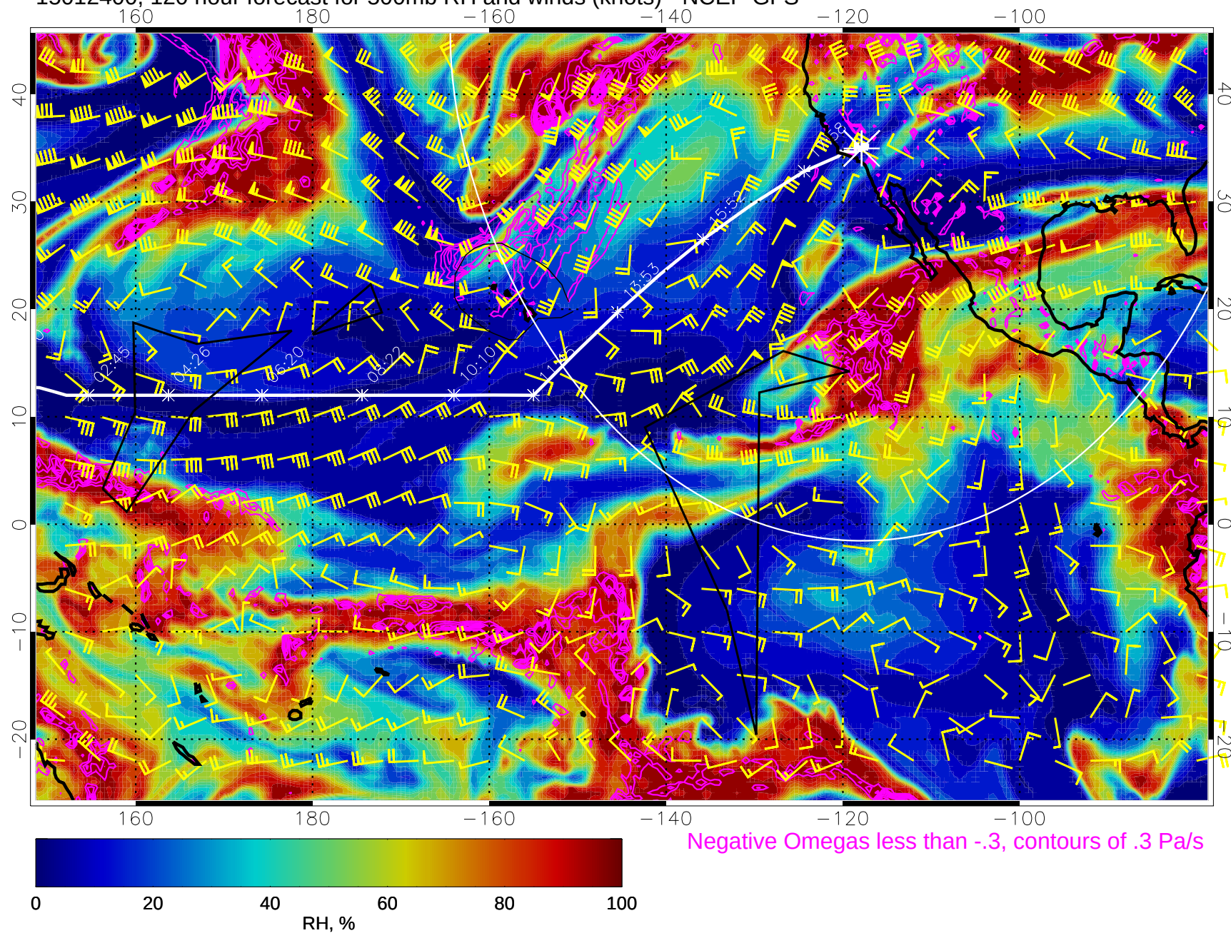
15012400, 120 hour forecast for 500mb RH and winds (knots) - NCEP GFS
