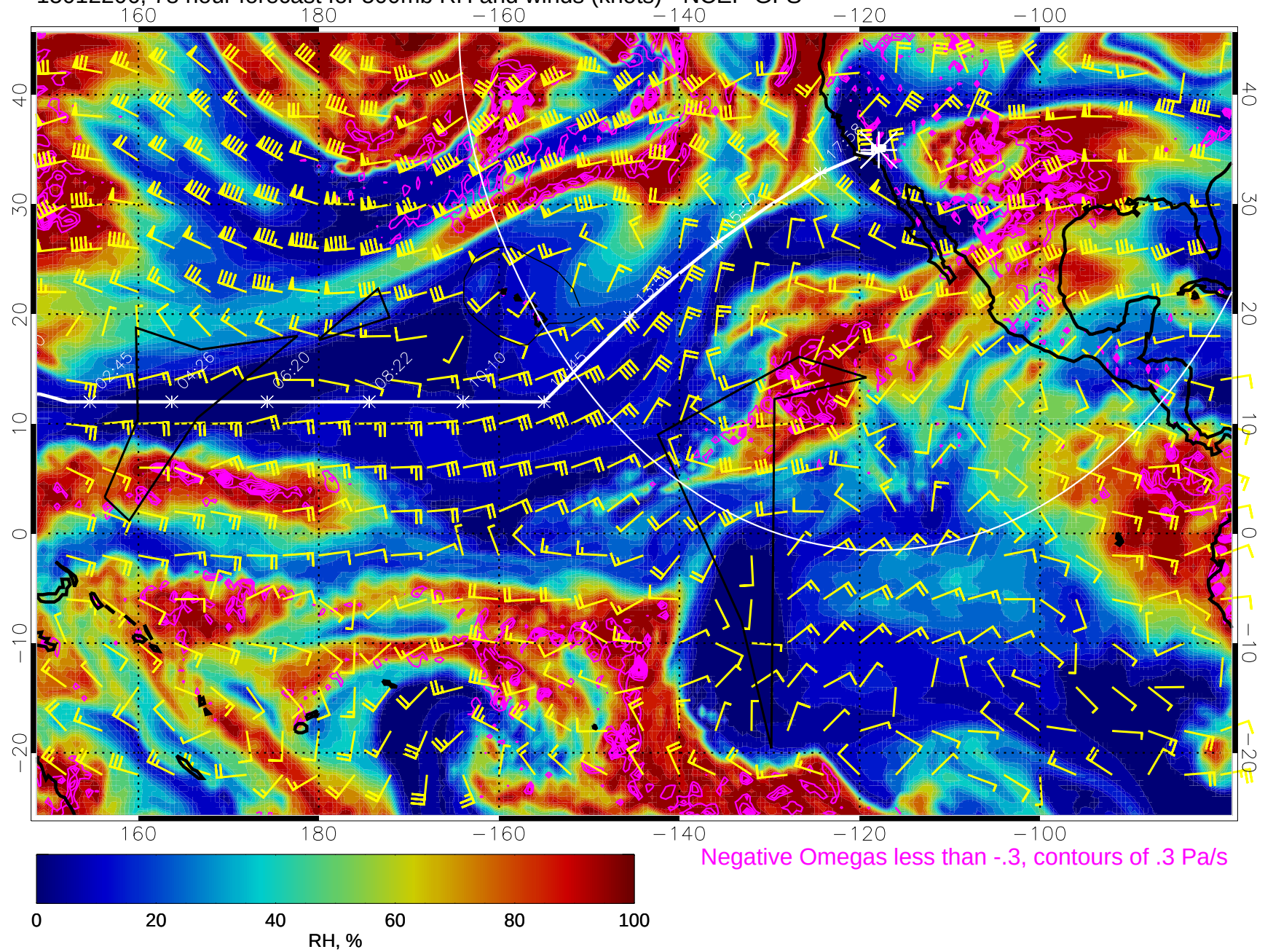
15012206, 78 hour forecast for 500mb RH and winds (knots) - NCEP GFS
