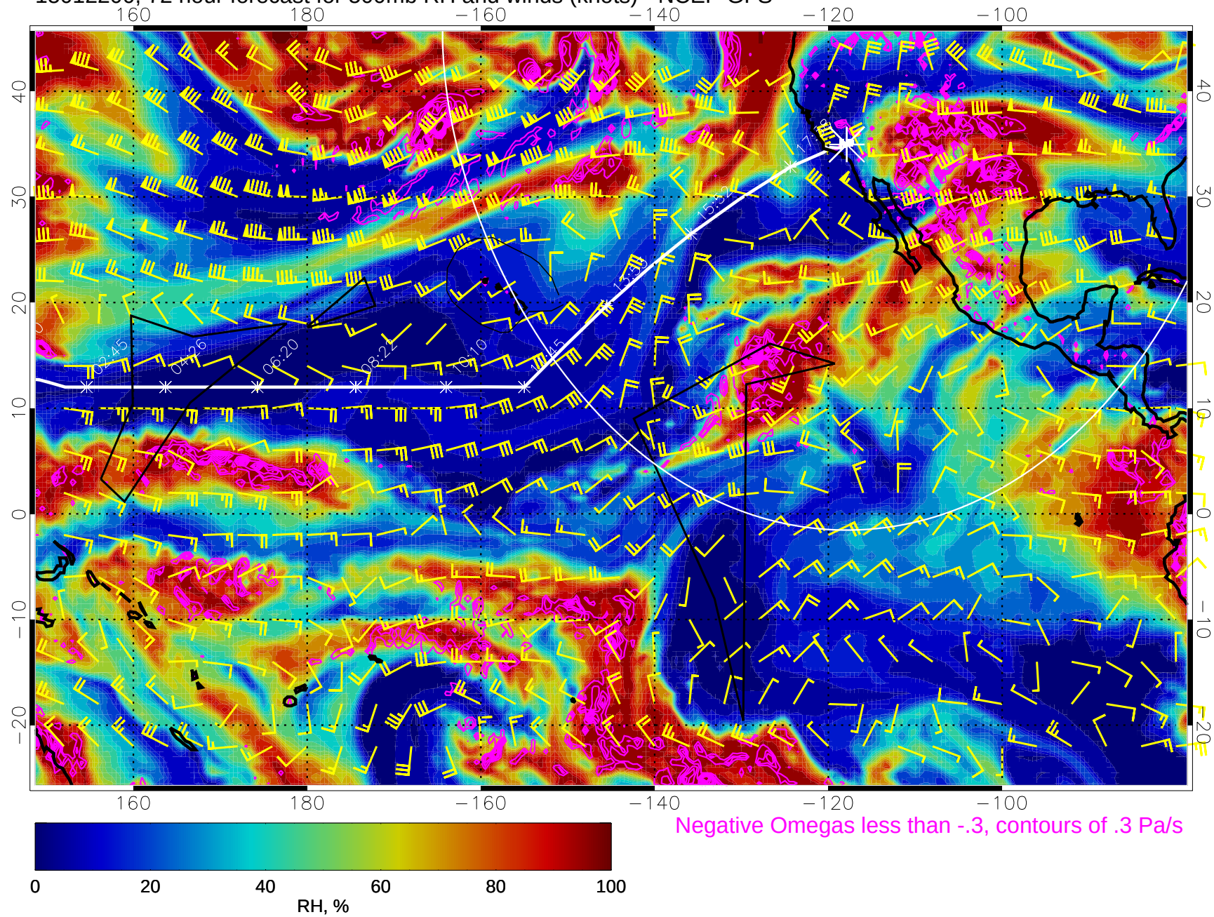
15012200, 72 hour forecast for 500mb RH and winds (knots) - NCEP GFS
