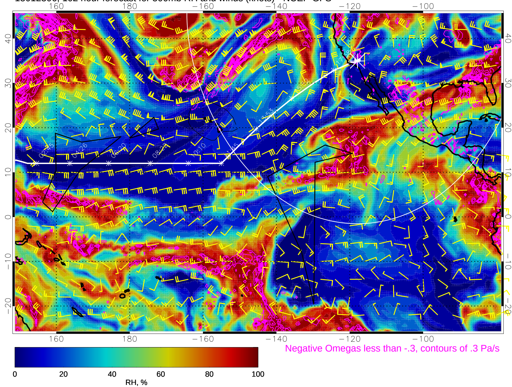
15012306, 102 hour forecast for 500mb RH and winds (knots) - NCEP GFS
