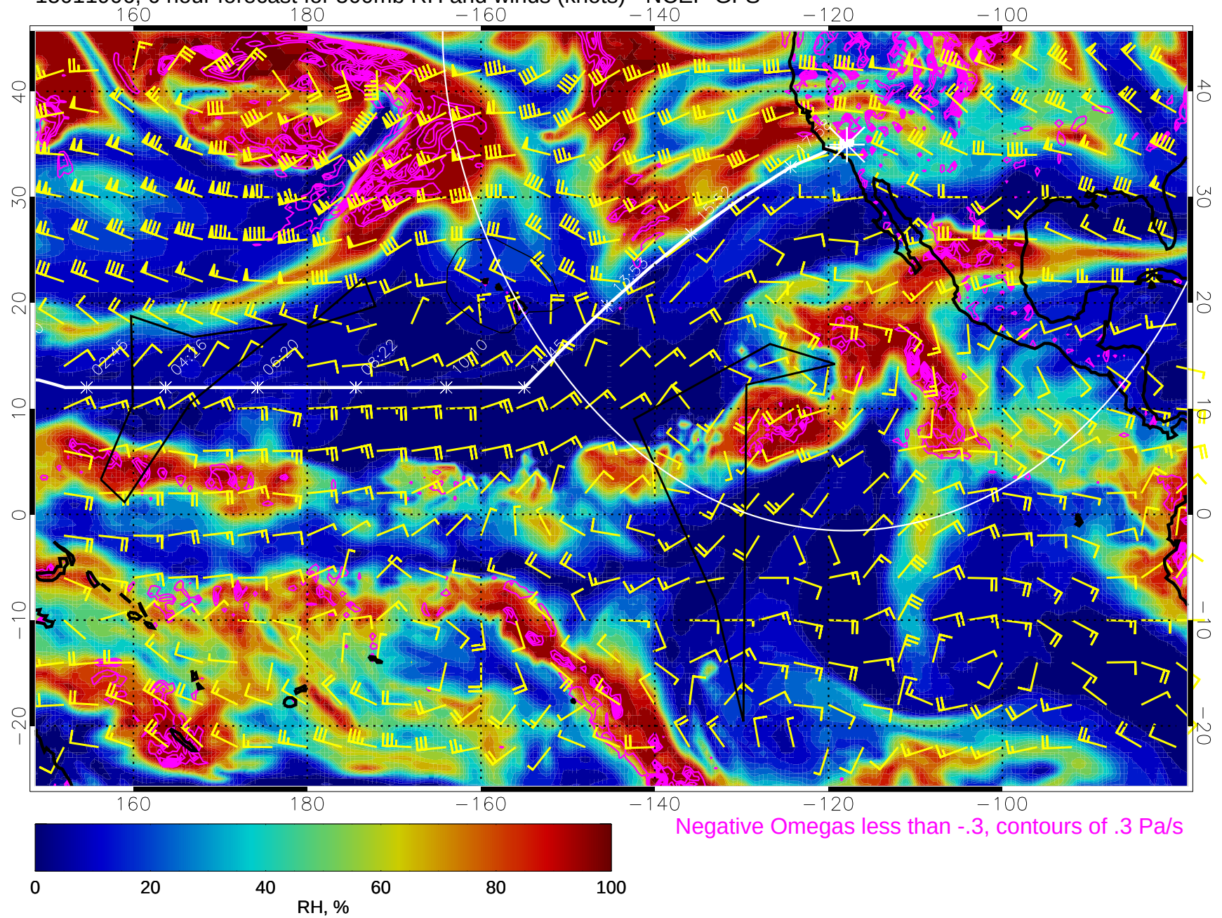
15011906, 6 hour forecast for 500mb RH and winds (knots) - NCEP GFS
