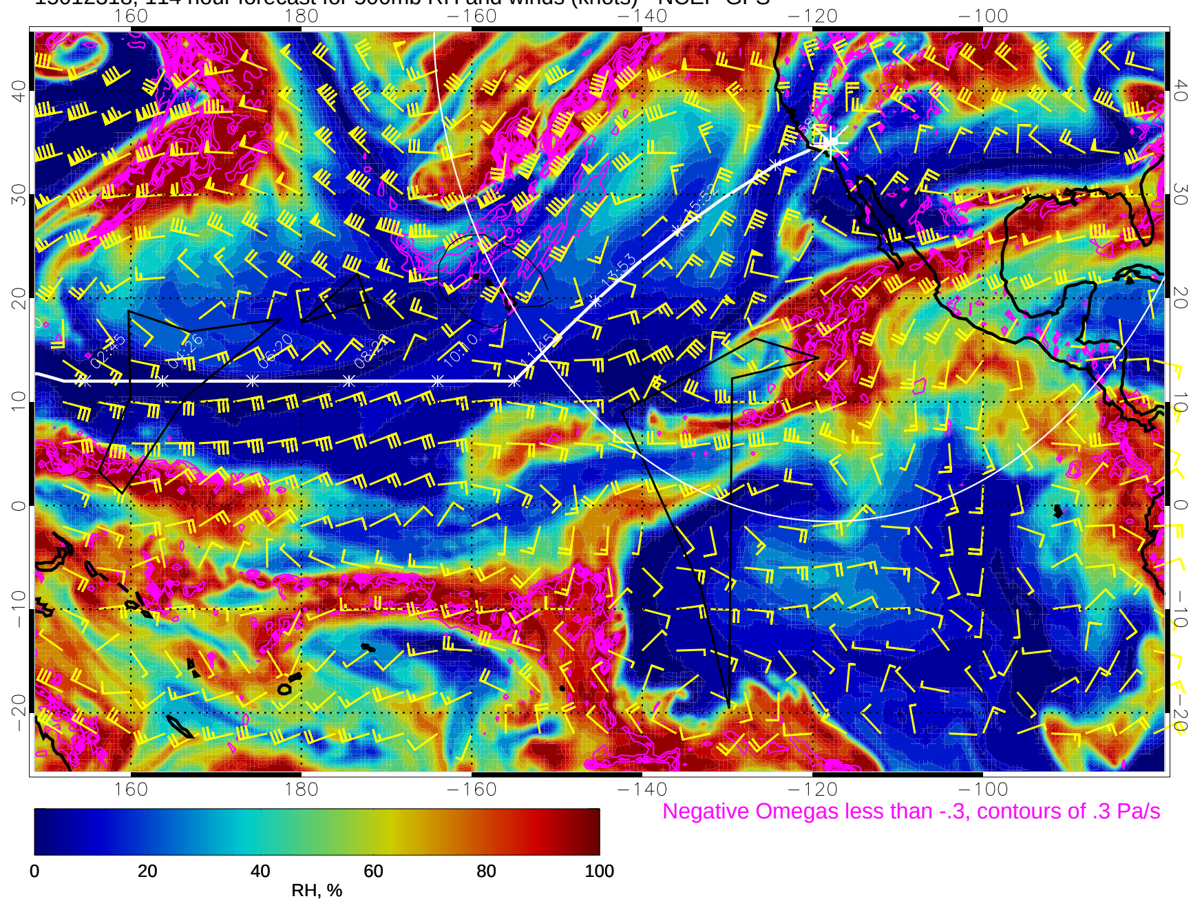
15012318, 114 hour forecast for 500mb RH and winds (knots) - NCEP GFS
