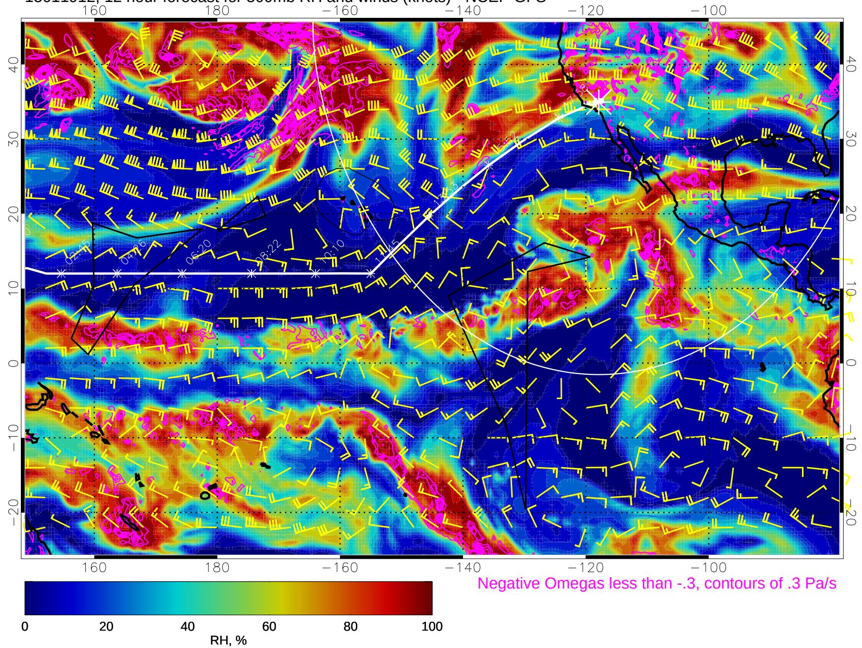
15011912, 12 hour forecast for 500mb RH and winds (knots) - NCEP GFS
