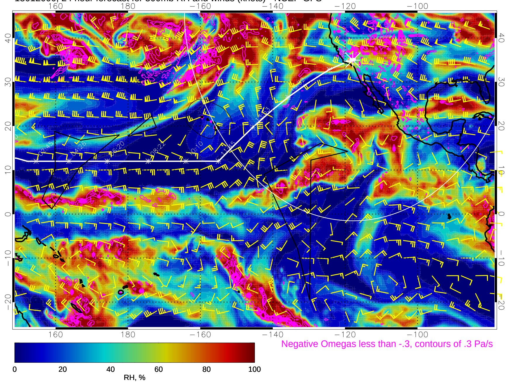
15012000, 24 hour forecast for 500mb RH and winds (knots) - NCEP GFS
