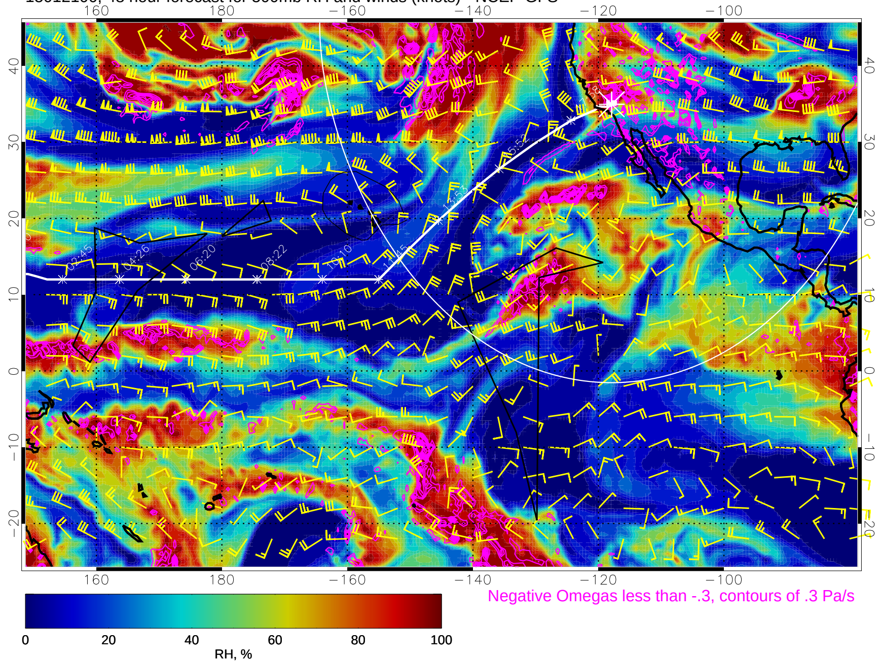
15012100, 48 hour forecast for 500mb RH and winds (knots) - NCEP GFS
