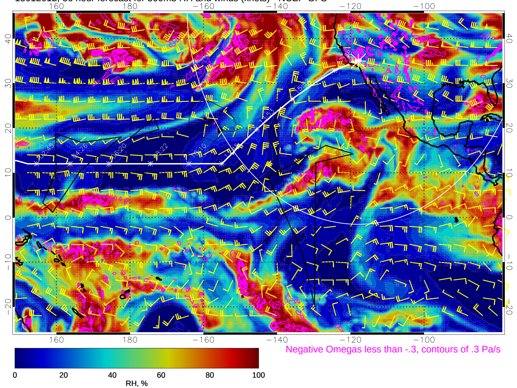
15012012, 36 hour forecast for 500mb RH and winds (knots) - NCEP GFS
