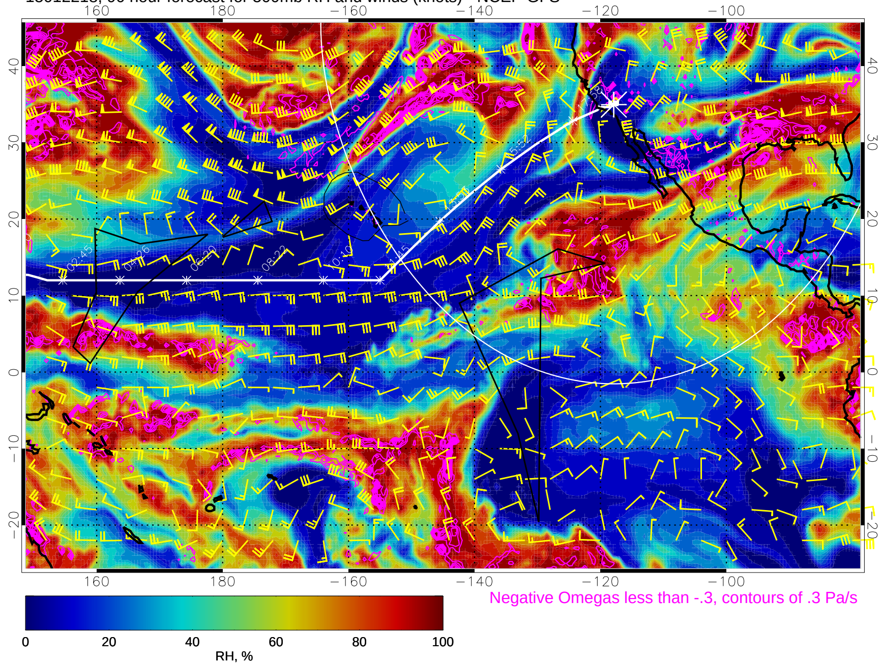
15012218, 90 hour forecast for 500mb RH and winds (knots) - NCEP GFS
