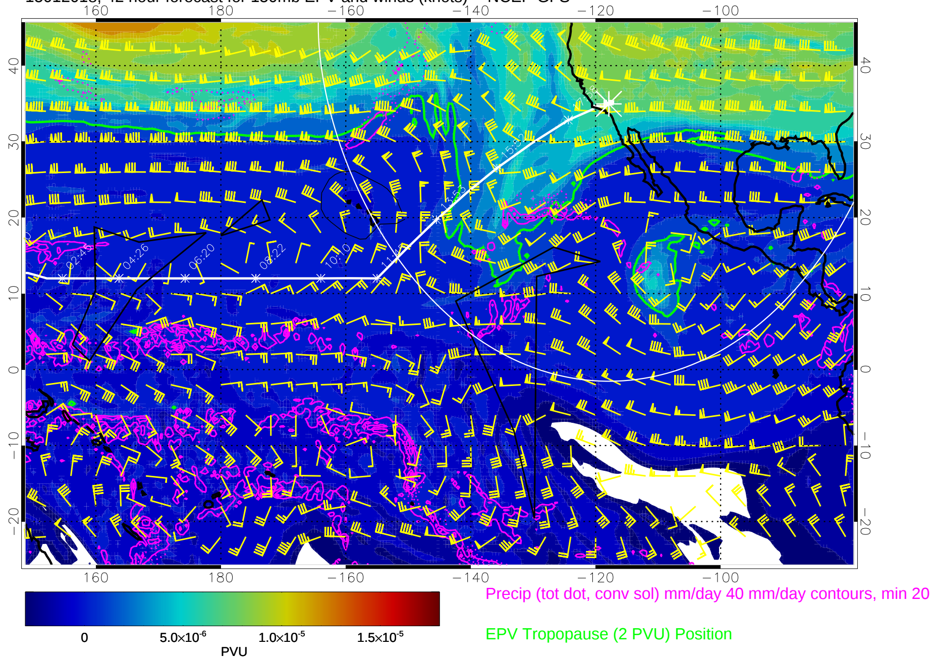
15012018, 42 hour forecast for 150mb EPV and winds (knots) -- NCEP GFS
