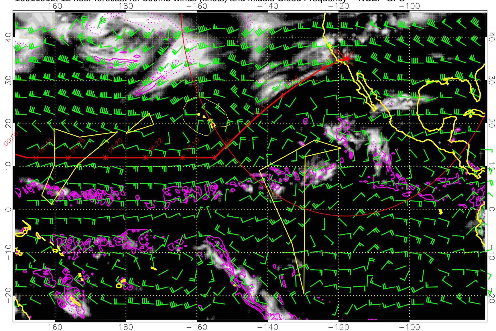
15011912, 12 hour forecast for 500mb winds (knots) and Middle Cloud Frequency -- NCEP GFS
