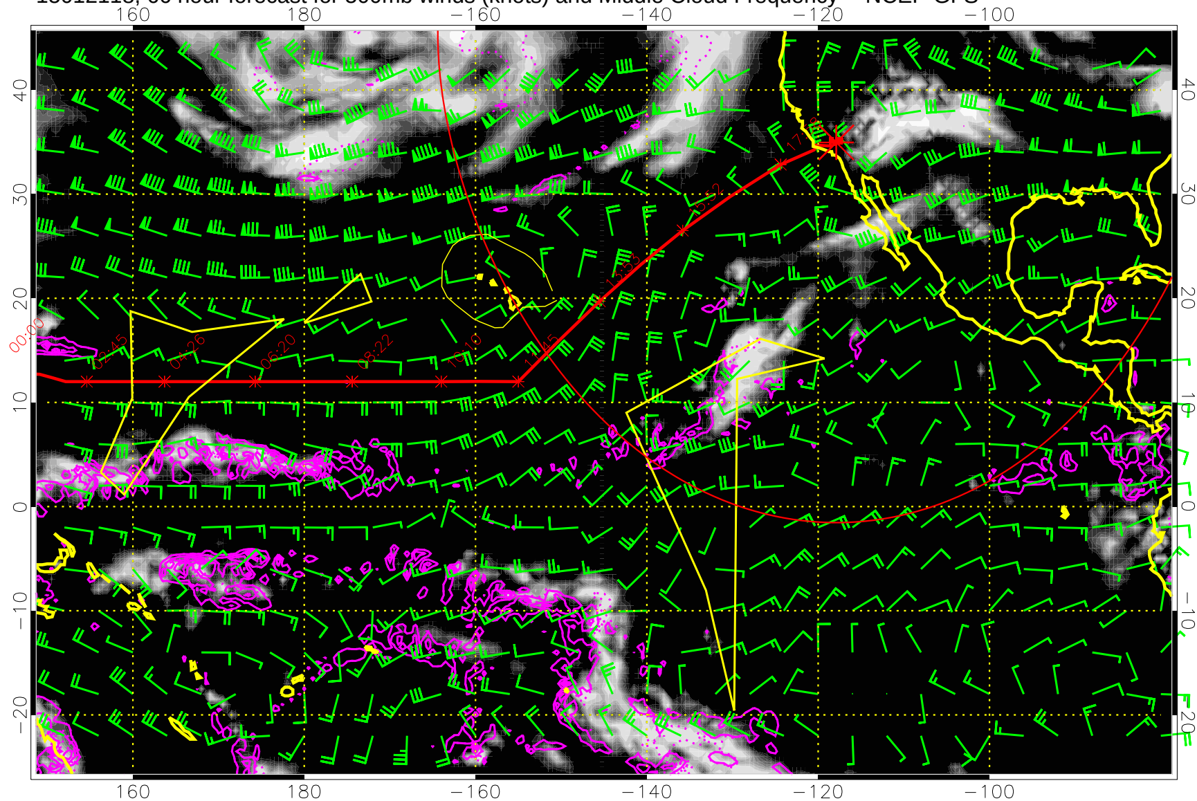
15012118, 66 hour forecast for 500mb winds (knots) and Middle Cloud Frequency -- NCEP GFS
