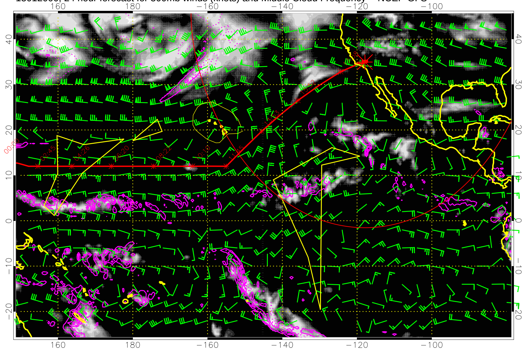
15012000, 24 hour forecast for 500mb winds (knots) and Middle Cloud Frequency -- NCEP GFS
