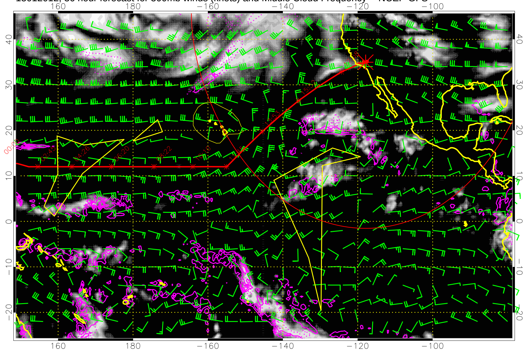
15012012, 36 hour forecast for 500mb winds (knots) and Middle Cloud Frequency -- NCEP GFS
