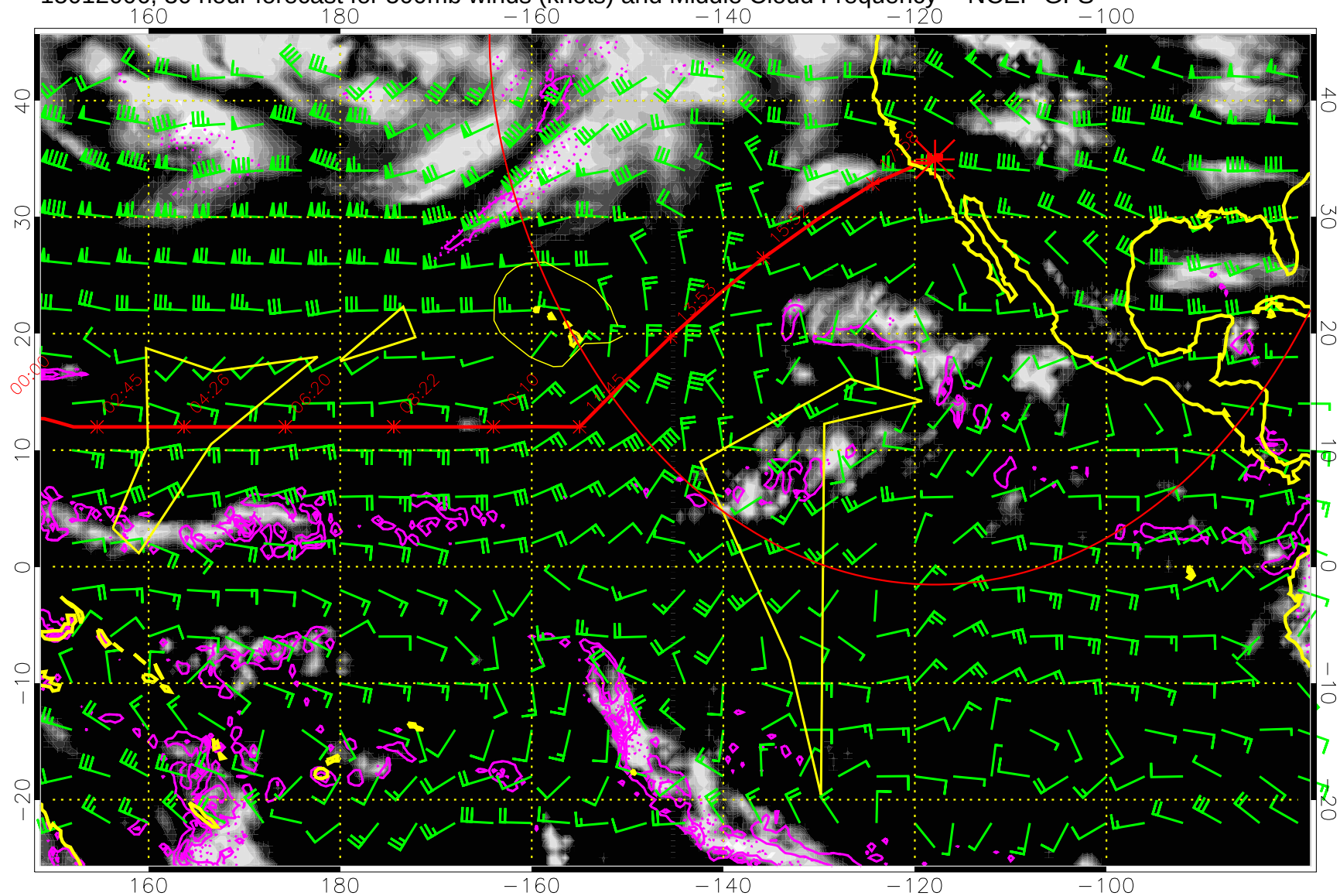
15012006, 30 hour forecast for 500mb winds (knots) and Middle Cloud Frequency -- NCEP GFS
