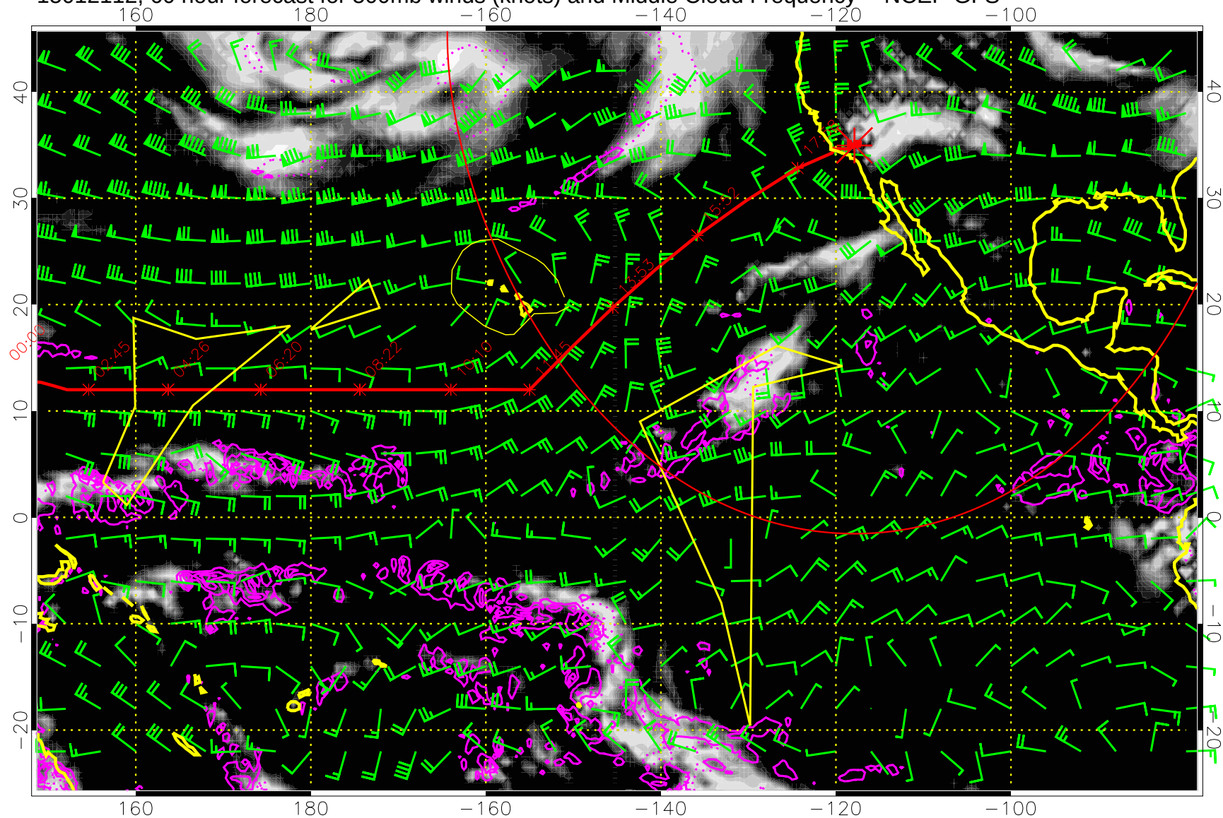
15012112, 60 hour forecast for 500mb winds (knots) and Middle Cloud Frequency -- NCEP GFS
