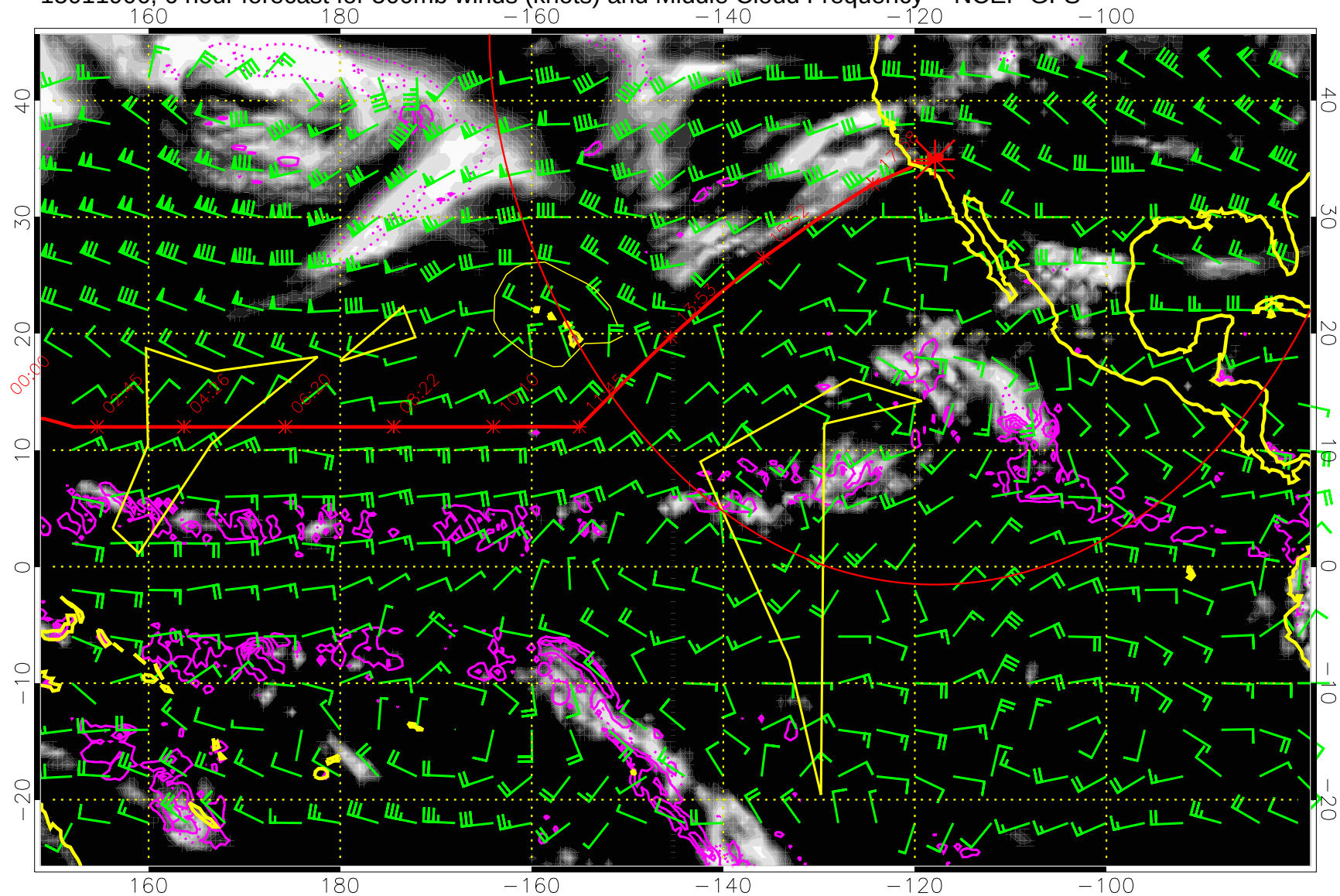
15011906, 6 hour forecast for 500mb winds (knots) and Middle Cloud Frequency -- NCEP GFS
