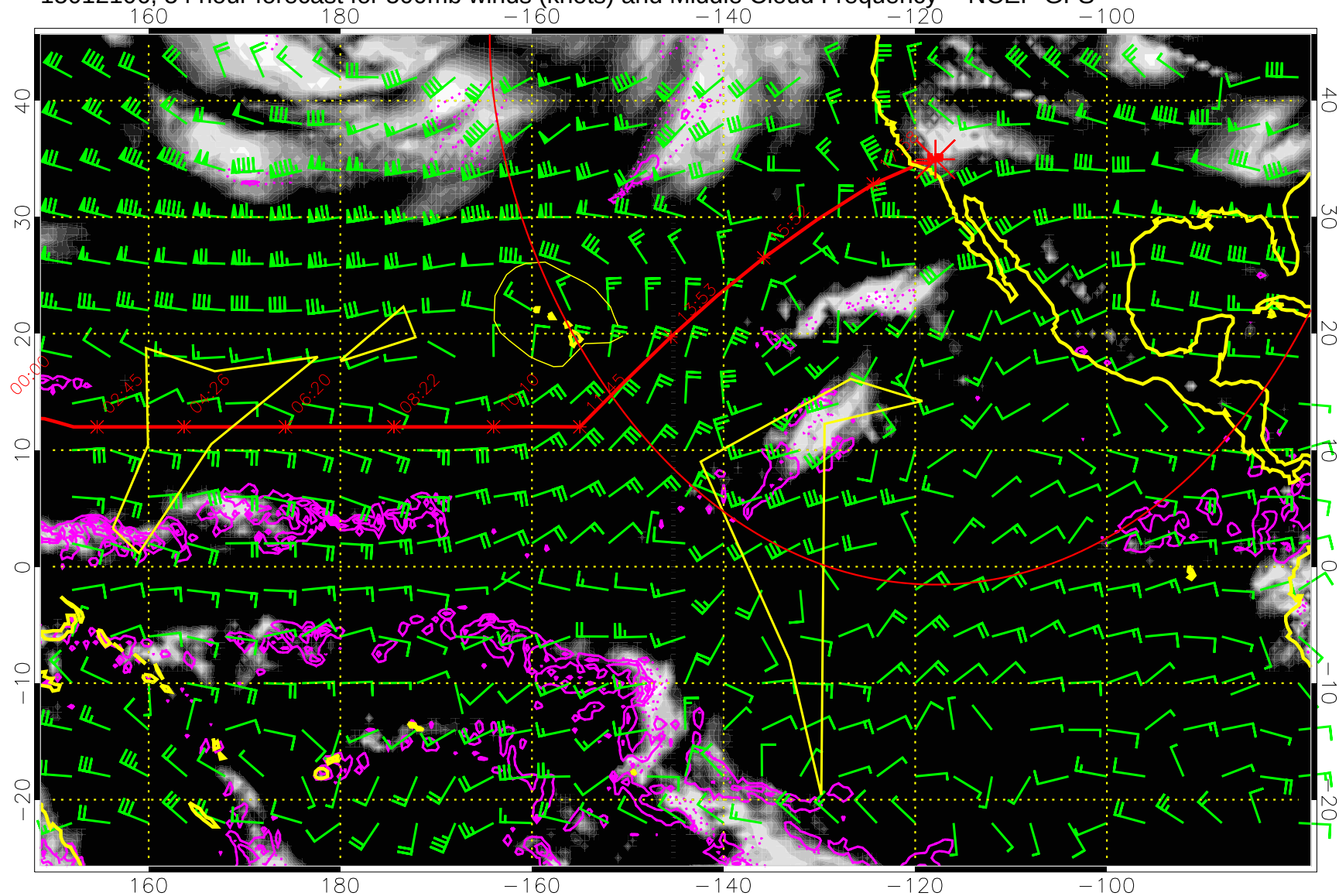
15012106, 54 hour forecast for 500mb winds (knots) and Middle Cloud Frequency -- NCEP GFS
