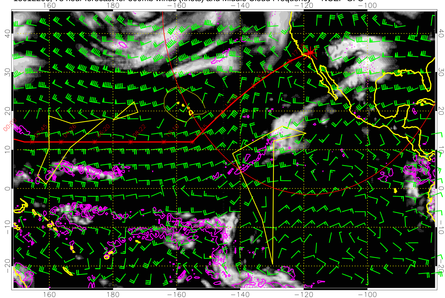
15012206, 78 hour forecast for 500mb winds (knots) and Middle Cloud Frequency -- NCEP GFS
