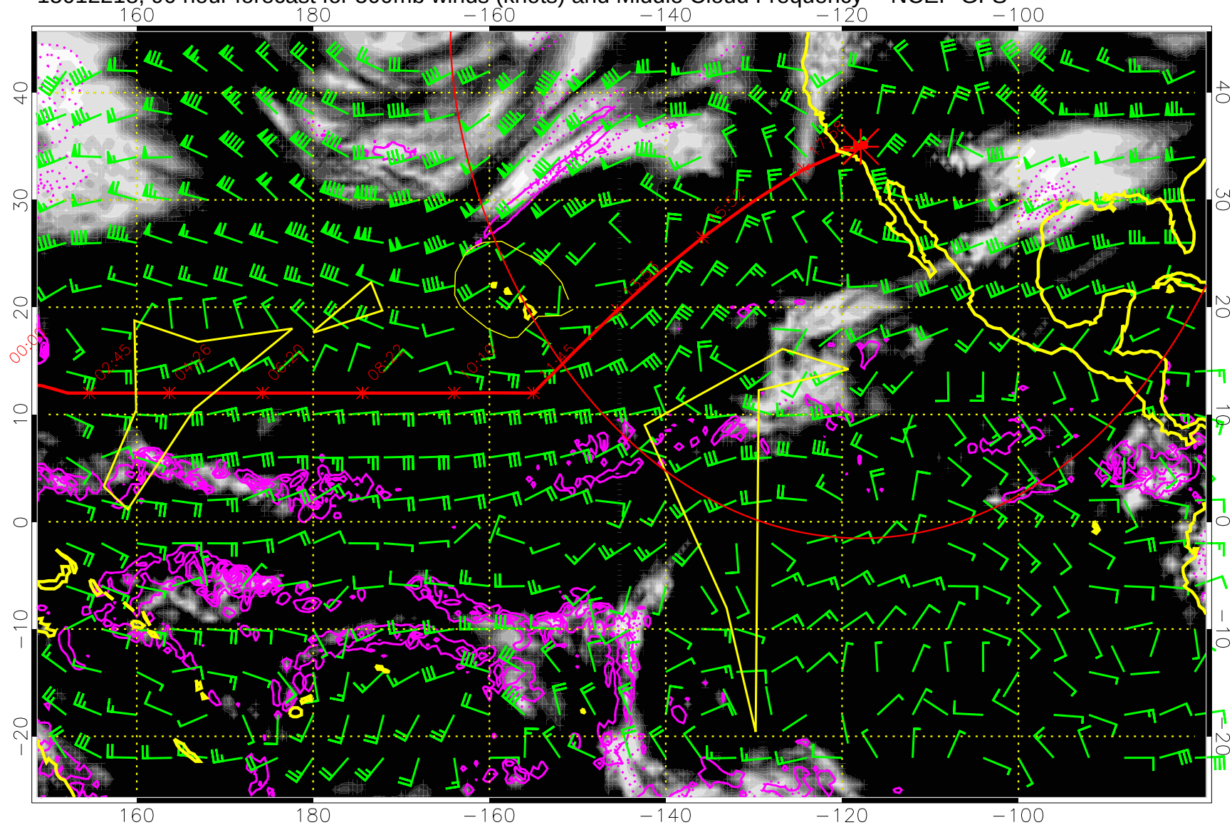
15012218, 90 hour forecast for 500mb winds (knots) and Middle Cloud Frequency -- NCEP GFS
