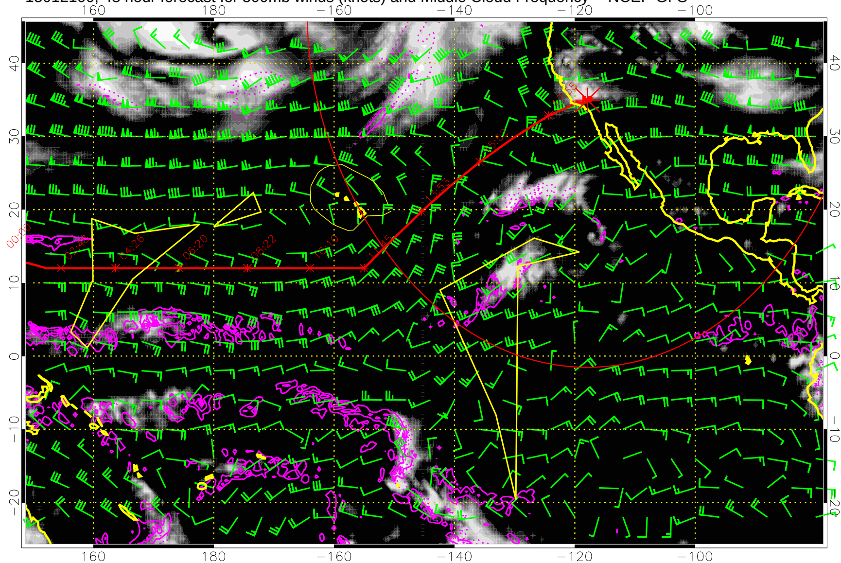
15012100, 48 hour forecast for 500mb winds (knots) and Middle Cloud Frequency -- NCEP GFS
