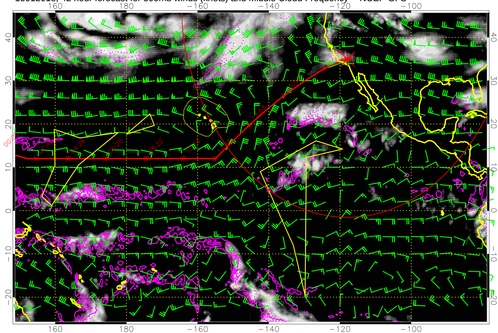
15012018, 42 hour forecast for 500mb winds (knots) and Middle Cloud Frequency -- NCEP GFS
