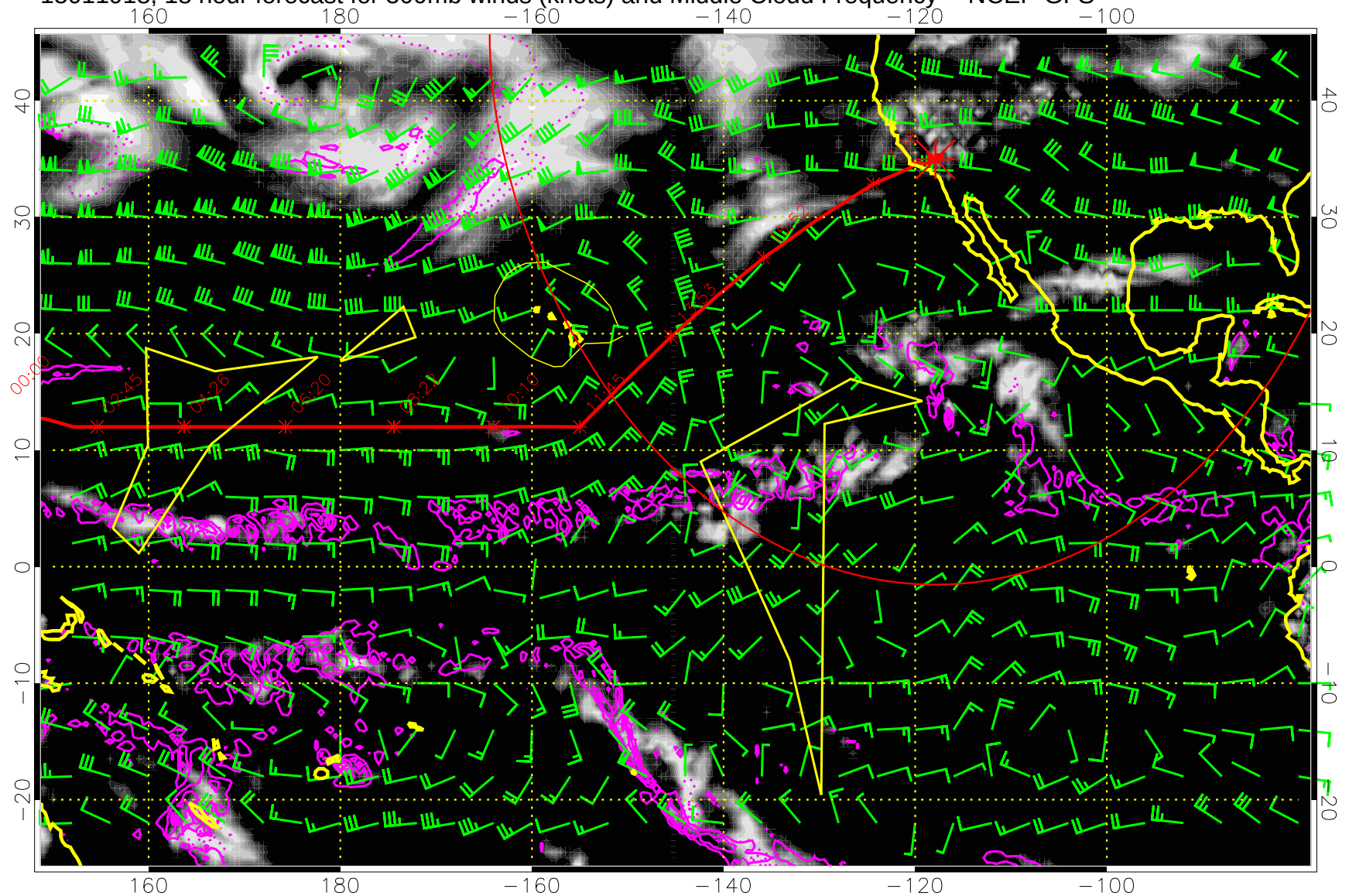
15011918, 18 hour forecast for 500mb winds (knots) and Middle Cloud Frequency -- NCEP GFS
