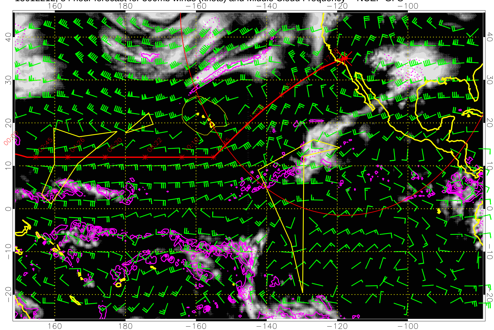
15012212, 84 hour forecast for 500mb winds (knots) and Middle Cloud Frequency -- NCEP GFS
