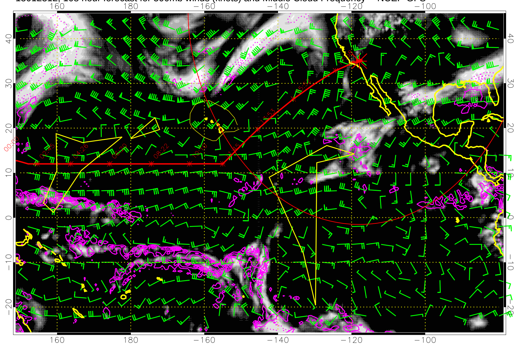
15012312, 108 hour forecast for 500mb winds (knots) and Middle Cloud Frequency -- NCEP GFS
