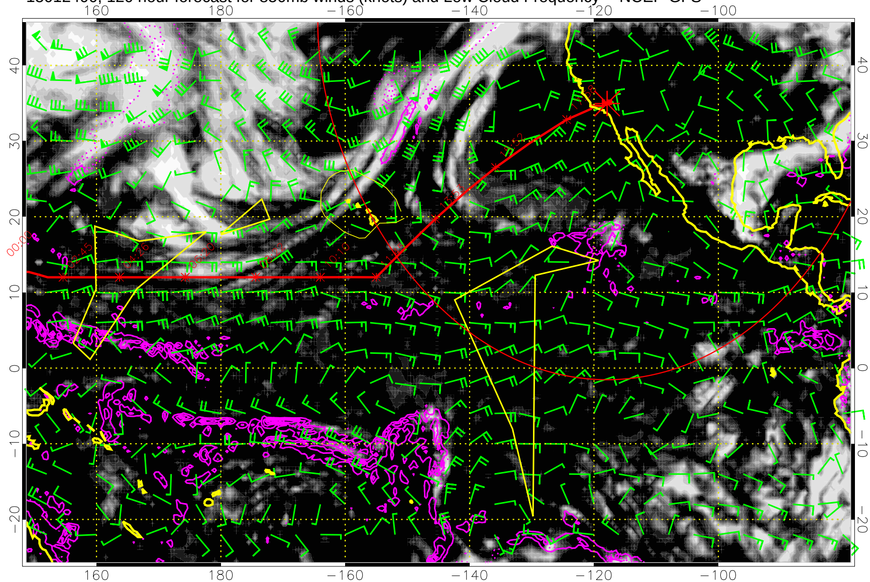
15012400, 120 hour forecast for 850mb winds (knots) and Low Cloud Frequency -- NCEP GFS
