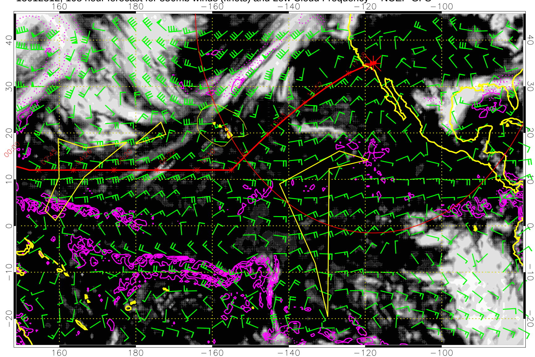
15012312, 108 hour forecast for 850mb winds (knots) and Low Cloud Frequency -- NCEP GFS
