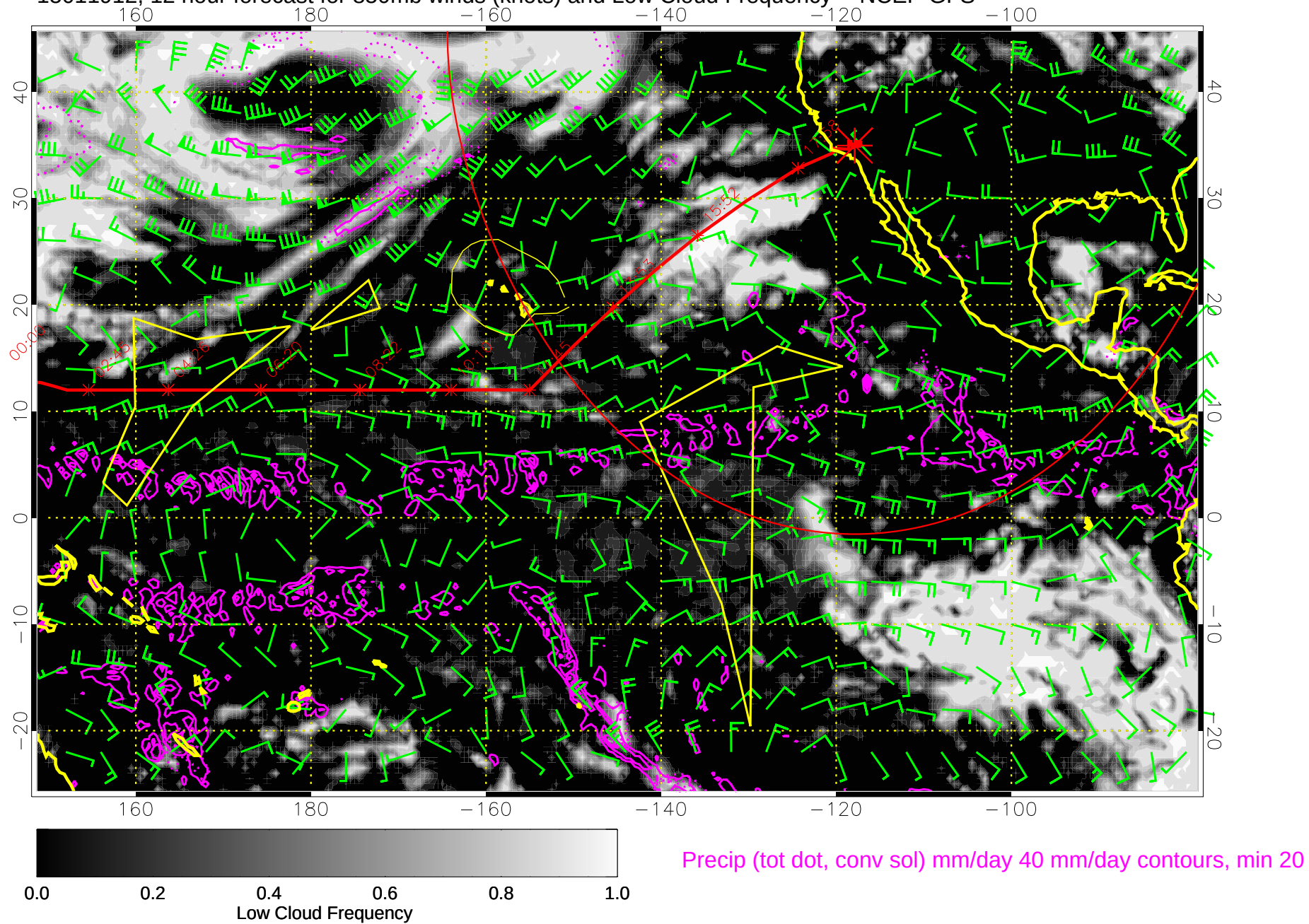
15011912, 12 hour forecast for 850mb winds (knots) and Low Cloud Frequency -- NCEP GFS
