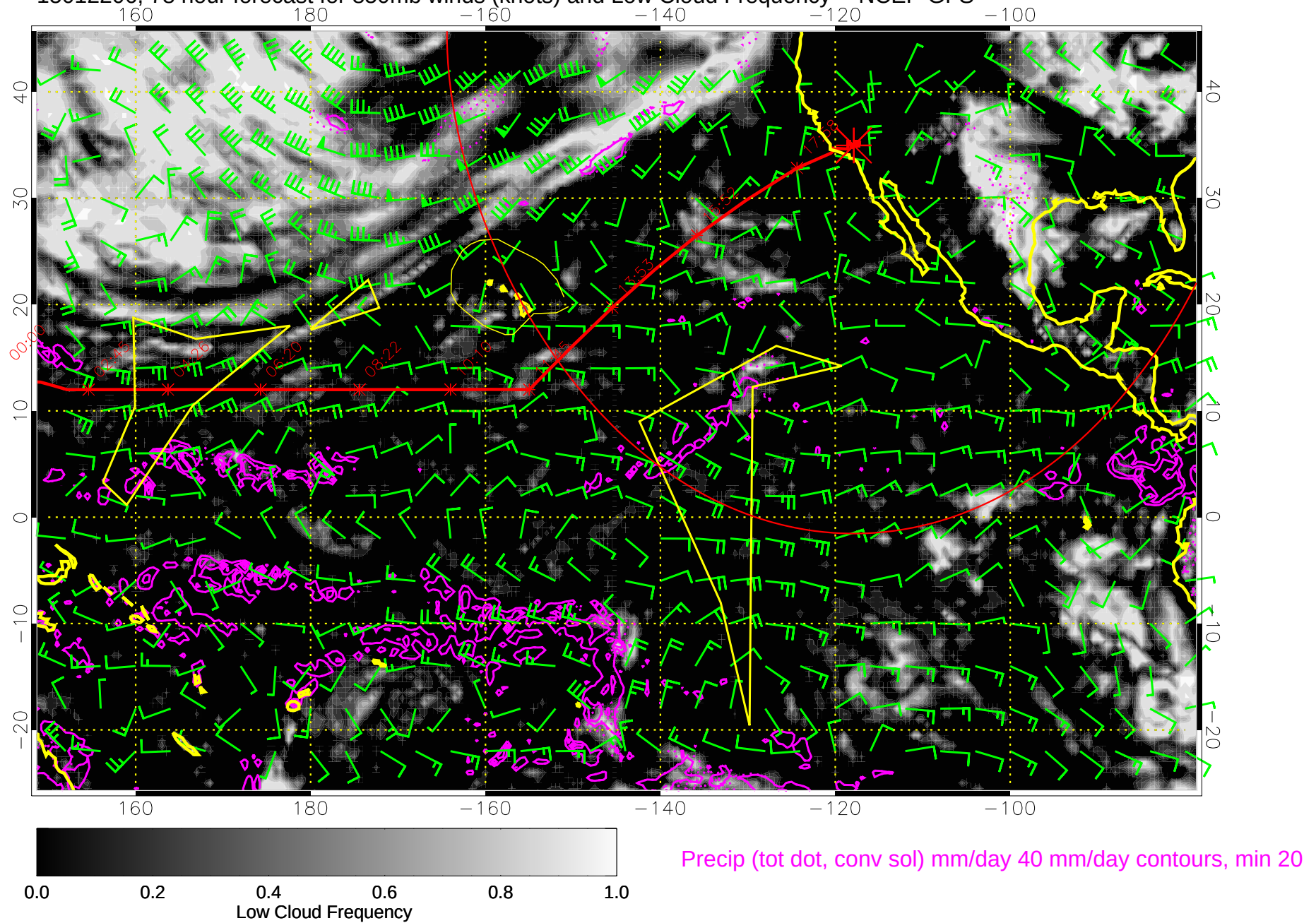
15012206, 78 hour forecast for 850mb winds (knots) and Low Cloud Frequency -- NCEP GFS
