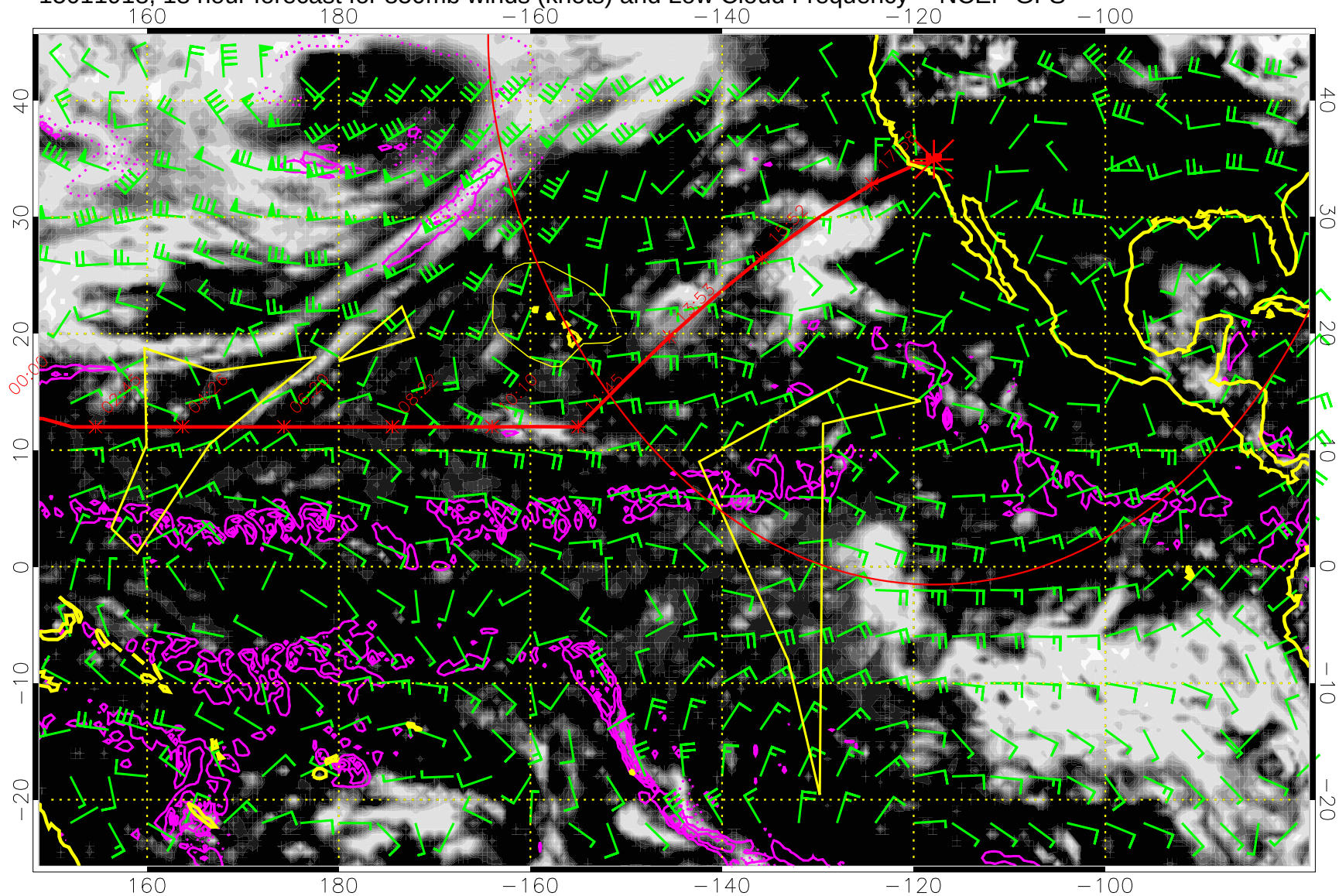
15011918, 18 hour forecast for 850mb winds (knots) and Low Cloud Frequency -- NCEP GFS
