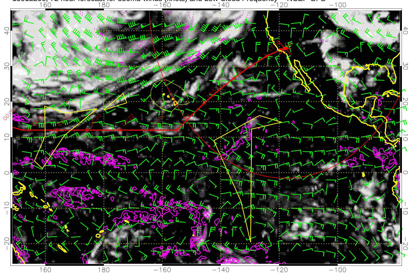
15012200, 72 hour forecast for 850mb winds (knots) and Low Cloud Frequency -- NCEP GFS
