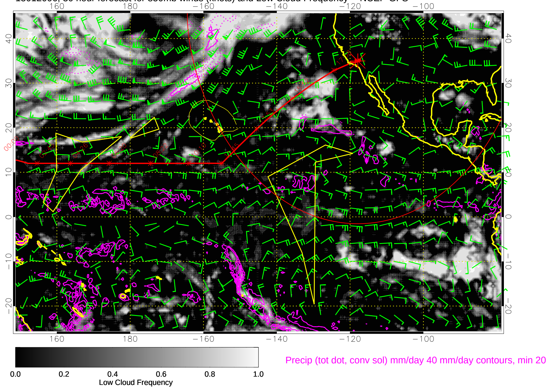
15012006, 30 hour forecast for 850mb winds (knots) and Low Cloud Frequency -- NCEP GFS
