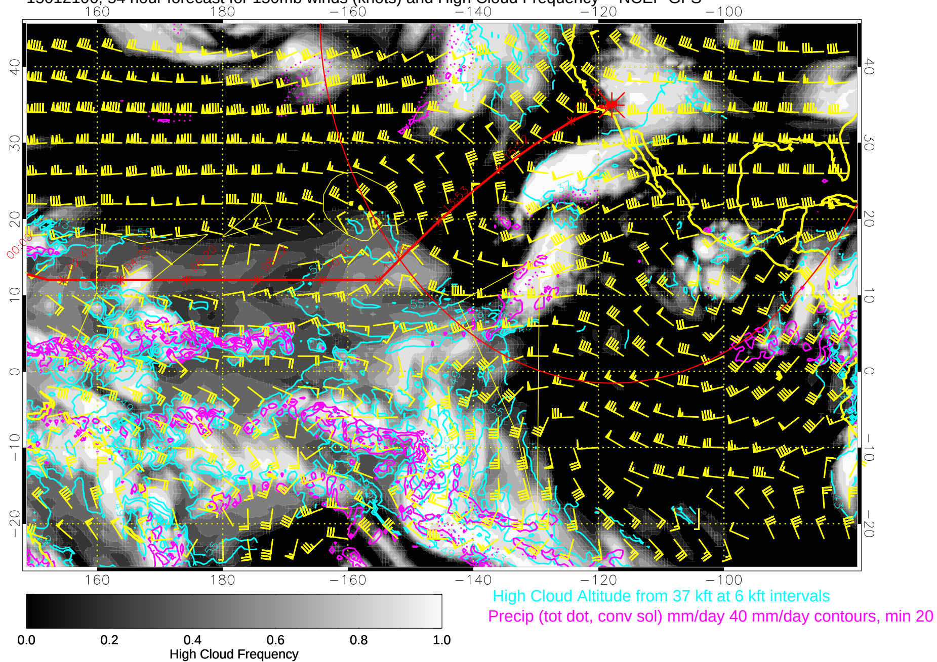
15012106, 54 hour forecast for 150mb winds (knots) and High Cloud Frequency -- NCEP GFS
