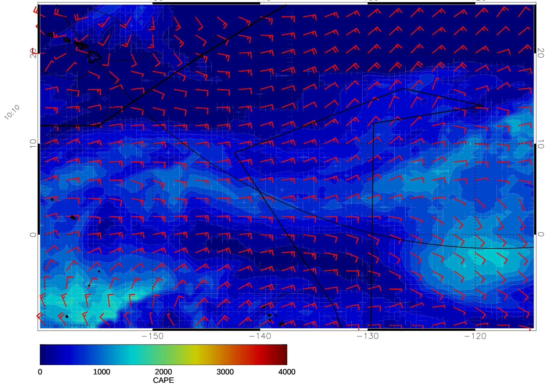
15012400, 120 hour forecast for CAPE and surface winds (knots) -- NCEP GFS
