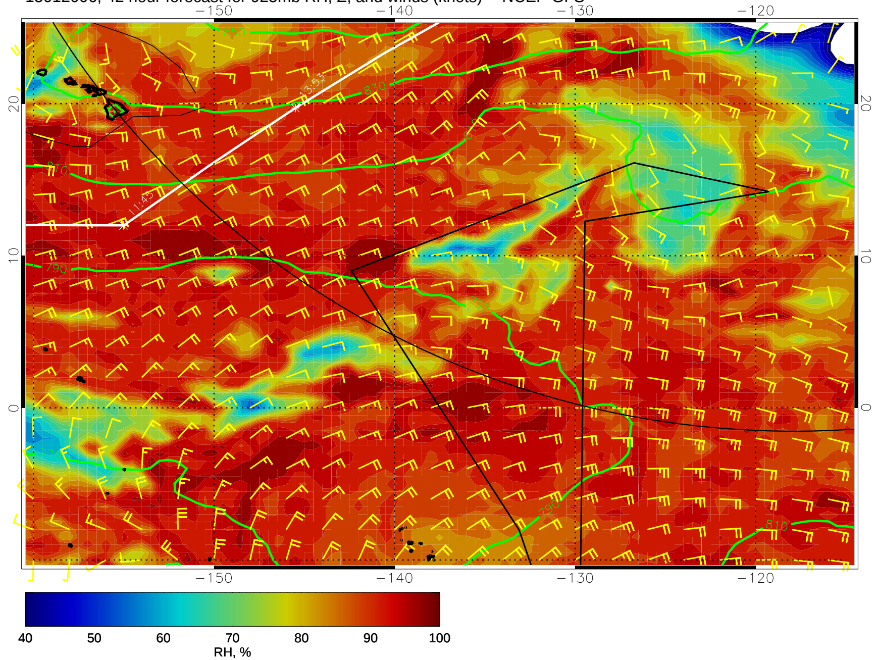
15012006, 42 hour forecast for 925mb RH, Z, and winds (knots) -- NCEP GFS
