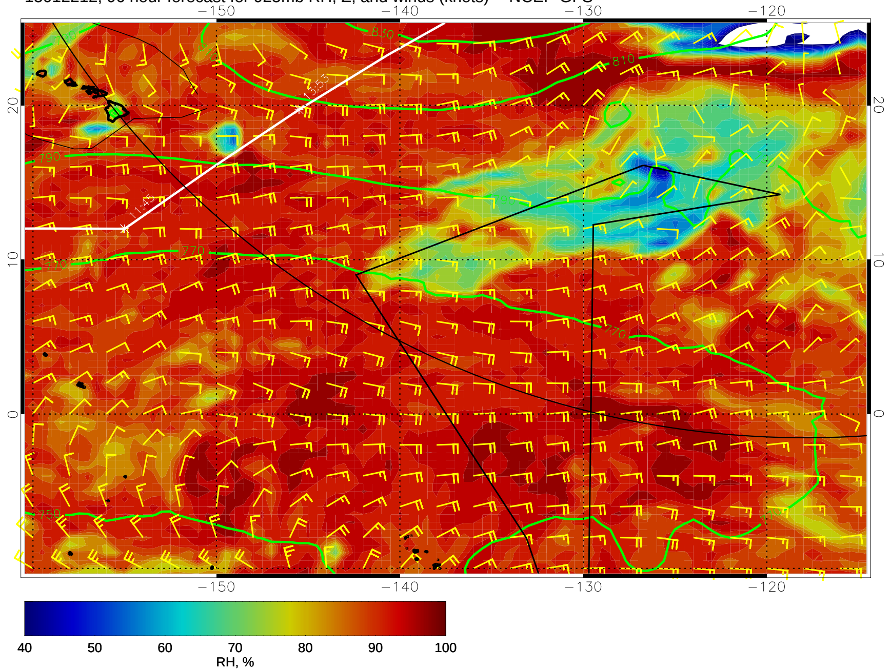
15012212, 96 hour forecast for 925mb RH, Z, and winds (knots) -- NCEP GFS
