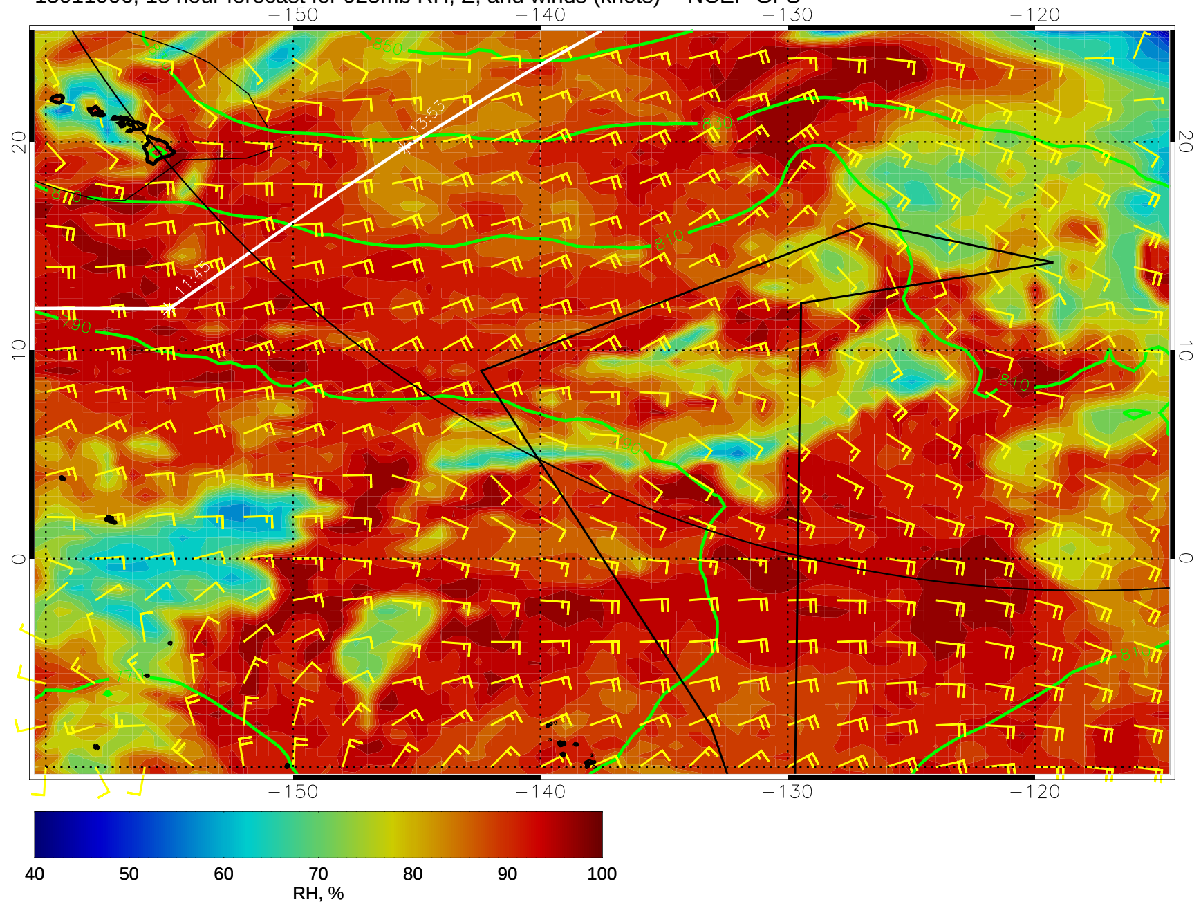
15011906, 18 hour forecast for 925mb RH, Z, and winds (knots) -- NCEP GFS
