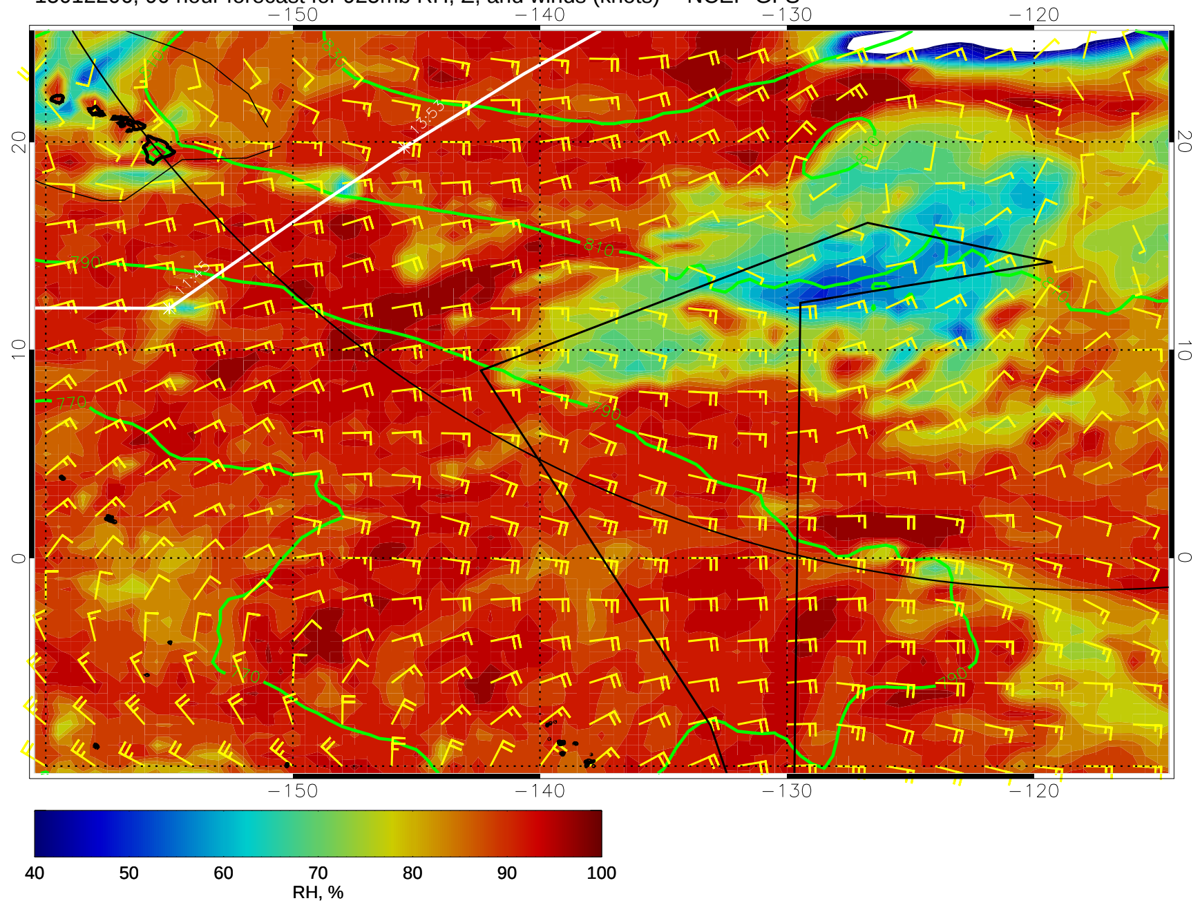
15012206, 90 hour forecast for 925mb RH, Z, and winds (knots) -- NCEP GFS
