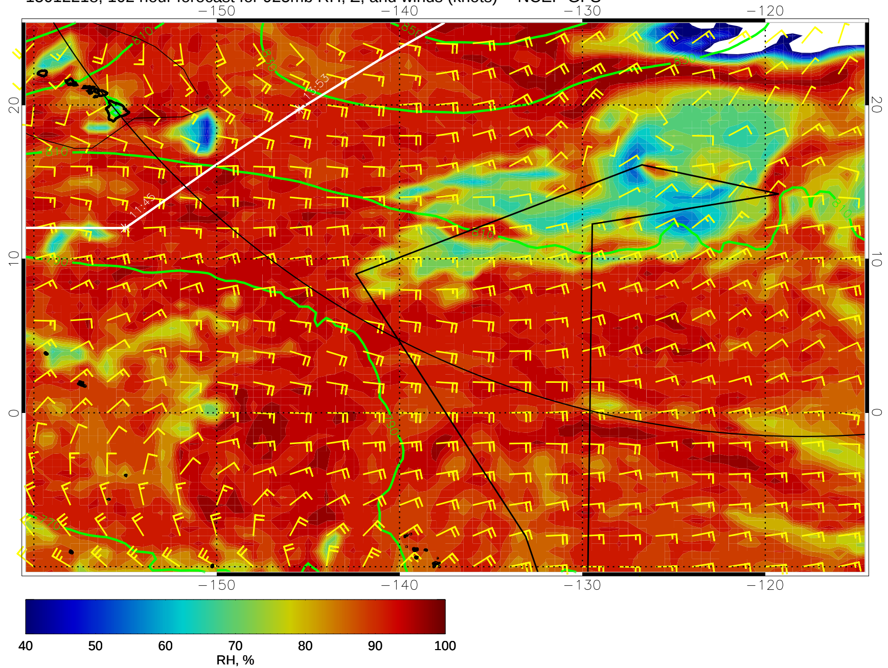
15012218, 102 hour forecast for 925mb RH, Z, and winds (knots) -- NCEP GFS
