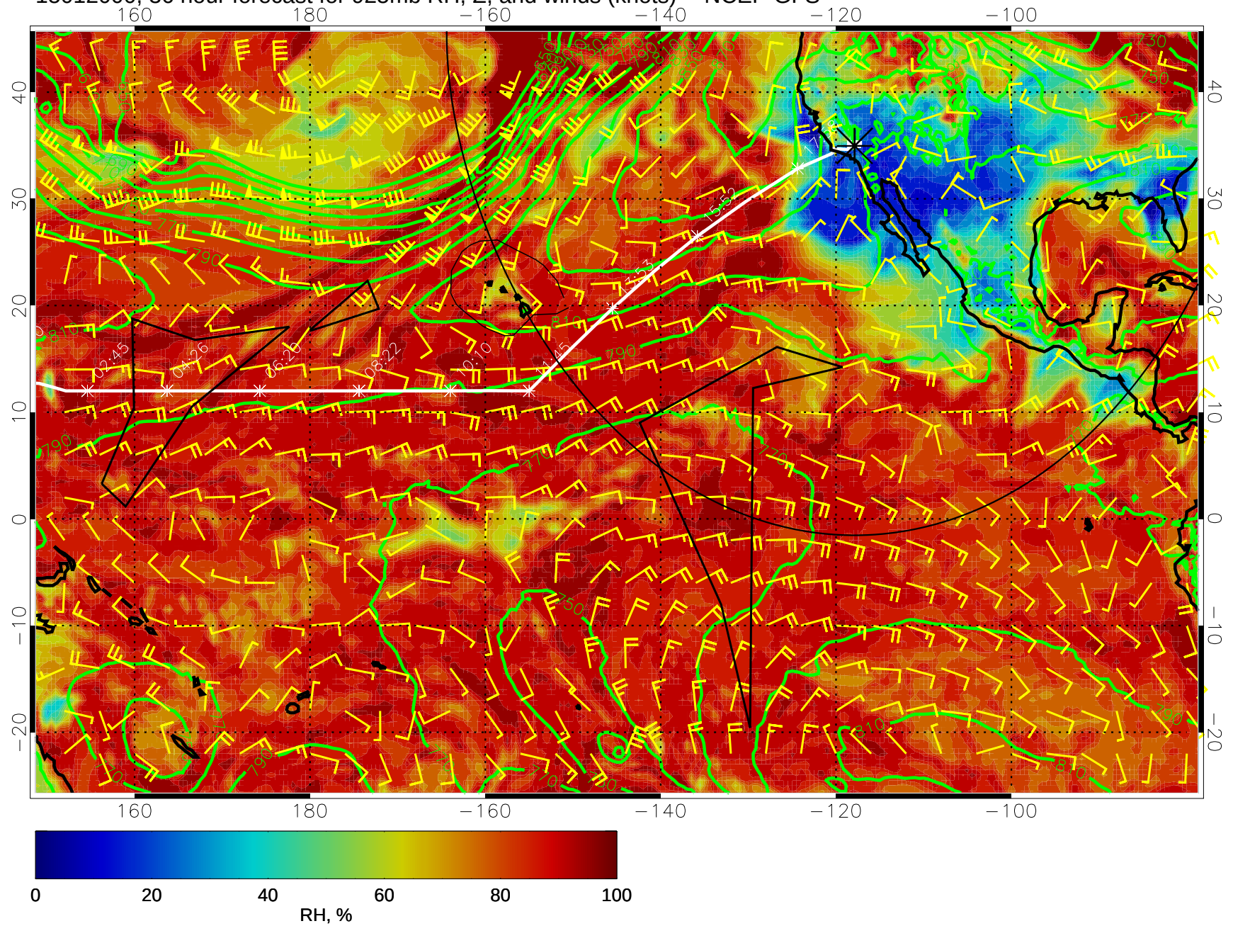
15012000, 36 hour forecast for 925mb RH, Z, and winds (knots) -- NCEP GFS
