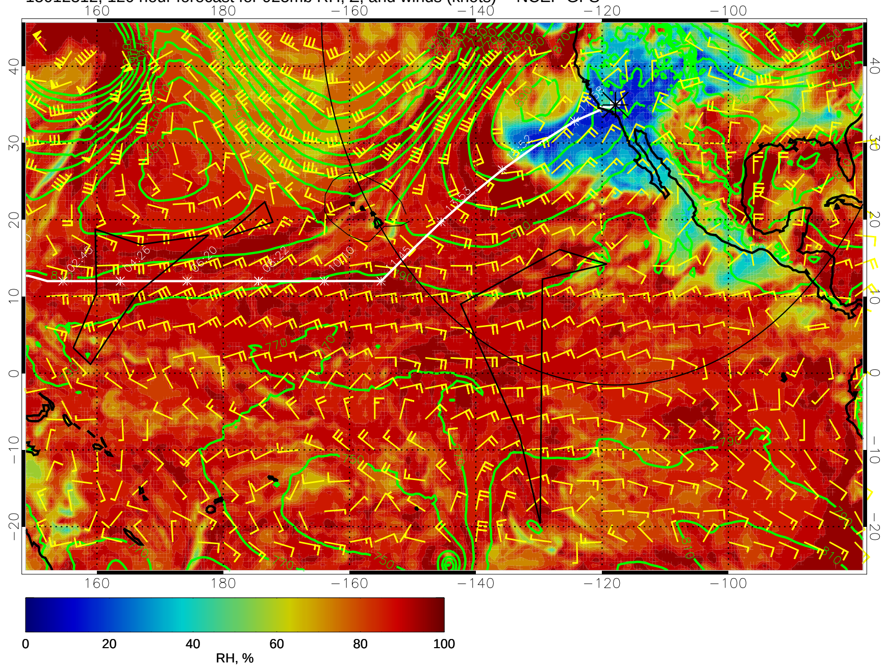
15012312, 120 hour forecast for 925mb RH, Z, and winds (knots) -- NCEP GFS
