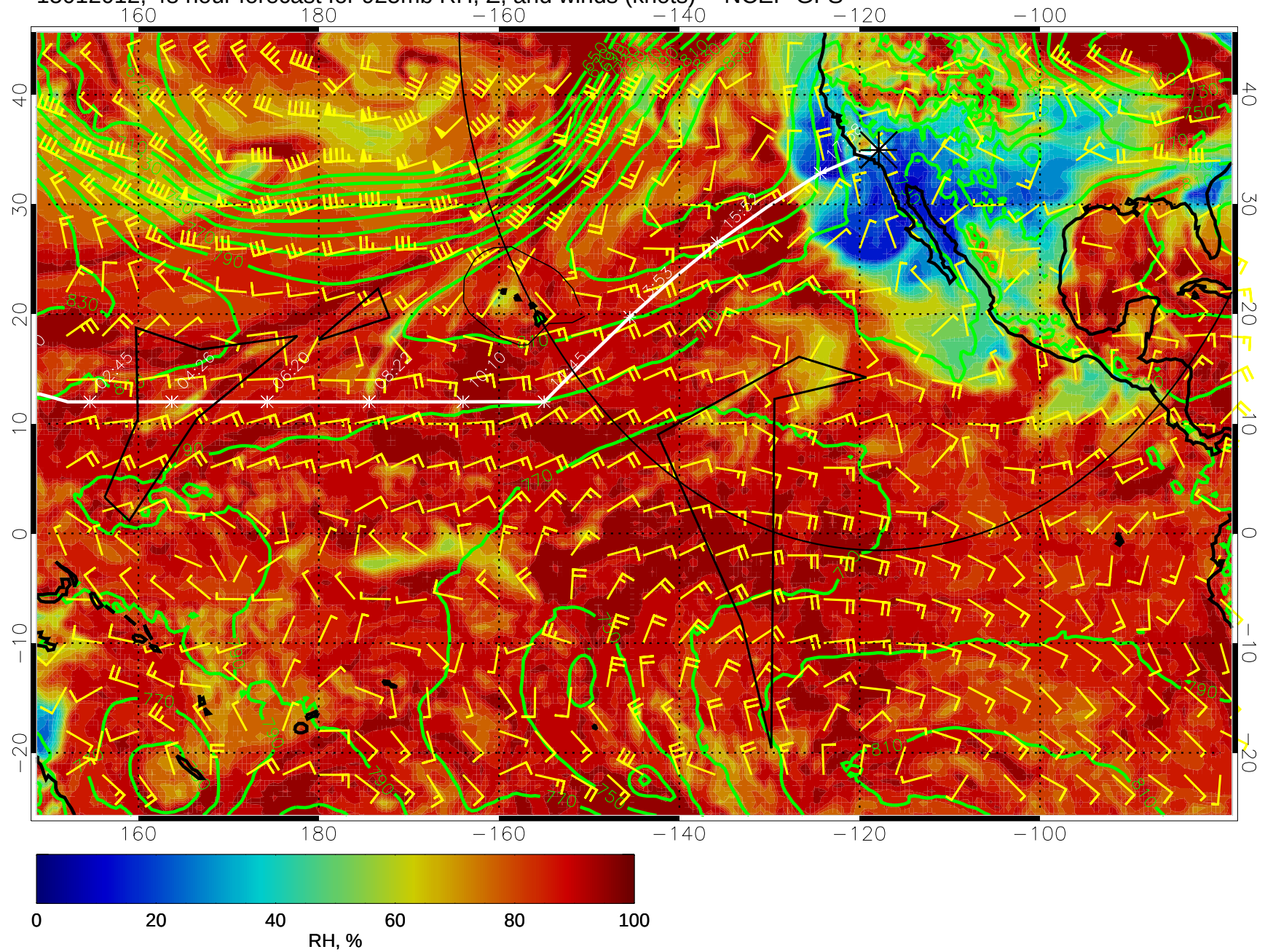
15012012, 48 hour forecast for 925mb RH, Z, and winds (knots) -- NCEP GFS
