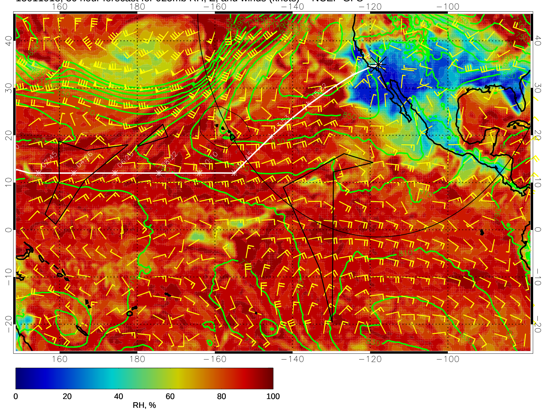
15011918, 30 hour forecast for 925mb RH, Z, and winds (knots) -- NCEP GFS
