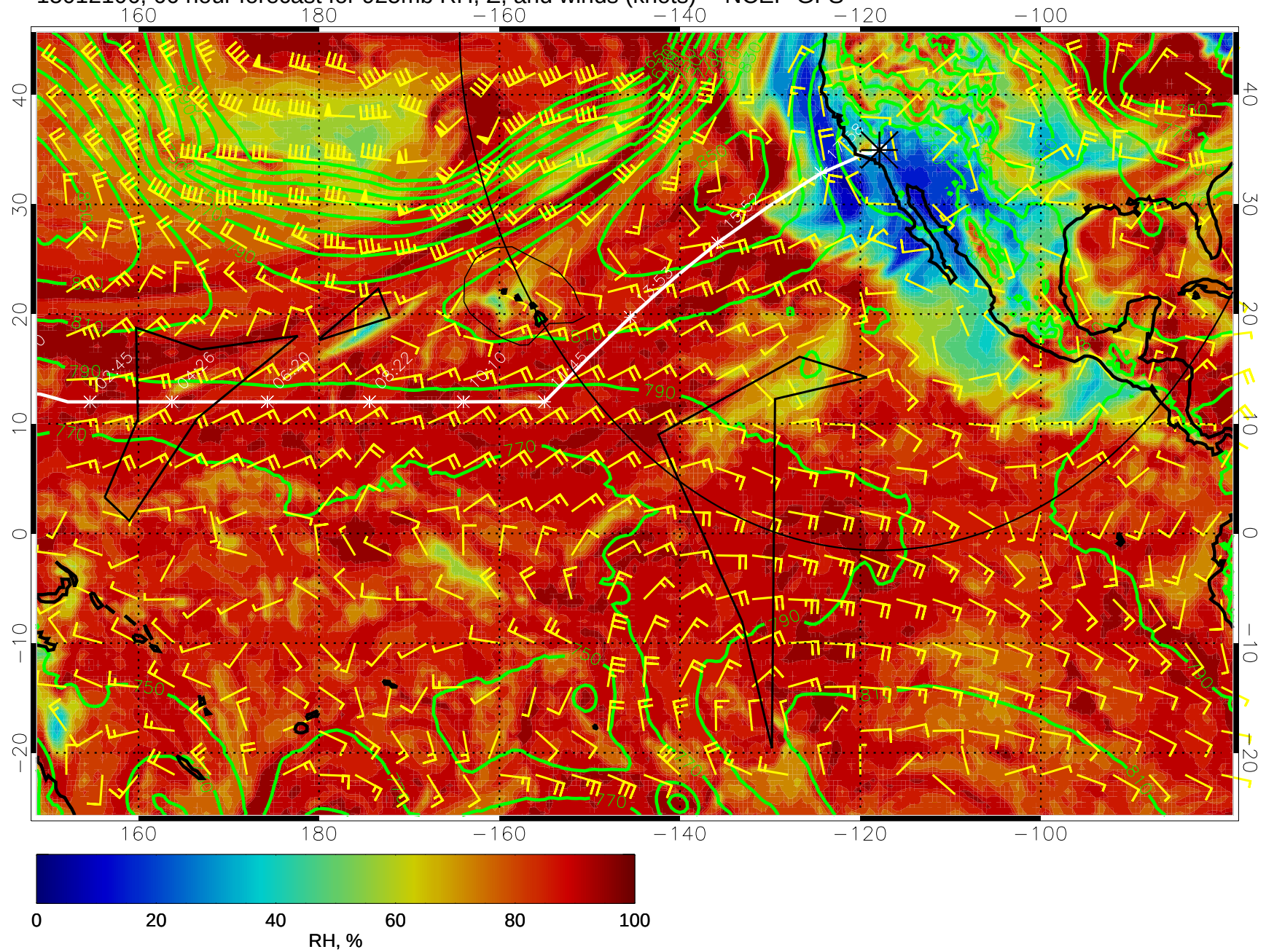
15012106, 66 hour forecast for 925mb RH, Z, and winds (knots) -- NCEP GFS
