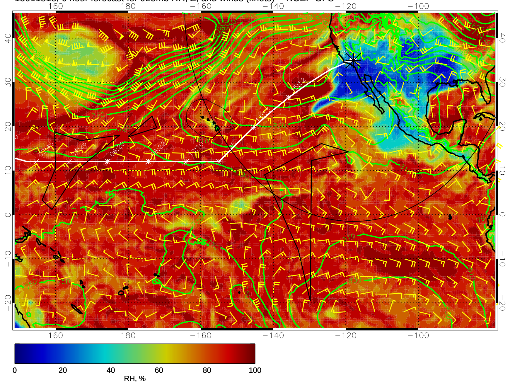
15011818, 6 hour forecast for 925mb RH, Z, and winds (knots) -- NCEP GFS
