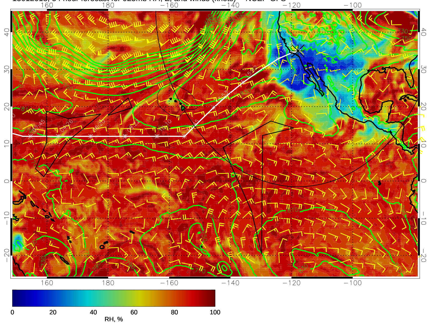
15012018, 54 hour forecast for 925mb RH, Z, and winds (knots) -- NCEP GFS
