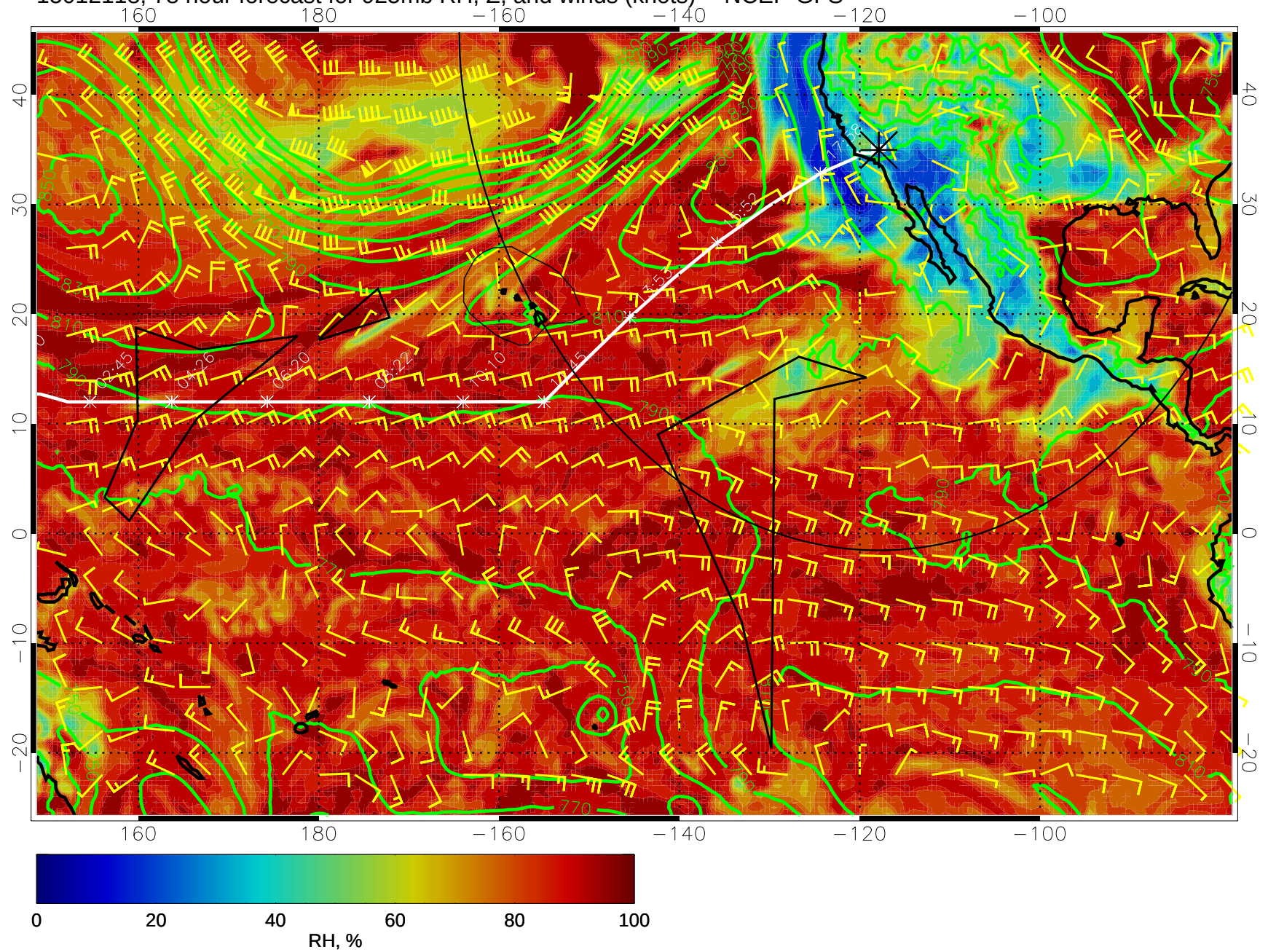
15012118, 78 hour forecast for 925mb RH, Z, and winds (knots) -- NCEP GFS
