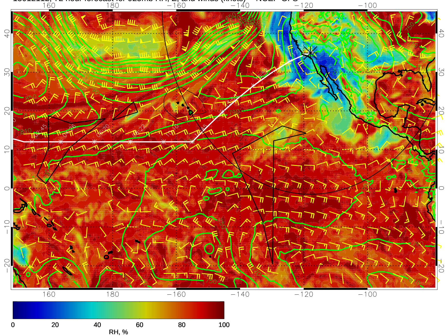
15012112, 72 hour forecast for 925mb RH, Z, and winds (knots) -- NCEP GFS
