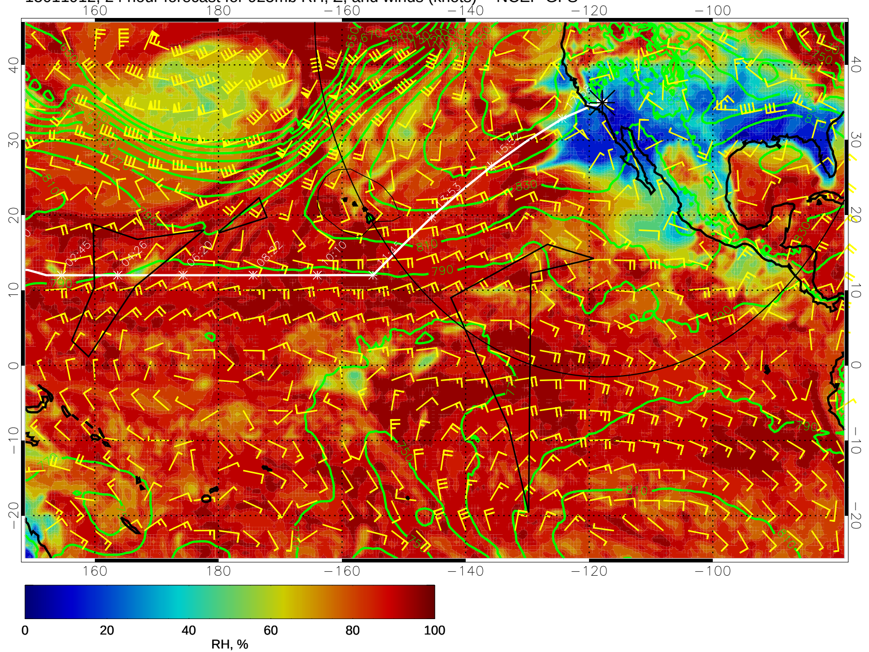
15011912, 24 hour forecast for 925mb RH, Z, and winds (knots) -- NCEP GFS
