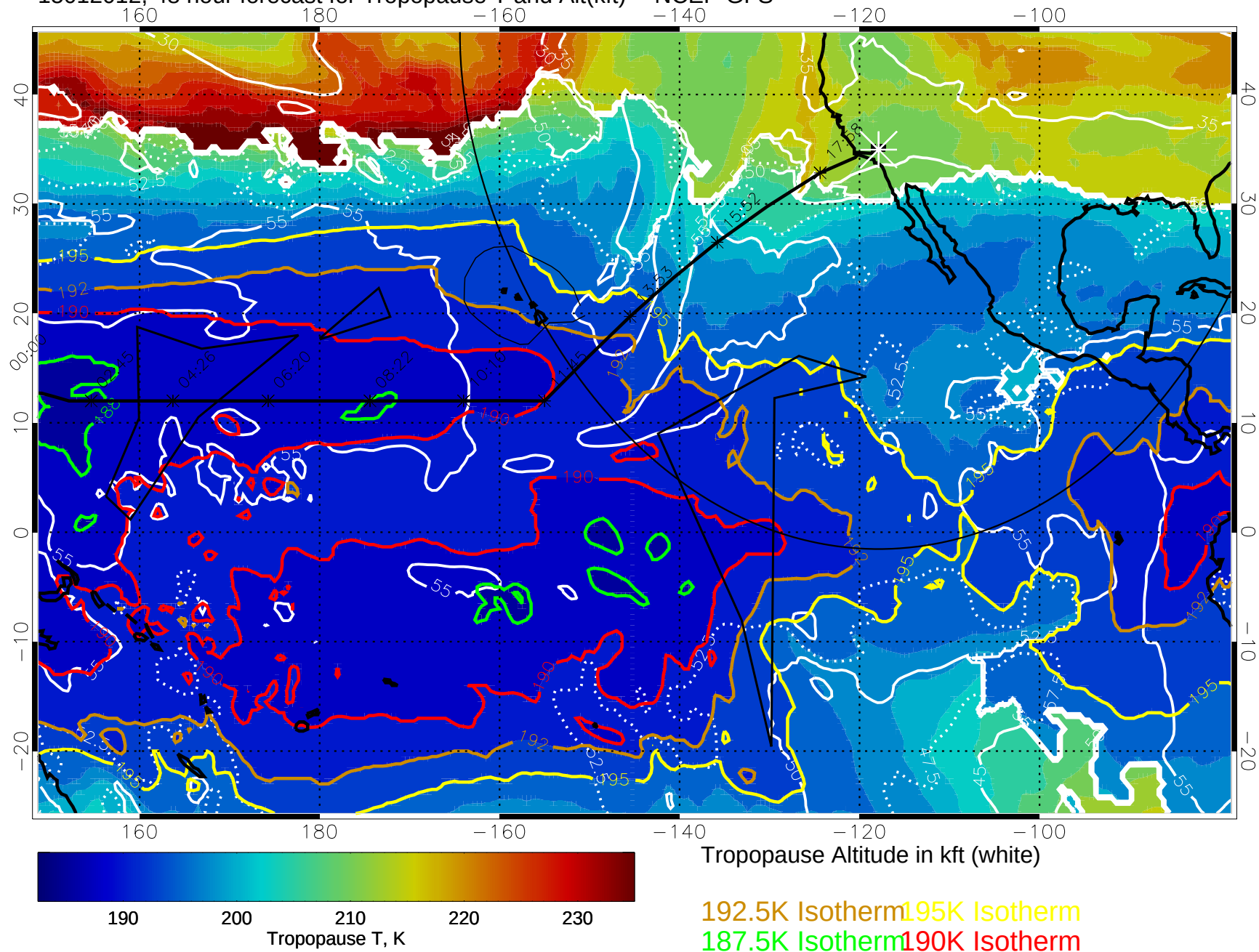
15012012, 48 hour forecast for Tropopause T and Alt(kft) -- NCEP GFS
