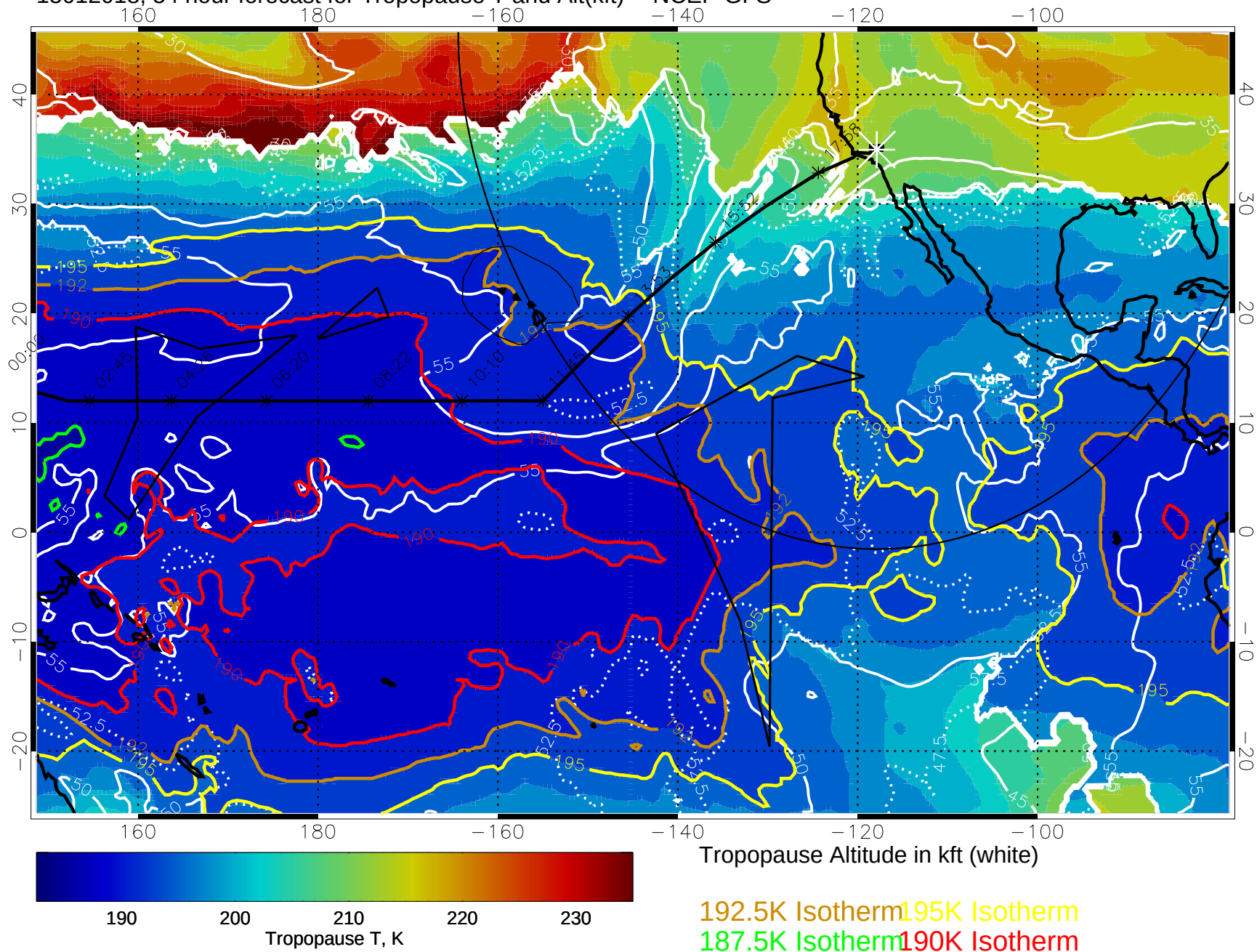
15012018, 54 hour forecast for Tropopause T and Alt(kft) -- NCEP GFS
