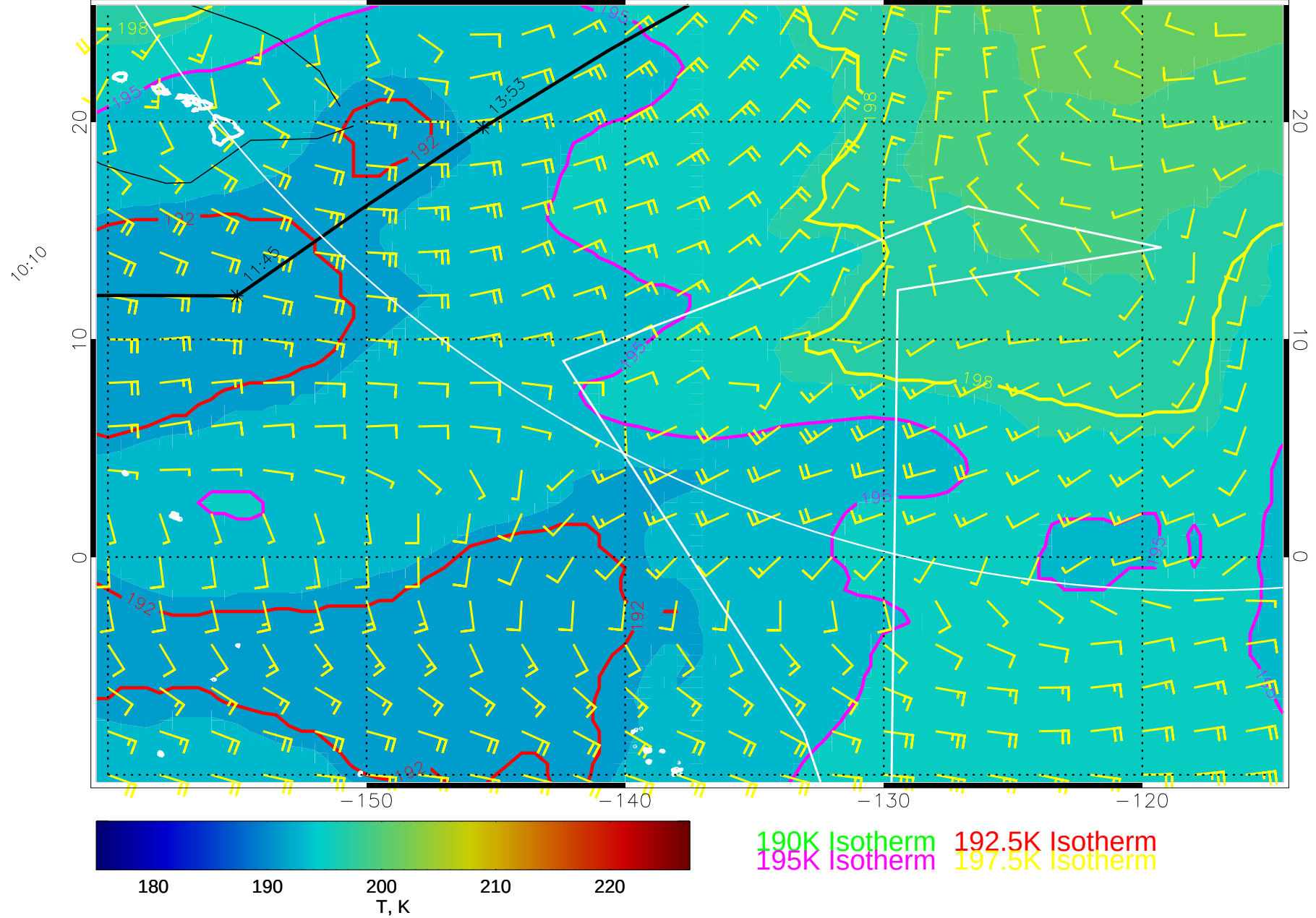
15012300, 108 hour forecast for 70mb T and winds (knots) -- NCEP GFS
