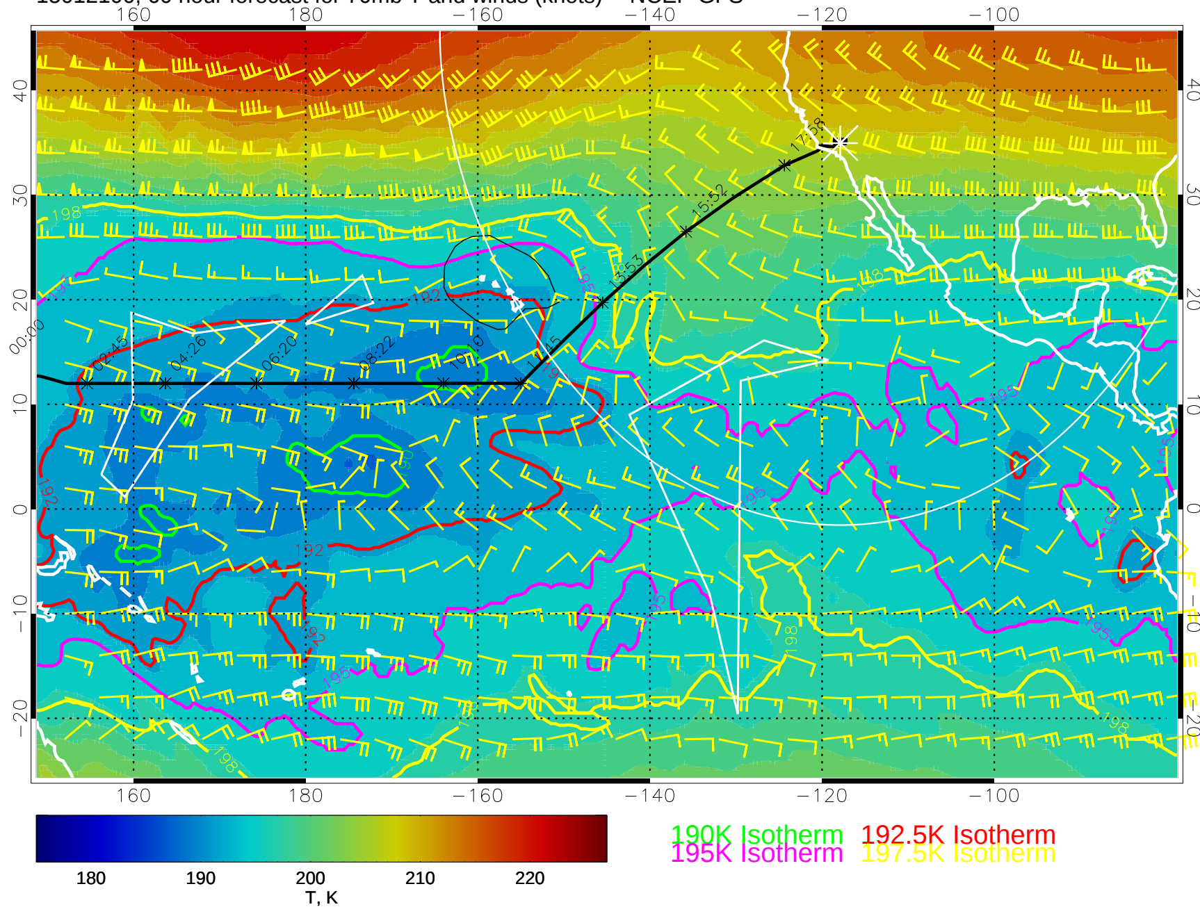
15012100, 60 hour forecast for 70mb T and winds (knots) -- NCEP GFS
