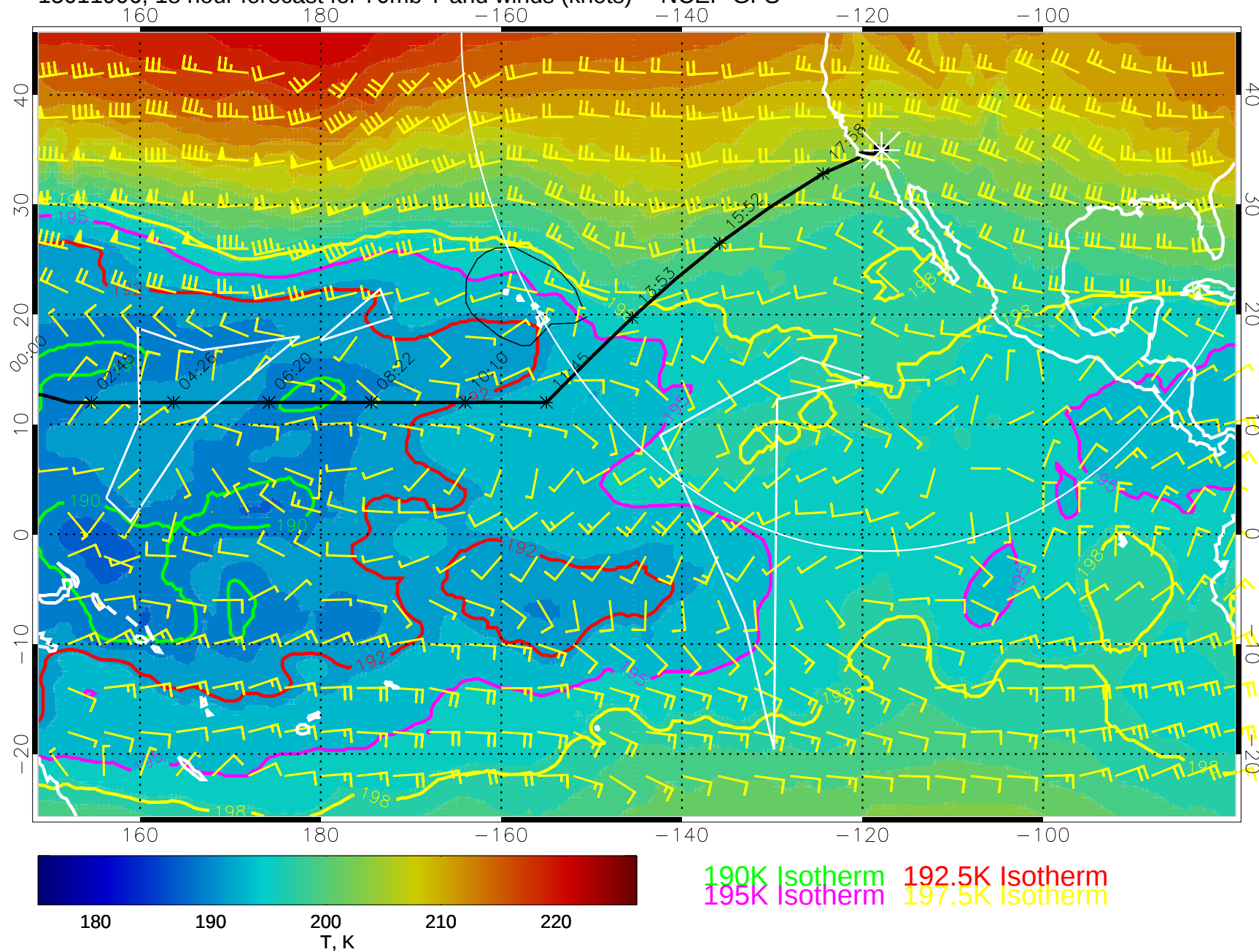
15011906, 18 hour forecast for 70mb T and winds (knots) -- NCEP GFS
