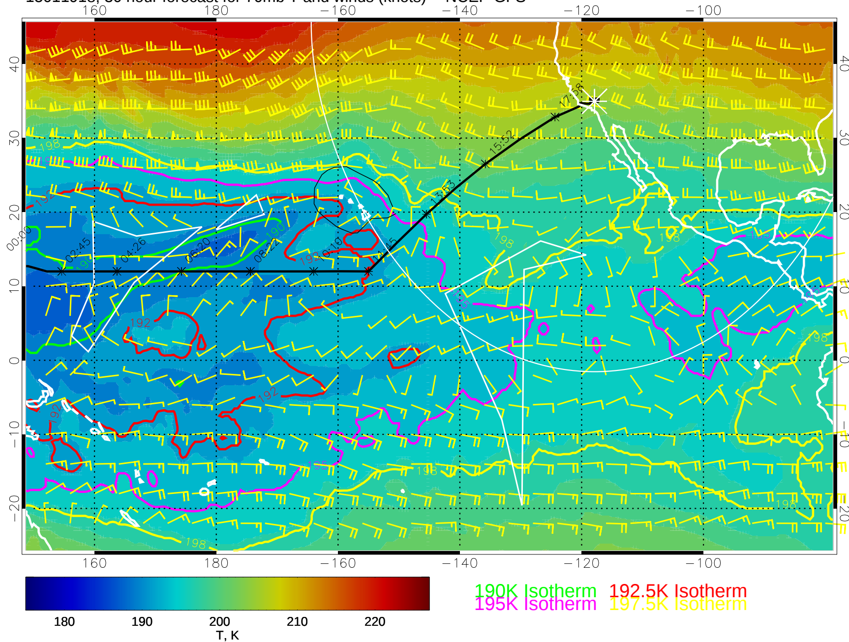
15011918, 30 hour forecast for 70mb T and winds (knots) -- NCEP GFS
