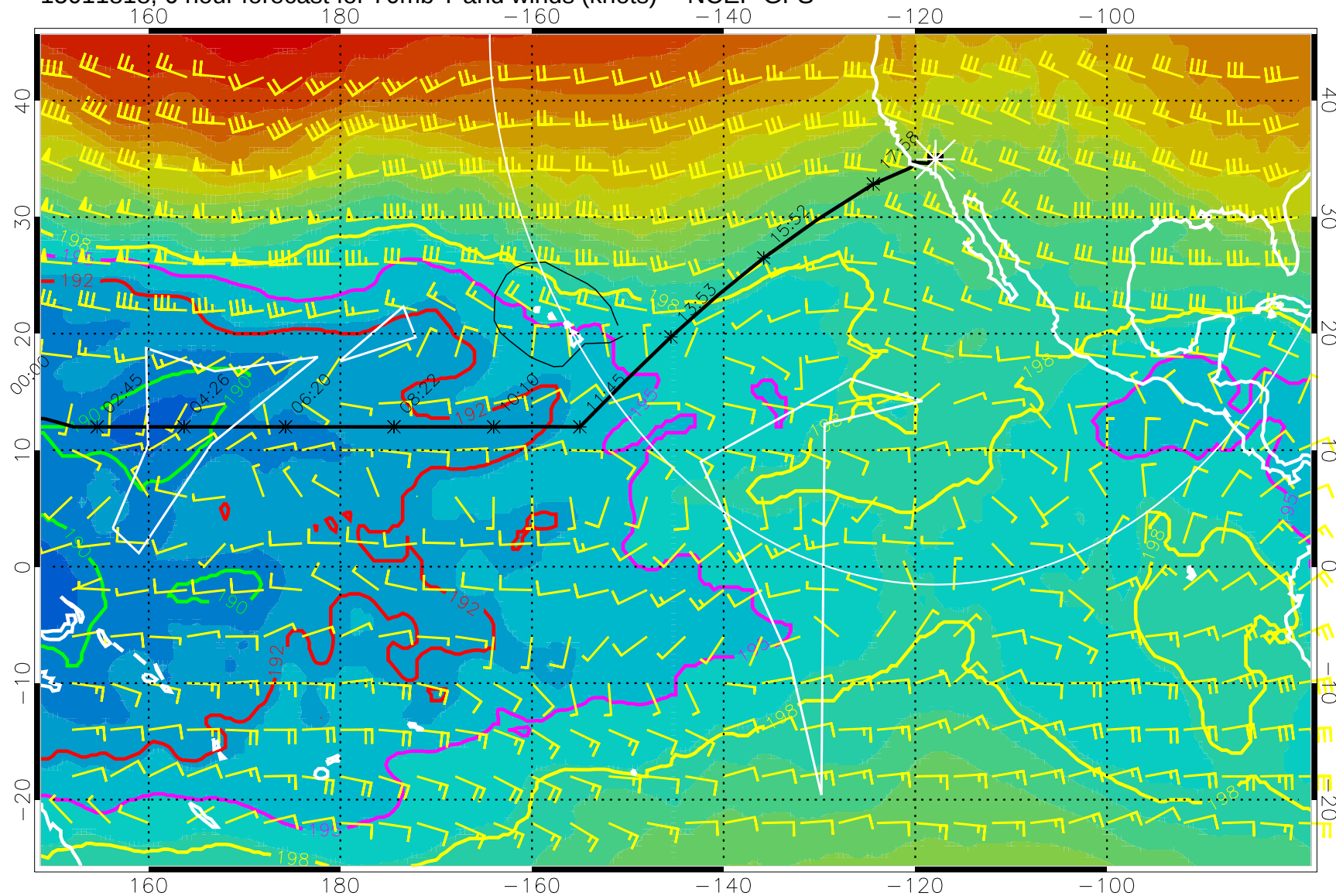
15011818, 6 hour forecast for 70mb T and winds (knots) -- NCEP GFS
