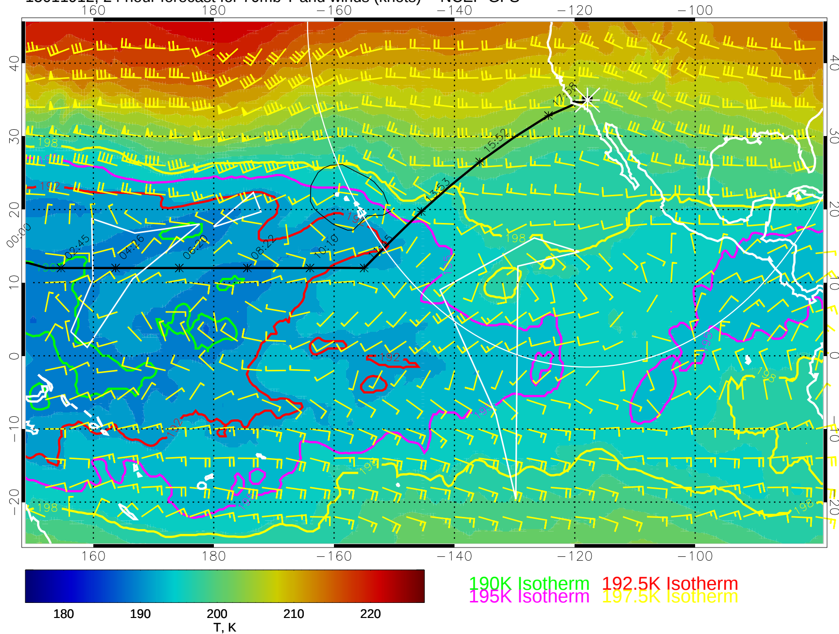
15011912, 24 hour forecast for 70mb T and winds (knots) -- NCEP GFS
