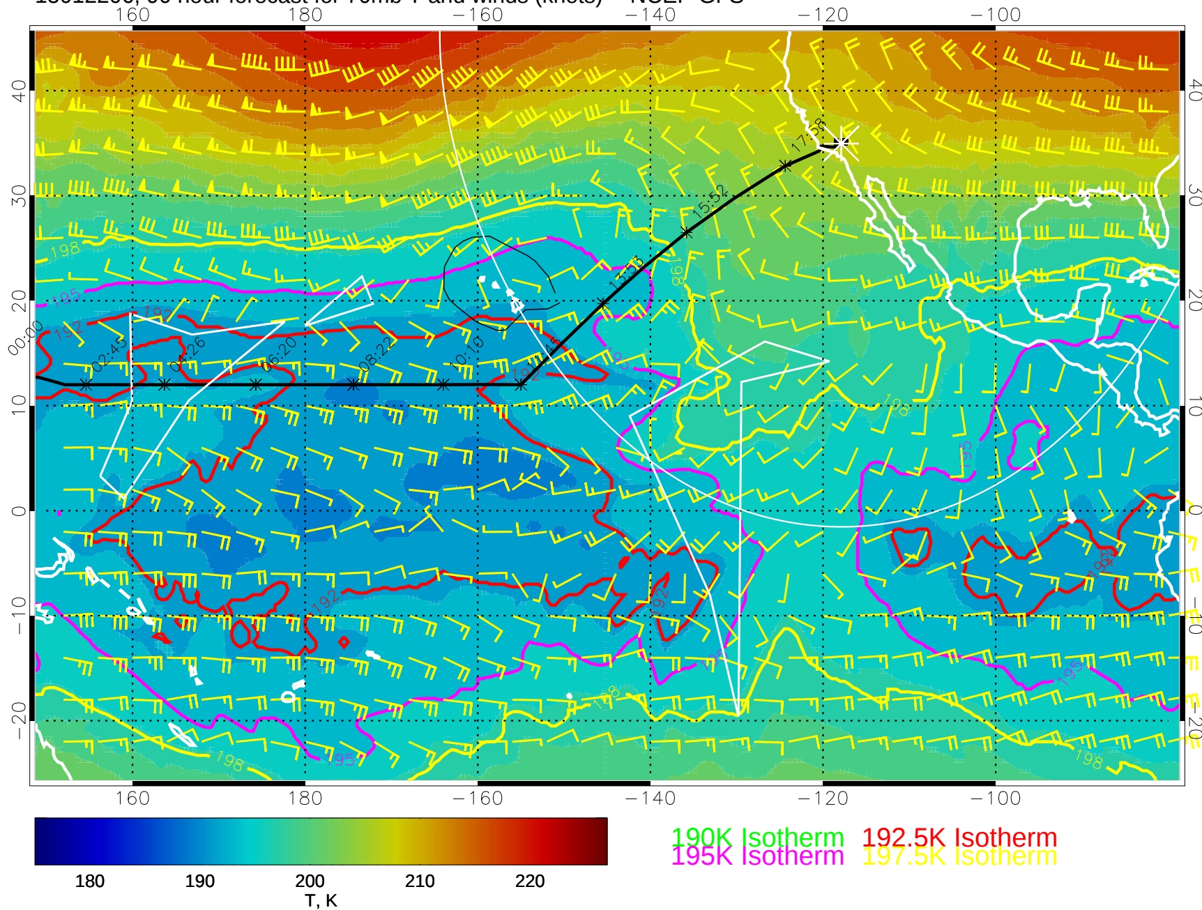
15012206, 90 hour forecast for 70mb T and winds (knots) -- NCEP GFS
