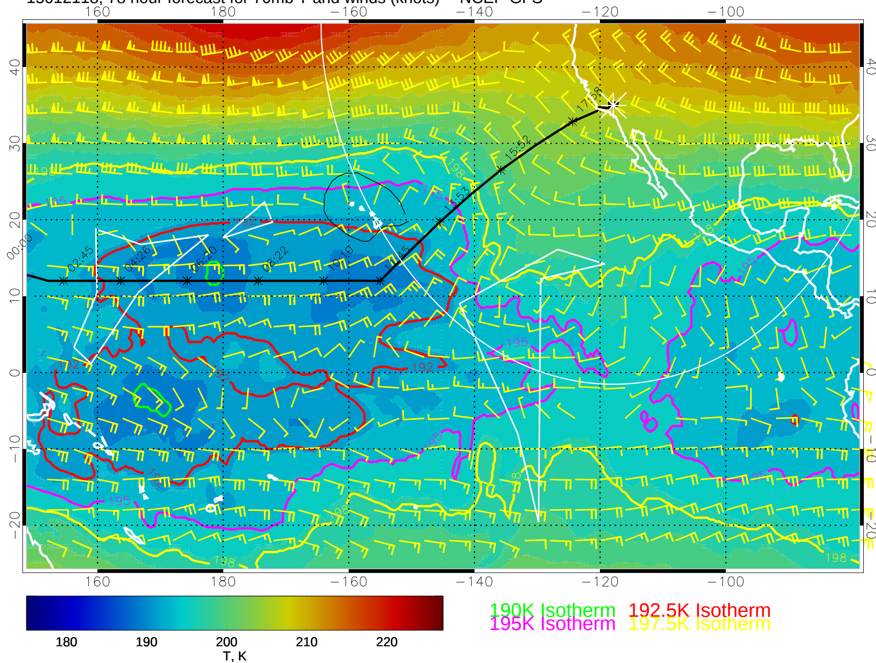
15012118, 78 hour forecast for 70mb T and winds (knots) -- NCEP GFS
