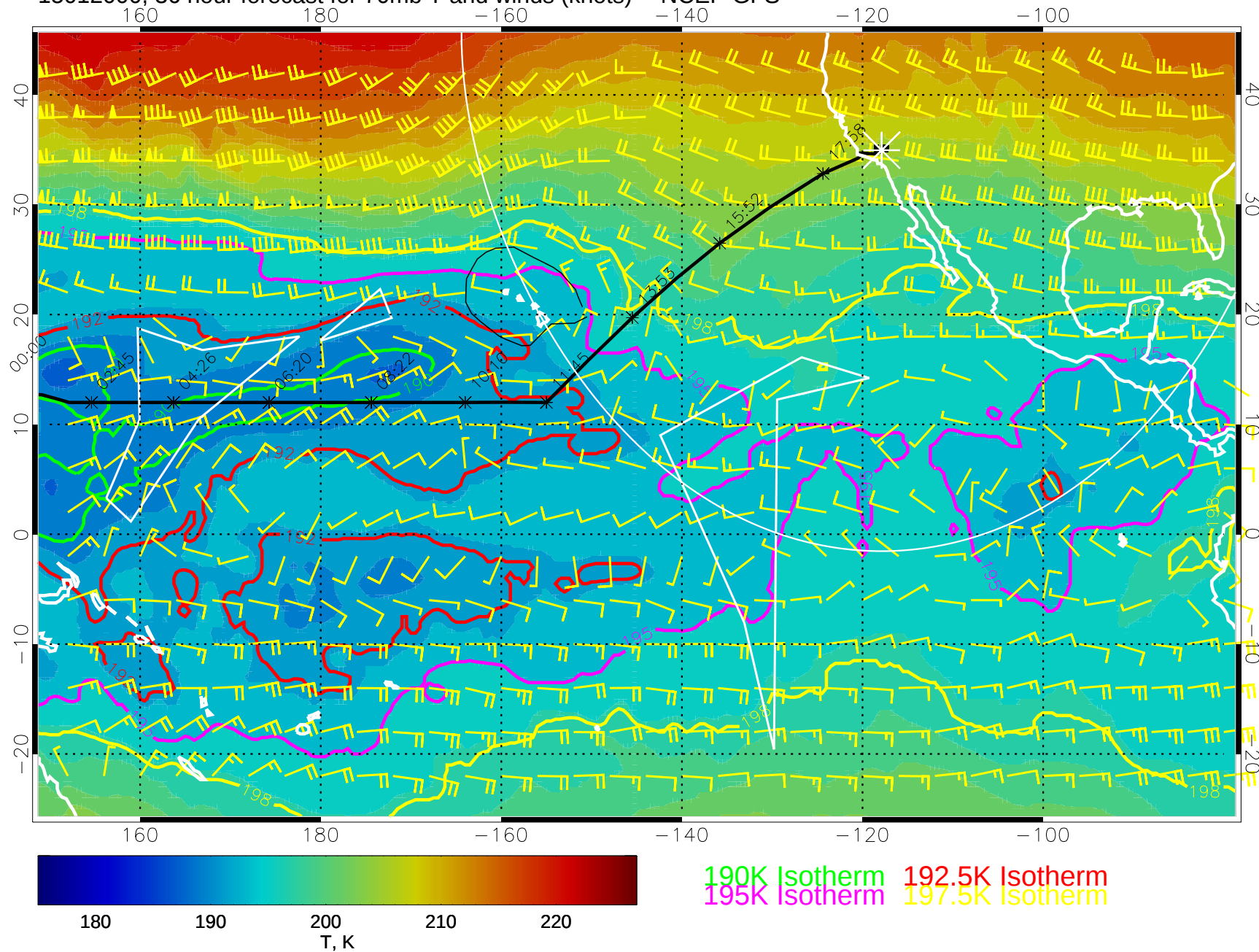
15012000, 36 hour forecast for 70mb T and winds (knots) -- NCEP GFS
