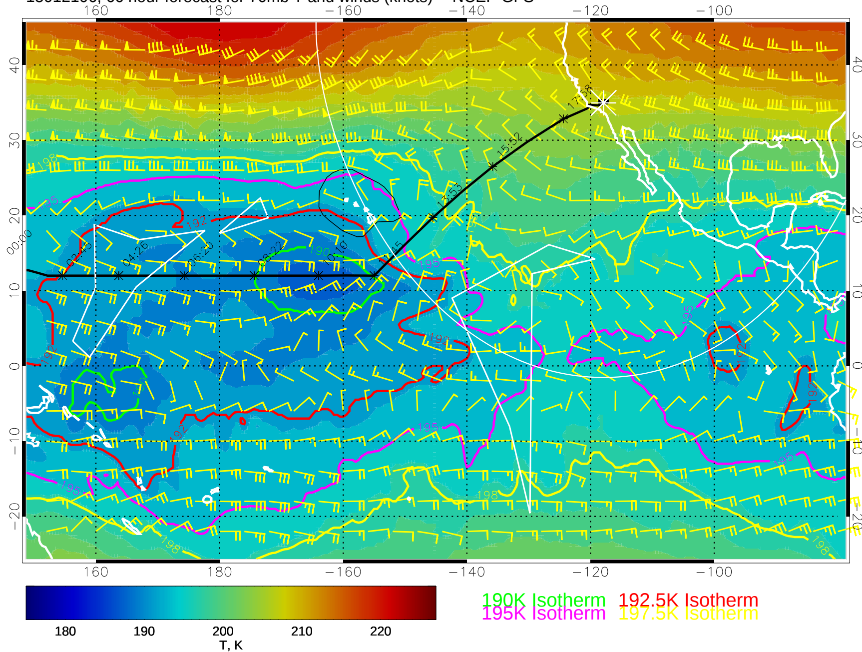
15012106, 66 hour forecast for 70mb T and winds (knots) -- NCEP GFS
