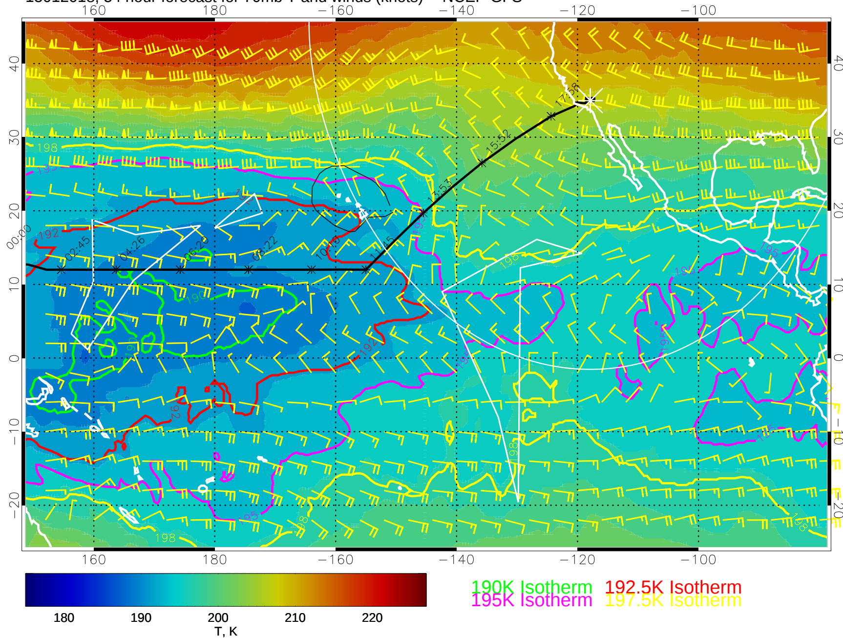
15012018, 54 hour forecast for 70mb T and winds (knots) -- NCEP GFS
