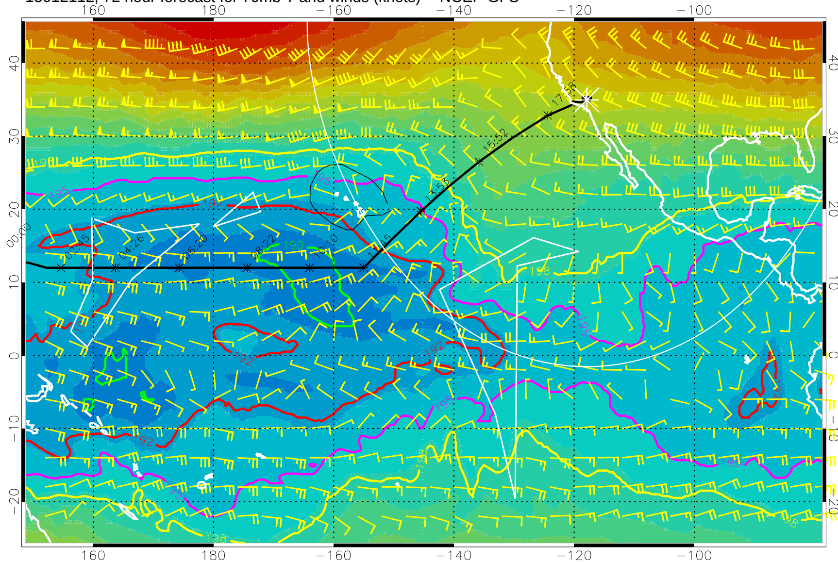
15012112, 72 hour forecast for 70mb T and winds (knots) -- NCEP GFS
