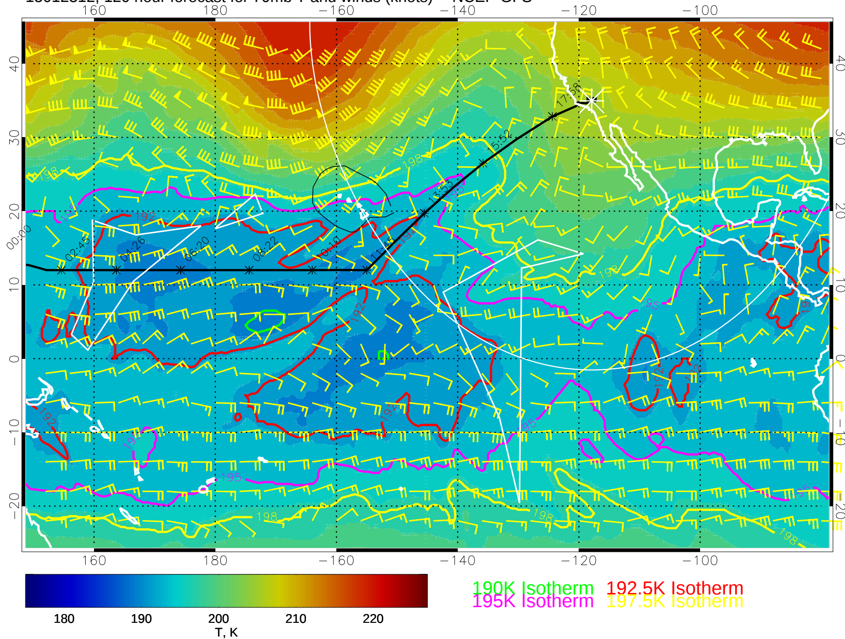
15012312, 120 hour forecast for 70mb T and winds (knots) -- NCEP GFS
