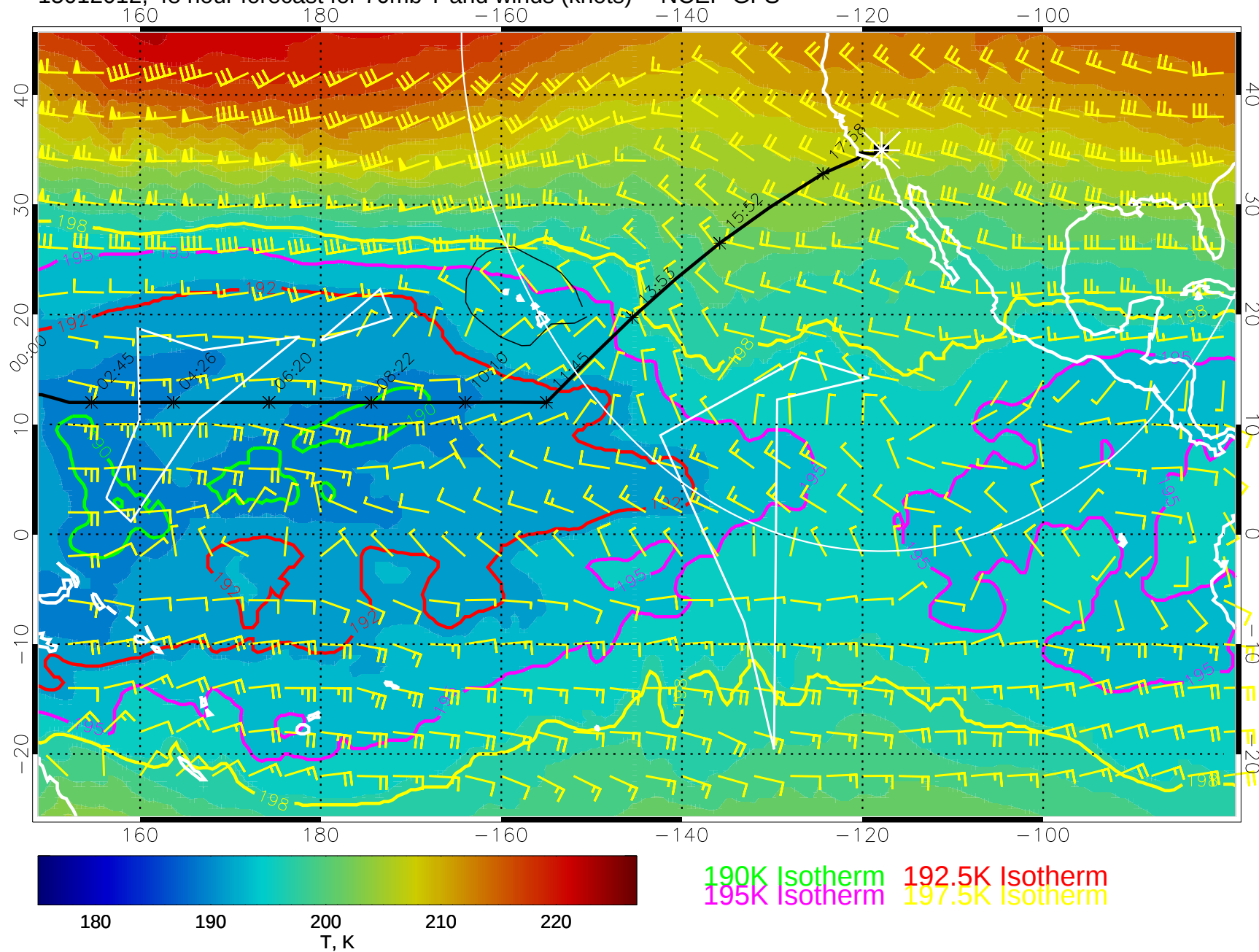
15012012, 48 hour forecast for 70mb T and winds (knots) -- NCEP GFS
