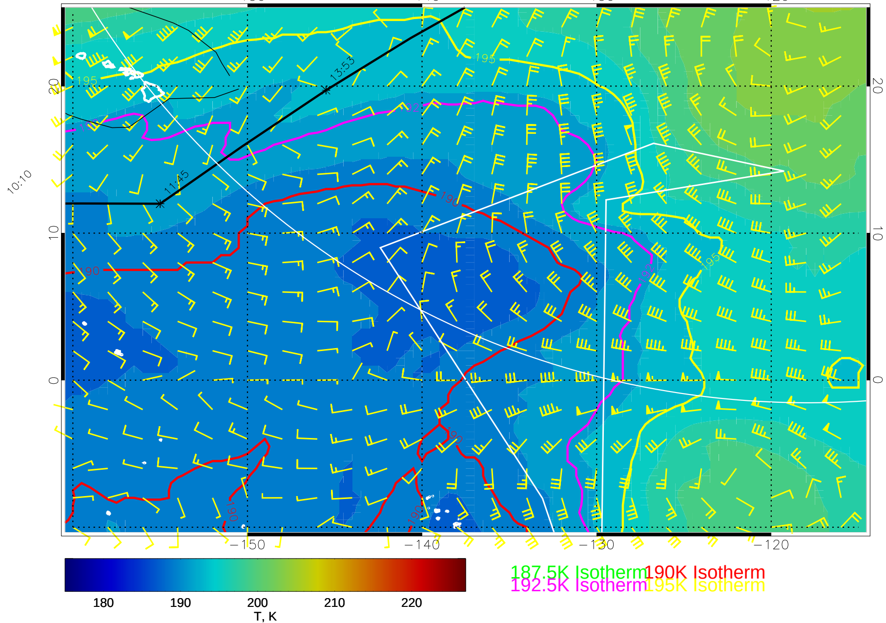
15012312, 120 hour forecast for 100mb T and winds (knots) -- NCEP GFS
