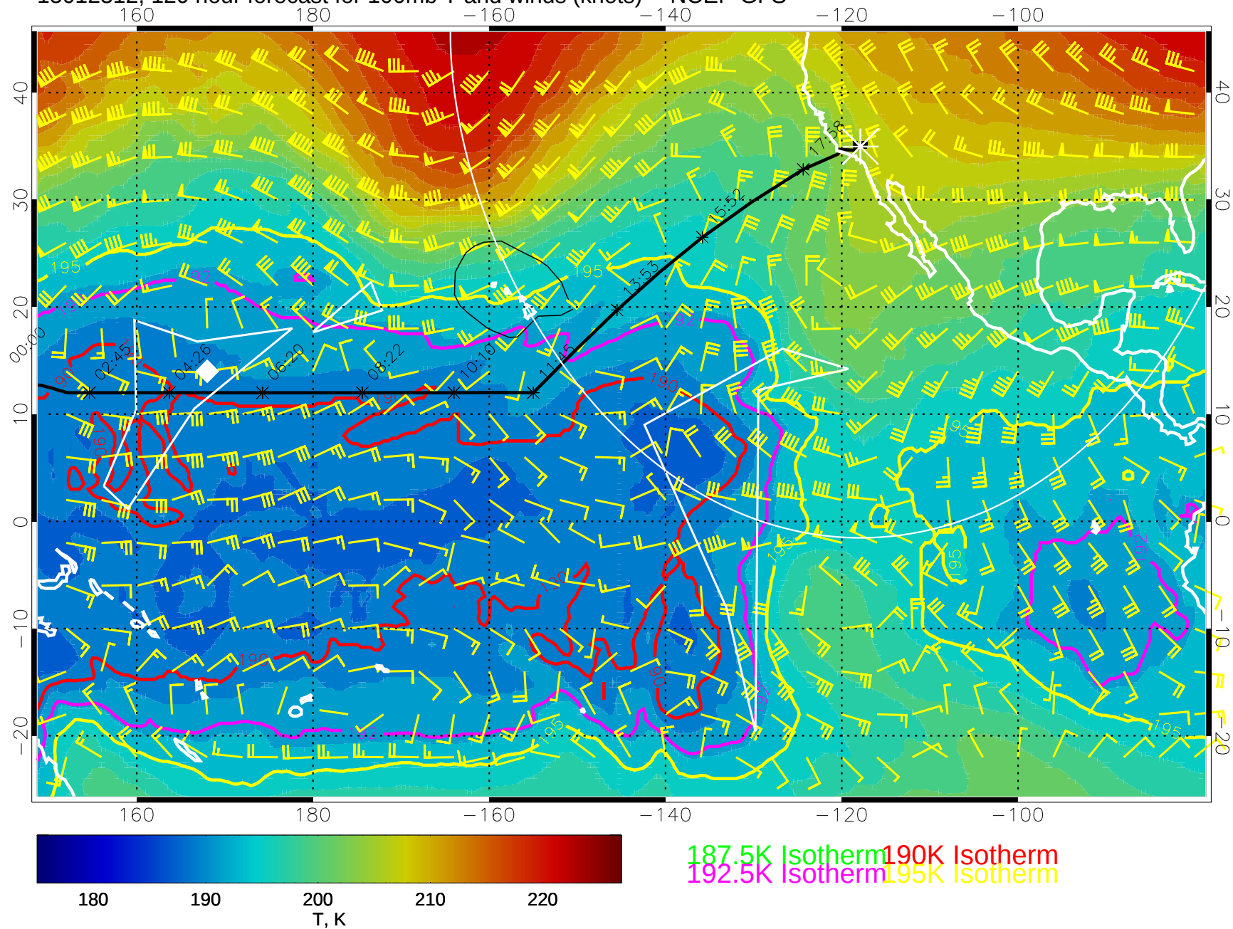
15012312, 120 hour forecast for 100mb T and winds (knots) -- NCEP GFS
