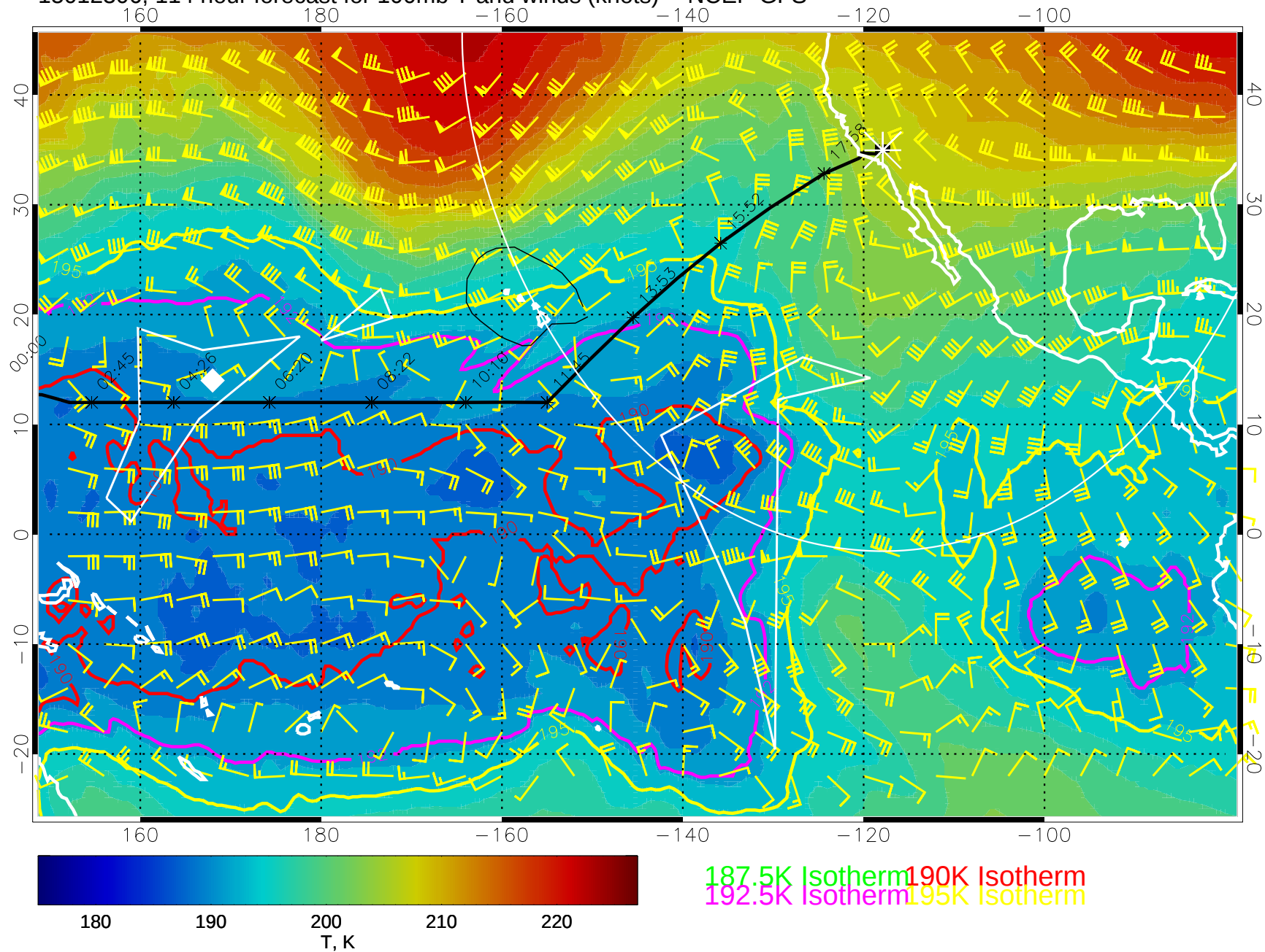
15012306, 114 hour forecast for 100mb T and winds (knots) -- NCEP GFS
