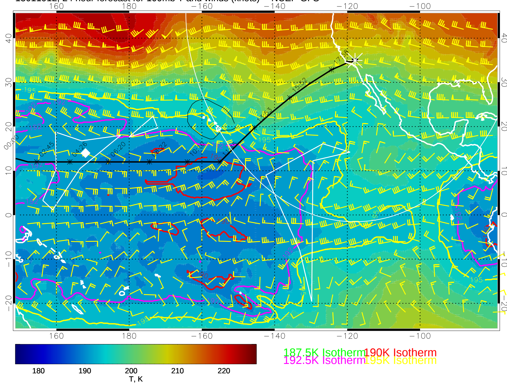
15011912, 24 hour forecast for 100mb T and winds (knots) -- NCEP GFS
