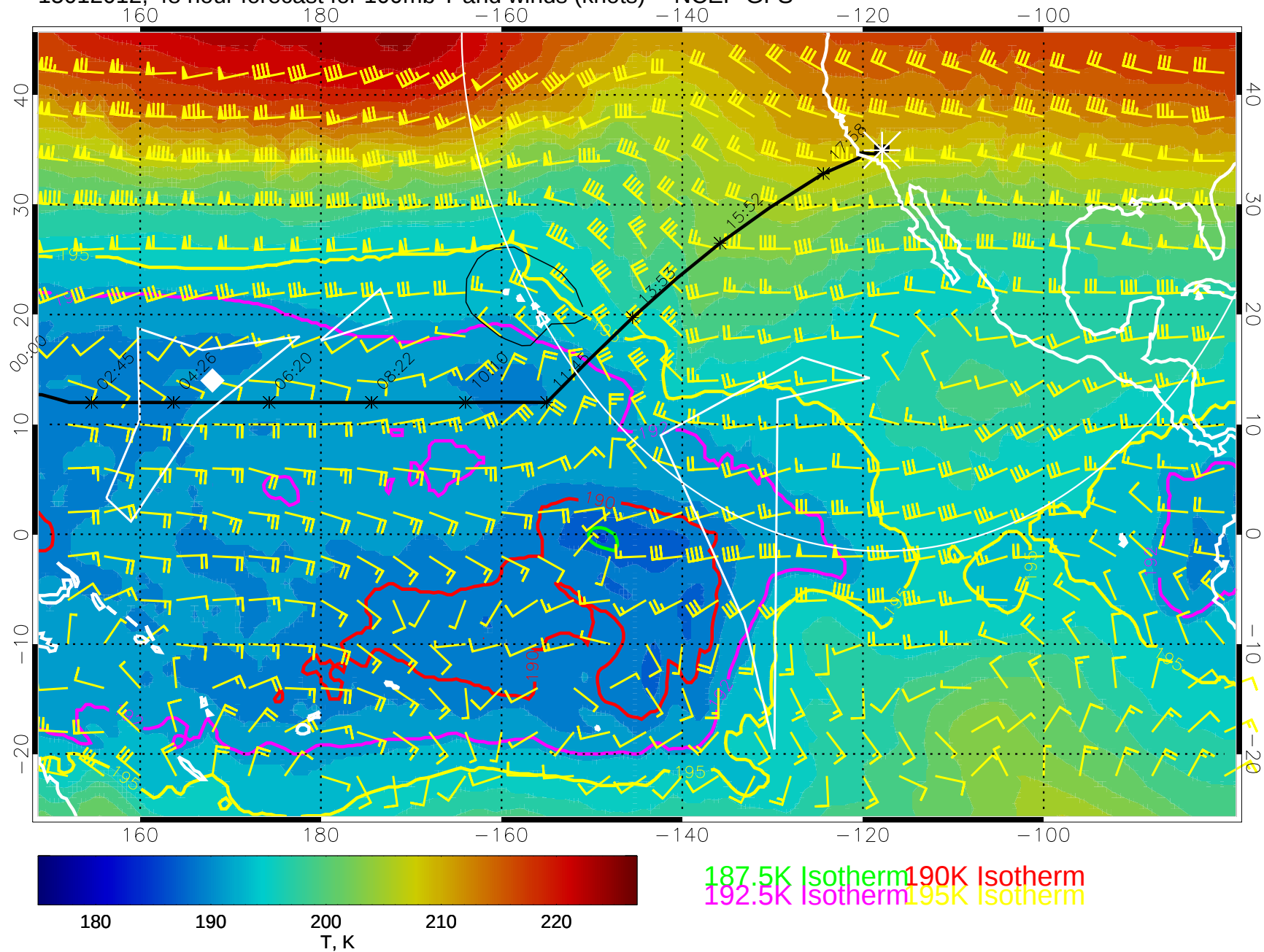
15012012, 48 hour forecast for 100mb T and winds (knots) -- NCEP GFS
