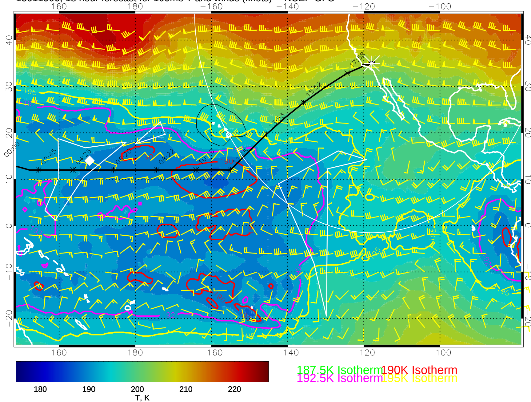
15011906, 18 hour forecast for 100mb T and winds (knots) -- NCEP GFS
