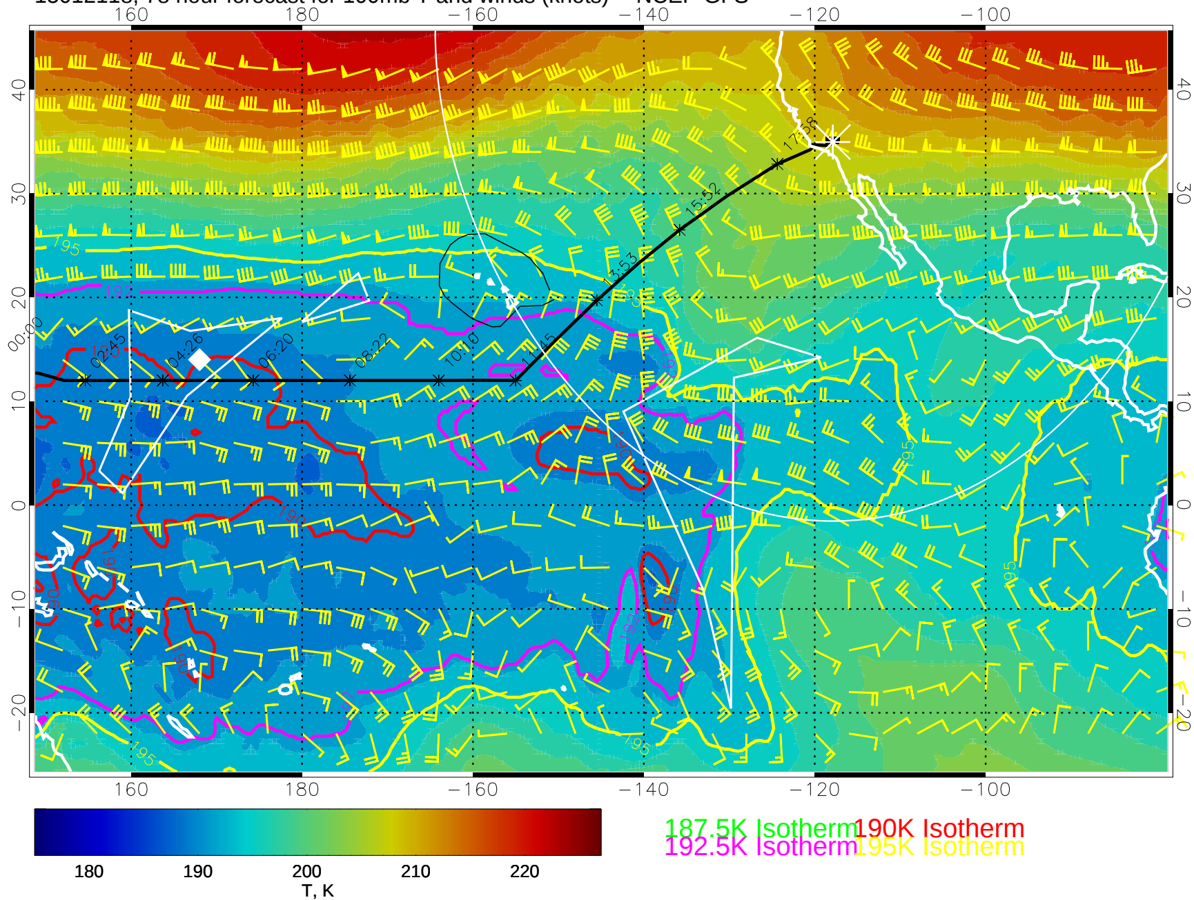
15012118, 78 hour forecast for 100mb T and winds (knots) -- NCEP GFS
