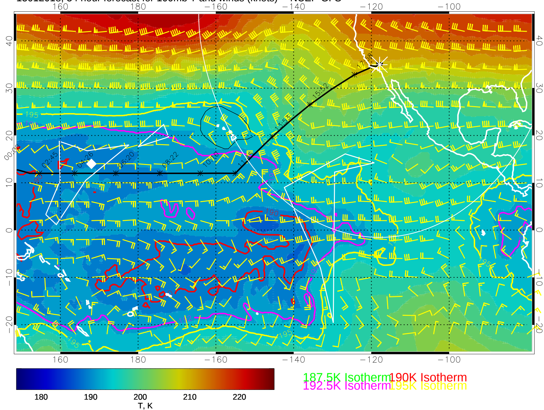
15012018, 54 hour forecast for 100mb T and winds (knots) -- NCEP GFS
