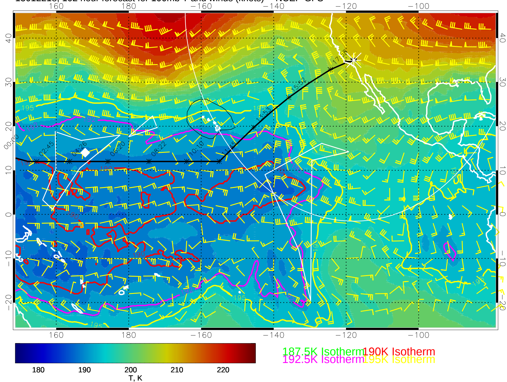
15012218, 102 hour forecast for 100mb T and winds (knots) -- NCEP GFS
