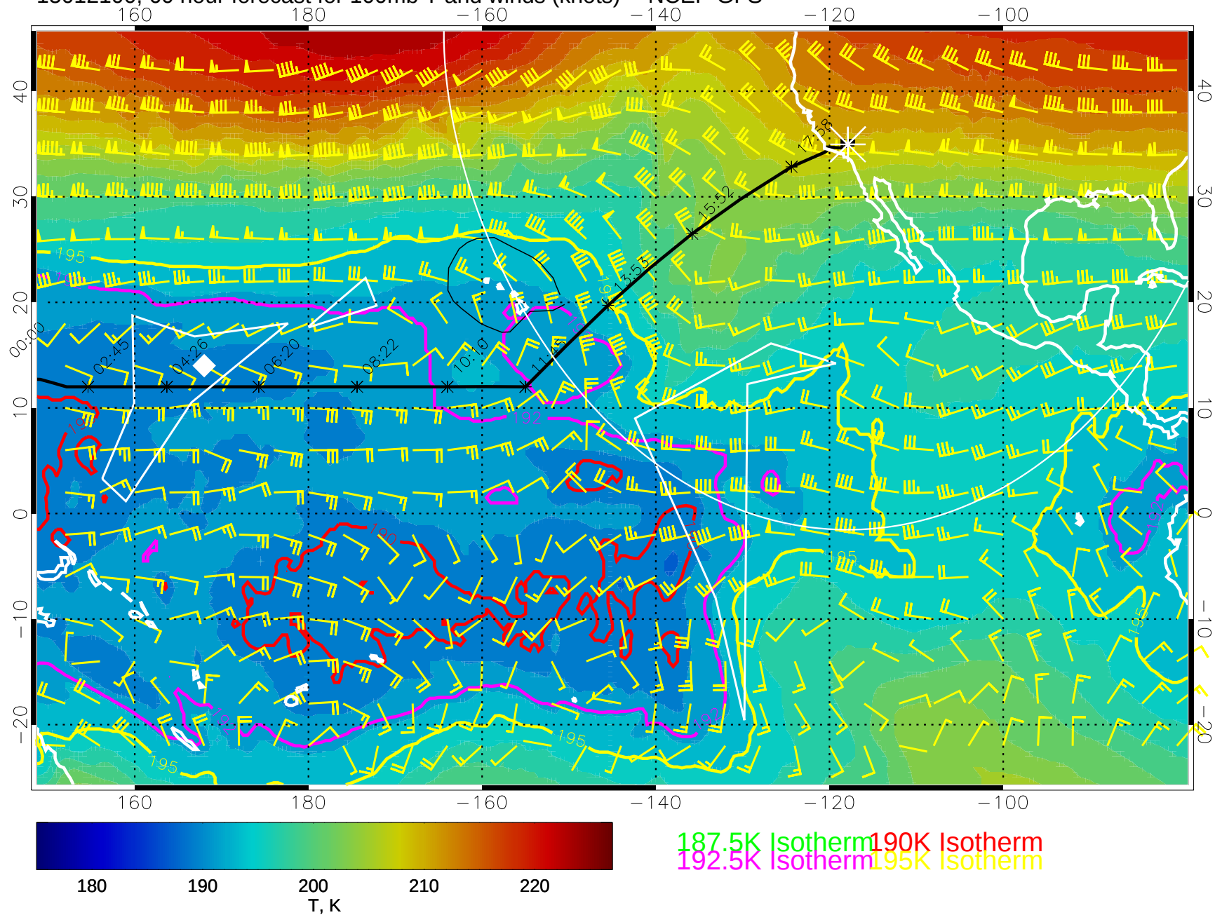
15012100, 60 hour forecast for 100mb T and winds (knots) -- NCEP GFS
