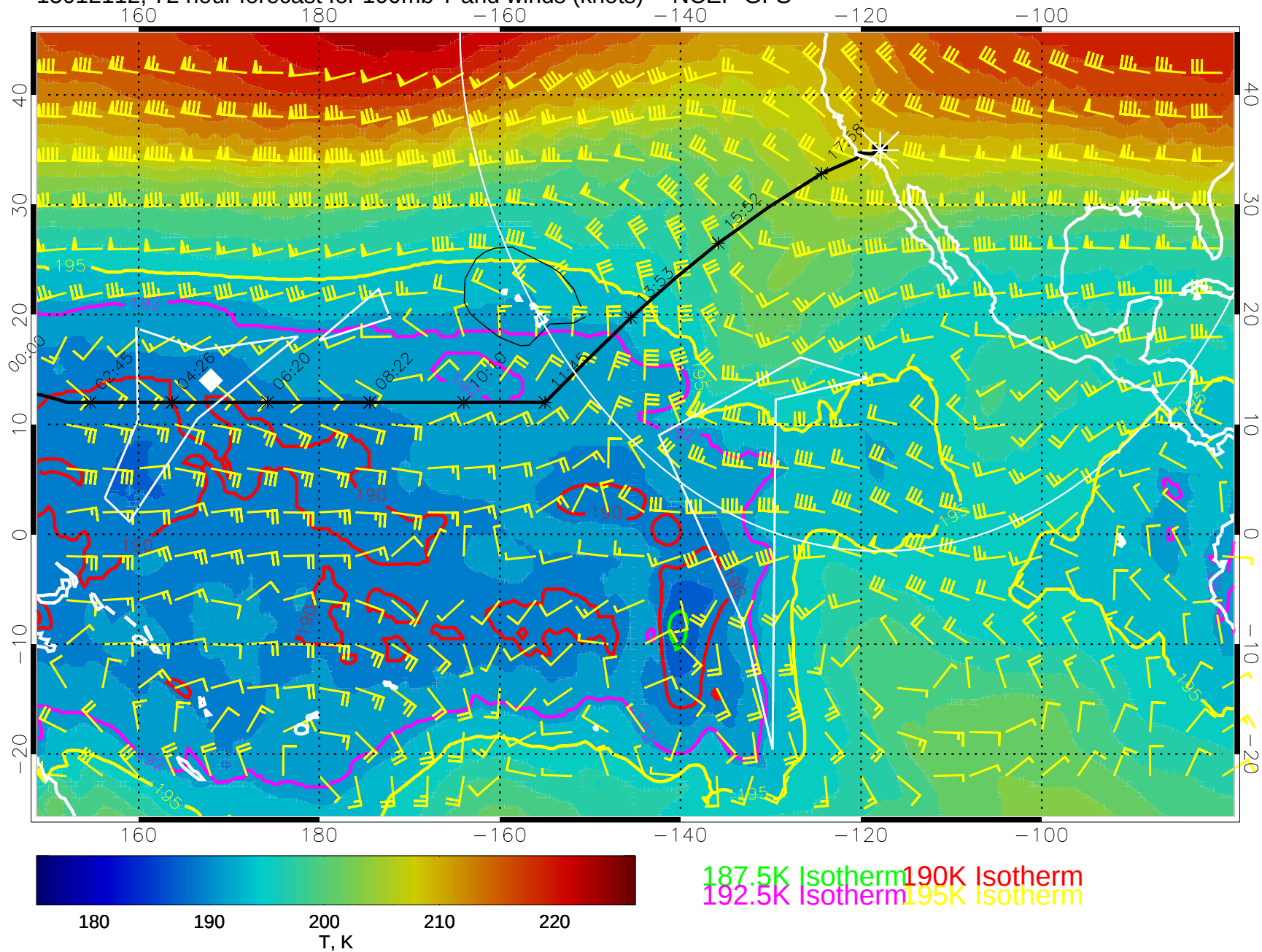
15012112, 72 hour forecast for 100mb T and winds (knots) -- NCEP GFS
