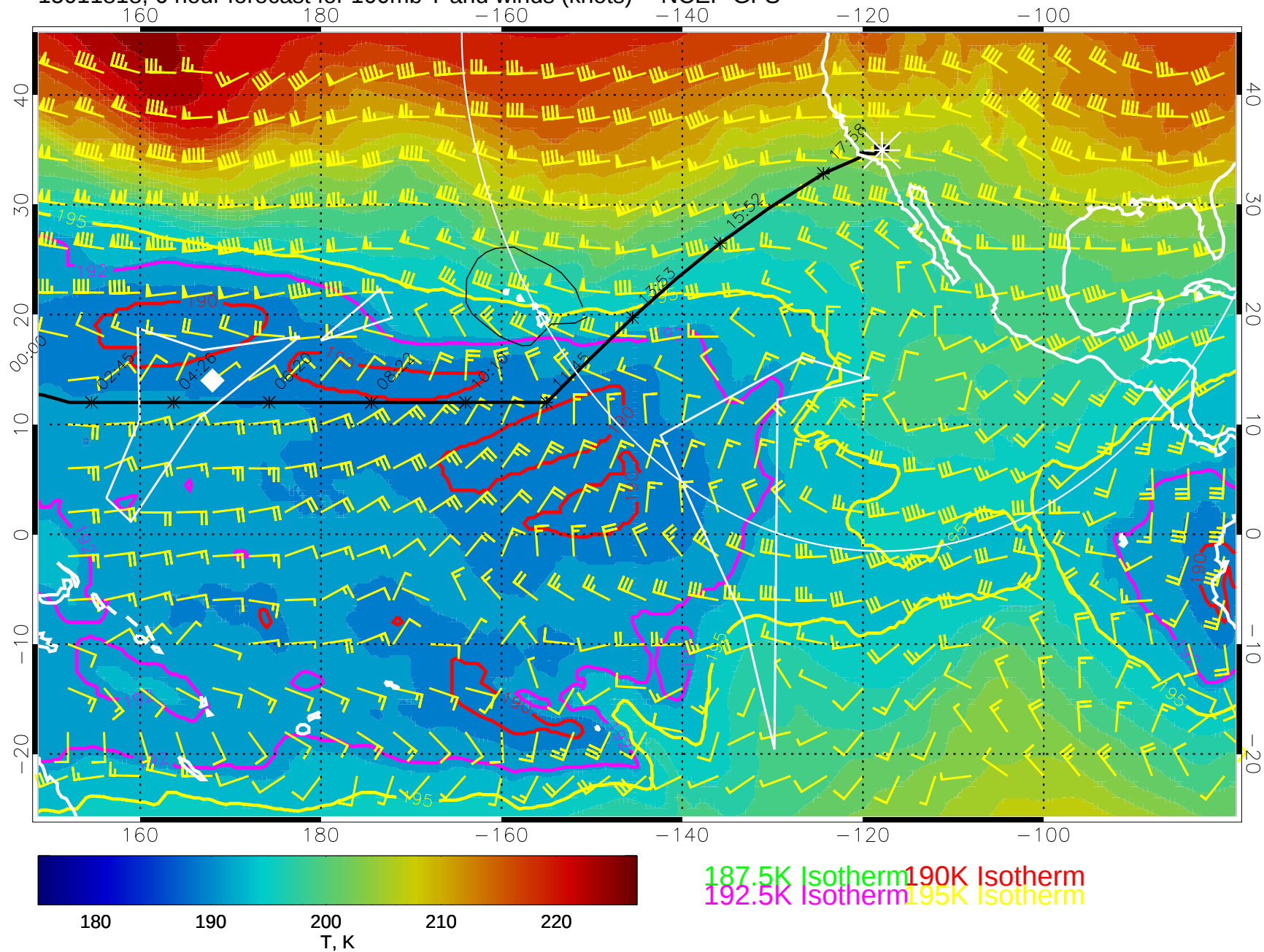
15011818, 6 hour forecast for 100mb T and winds (knots) -- NCEP GFS
