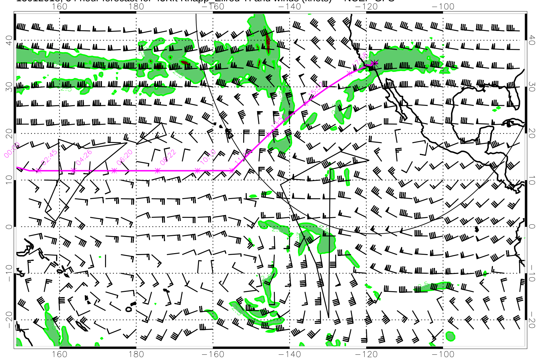
15012018, 54 hour forecast for 45Kft Knapp_Ellrod TI and winds (knots) -- NCEP GFS
