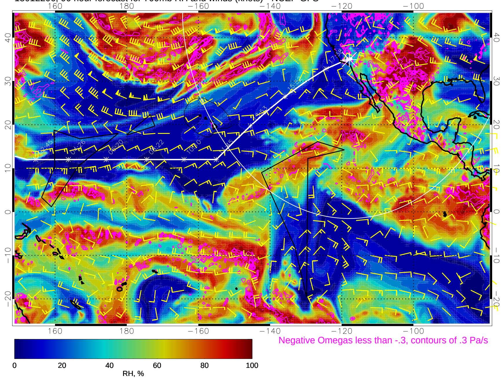
15012206, 90 hour forecast for 700mb RH and winds (knots) - NCEP GFS
