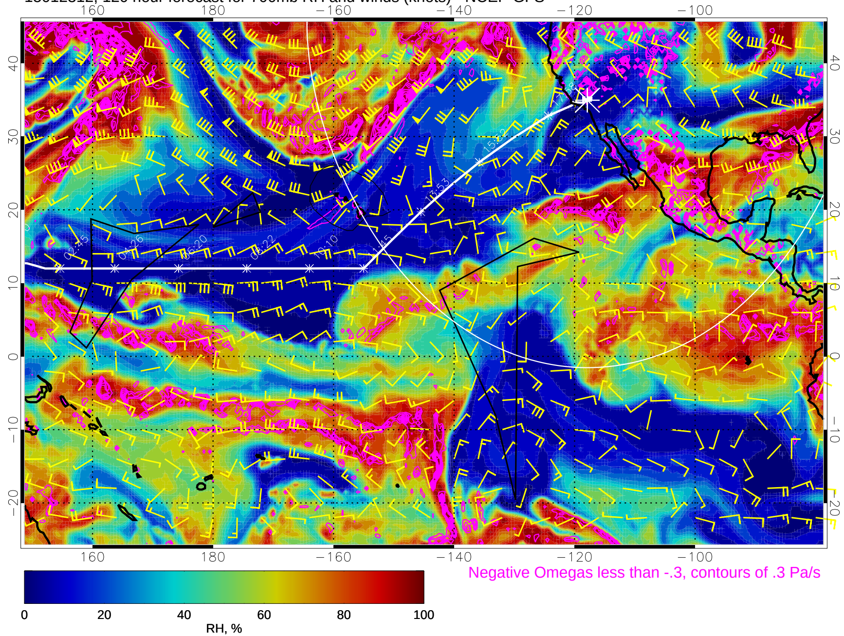
15012312, 120 hour forecast for 700mb RH and winds (knots) - NCEP GFS
