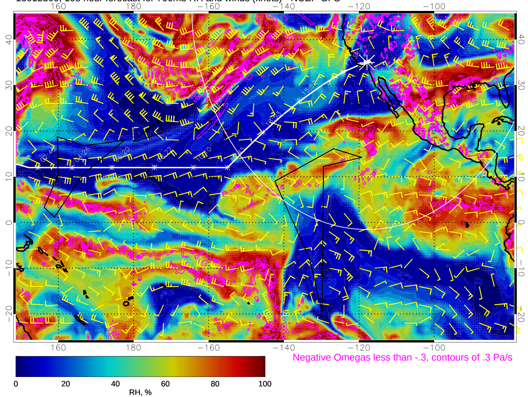
15012300, 108 hour forecast for 700mb RH and winds (knots) - NCEP GFS
