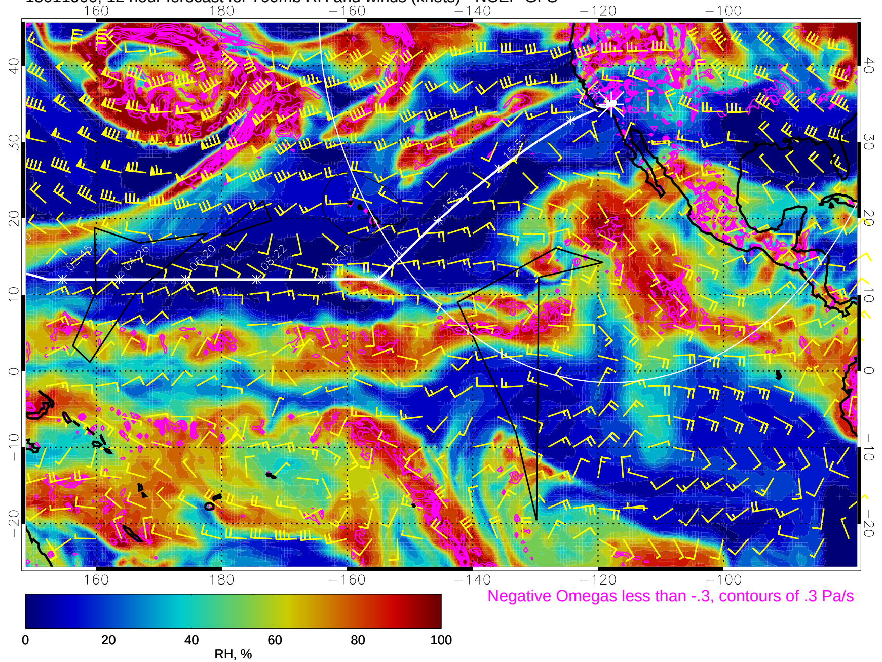
15011900, 12 hour forecast for 700mb RH and winds (knots) - NCEP GFS
