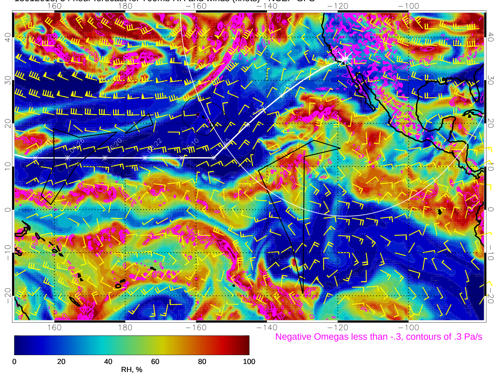
15012018, 54 hour forecast for 700mb RH and winds (knots) - NCEP GFS
