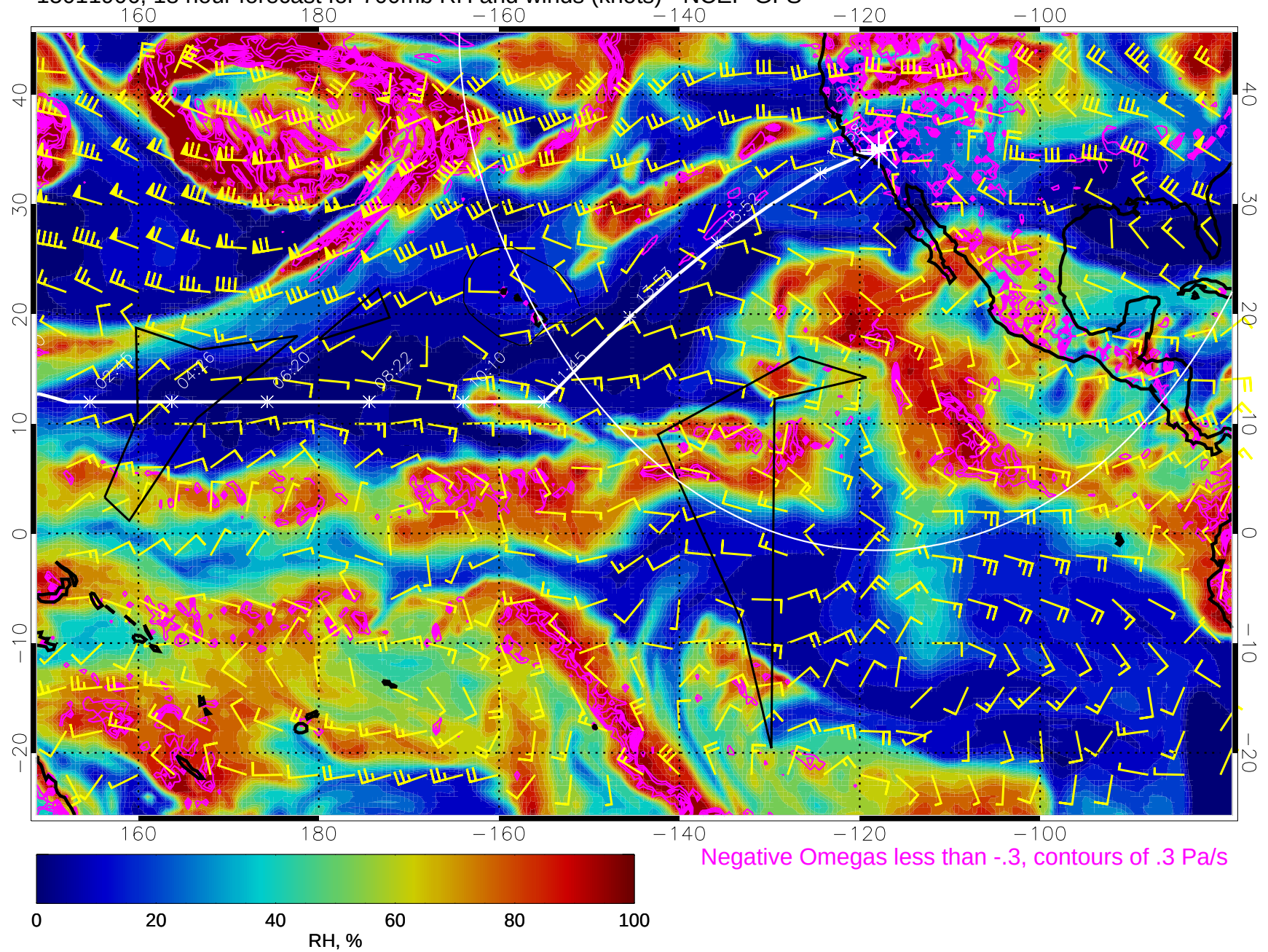
15011906, 18 hour forecast for 700mb RH and winds (knots) - NCEP GFS
