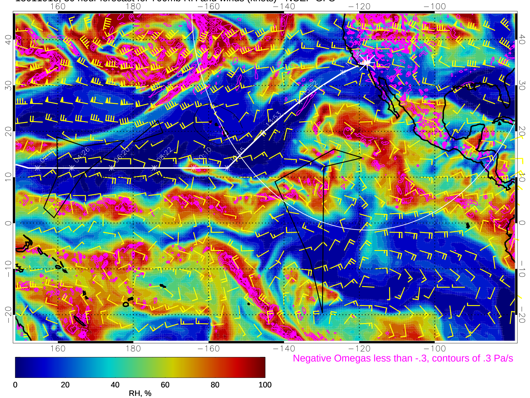
15011918, 30 hour forecast for 700mb RH and winds (knots) - NCEP GFS
