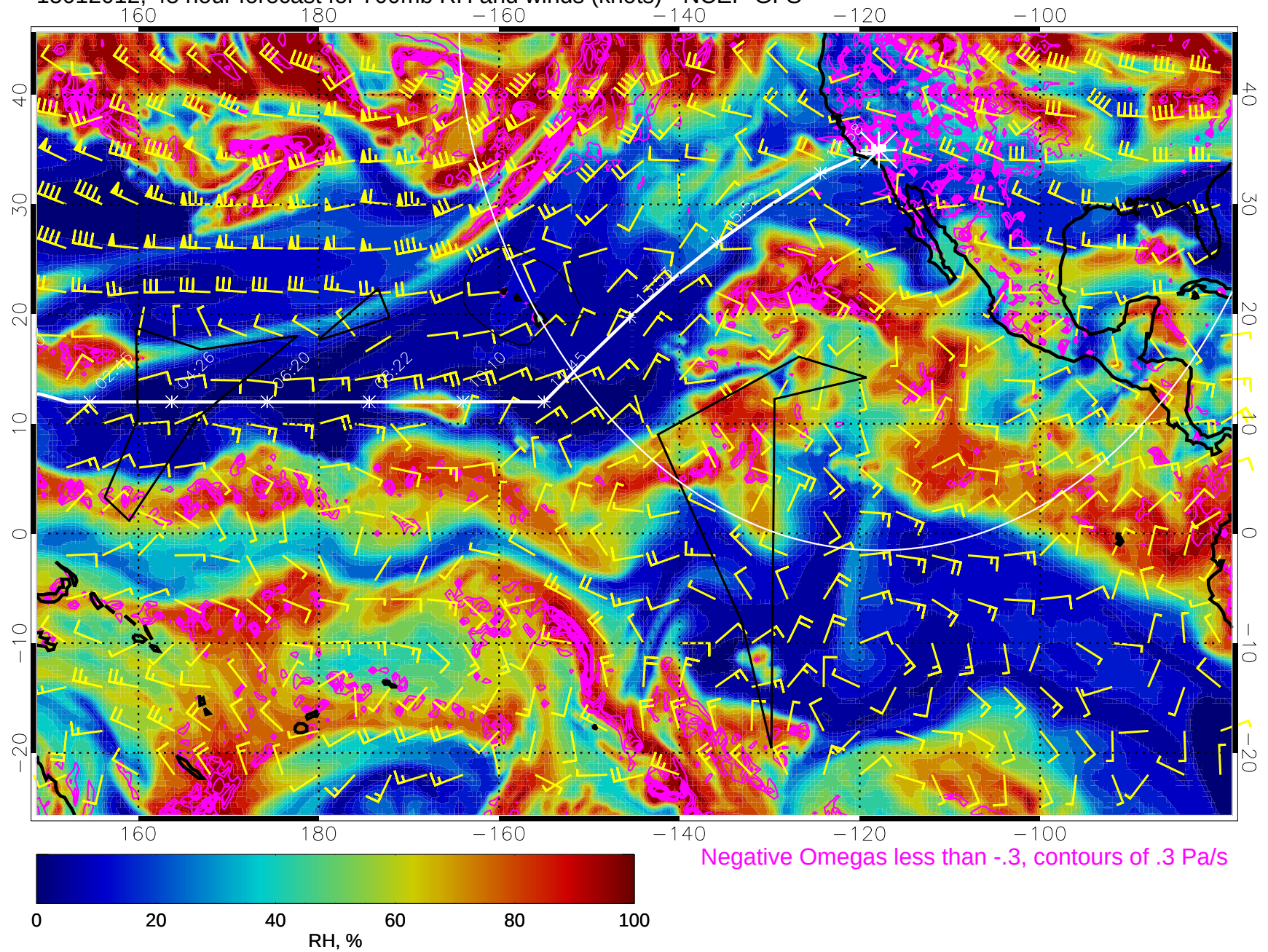
15012012, 48 hour forecast for 700mb RH and winds (knots) - NCEP GFS
