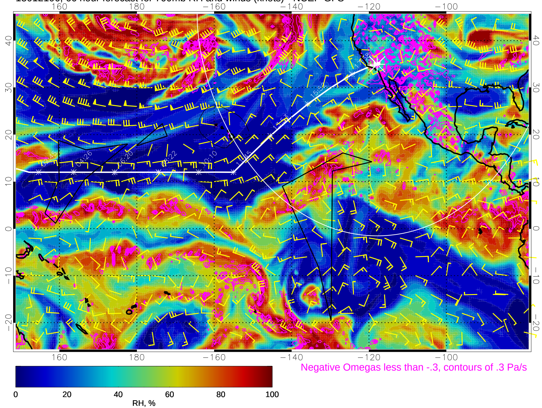
15012106, 66 hour forecast for 700mb RH and winds (knots) - NCEP GFS
