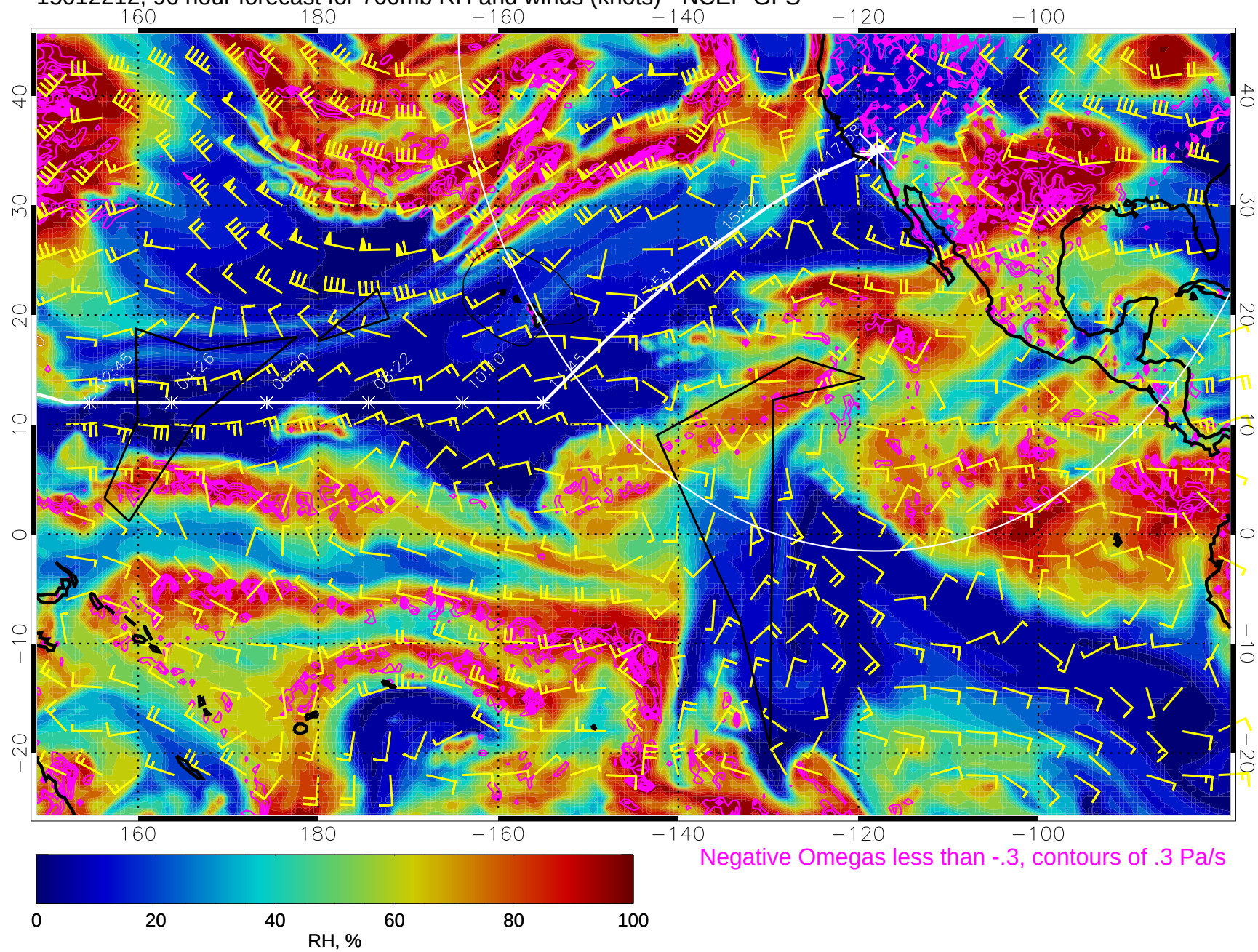
15012212, 96 hour forecast for 700mb RH and winds (knots) - NCEP GFS
