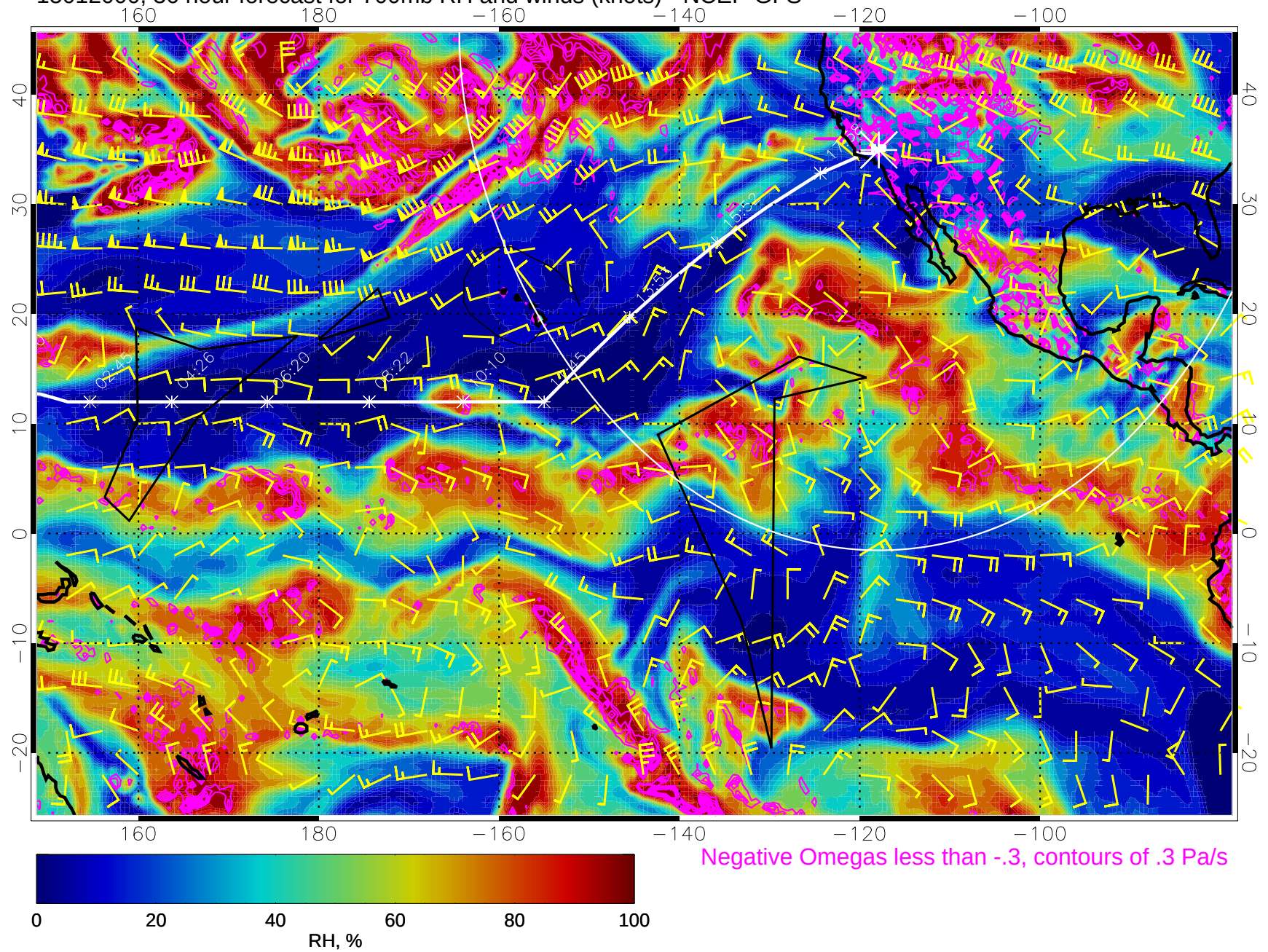
15012000, 36 hour forecast for 700mb RH and winds (knots) - NCEP GFS
