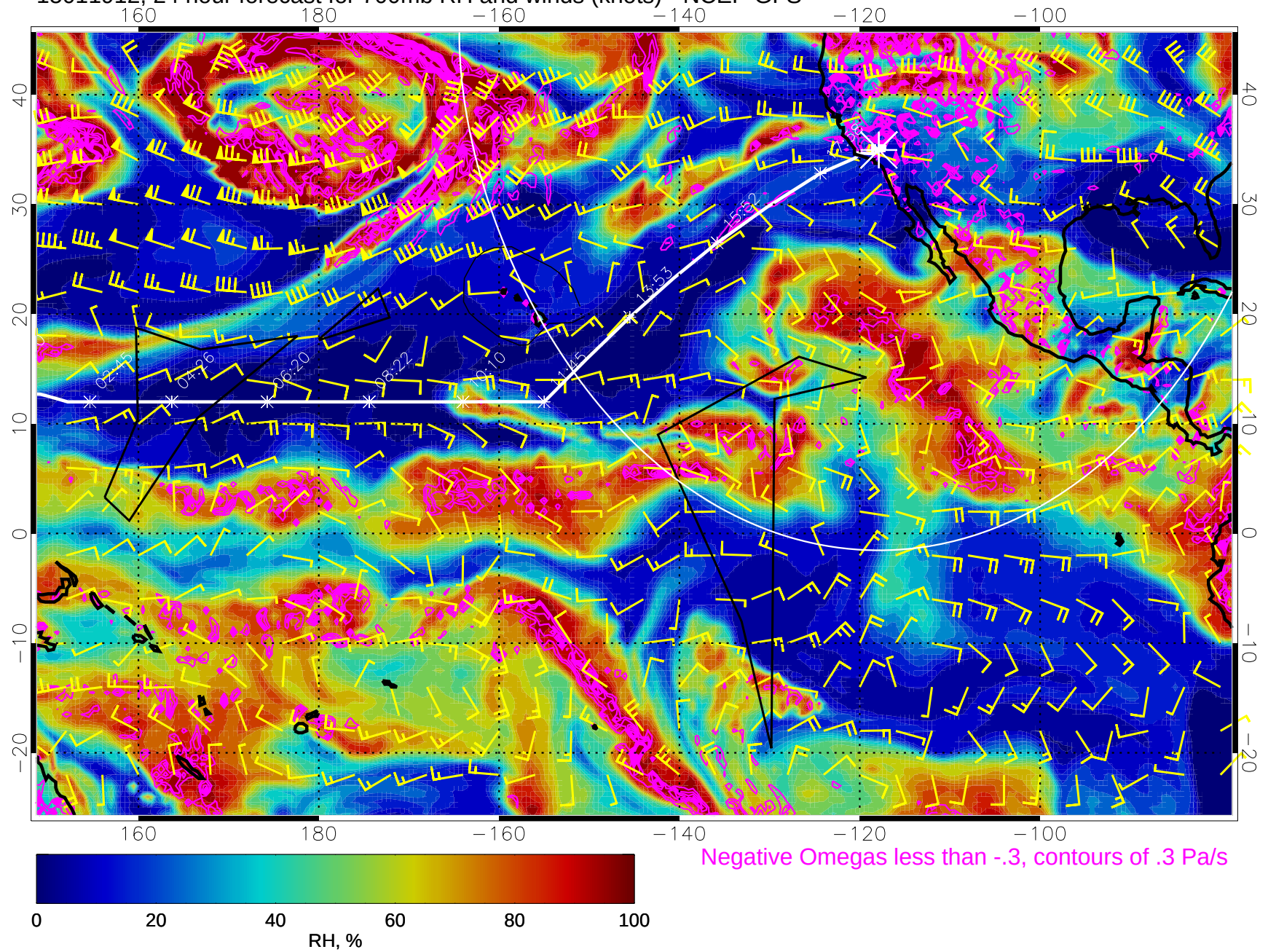
15011912, 24 hour forecast for 700mb RH and winds (knots) - NCEP GFS
