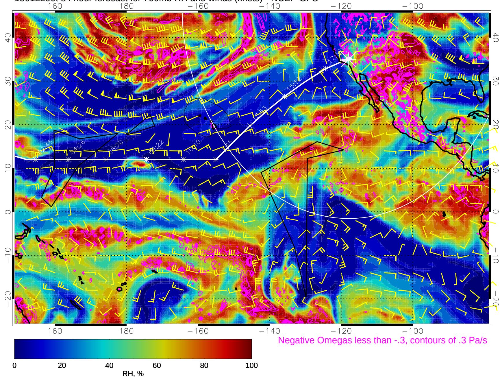
15012200, 84 hour forecast for 700mb RH and winds (knots) - NCEP GFS
