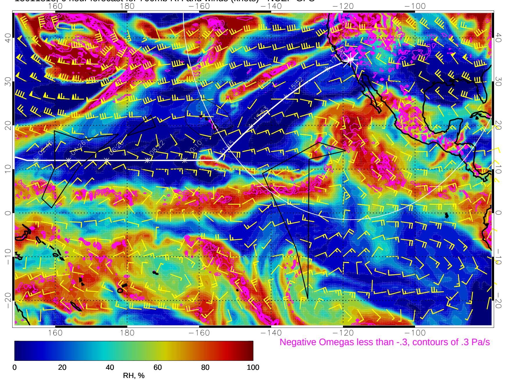
15011818, 6 hour forecast for 700mb RH and winds (knots) - NCEP GFS
