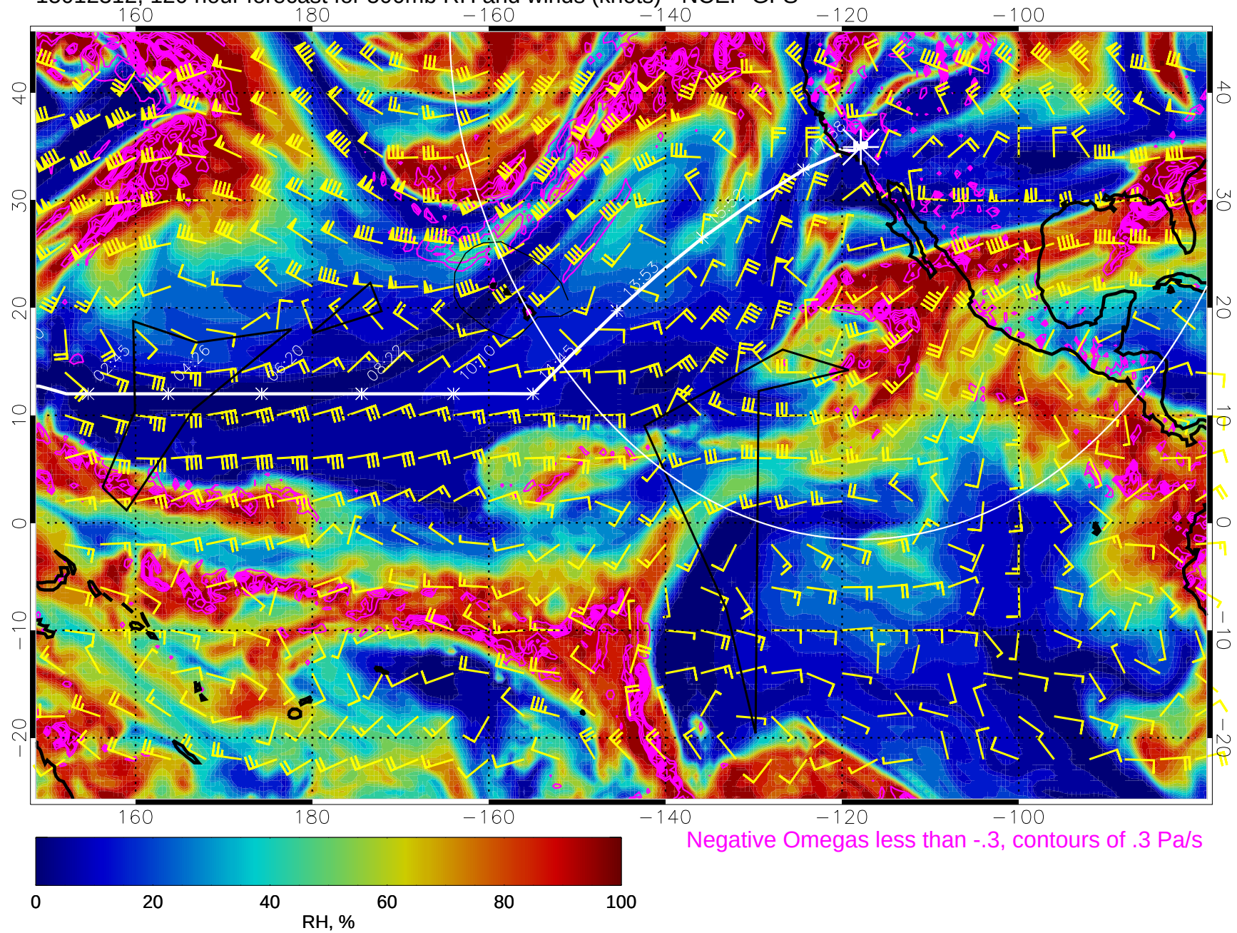
15012312, 120 hour forecast for 500mb RH and winds (knots) - NCEP GFS
