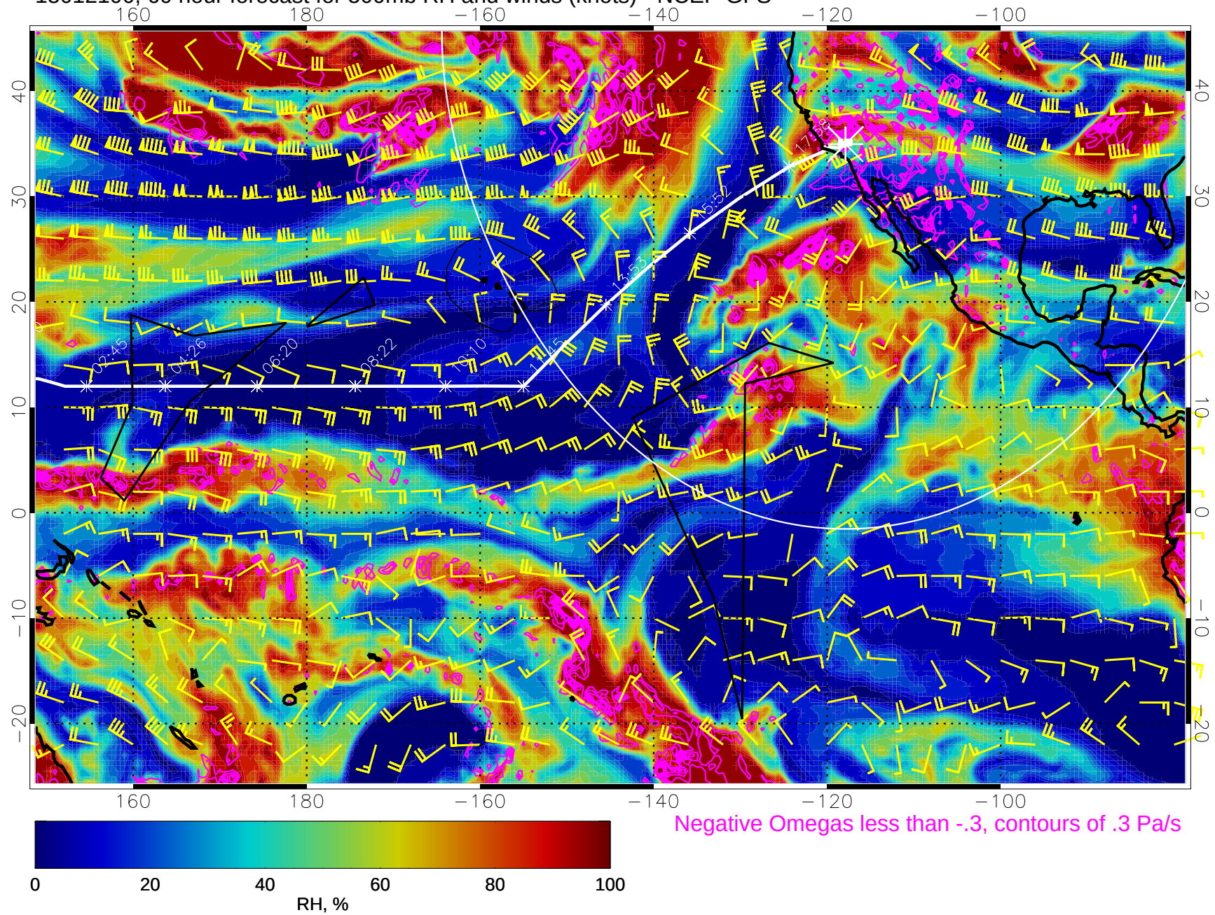
15012100, 60 hour forecast for 500mb RH and winds (knots) - NCEP GFS
