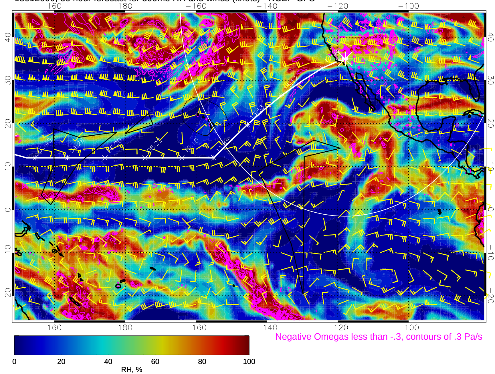
15012000, 36 hour forecast for 500mb RH and winds (knots) - NCEP GFS
