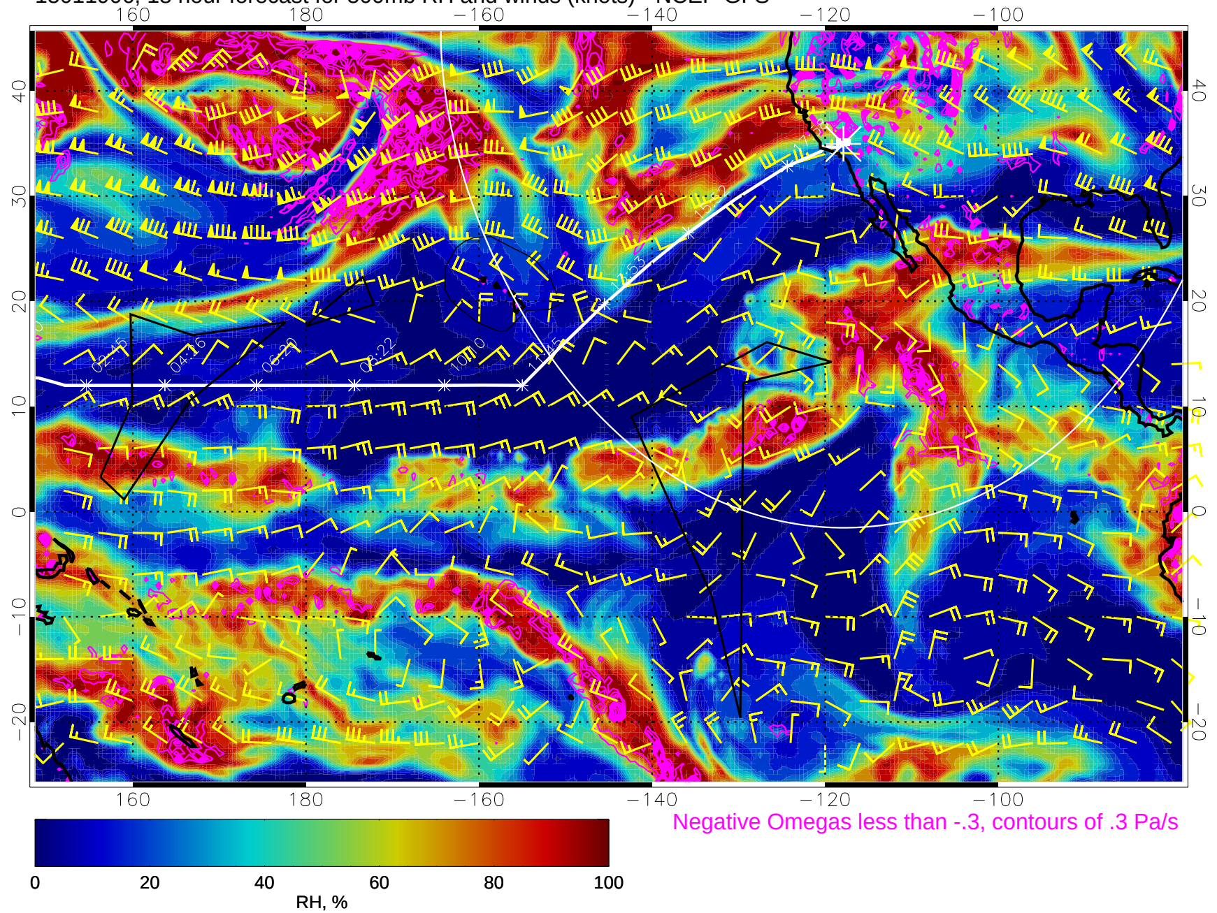
15011906, 18 hour forecast for 500mb RH and winds (knots) - NCEP GFS
