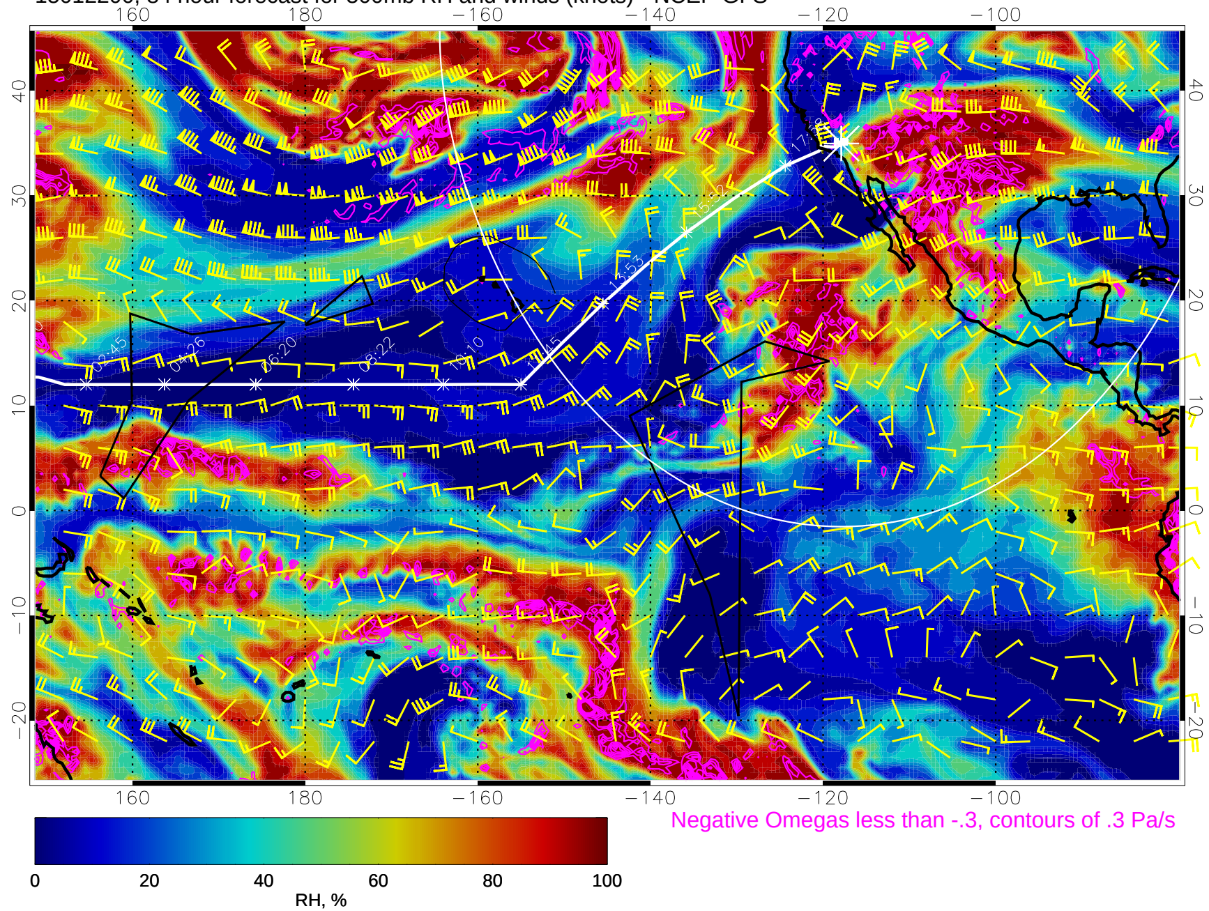
15012200, 84 hour forecast for 500mb RH and winds (knots) - NCEP GFS
