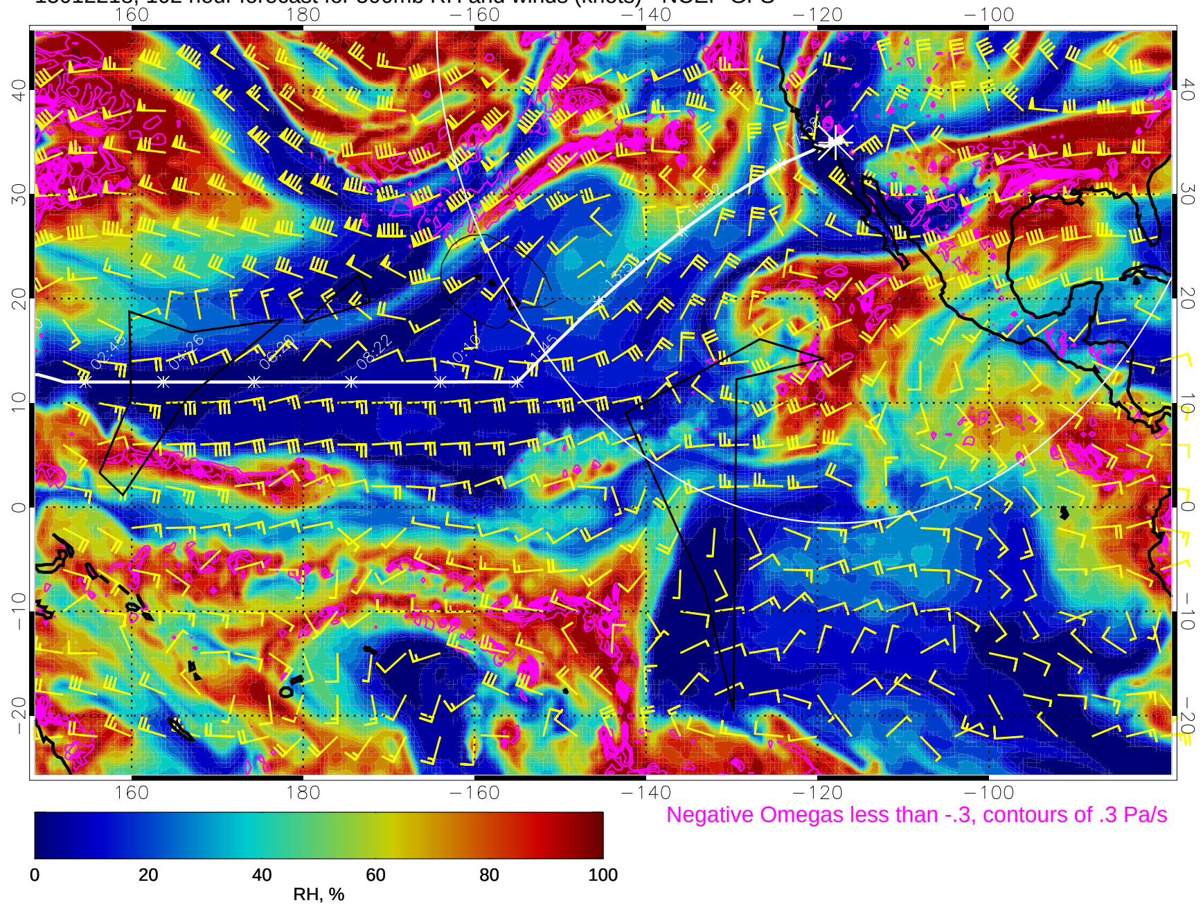
15012218, 102 hour forecast for 500mb RH and winds (knots) - NCEP GFS
