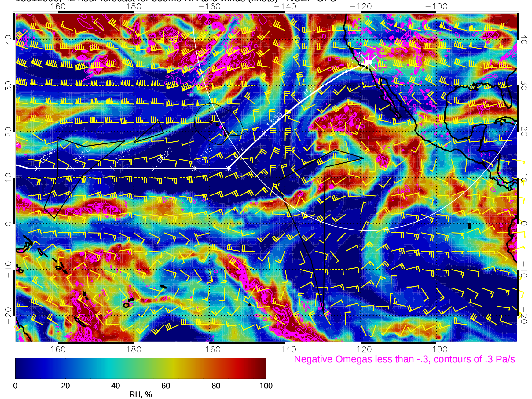
15012006, 42 hour forecast for 500mb RH and winds (knots) - NCEP GFS
