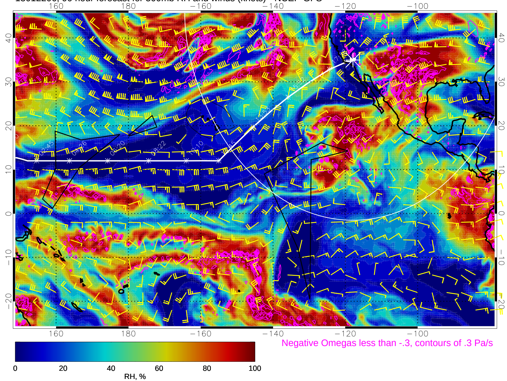
15012206, 90 hour forecast for 500mb RH and winds (knots) - NCEP GFS
