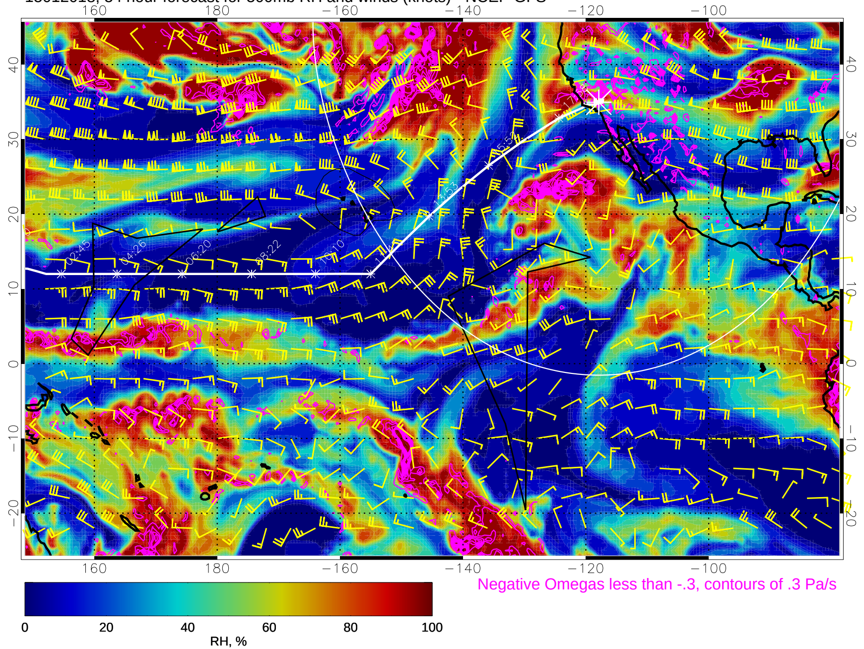
15012018, 54 hour forecast for 500mb RH and winds (knots) - NCEP GFS
