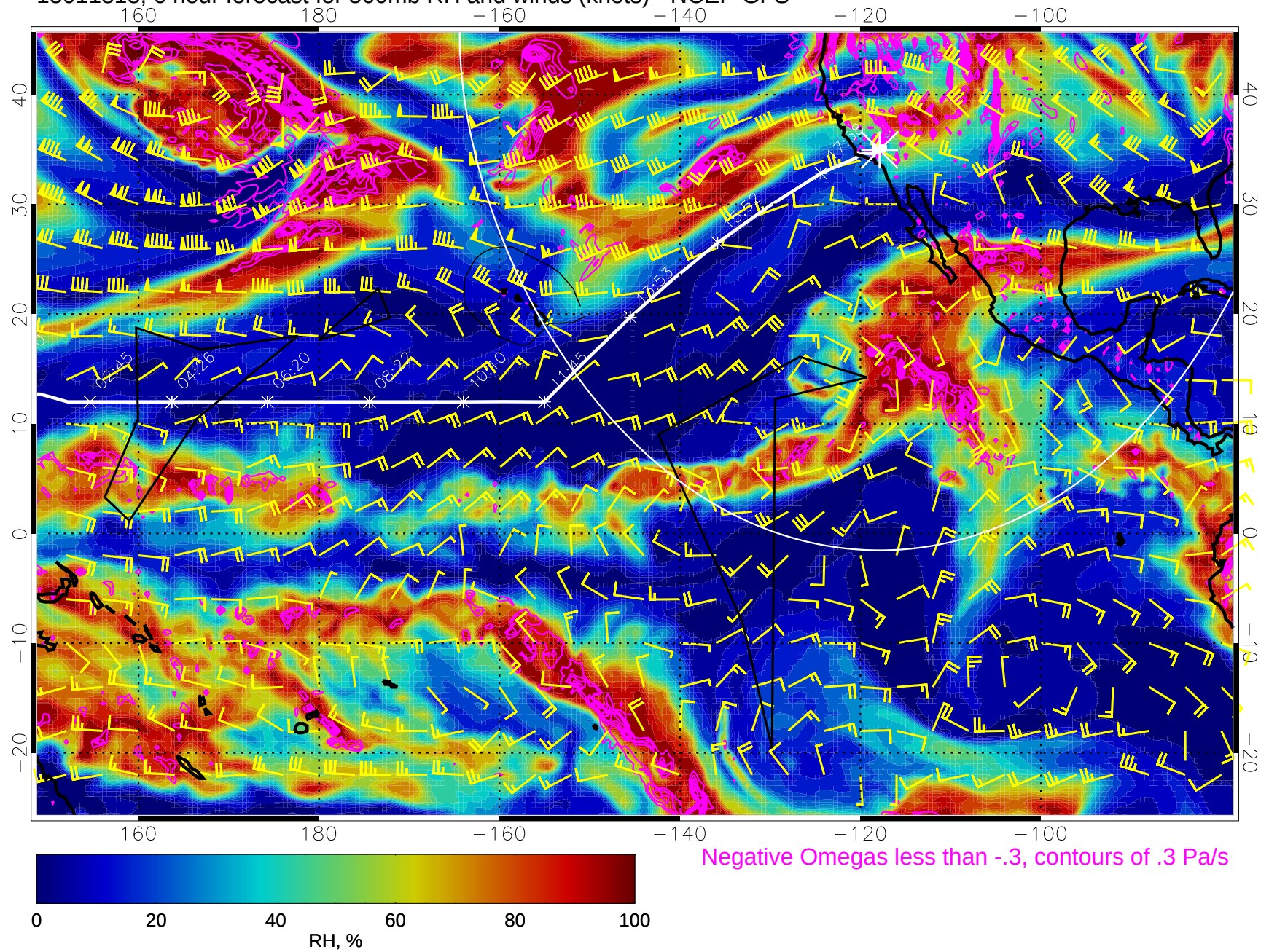
15011818, 6 hour forecast for 500mb RH and winds (knots) - NCEP GFS
