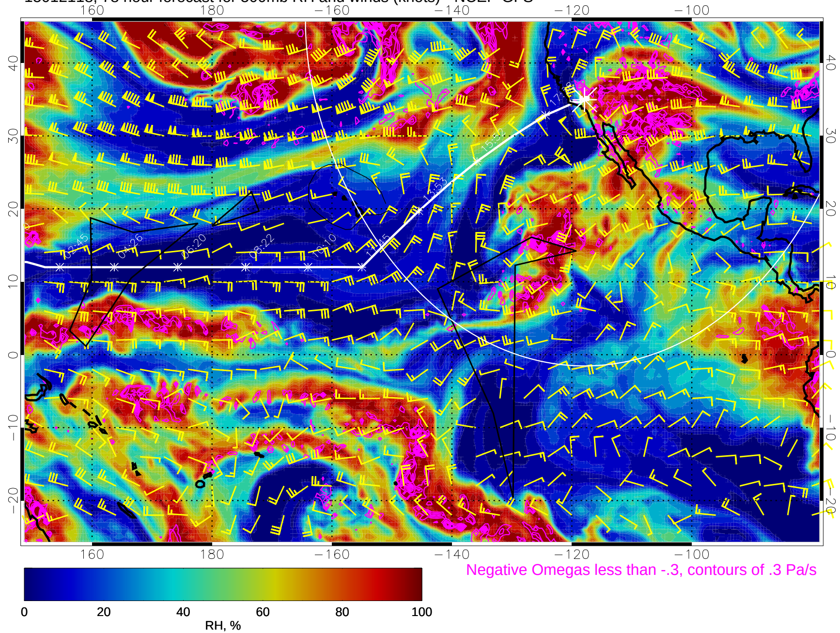
15012118, 78 hour forecast for 500mb RH and winds (knots) - NCEP GFS
