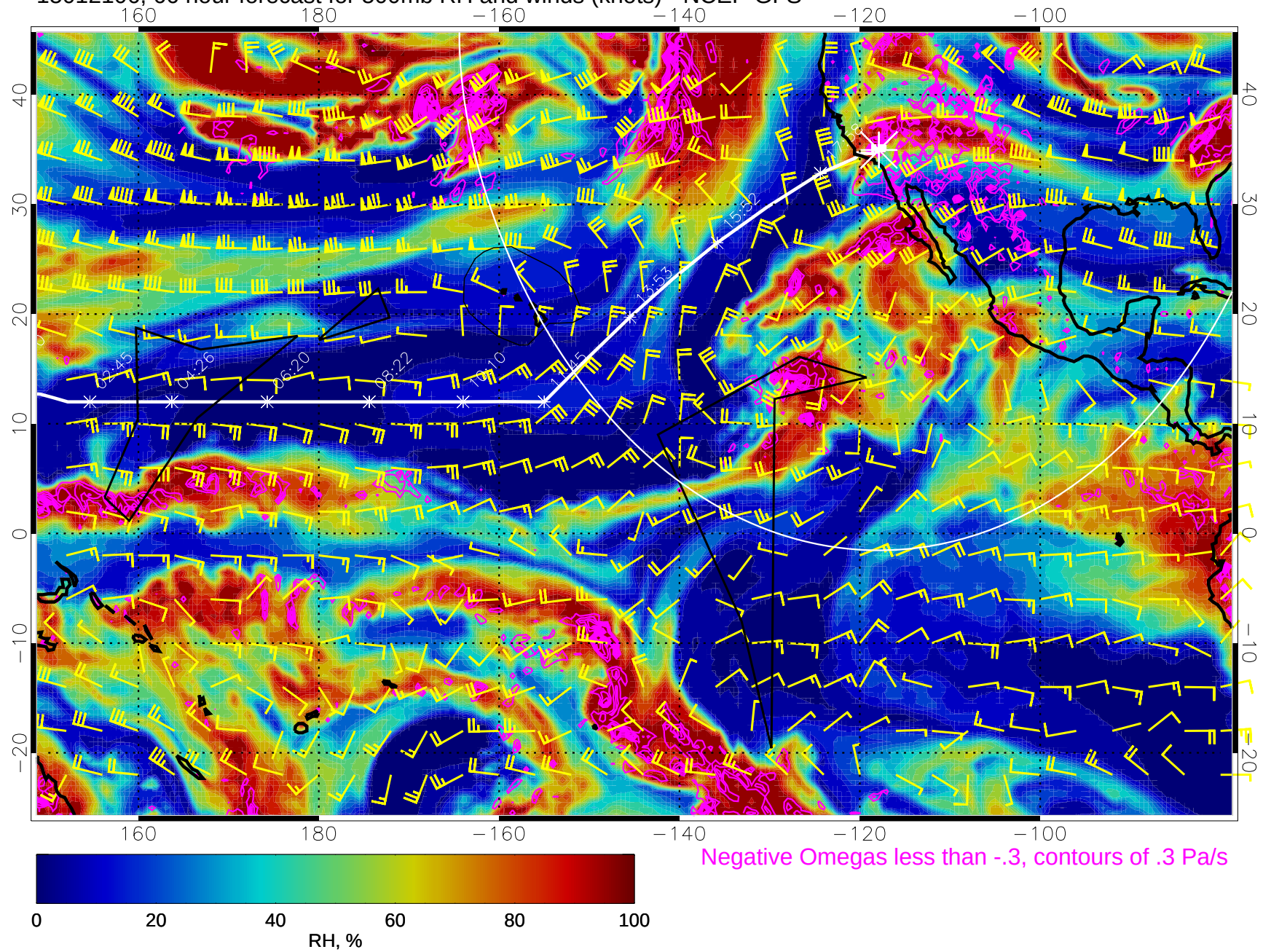
15012106, 66 hour forecast for 500mb RH and winds (knots) - NCEP GFS
