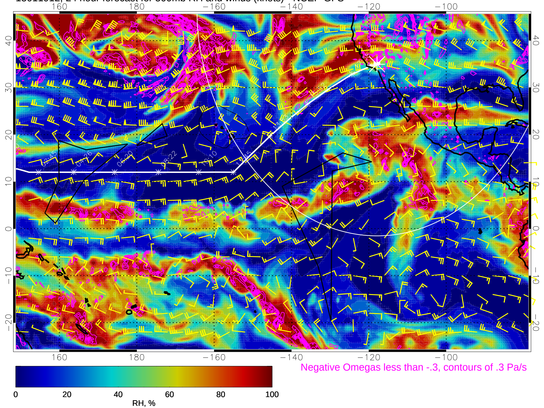
15011912, 24 hour forecast for 500mb RH and winds (knots) - NCEP GFS
