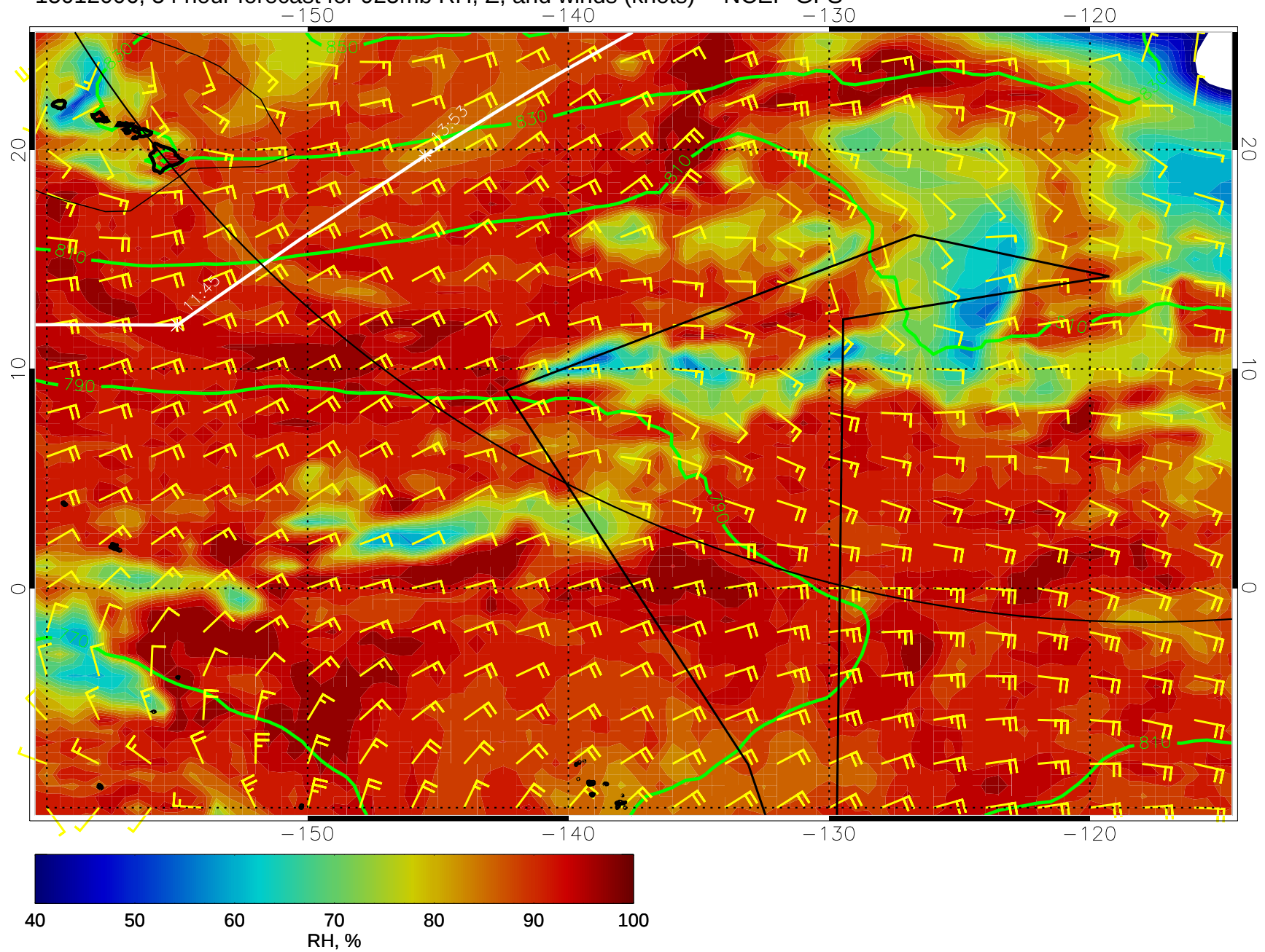
15012006, 54 hour forecast for 925mb RH, Z, and winds (knots) -- NCEP GFS
