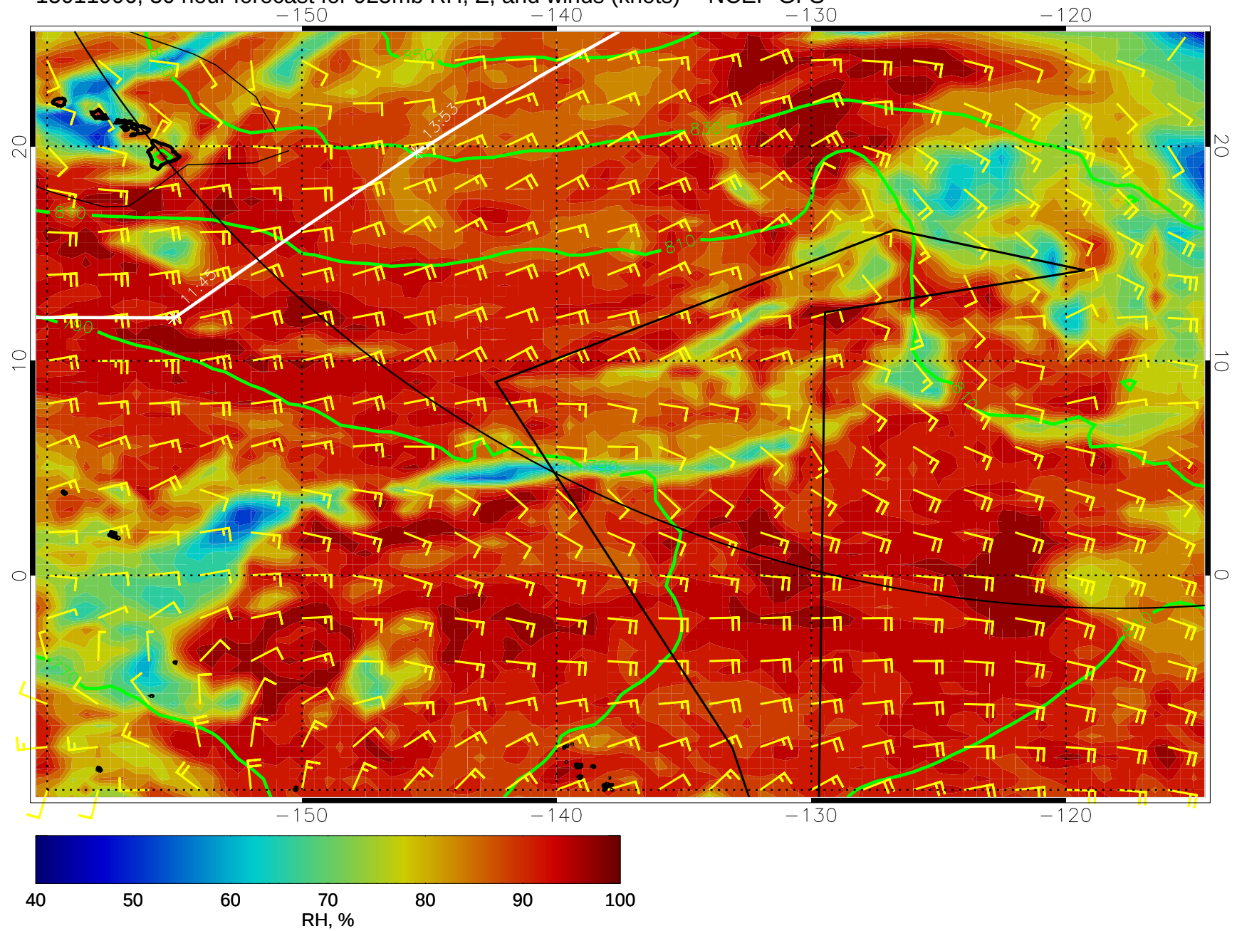
15011906, 30 hour forecast for 925mb RH, Z, and winds (knots) -- NCEP GFS
