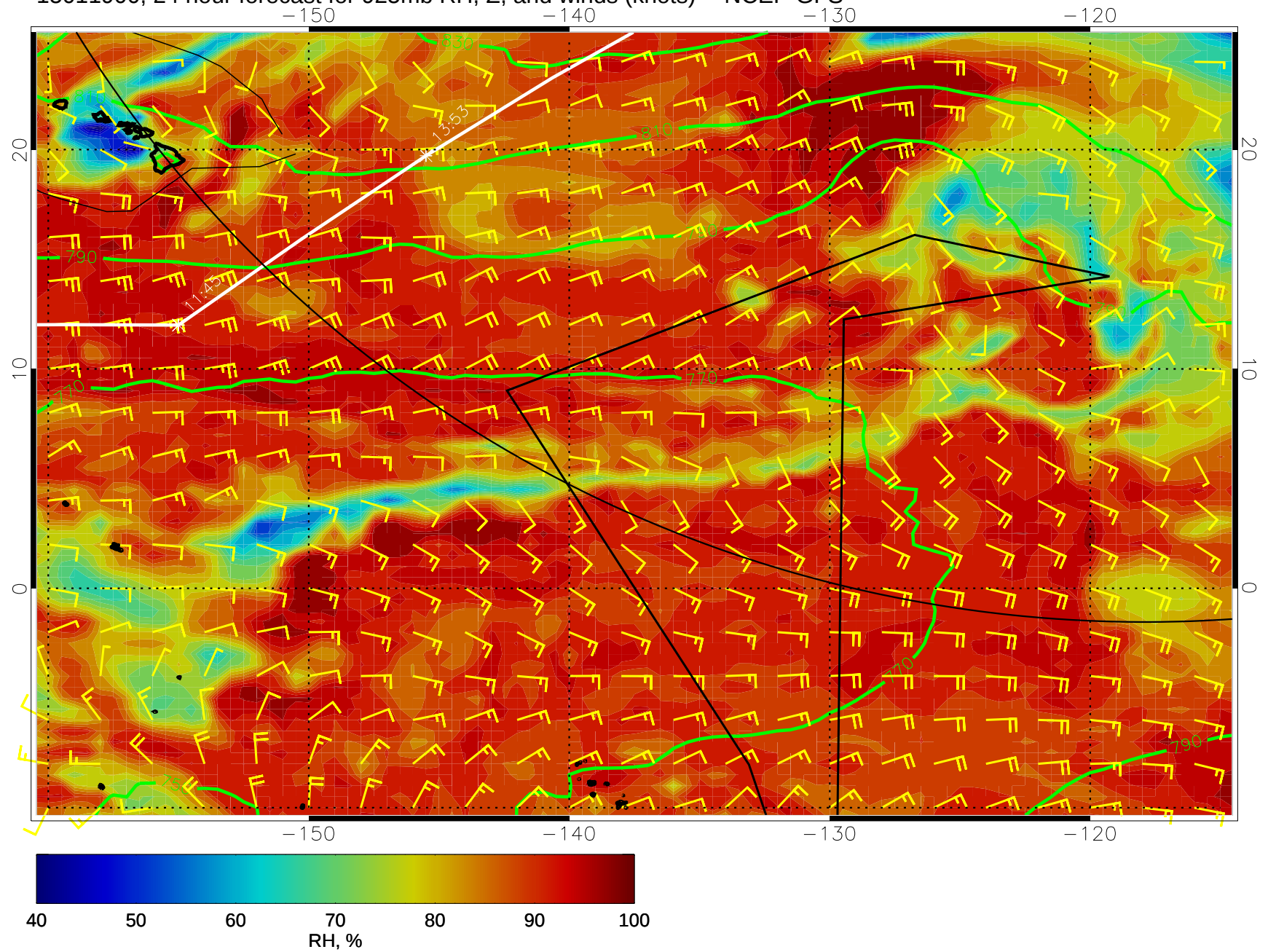
15011900, 24 hour forecast for 925mb RH, Z, and winds (knots) -- NCEP GFS
