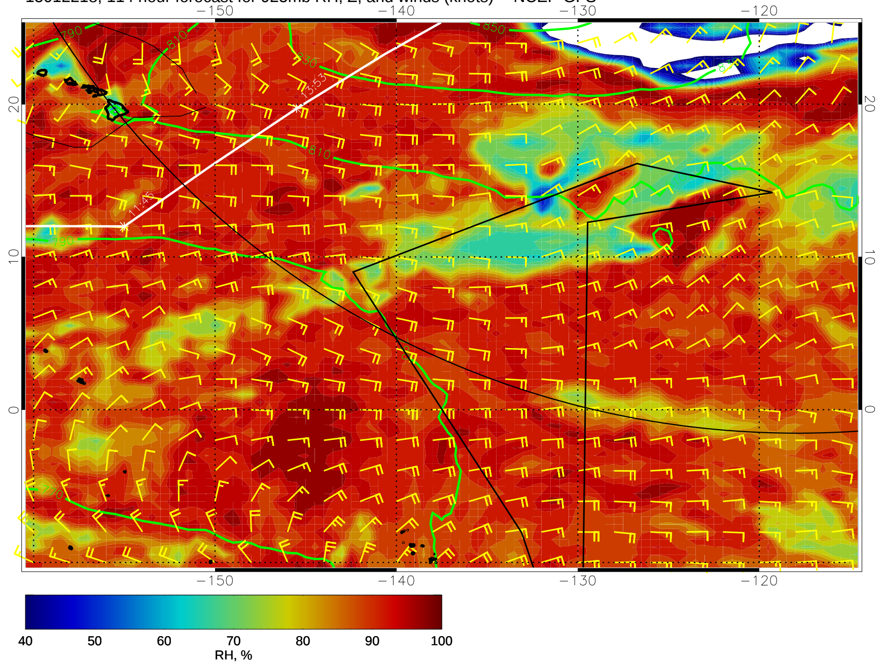
15012218, 114 hour forecast for 925mb RH, Z, and winds (knots) -- NCEP GFS
