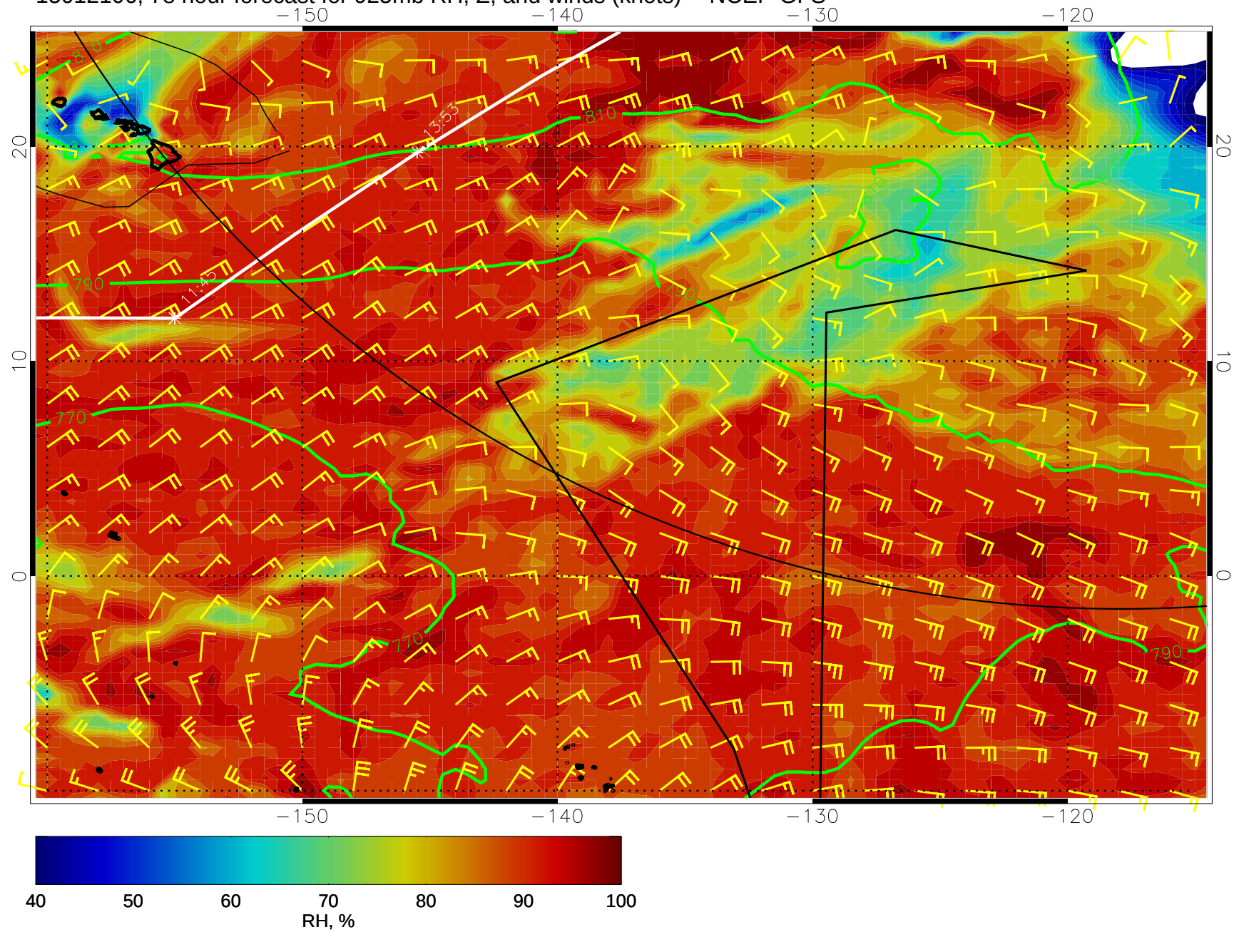
15012106, 78 hour forecast for 925mb RH, Z, and winds (knots) -- NCEP GFS
