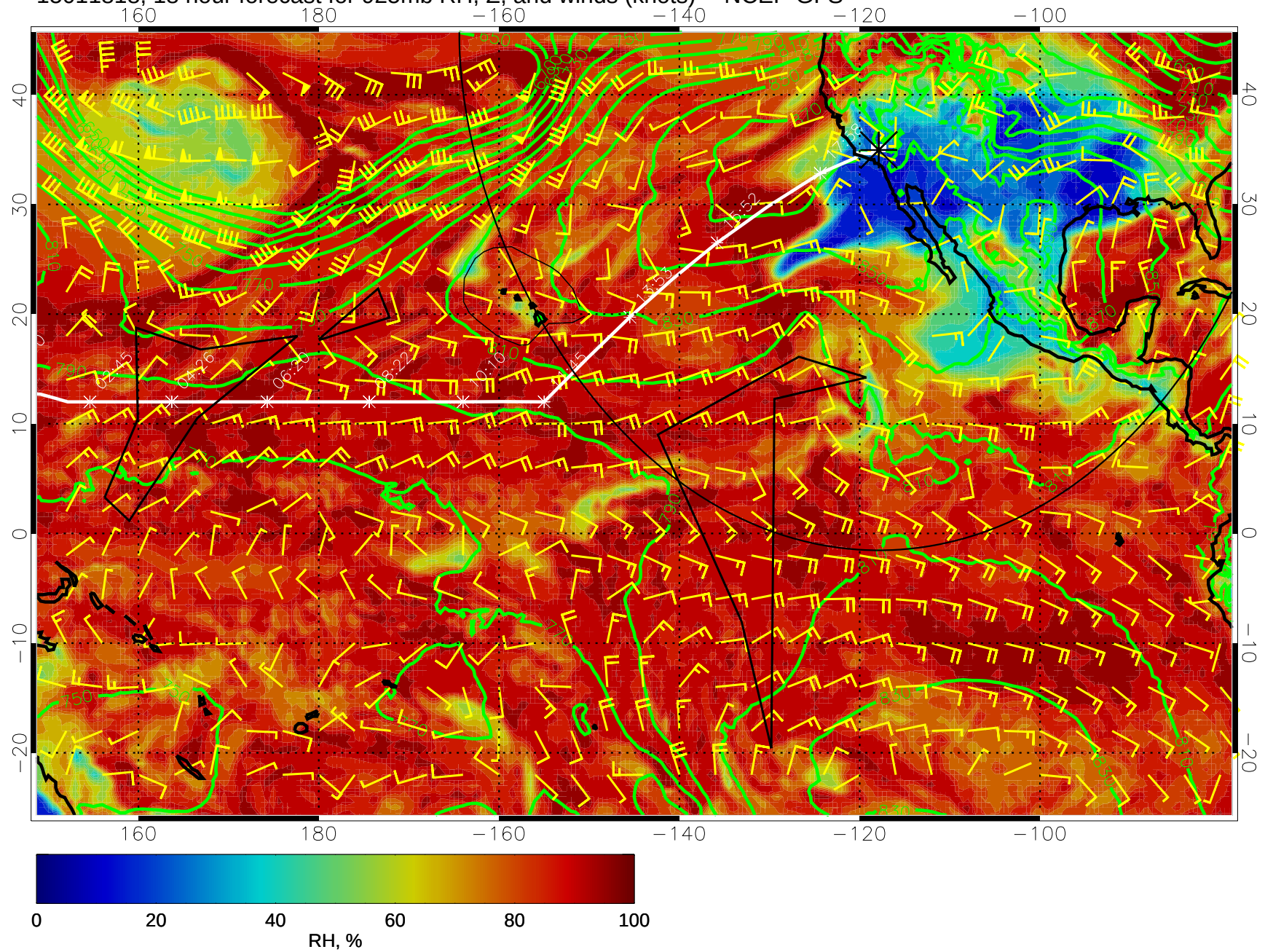
15011818, 18 hour forecast for 925mb RH, Z, and winds (knots) -- NCEP GFS
