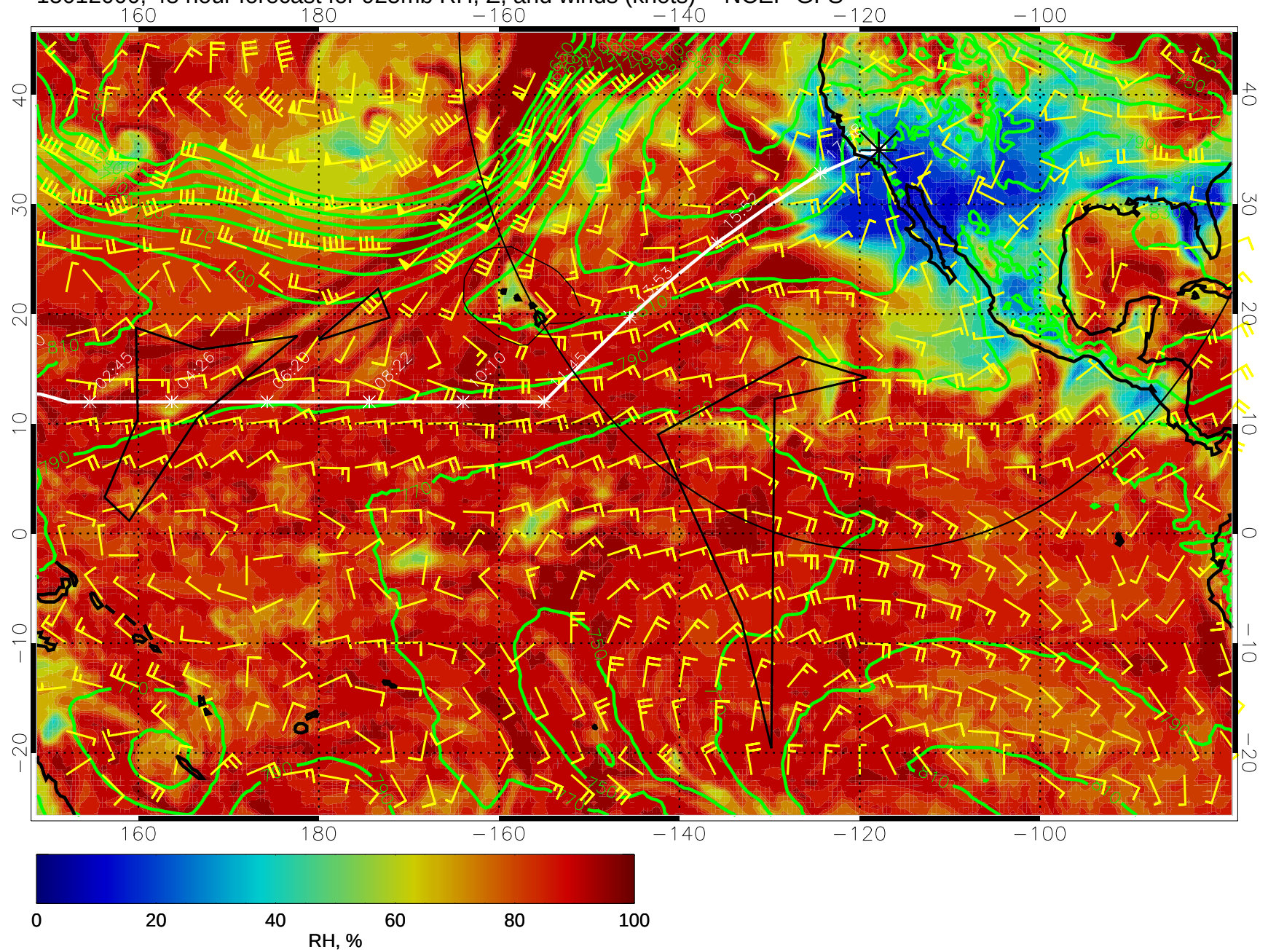
15012000, 48 hour forecast for 925mb RH, Z, and winds (knots) -- NCEP GFS
