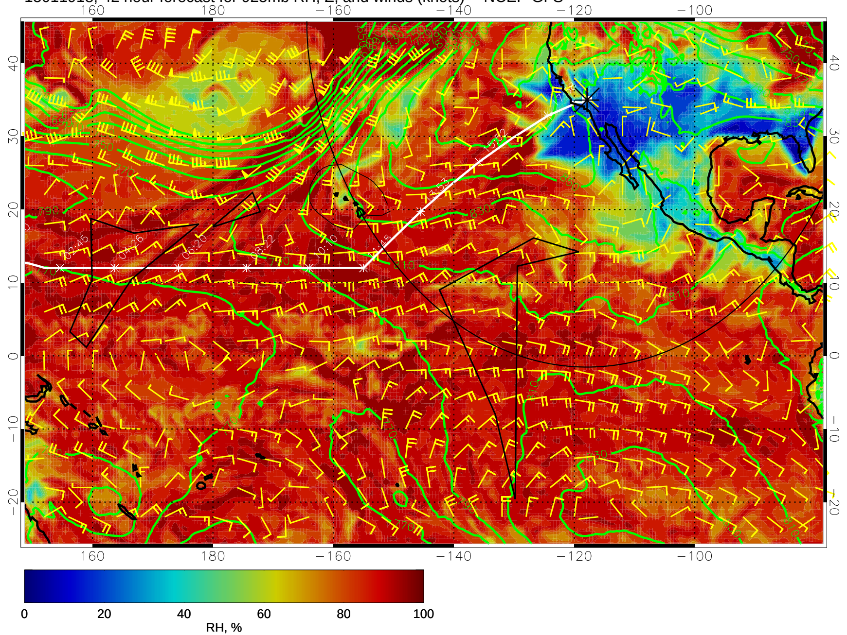
15011918, 42 hour forecast for 925mb RH, Z, and winds (knots) -- NCEP GFS
