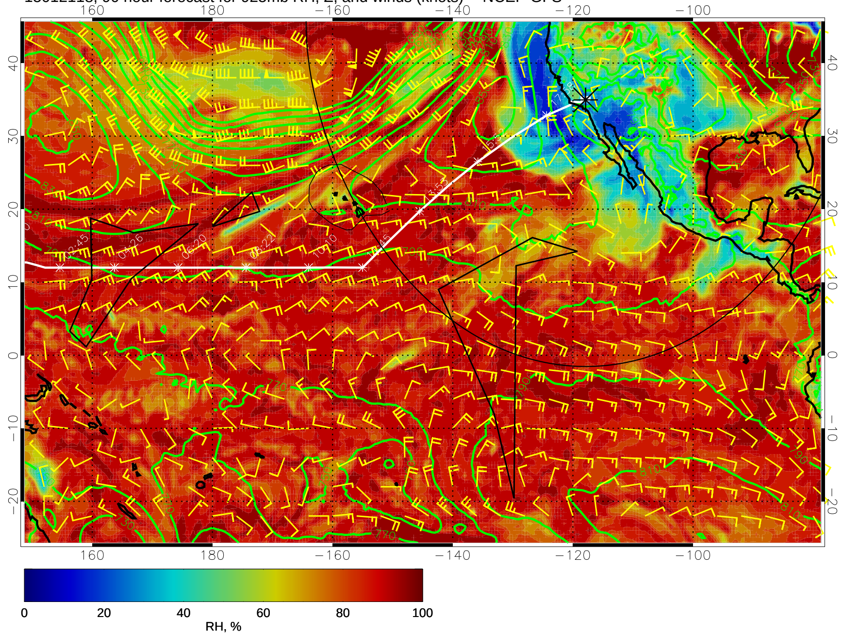
15012118, 90 hour forecast for 925mb RH, Z, and winds (knots) -- NCEP GFS
