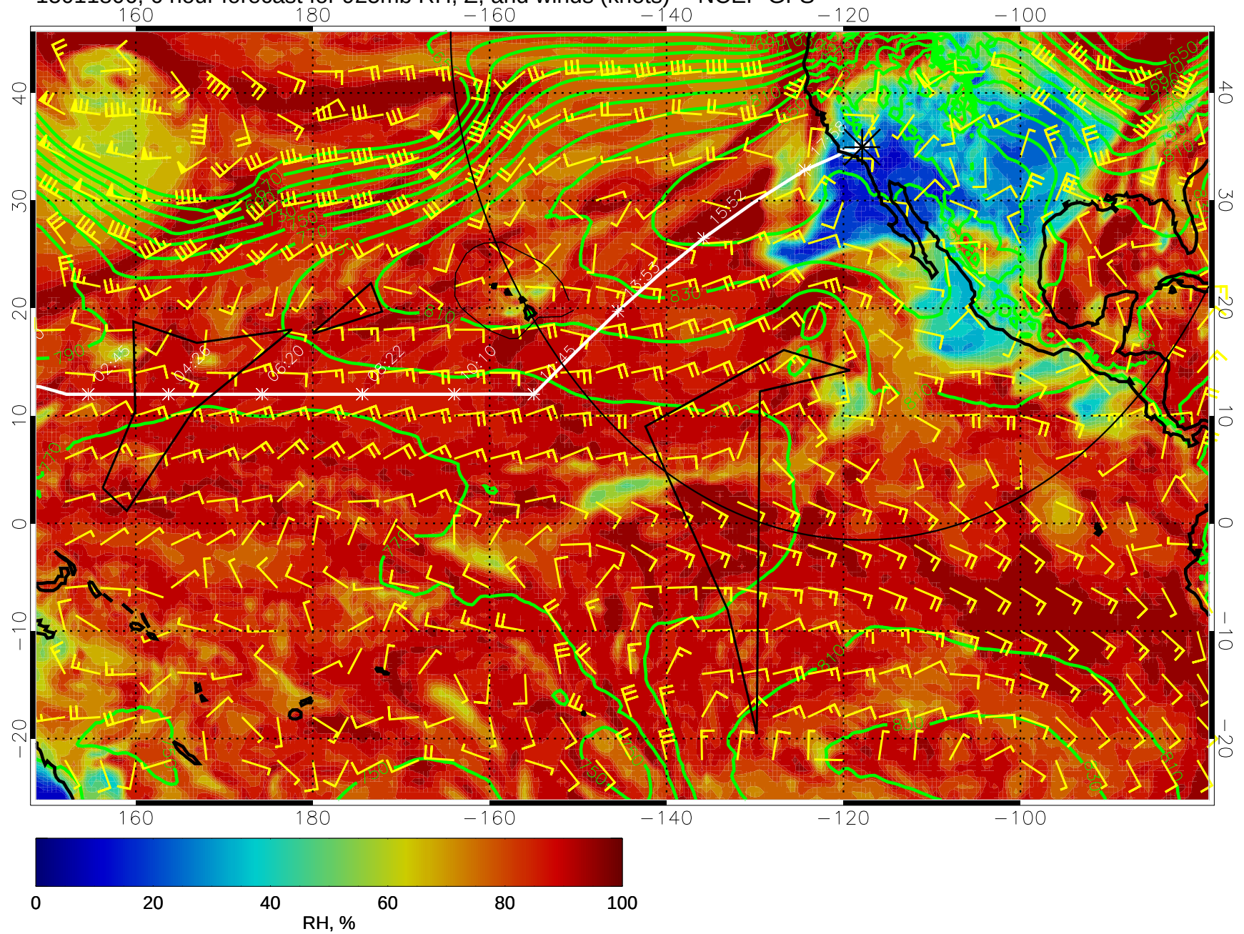
15011806, 6 hour forecast for 925mb RH, Z, and winds (knots) -- NCEP GFS
