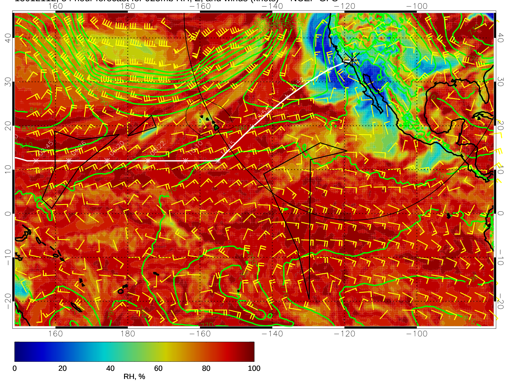
15012112, 84 hour forecast for 925mb RH, Z, and winds (knots) -- NCEP GFS
