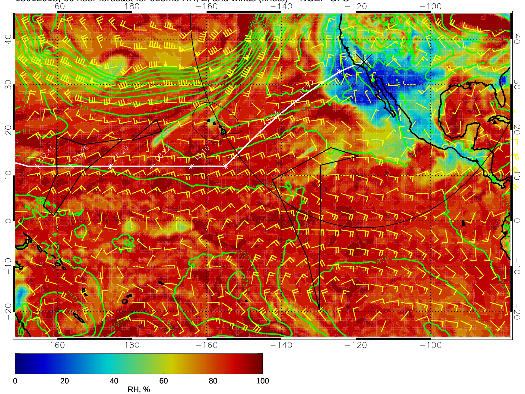
15012018, 66 hour forecast for 925mb RH, Z, and winds (knots) -- NCEP GFS
