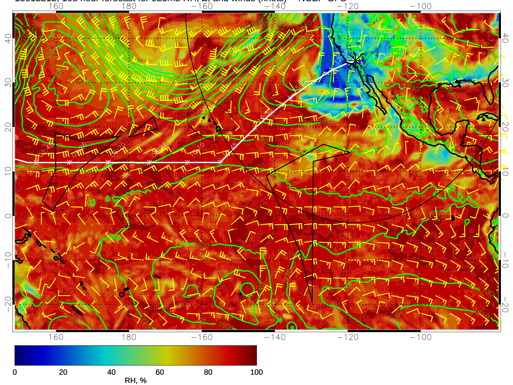
15012212, 108 hour forecast for 925mb RH, Z, and winds (knots) -- NCEP GFS
