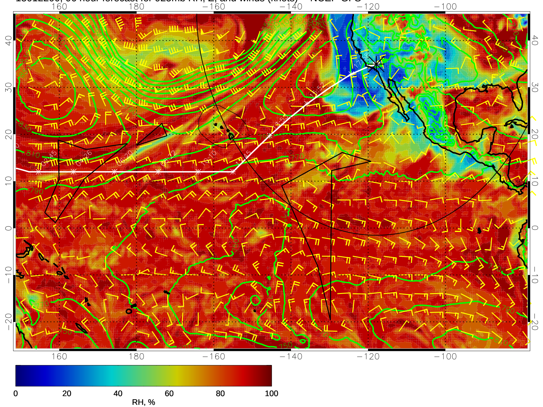
15012200, 96 hour forecast for 925mb RH, Z, and winds (knots) -- NCEP GFS
