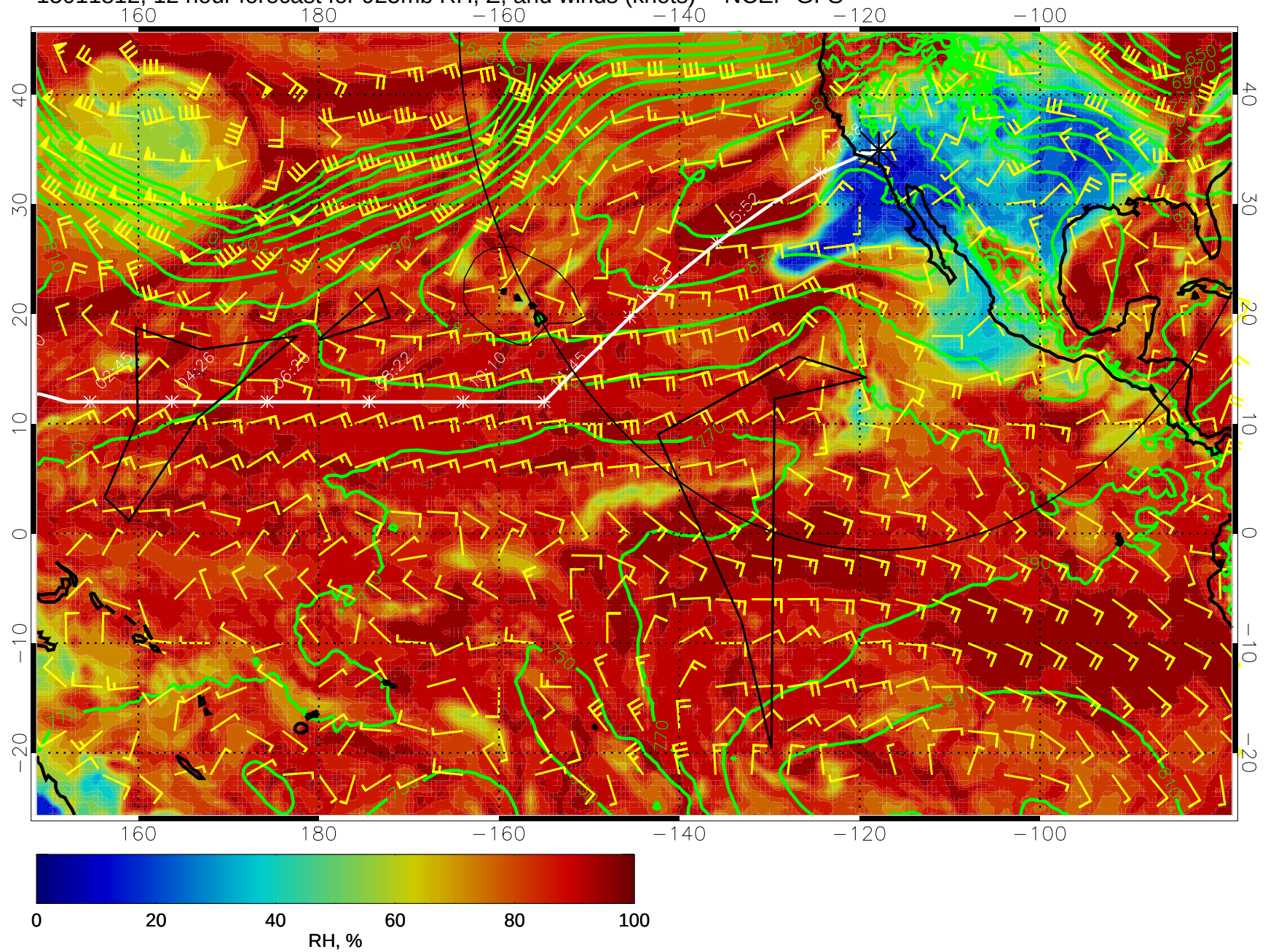
15011812, 12 hour forecast for 925mb RH, Z, and winds (knots) -- NCEP GFS
