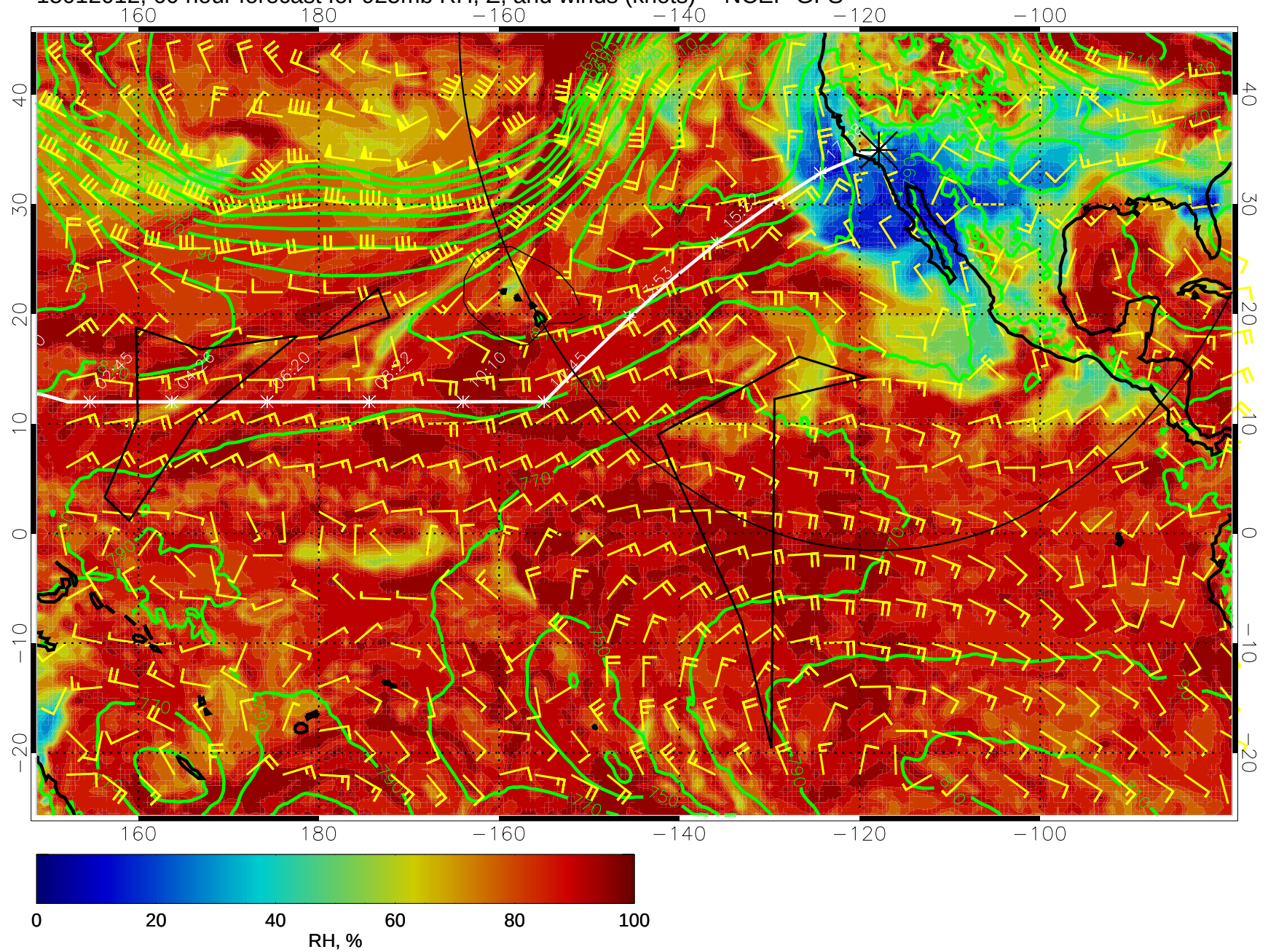
15012012, 60 hour forecast for 925mb RH, Z, and winds (knots) -- NCEP GFS
