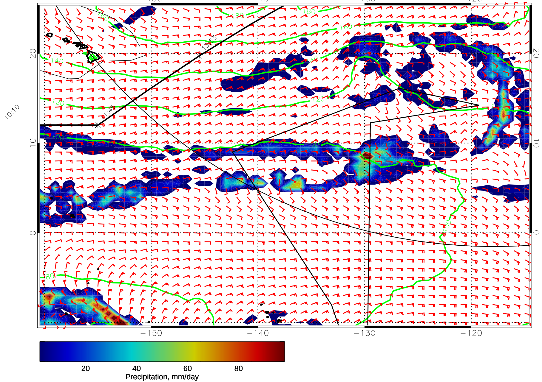
15011912, 36 hour forecast for precip, 1000mb Z, and winds (knots) -- NCEP GFS
