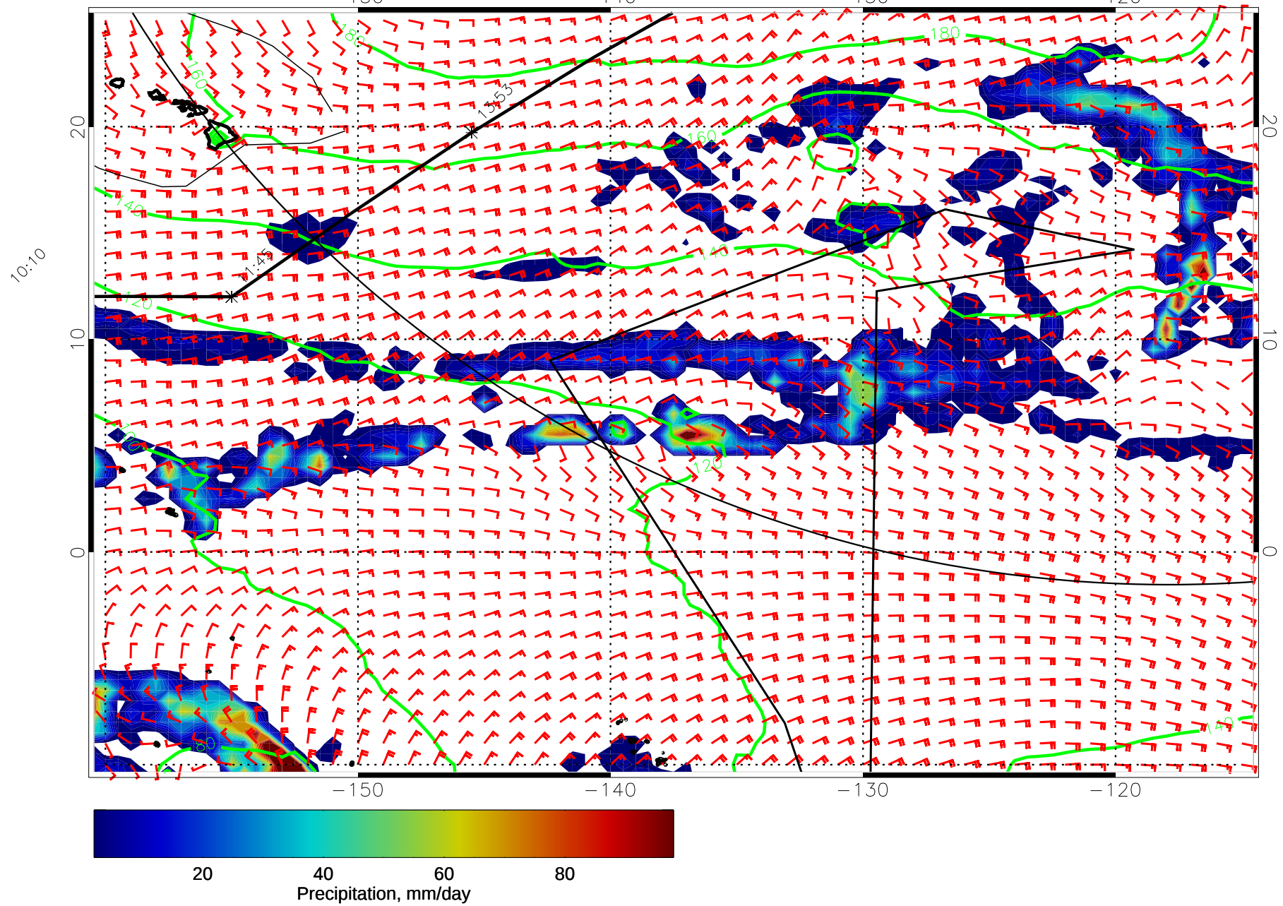
15011918, 42 hour forecast for precip, 1000mb Z, and winds (knots) -- NCEP GFS
