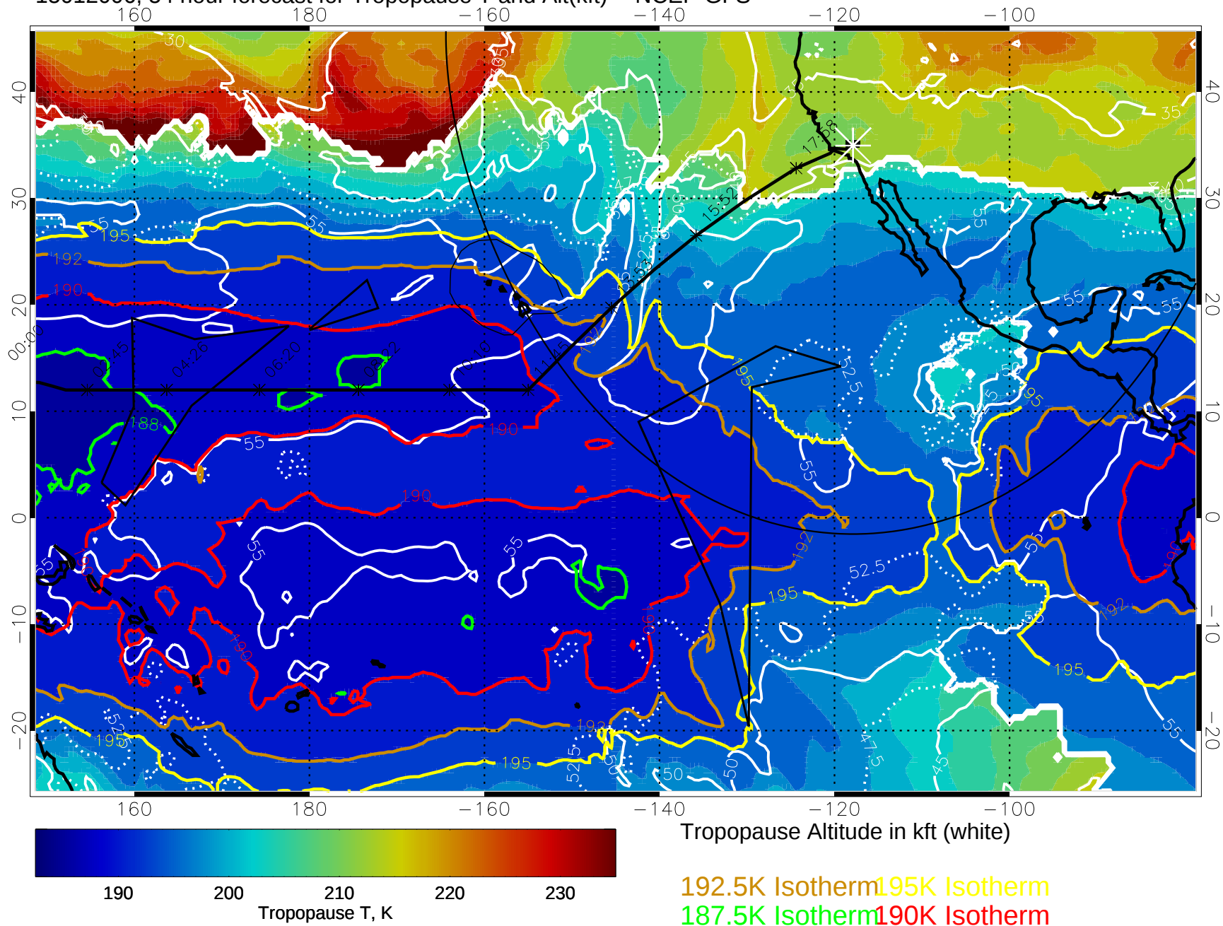
15012006, 54 hour forecast for Tropopause T and Alt(kft) -- NCEP GFS
