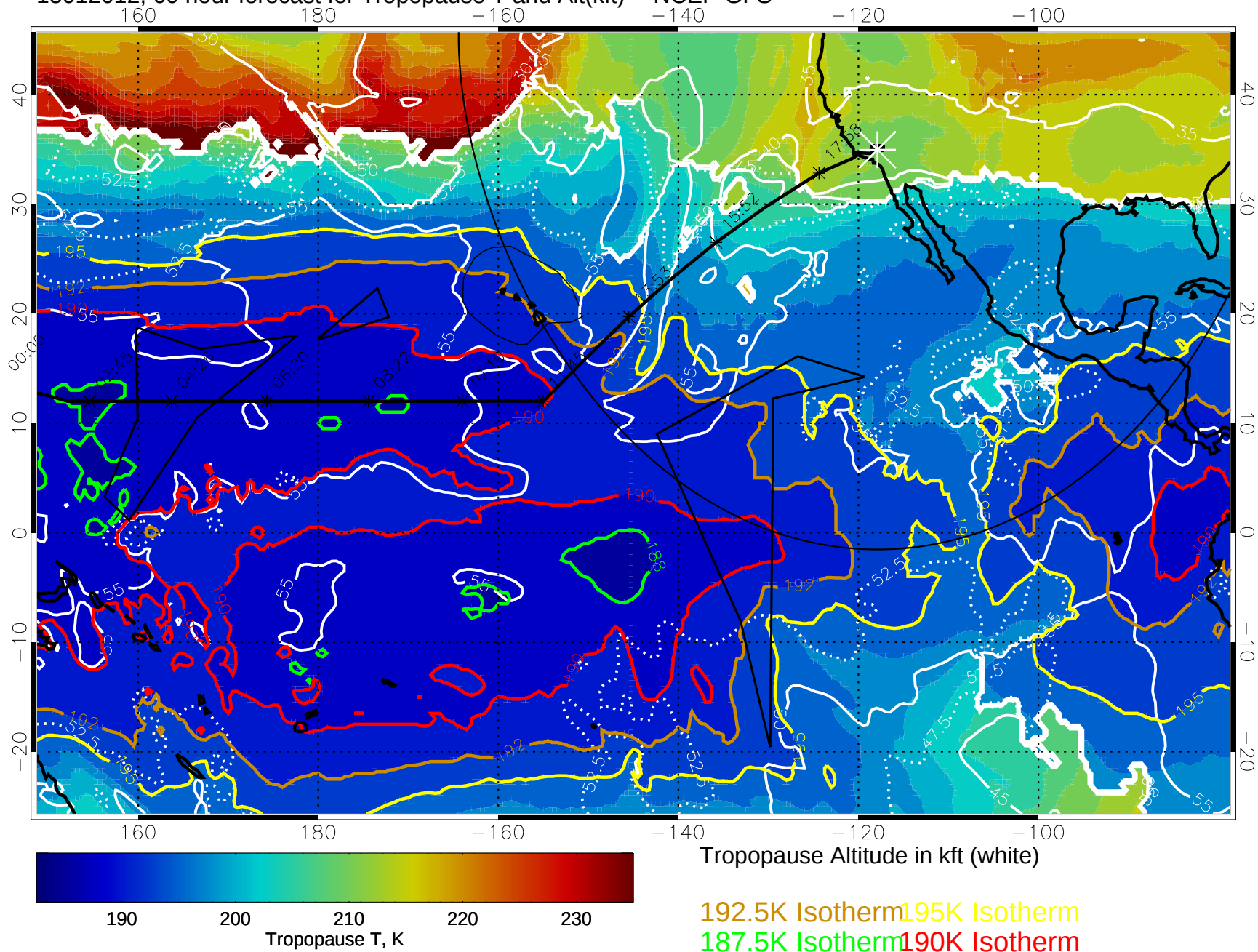
15012012, 60 hour forecast for Tropopause T and Alt(kft) -- NCEP GFS
