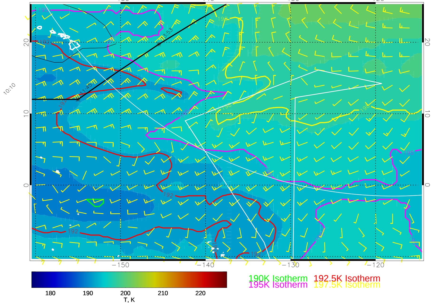
15012206, 102 hour forecast for 70mb T and winds (knots) -- NCEP GFS
