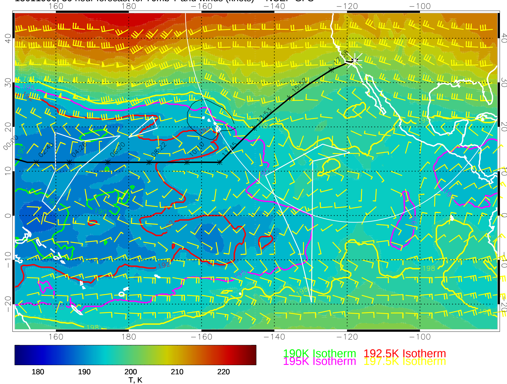
15011906, 30 hour forecast for 70mb T and winds (knots) -- NCEP GFS
