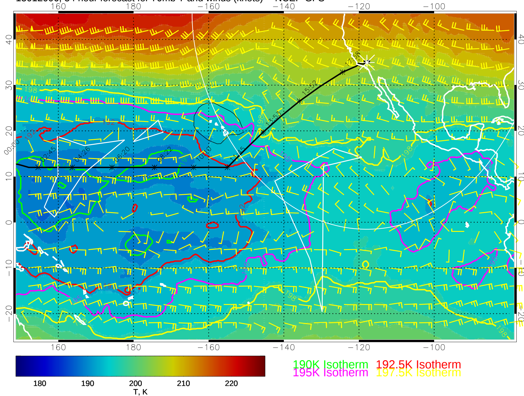
15012006, 54 hour forecast for 70mb T and winds (knots) -- NCEP GFS
