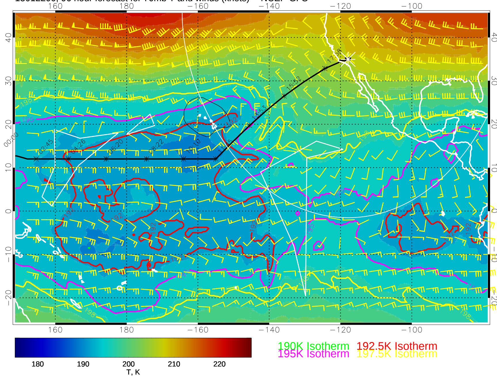
15012200, 96 hour forecast for 70mb T and winds (knots) -- NCEP GFS
