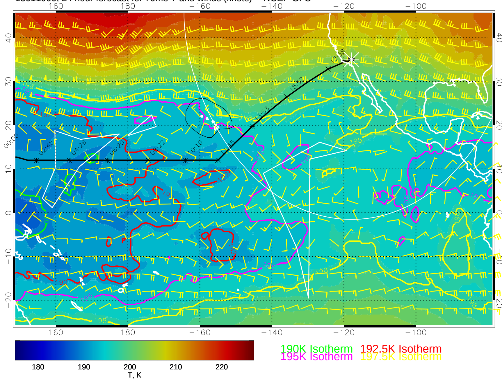
15011900, 24 hour forecast for 70mb T and winds (knots) -- NCEP GFS
