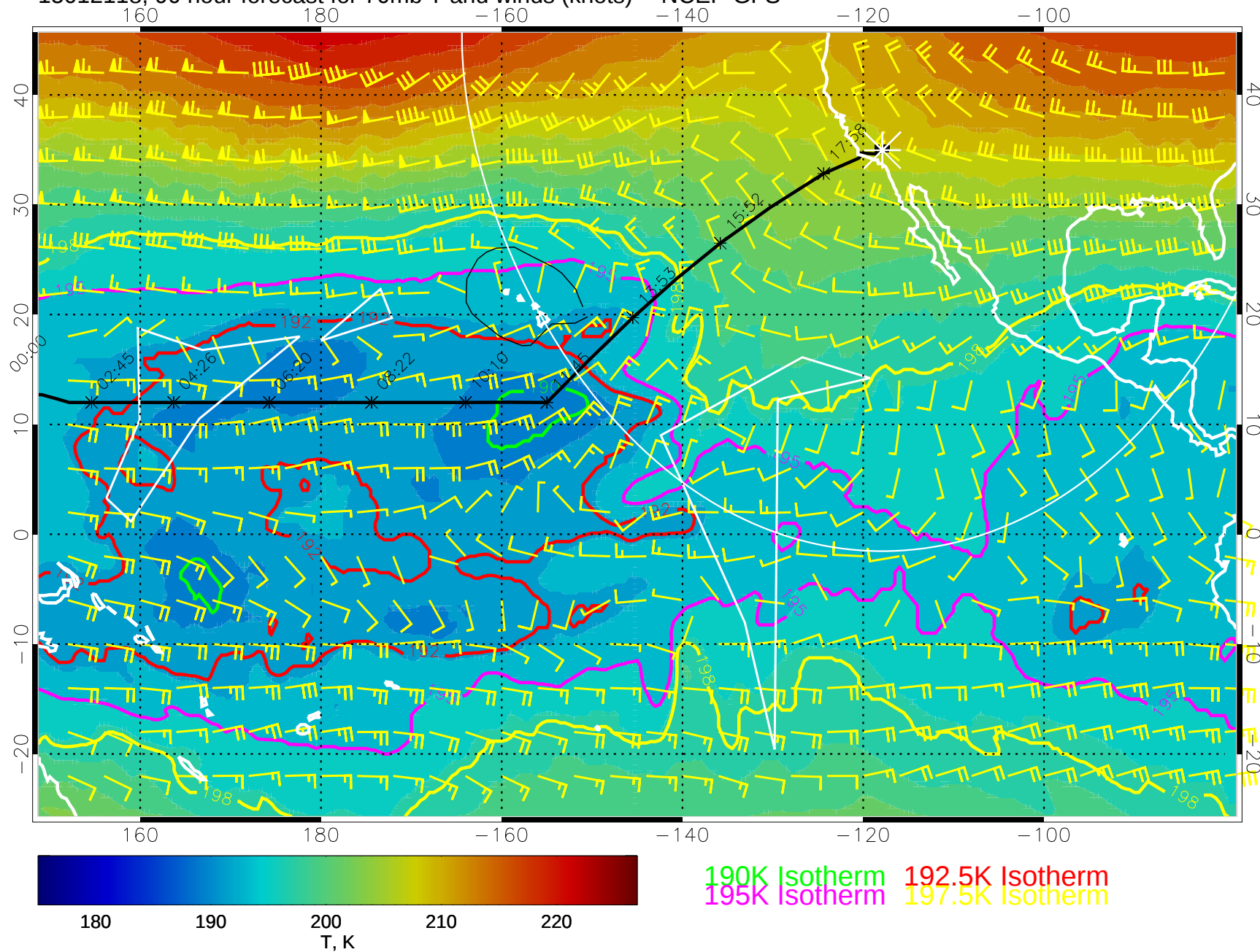
15012118, 90 hour forecast for 70mb T and winds (knots) -- NCEP GFS
