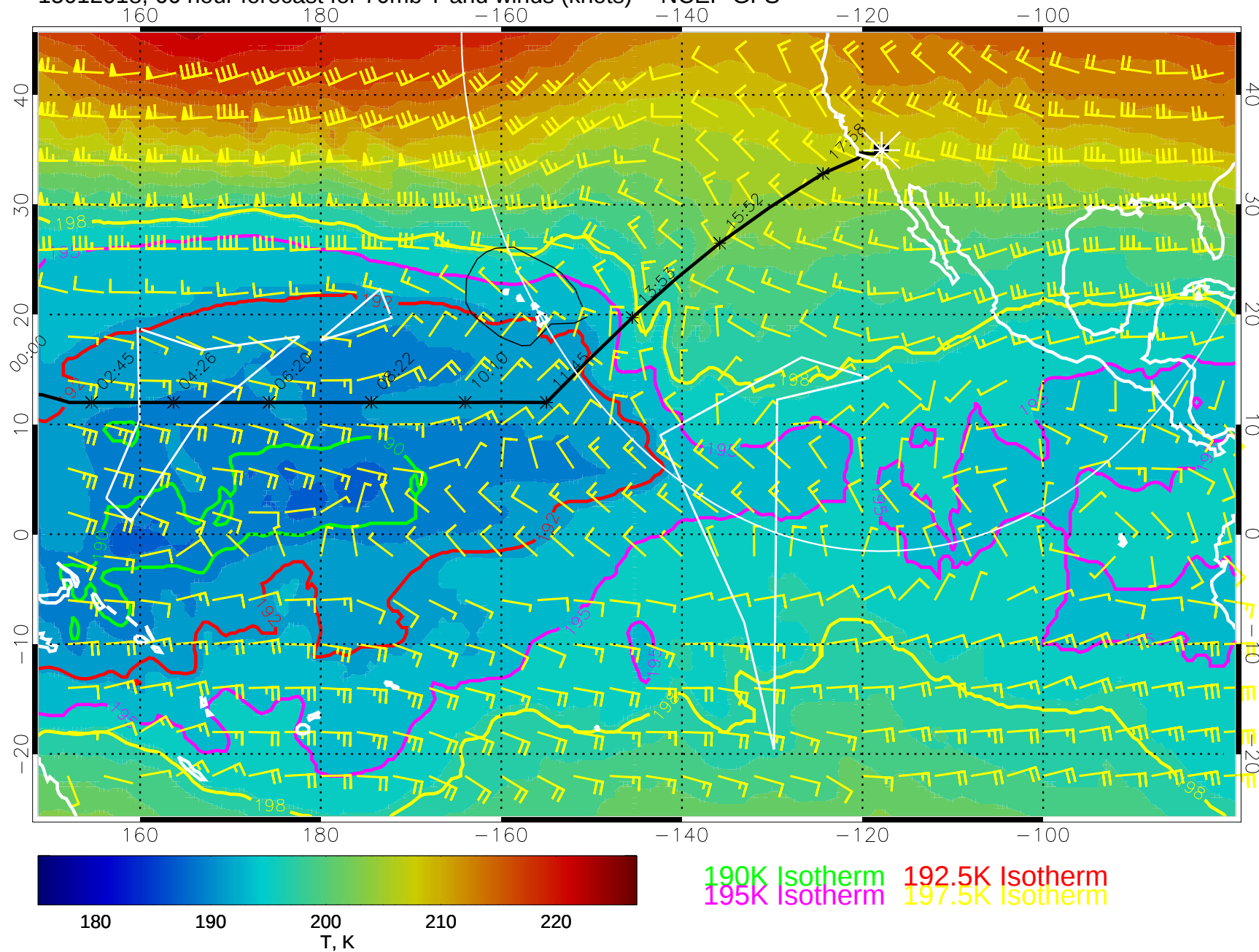
15012018, 66 hour forecast for 70mb T and winds (knots) -- NCEP GFS
