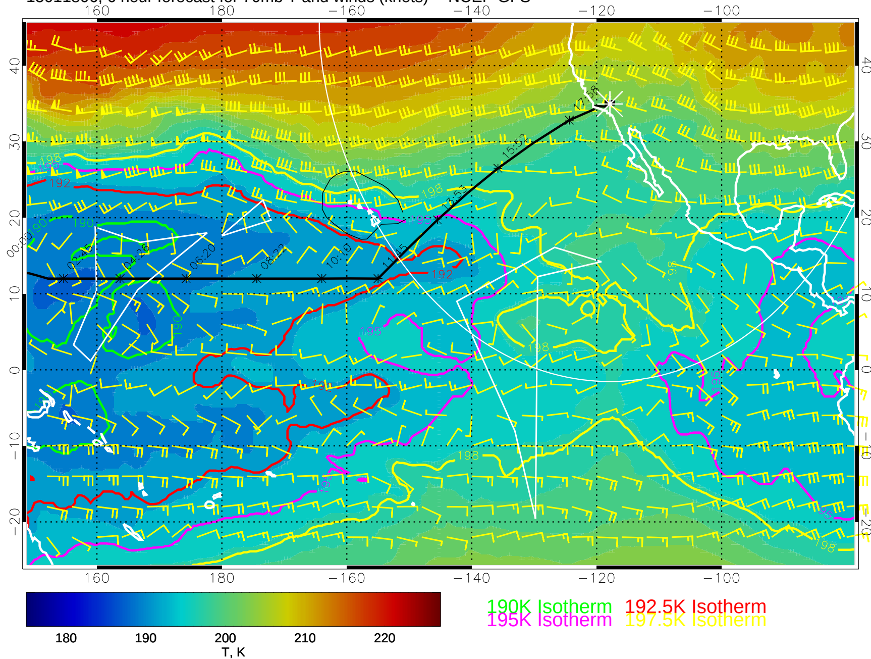
15011806, 6 hour forecast for 70mb T and winds (knots) -- NCEP GFS
