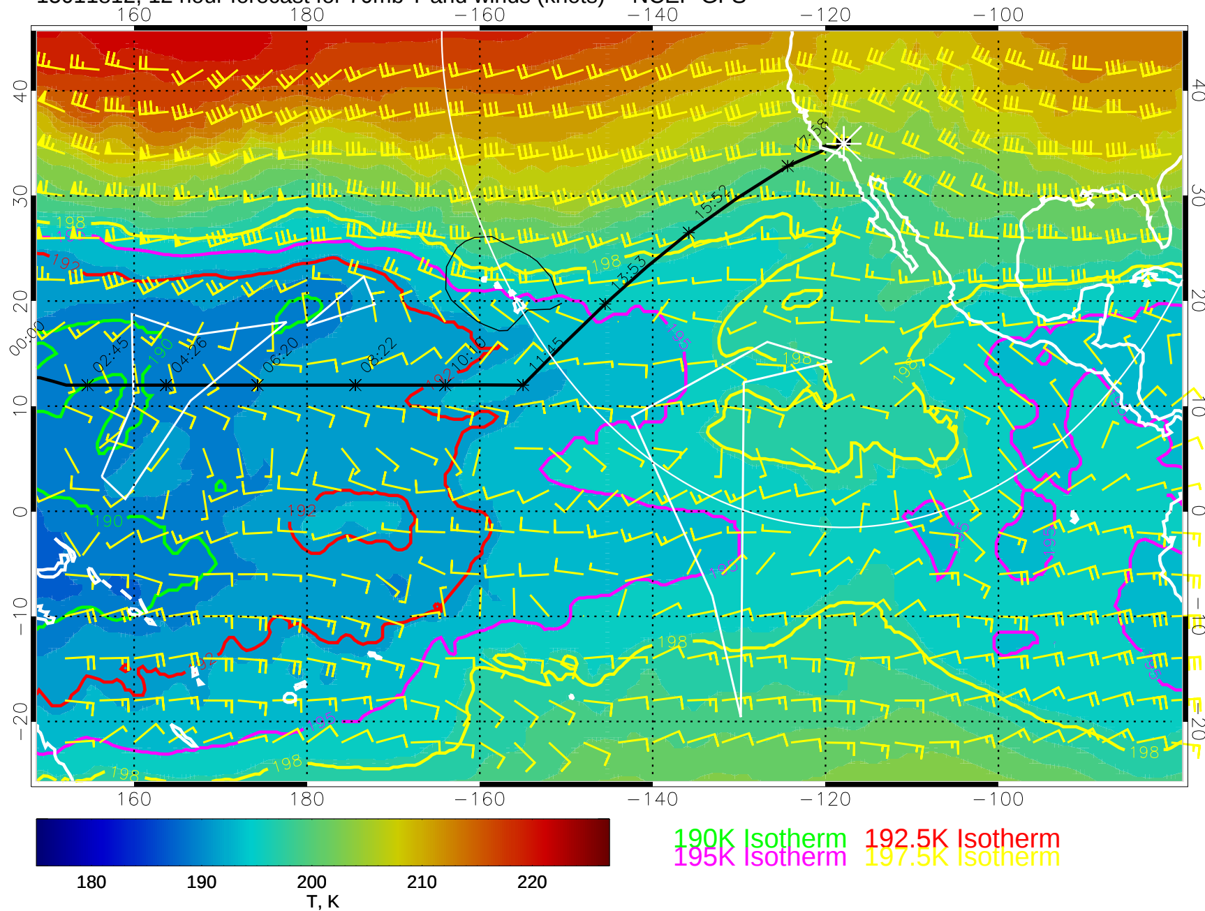
15011812, 12 hour forecast for 70mb T and winds (knots) -- NCEP GFS
