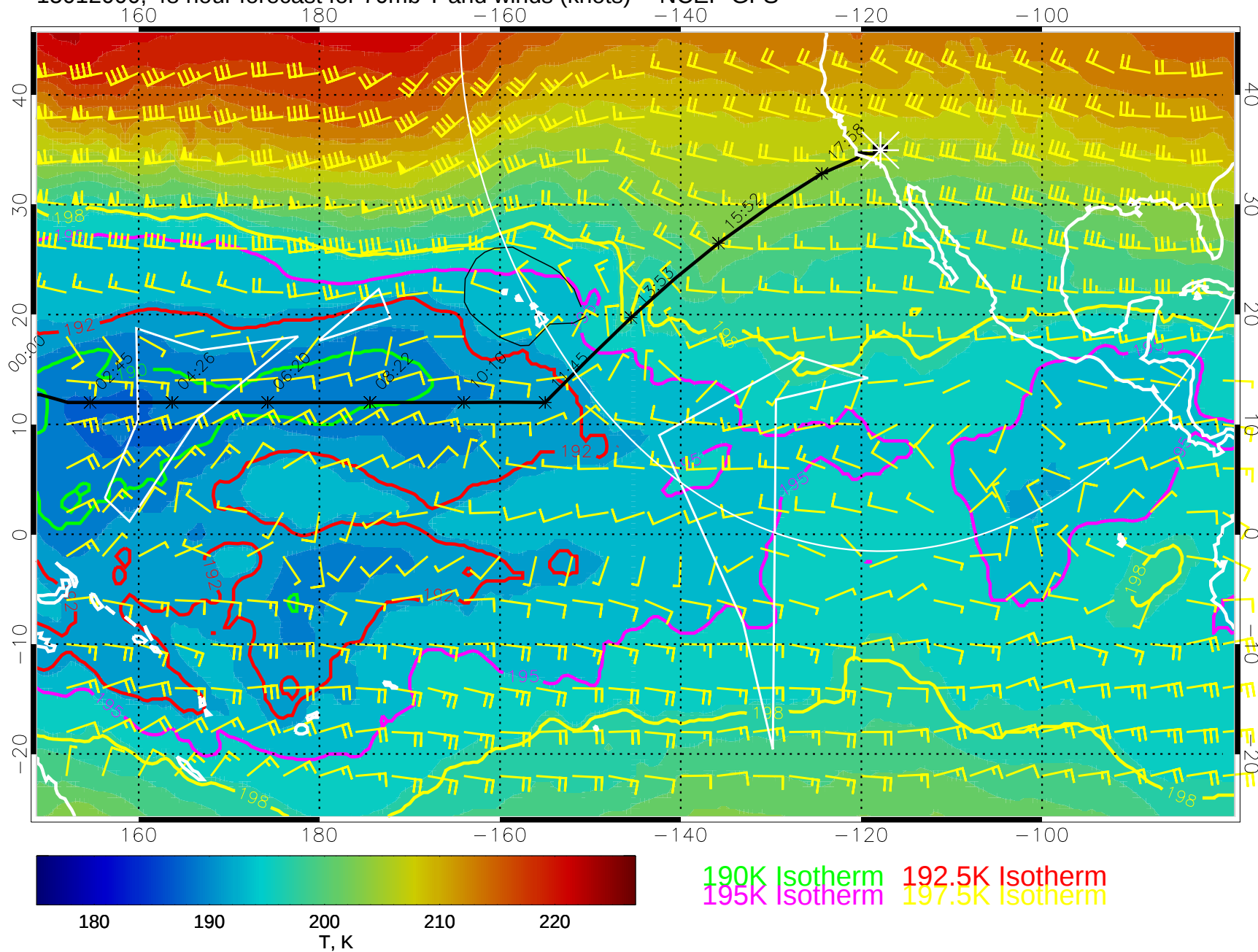
15012000, 48 hour forecast for 70mb T and winds (knots) -- NCEP GFS
