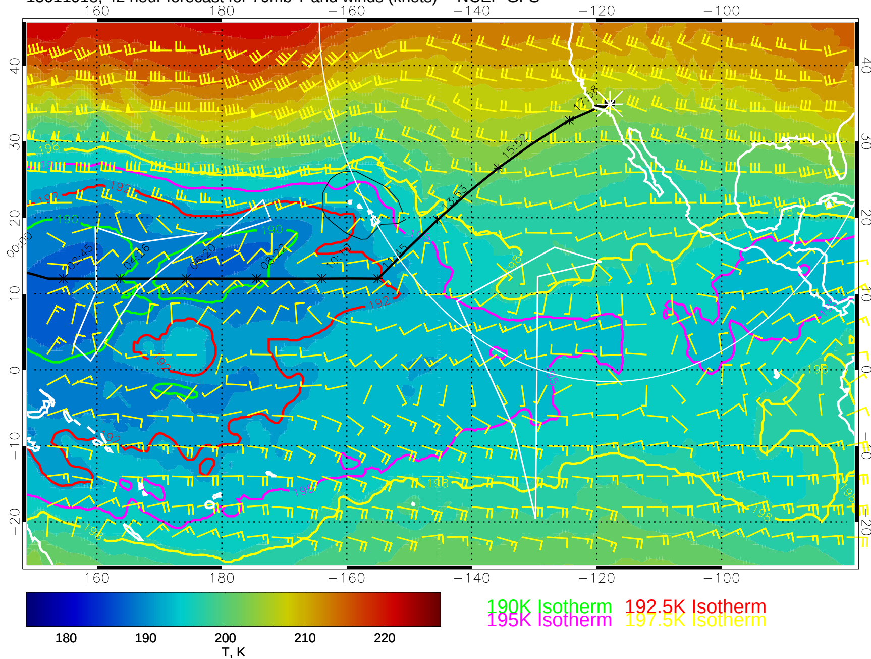
15011918, 42 hour forecast for 70mb T and winds (knots) -- NCEP GFS
