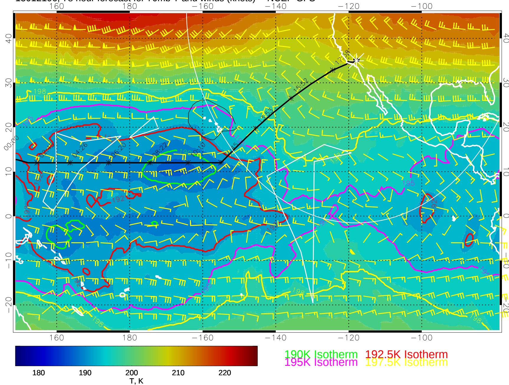
15012106, 78 hour forecast for 70mb T and winds (knots) -- NCEP GFS
