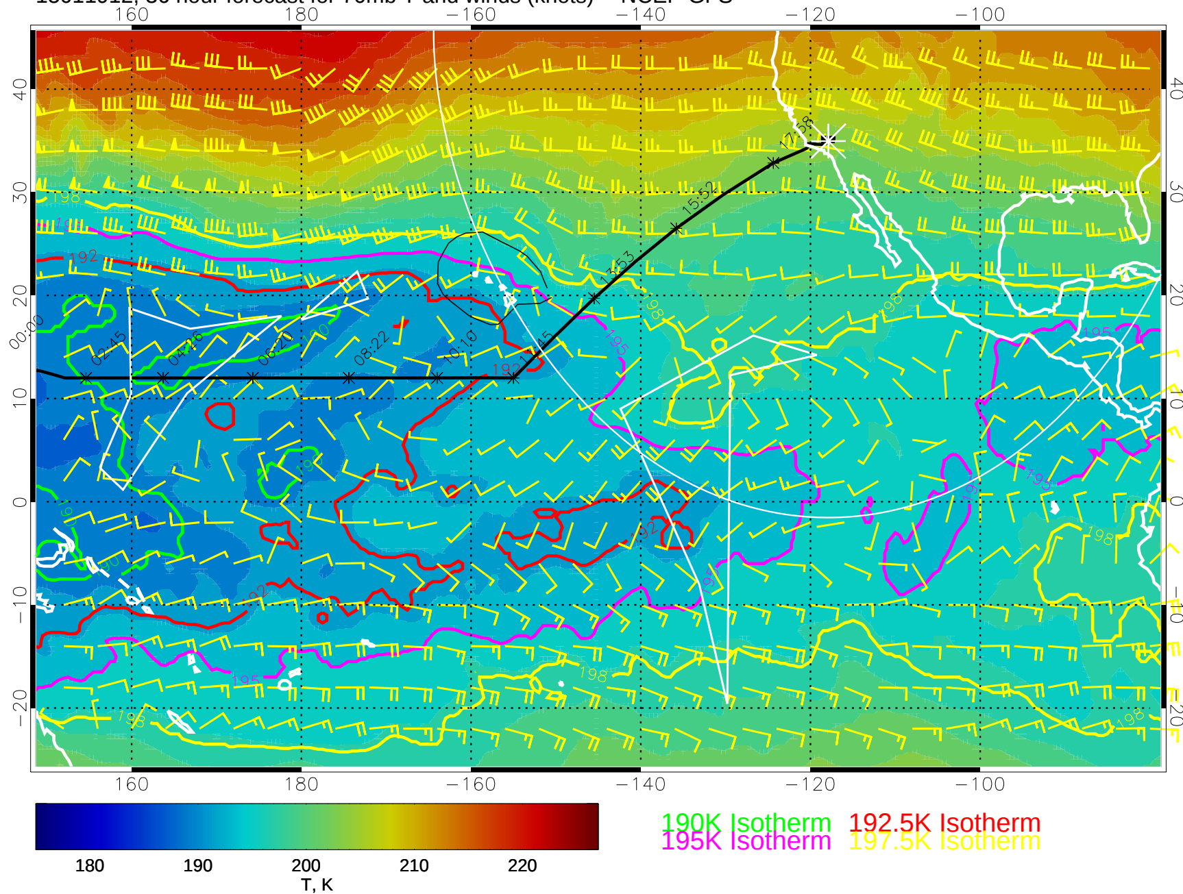
15011912, 36 hour forecast for 70mb T and winds (knots) -- NCEP GFS
