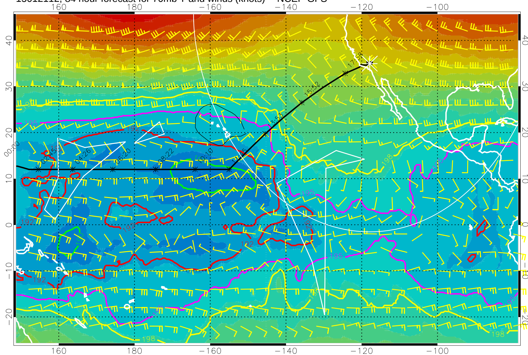
15012112, 84 hour forecast for 70mb T and winds (knots) -- NCEP GFS
