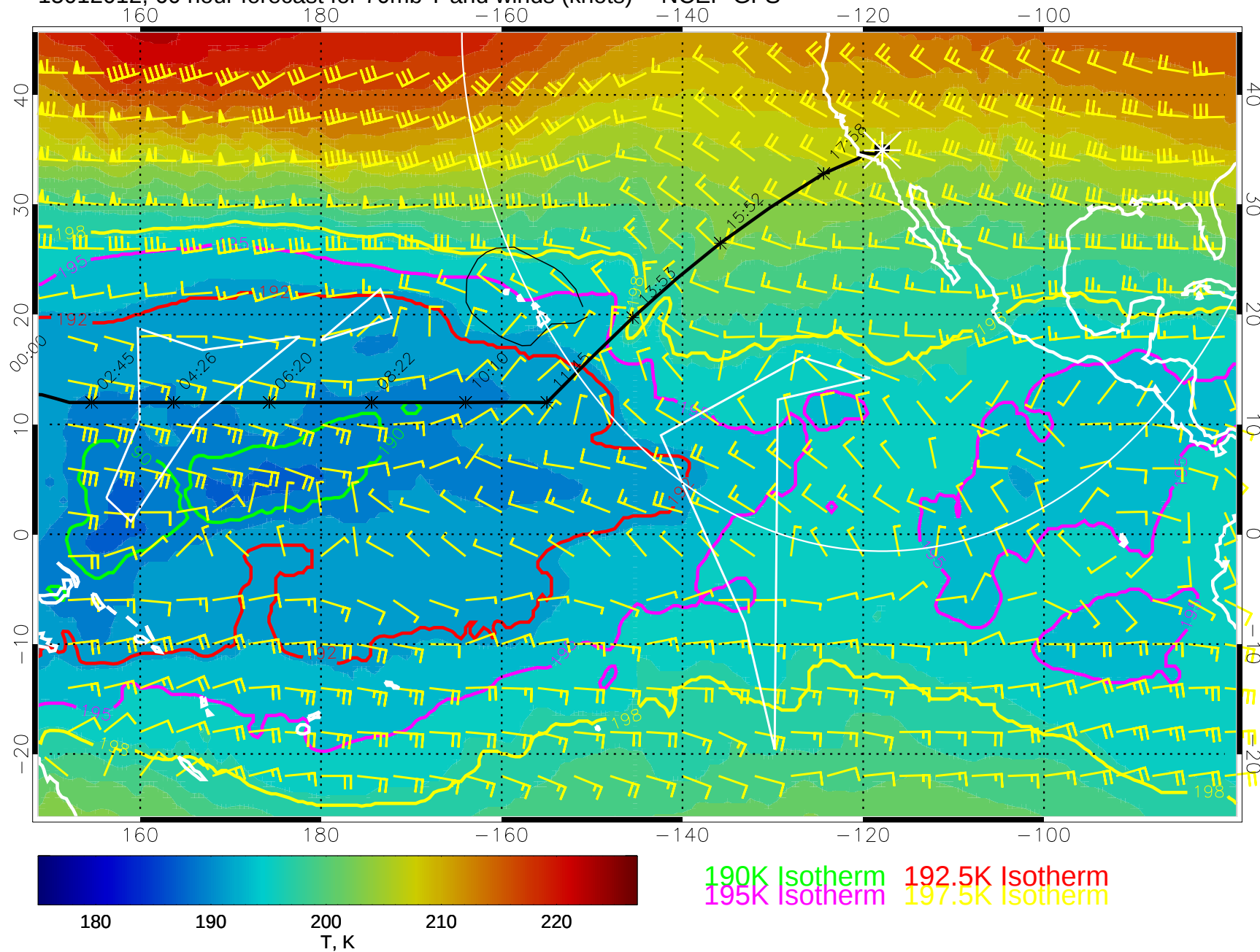
15012012, 60 hour forecast for 70mb T and winds (knots) -- NCEP GFS
