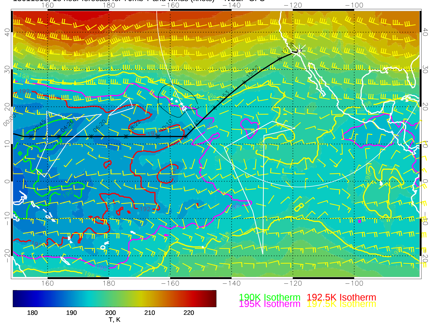
15011818, 18 hour forecast for 70mb T and winds (knots) -- NCEP GFS
