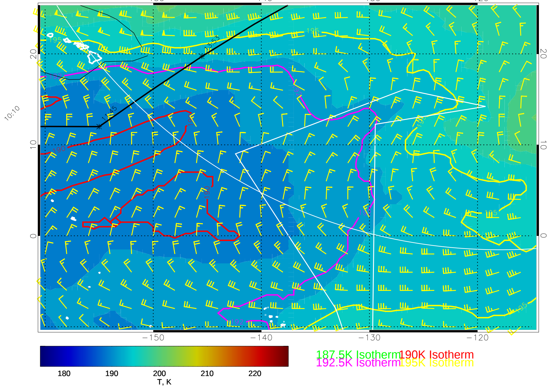
15011818, 18 hour forecast for 100mb T and winds (knots) -- NCEP GFS
