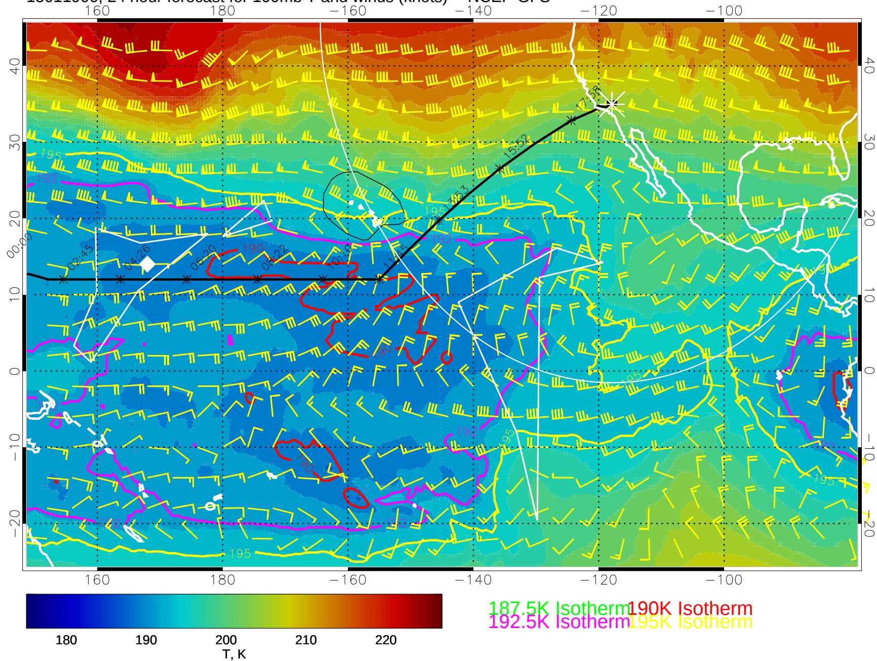
15011900, 24 hour forecast for 100mb T and winds (knots) -- NCEP GFS
