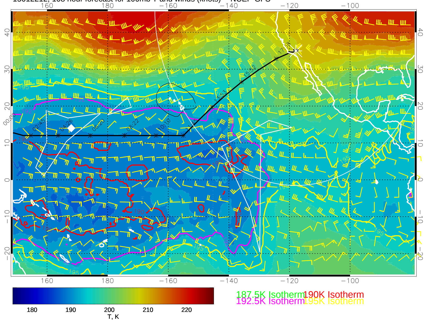
15012212, 108 hour forecast for 100mb T and winds (knots) -- NCEP GFS
