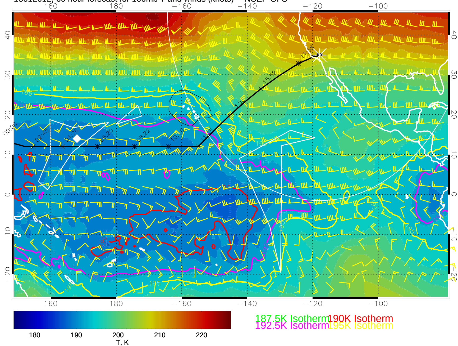
15012012, 60 hour forecast for 100mb T and winds (knots) -- NCEP GFS
