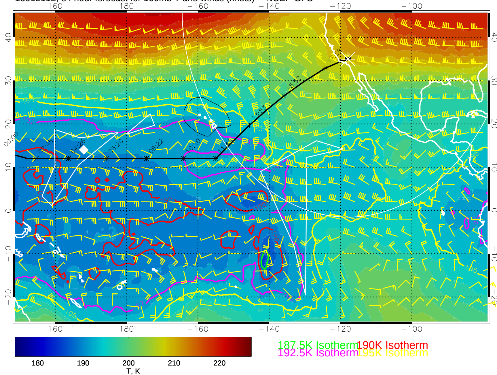
15012112, 84 hour forecast for 100mb T and winds (knots) -- NCEP GFS
