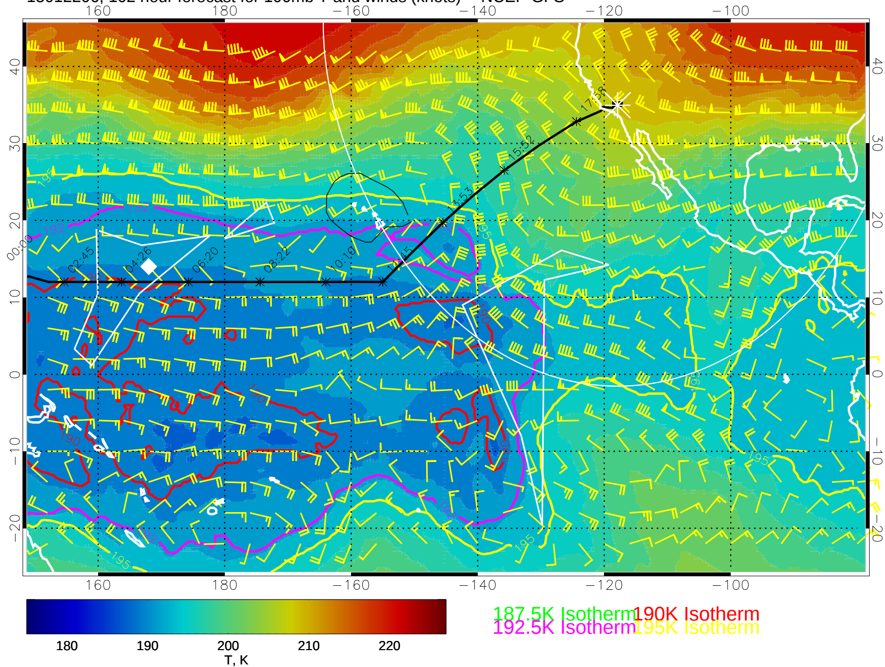
15012206, 102 hour forecast for 100mb T and winds (knots) -- NCEP GFS
