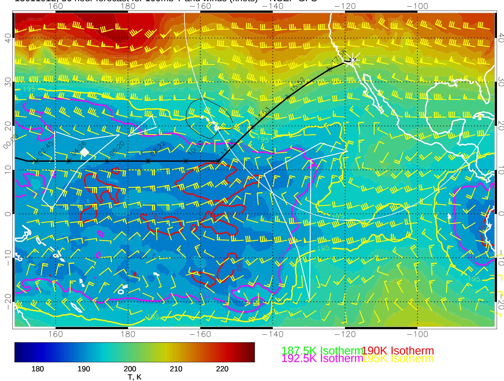
15011912, 36 hour forecast for 100mb T and winds (knots) -- NCEP GFS
