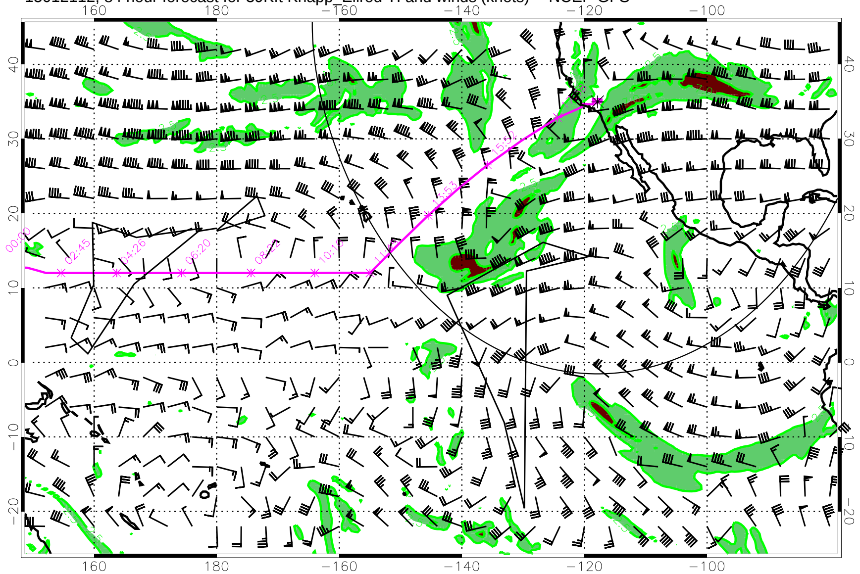
15012112, 84 hour forecast for 39Kft Knapp_Ellrod TI and winds (knots) -- NCEP GFS
