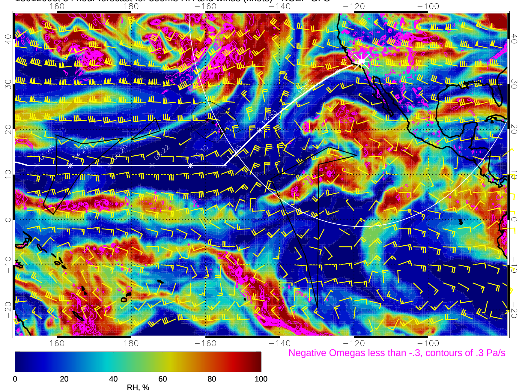
15012006, 54 hour forecast for 500mb RH and winds (knots) - NCEP GFS
