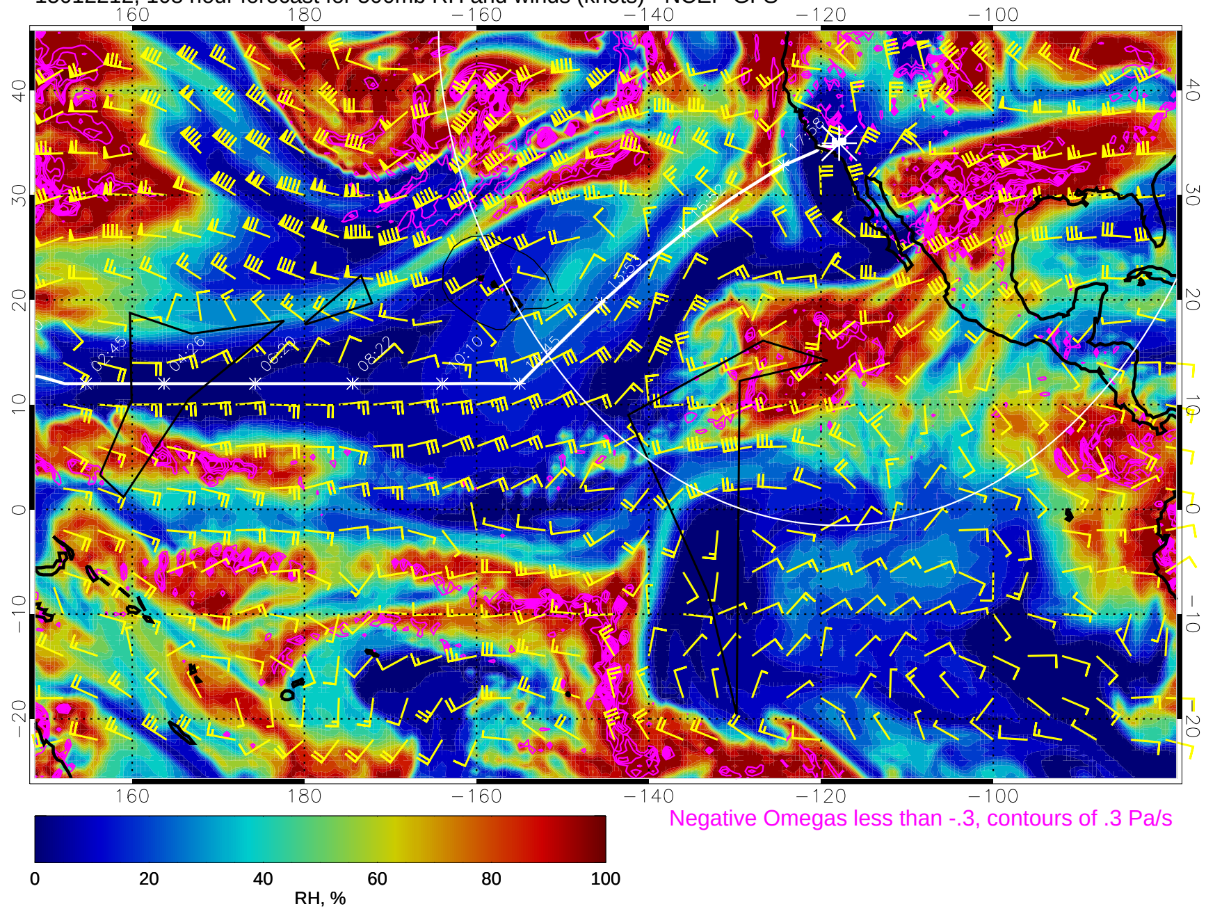
15012212, 108 hour forecast for 500mb RH and winds (knots) - NCEP GFS
