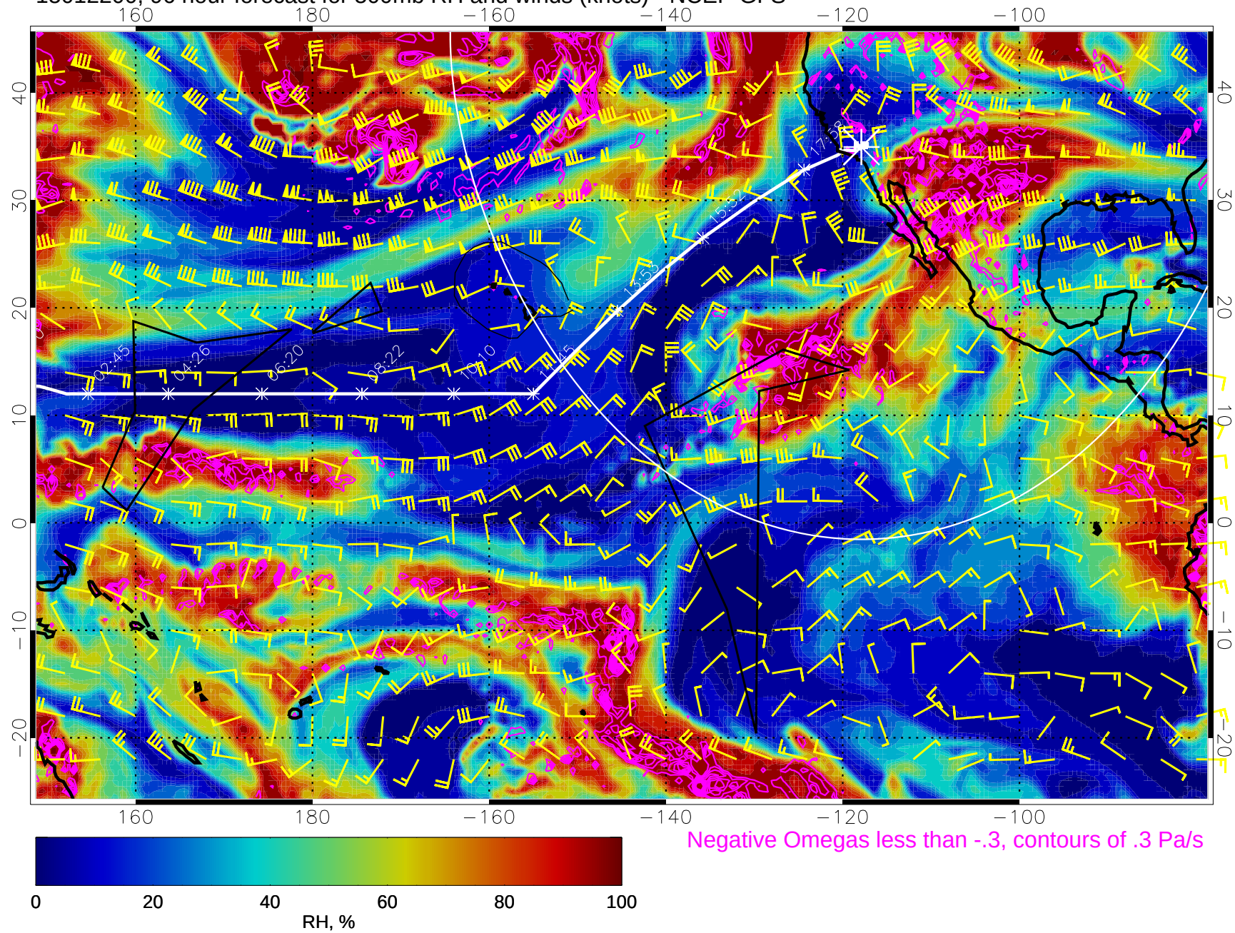
15012200, 96 hour forecast for 500mb RH and winds (knots) - NCEP GFS
