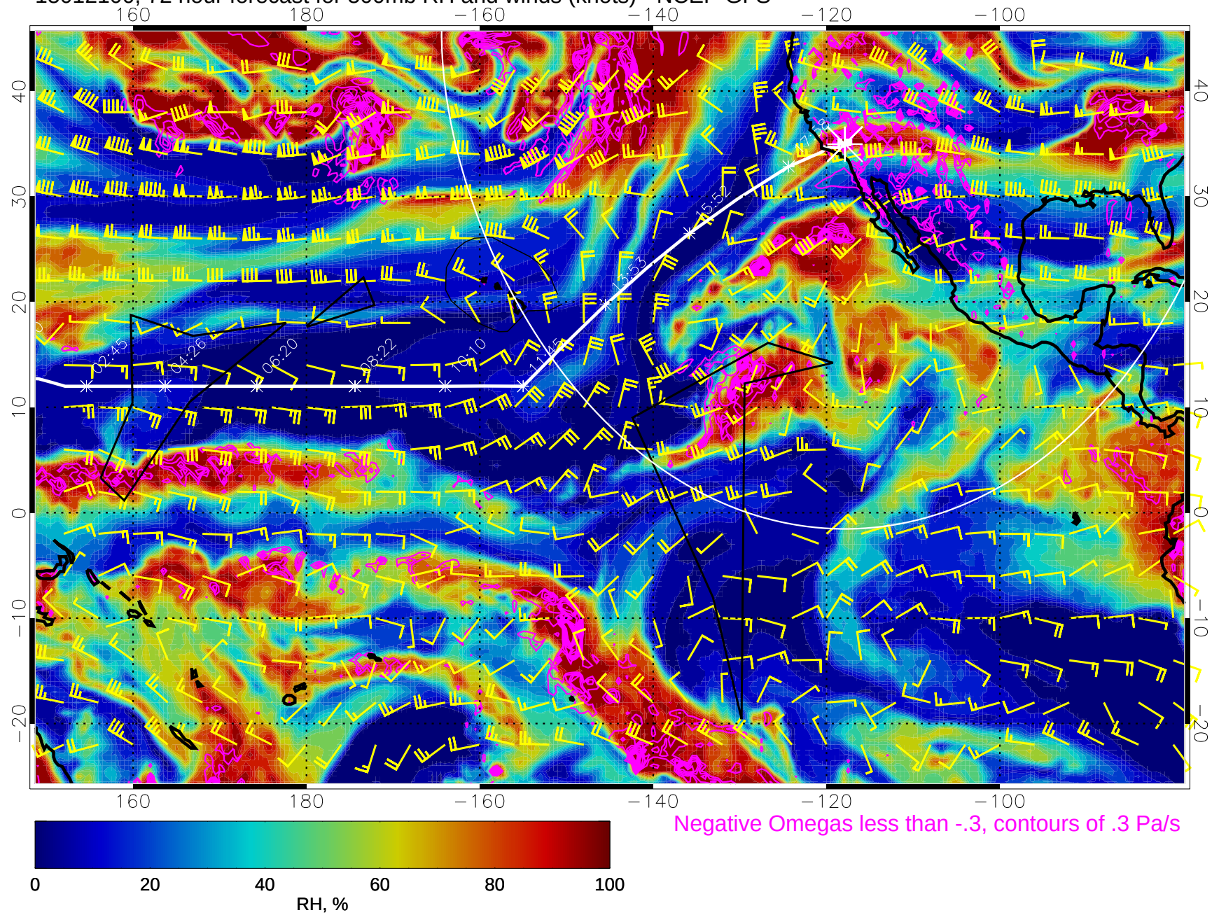
15012100, 72 hour forecast for 500mb RH and winds (knots) - NCEP GFS
