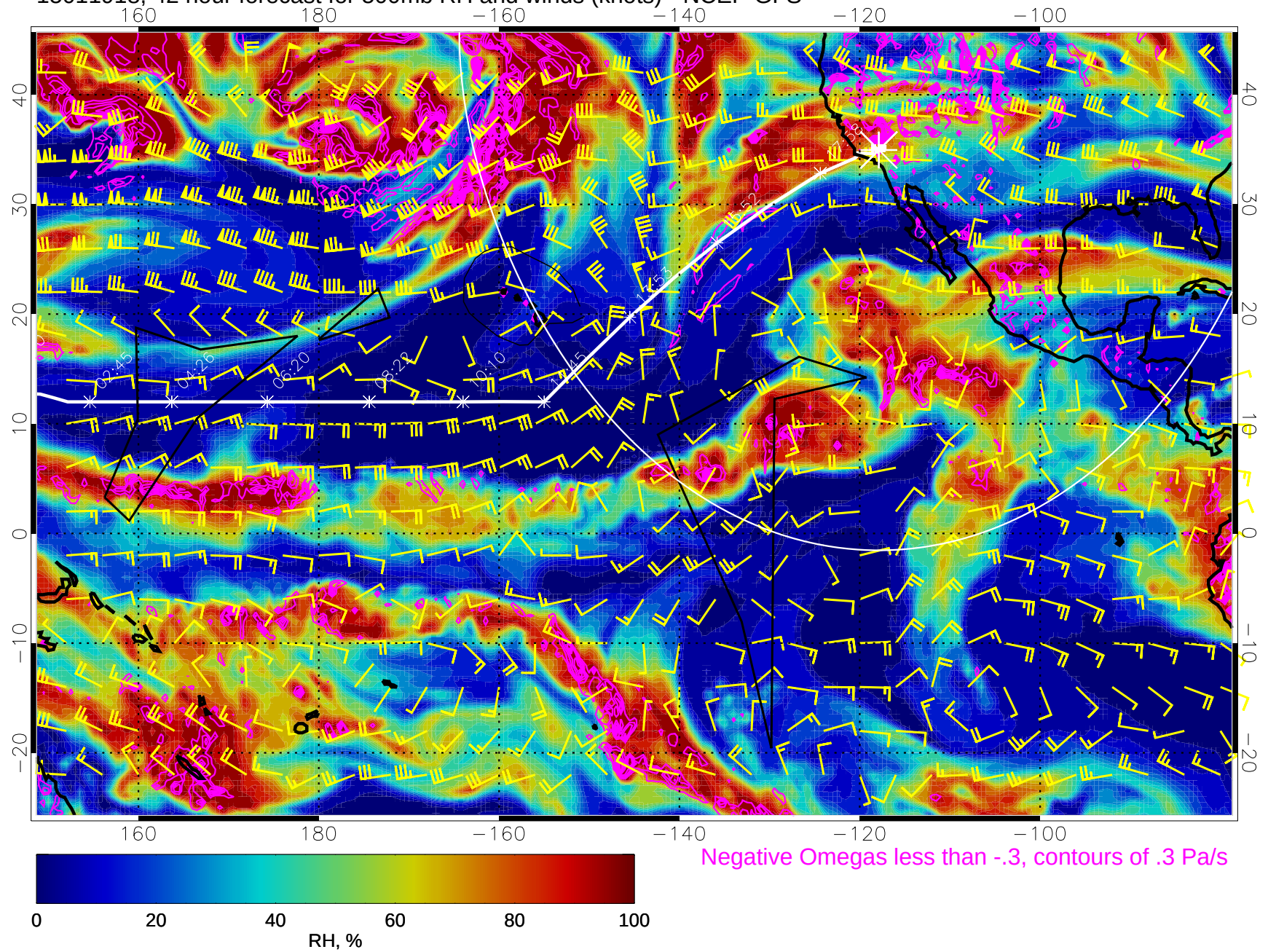
15011918, 42 hour forecast for 500mb RH and winds (knots) - NCEP GFS
