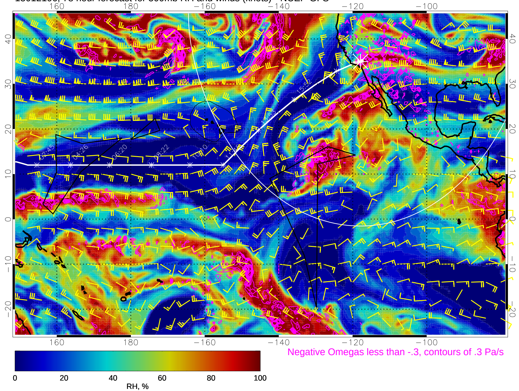
15012106, 78 hour forecast for 500mb RH and winds (knots) - NCEP GFS
