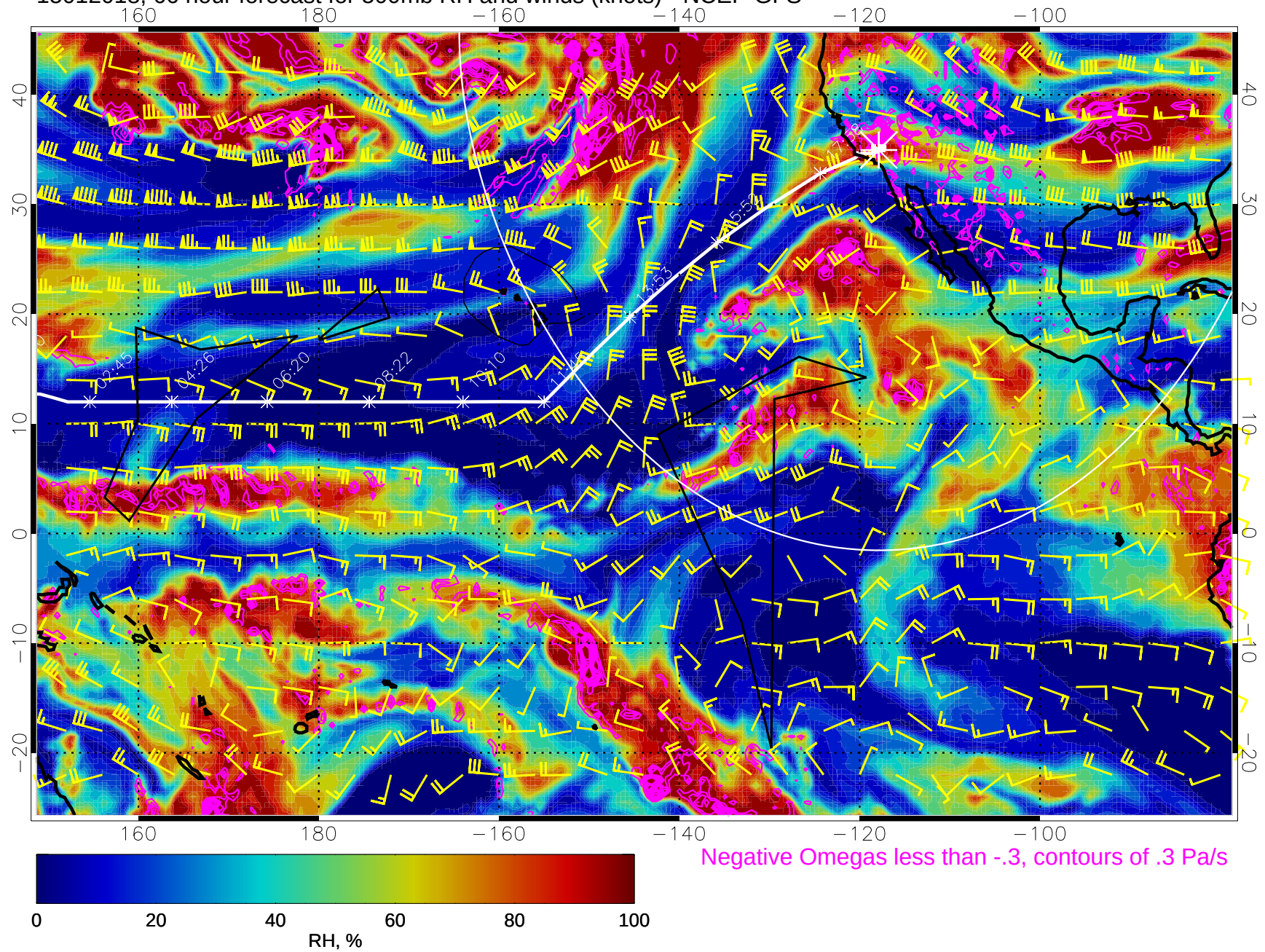
15012018, 66 hour forecast for 500mb RH and winds (knots) - NCEP GFS
