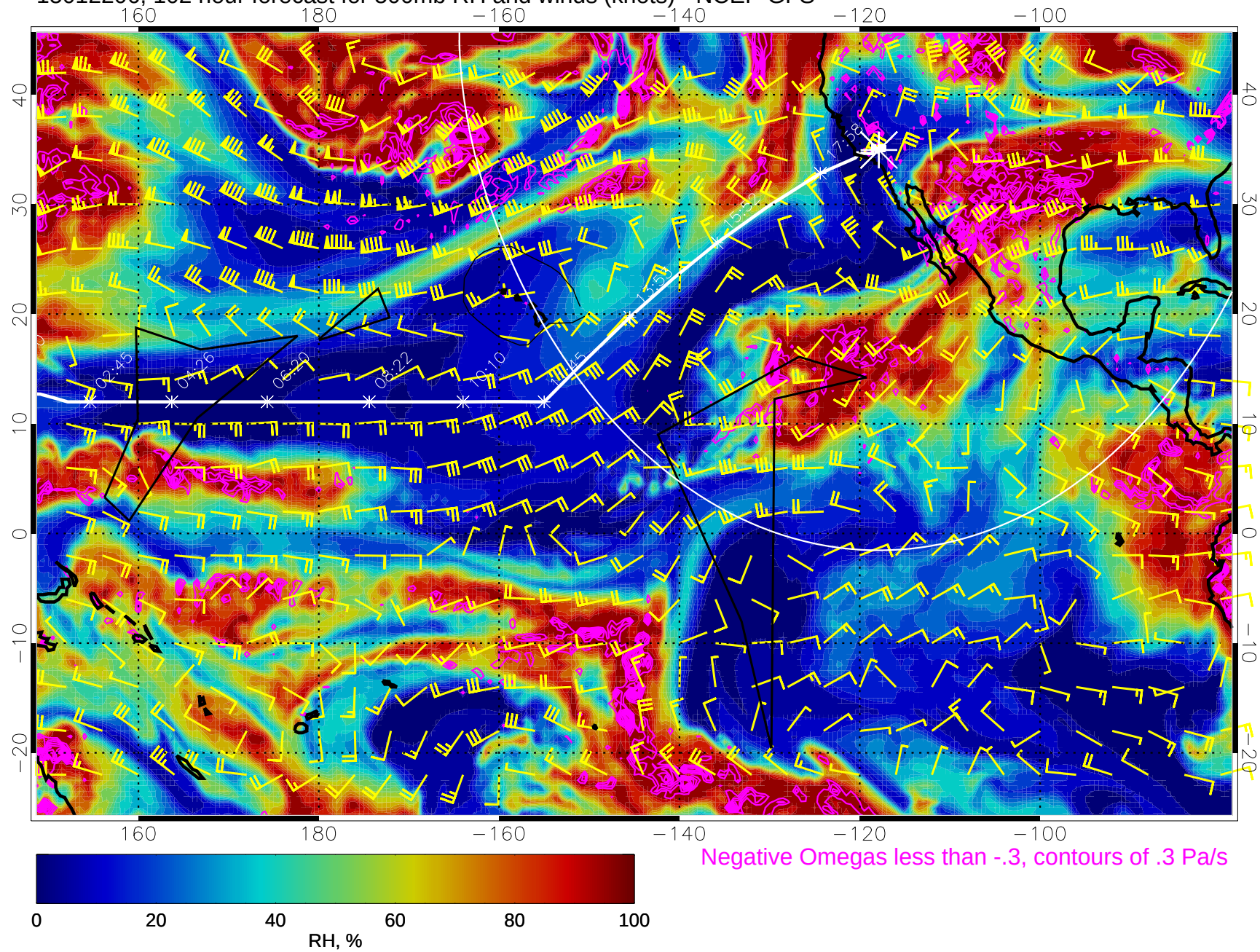
15012206, 102 hour forecast for 500mb RH and winds (knots) - NCEP GFS
