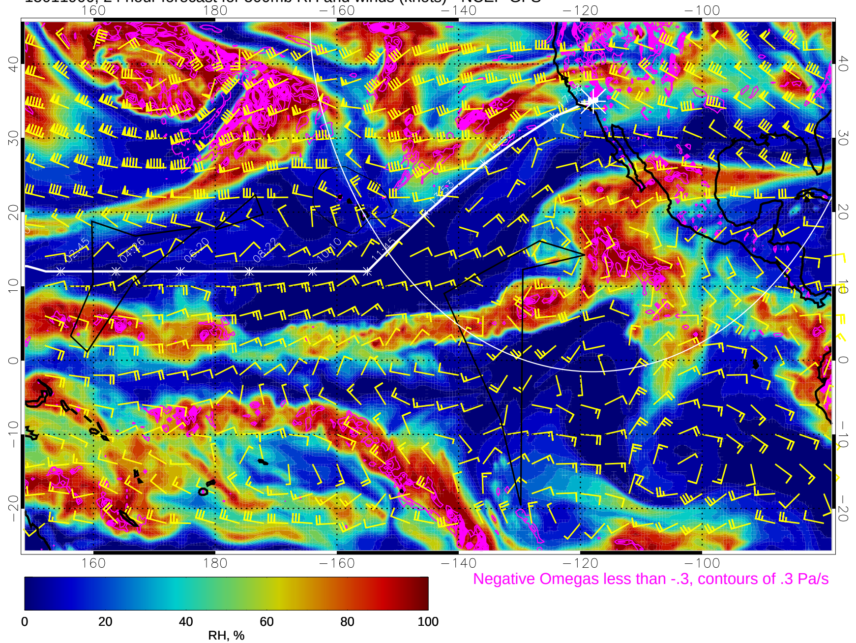
15011900, 24 hour forecast for 500mb RH and winds (knots) - NCEP GFS
