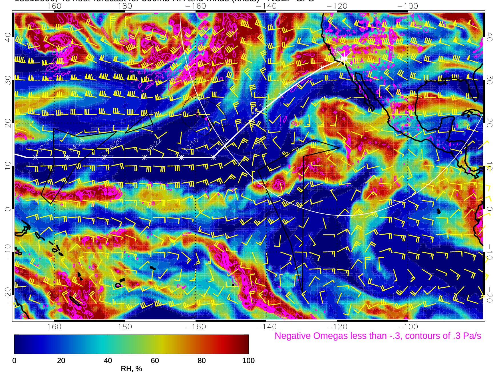
15012000, 48 hour forecast for 500mb RH and winds (knots) - NCEP GFS
