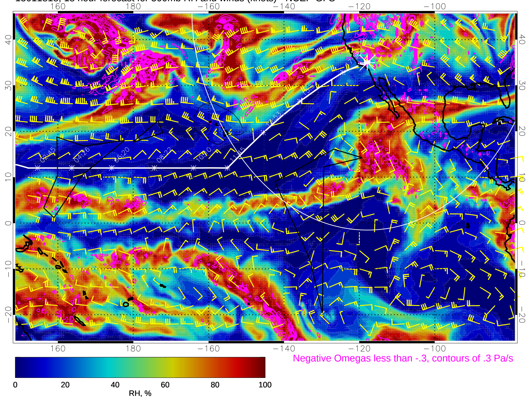
15011818, 18 hour forecast for 500mb RH and winds (knots) - NCEP GFS
