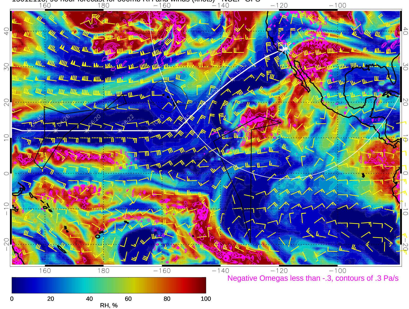
15012118, 90 hour forecast for 500mb RH and winds (knots) - NCEP GFS
