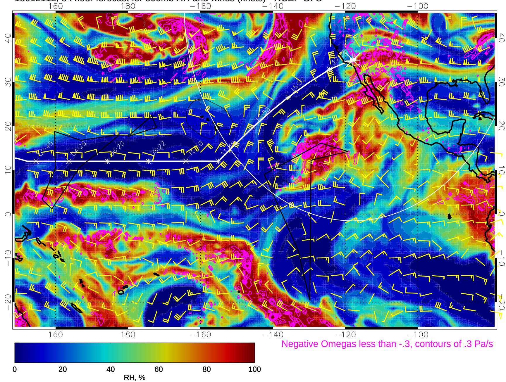
15012112, 84 hour forecast for 500mb RH and winds (knots) - NCEP GFS
