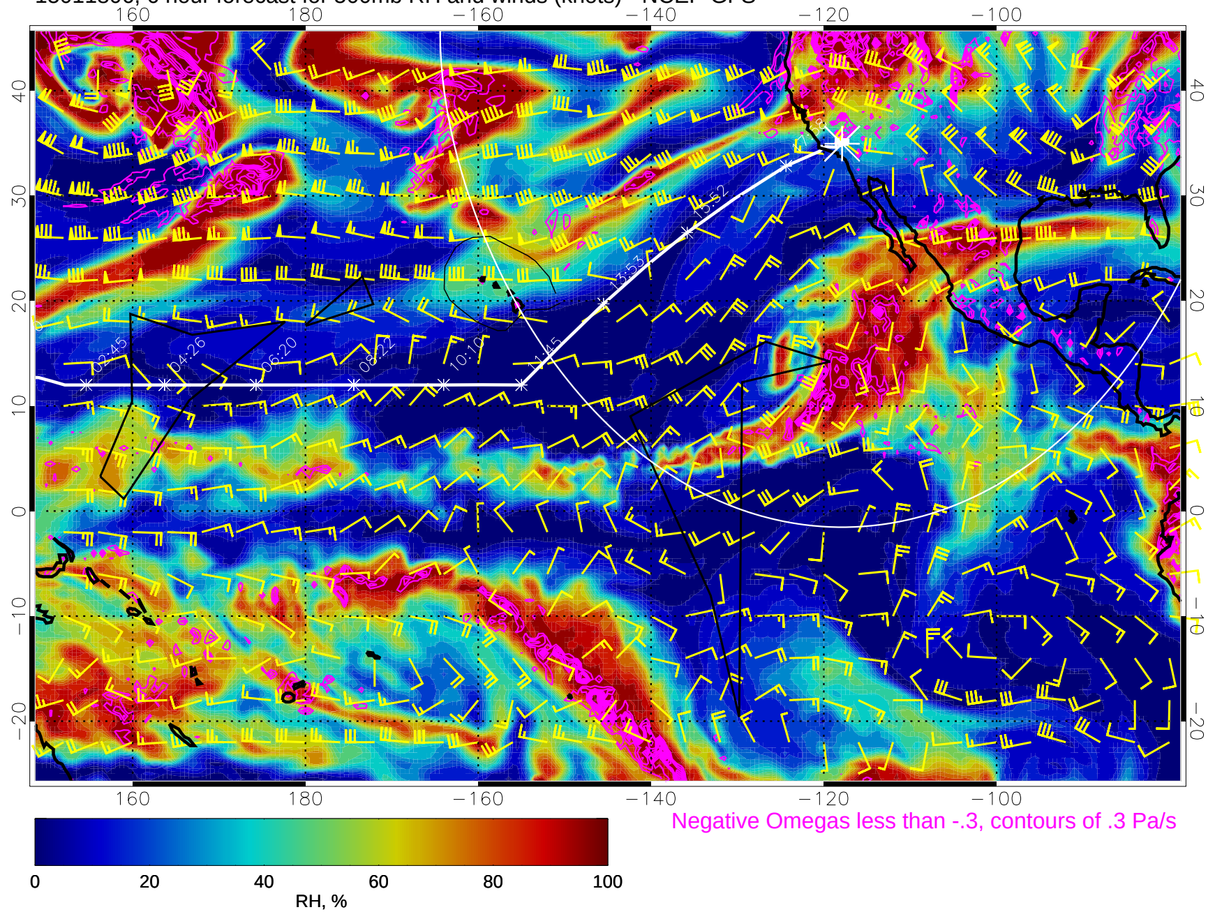
15011806, 6 hour forecast for 500mb RH and winds (knots) - NCEP GFS
