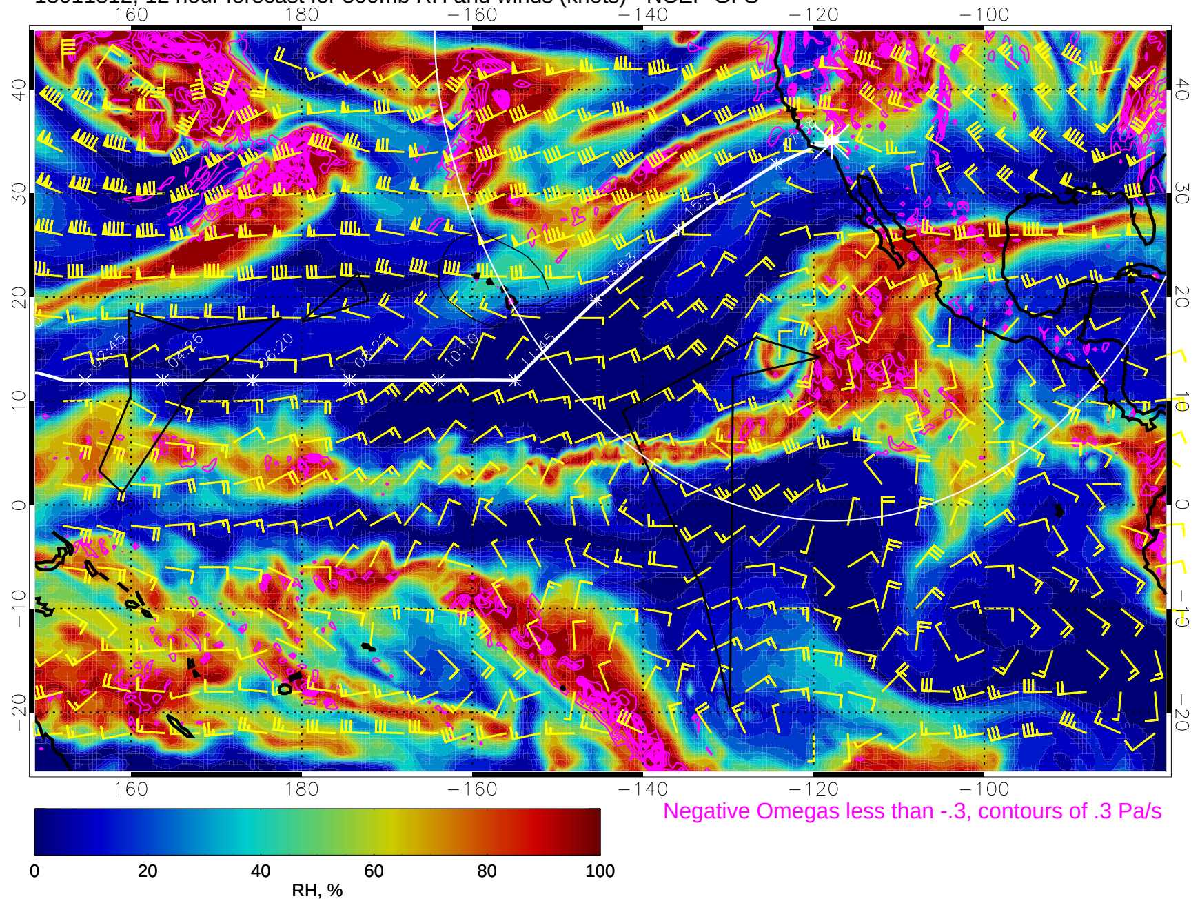
15011812, 12 hour forecast for 500mb RH and winds (knots) - NCEP GFS
