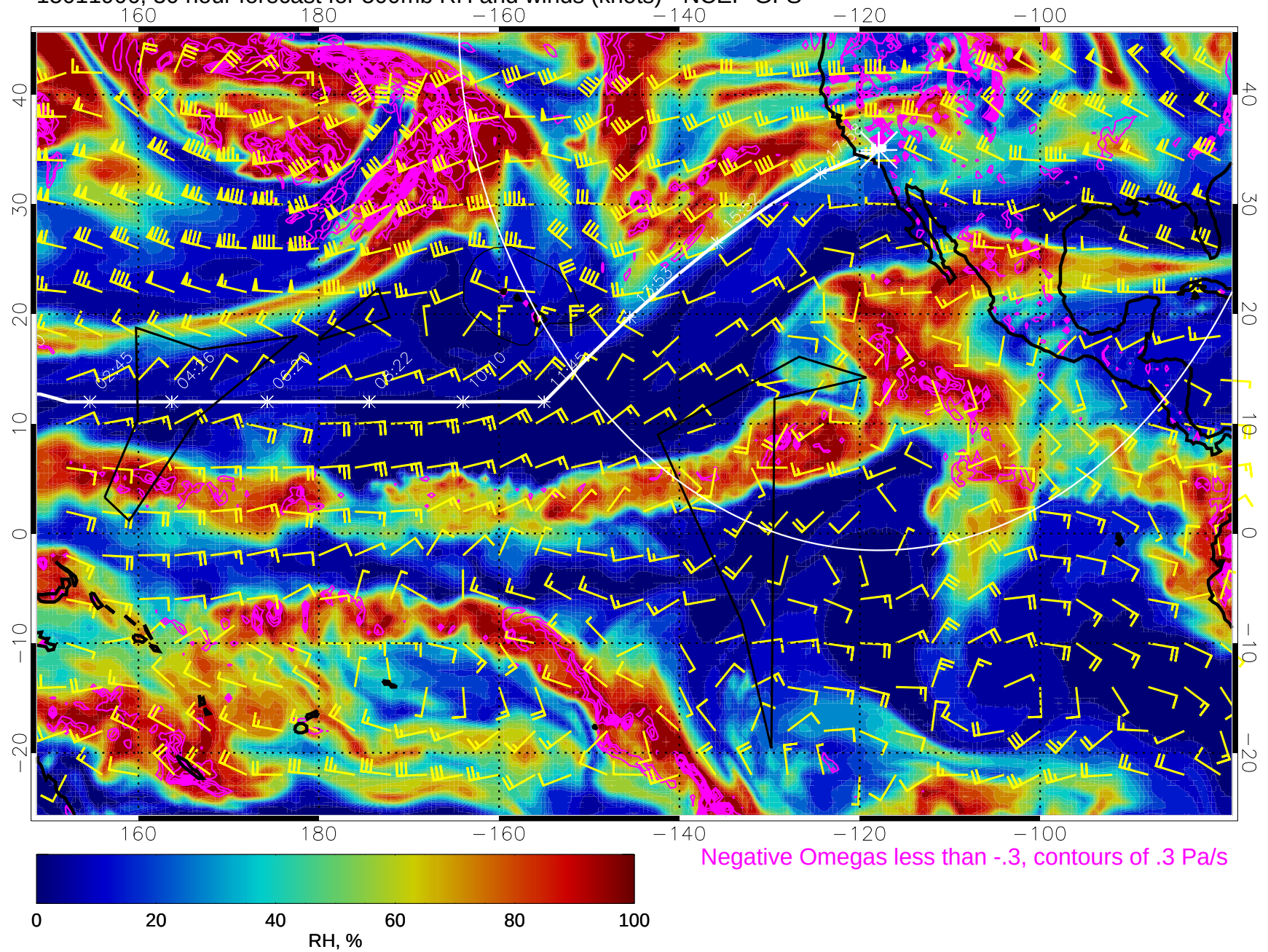
15011906, 30 hour forecast for 500mb RH and winds (knots) - NCEP GFS
