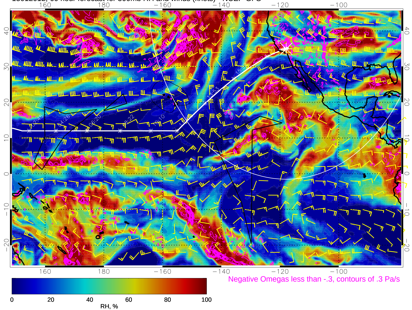
15012012, 60 hour forecast for 500mb RH and winds (knots) - NCEP GFS
