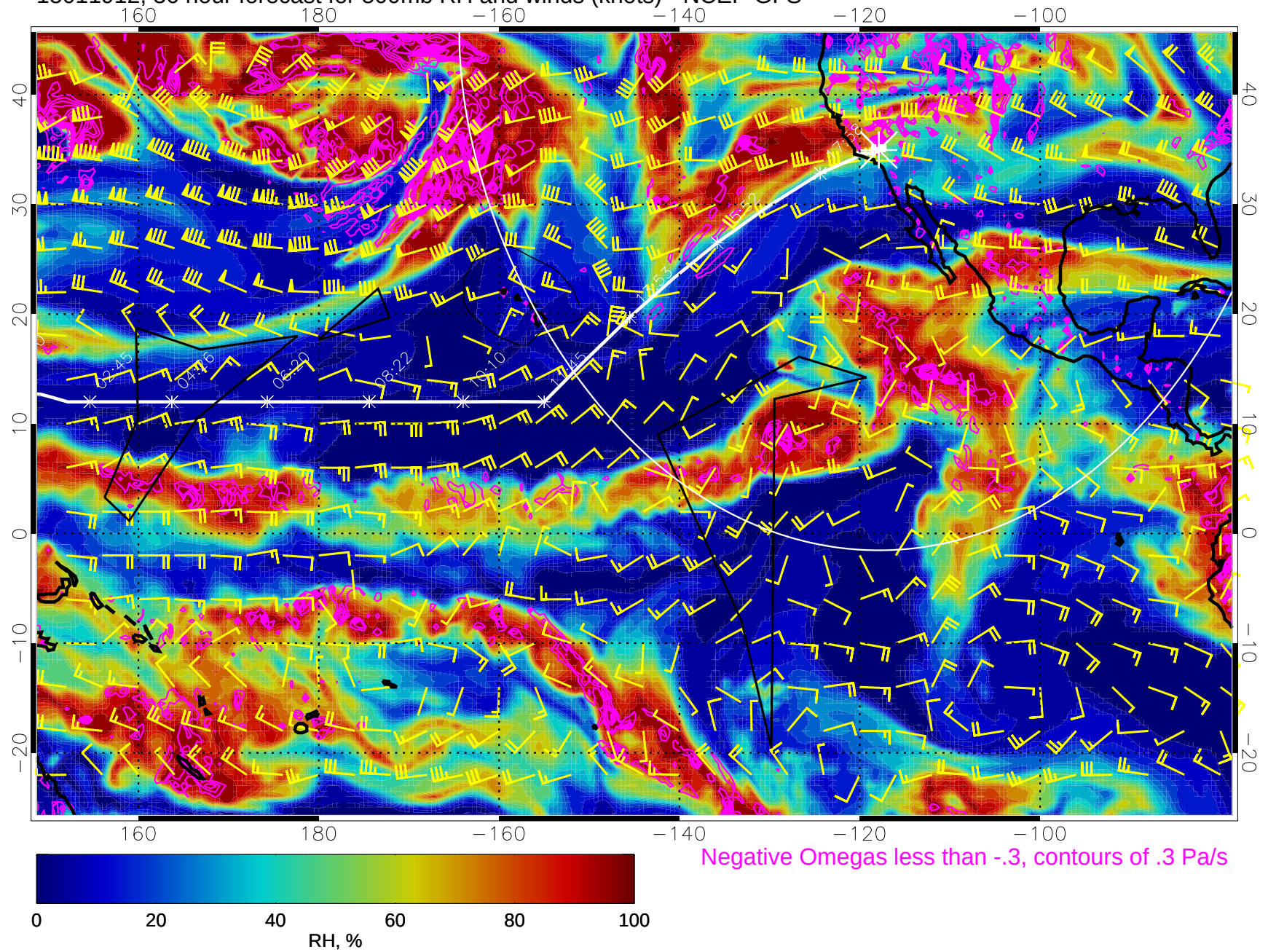
15011912, 36 hour forecast for 500mb RH and winds (knots) - NCEP GFS
