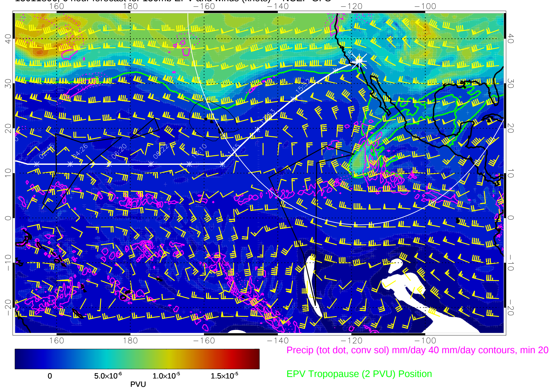
15011806, 6 hour forecast for 150mb EPV and winds (knots) -- NCEP GFS
