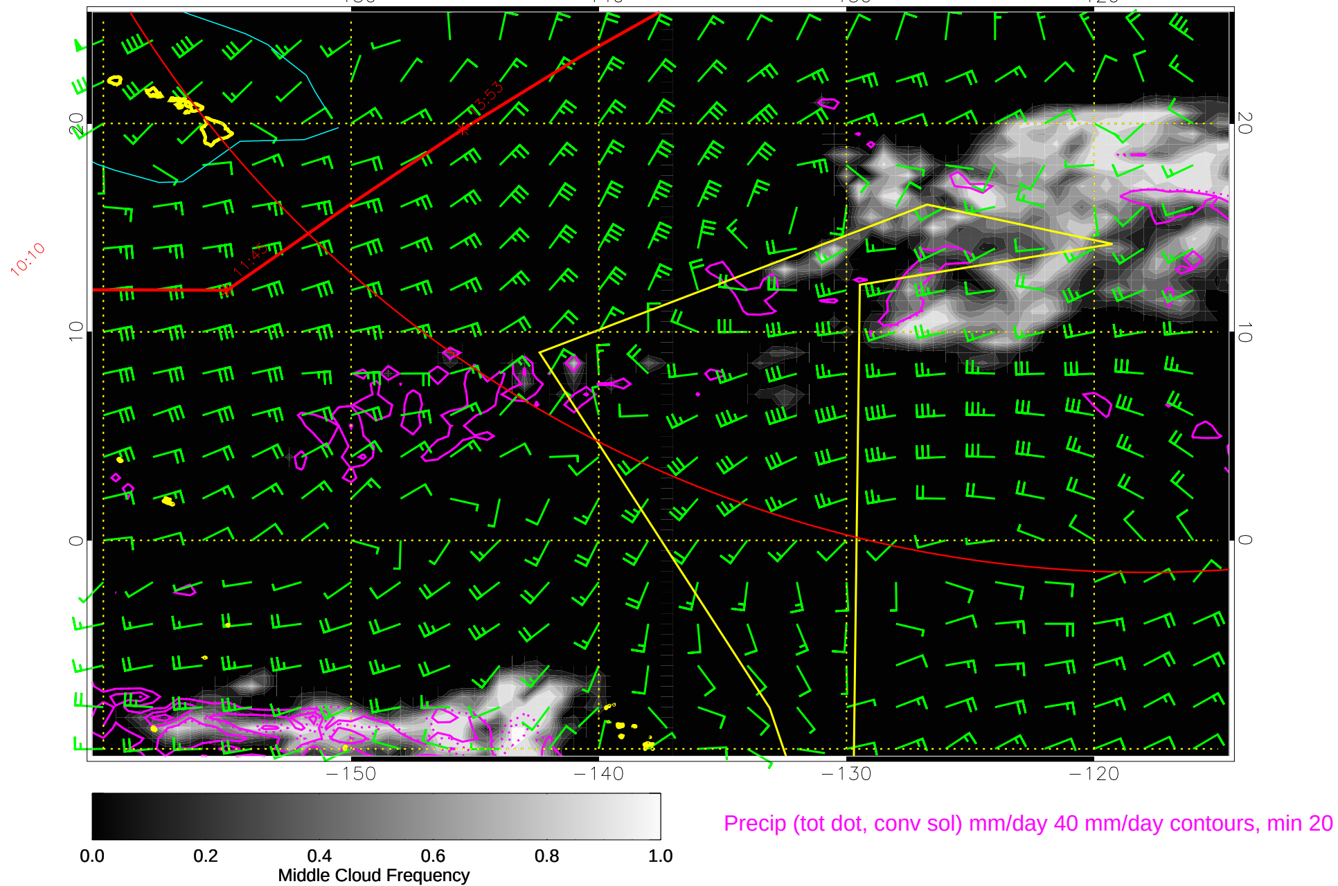
15012218, 114 hour forecast for 500mb winds (knots) and Middle Cloud Frequency -- NCEP GFS
