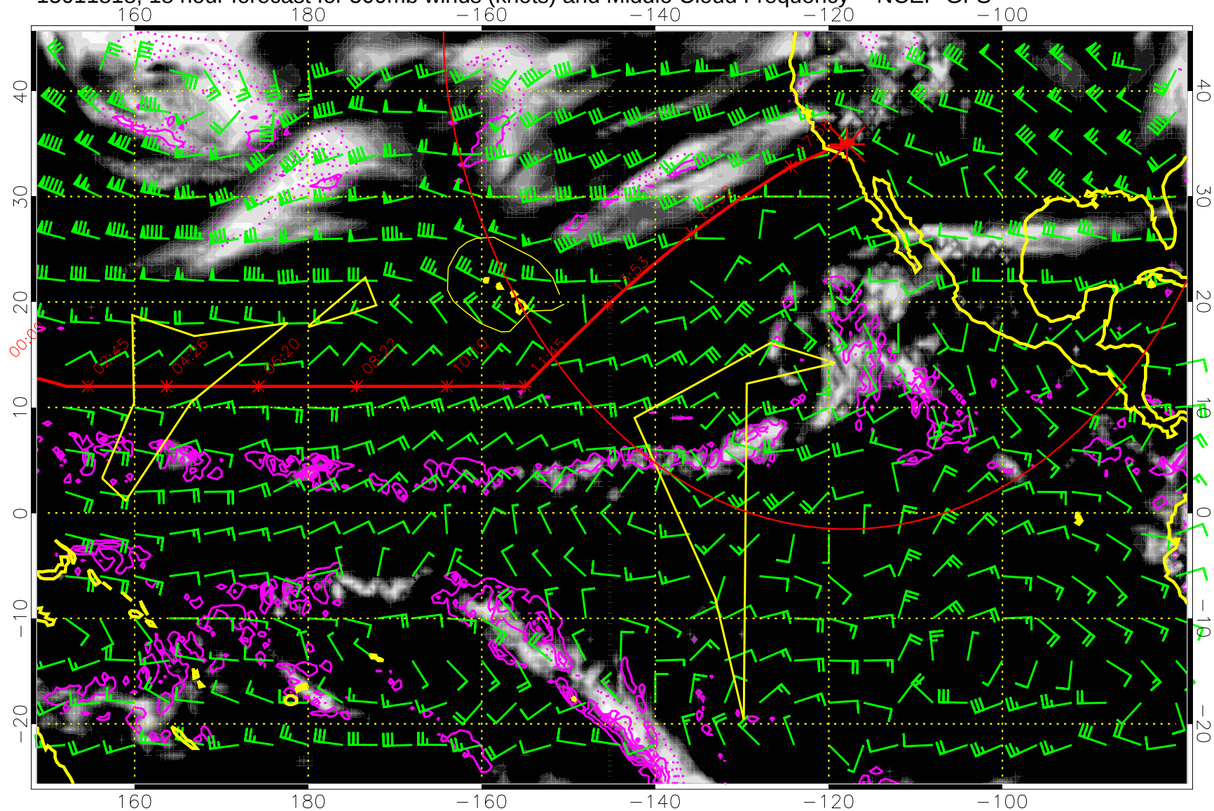
15011818, 18 hour forecast for 500mb winds (knots) and Middle Cloud Frequency -- NCEP GFS
