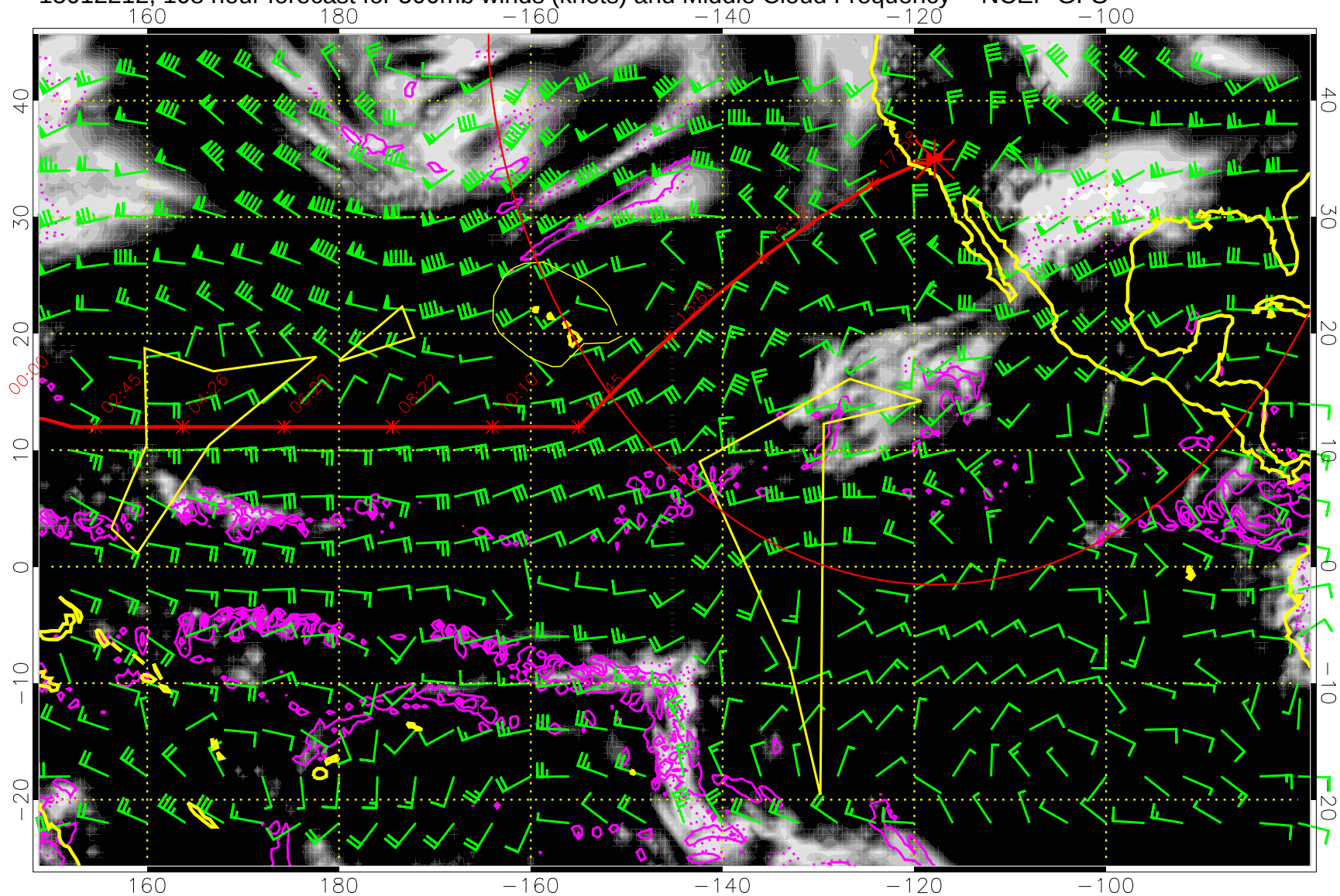
15012212, 108 hour forecast for 500mb winds (knots) and Middle Cloud Frequency -- NCEP GFS
