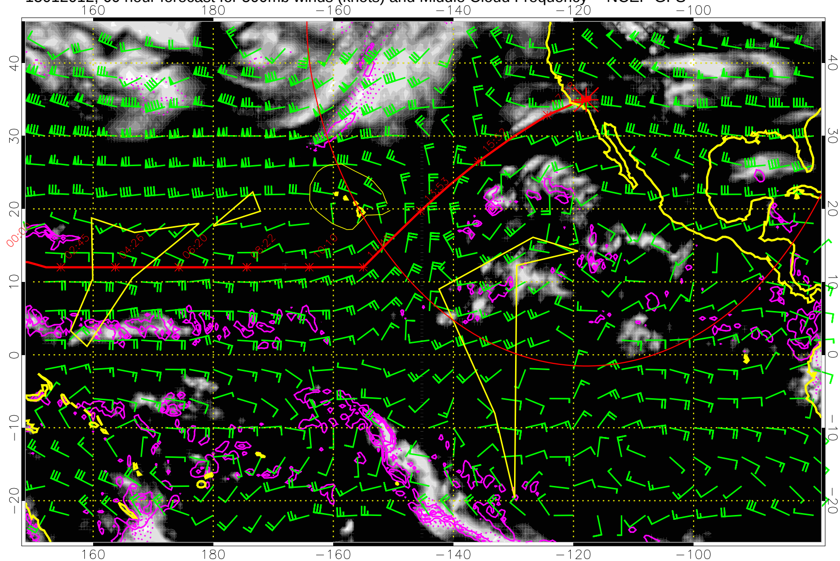
15012012, 60 hour forecast for 500mb winds (knots) and Middle Cloud Frequency -- NCEP GFS
