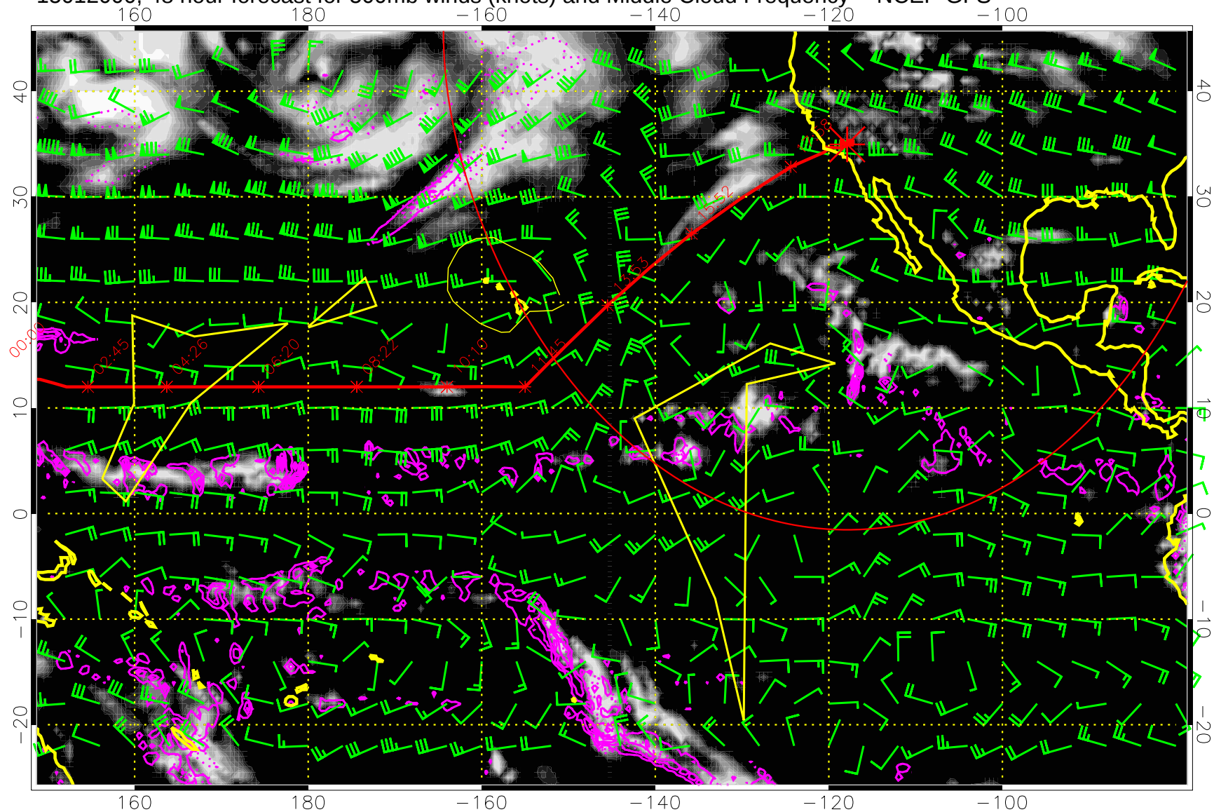
15012000, 48 hour forecast for 500mb winds (knots) and Middle Cloud Frequency -- NCEP GFS
