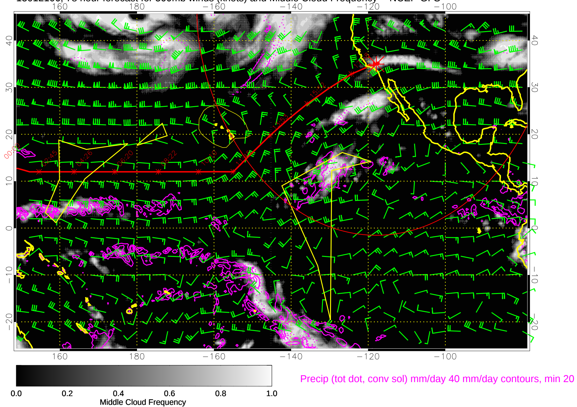
15012106, 78 hour forecast for 500mb winds (knots) and Middle Cloud Frequency -- NCEP GFS
