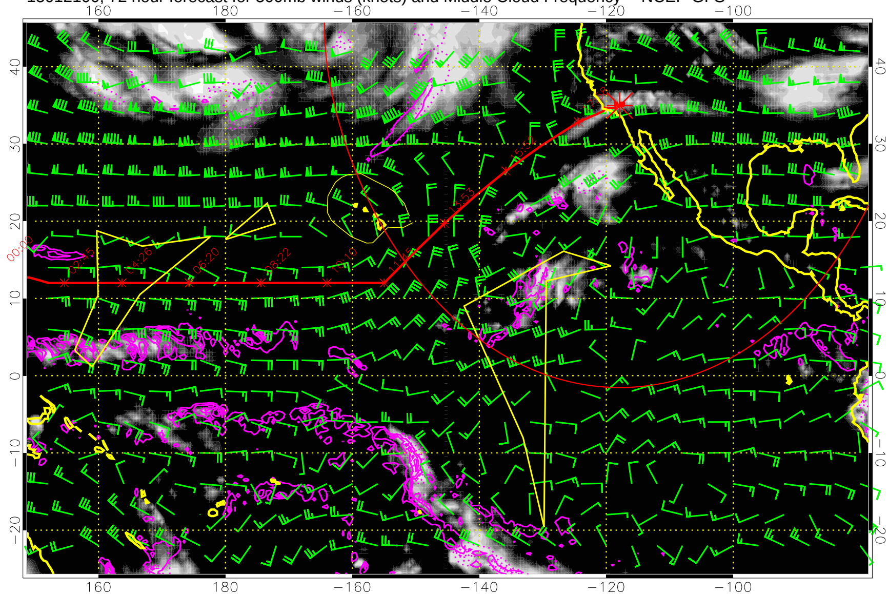
15012100, 72 hour forecast for 500mb winds (knots) and Middle Cloud Frequency -- NCEP GFS
