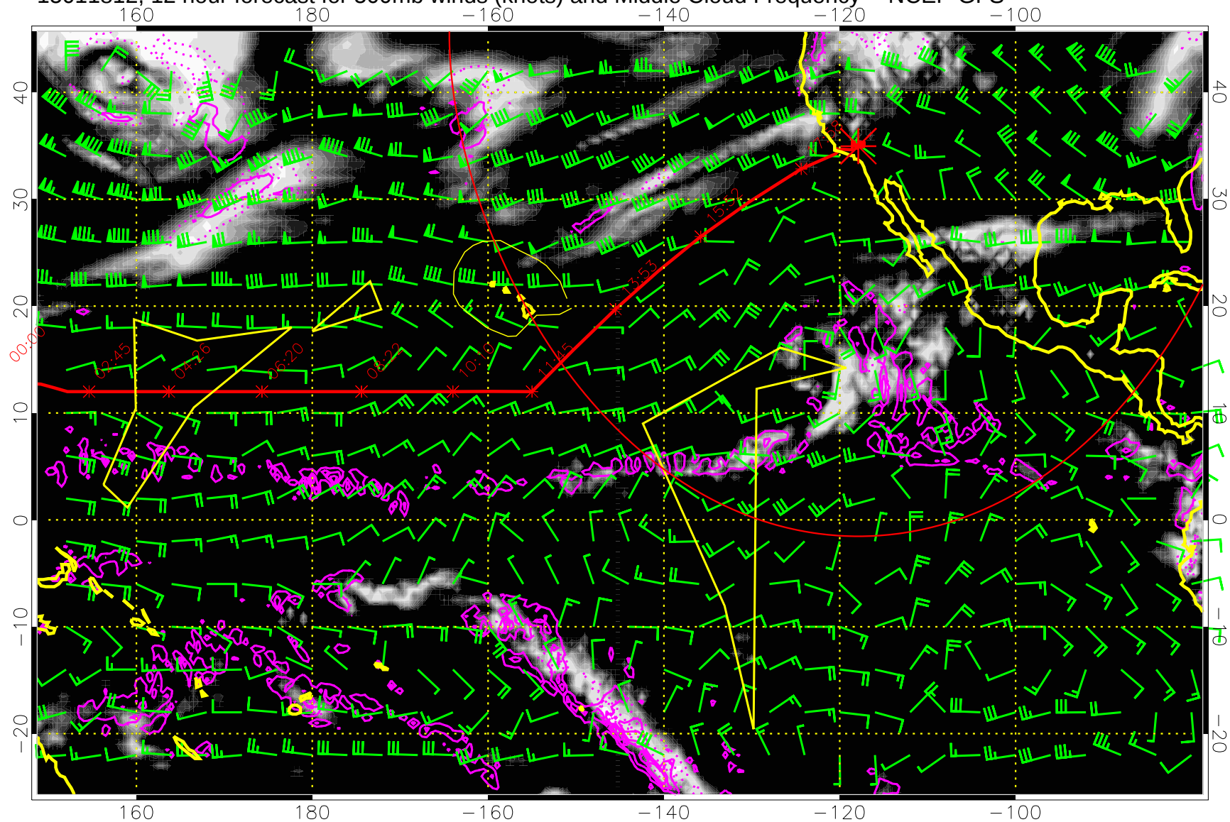
15011812, 12 hour forecast for 500mb winds (knots) and Middle Cloud Frequency -- NCEP GFS
