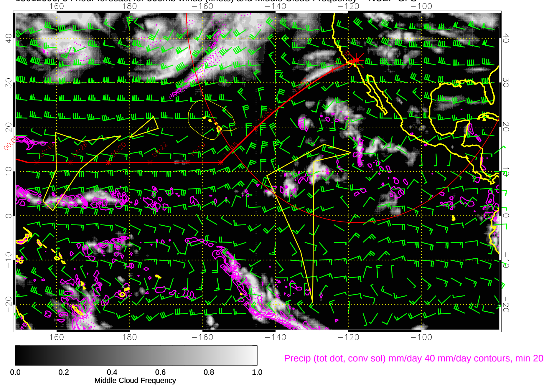
15012006, 54 hour forecast for 500mb winds (knots) and Middle Cloud Frequency -- NCEP GFS
