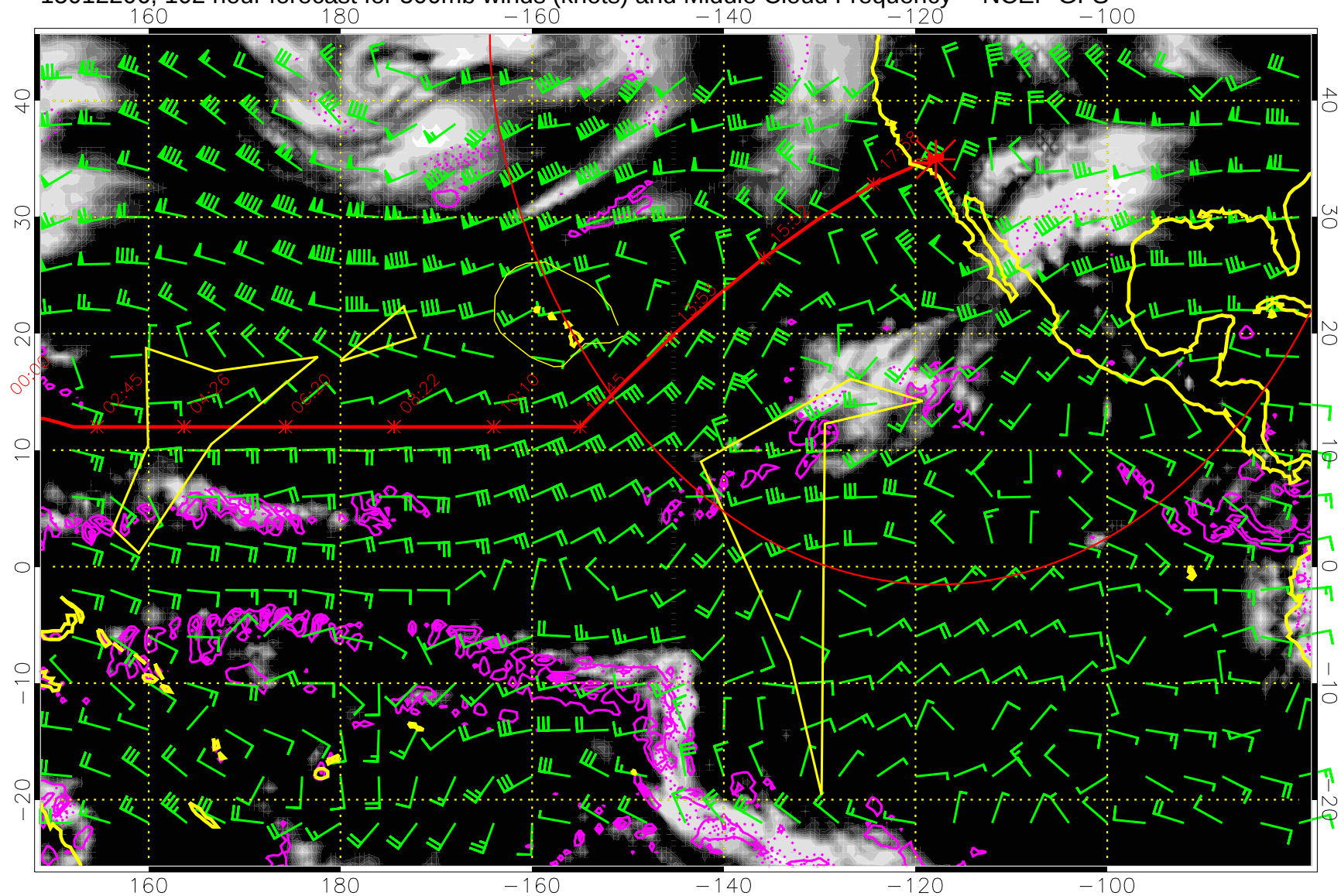
15012206, 102 hour forecast for 500mb winds (knots) and Middle Cloud Frequency -- NCEP GFS
