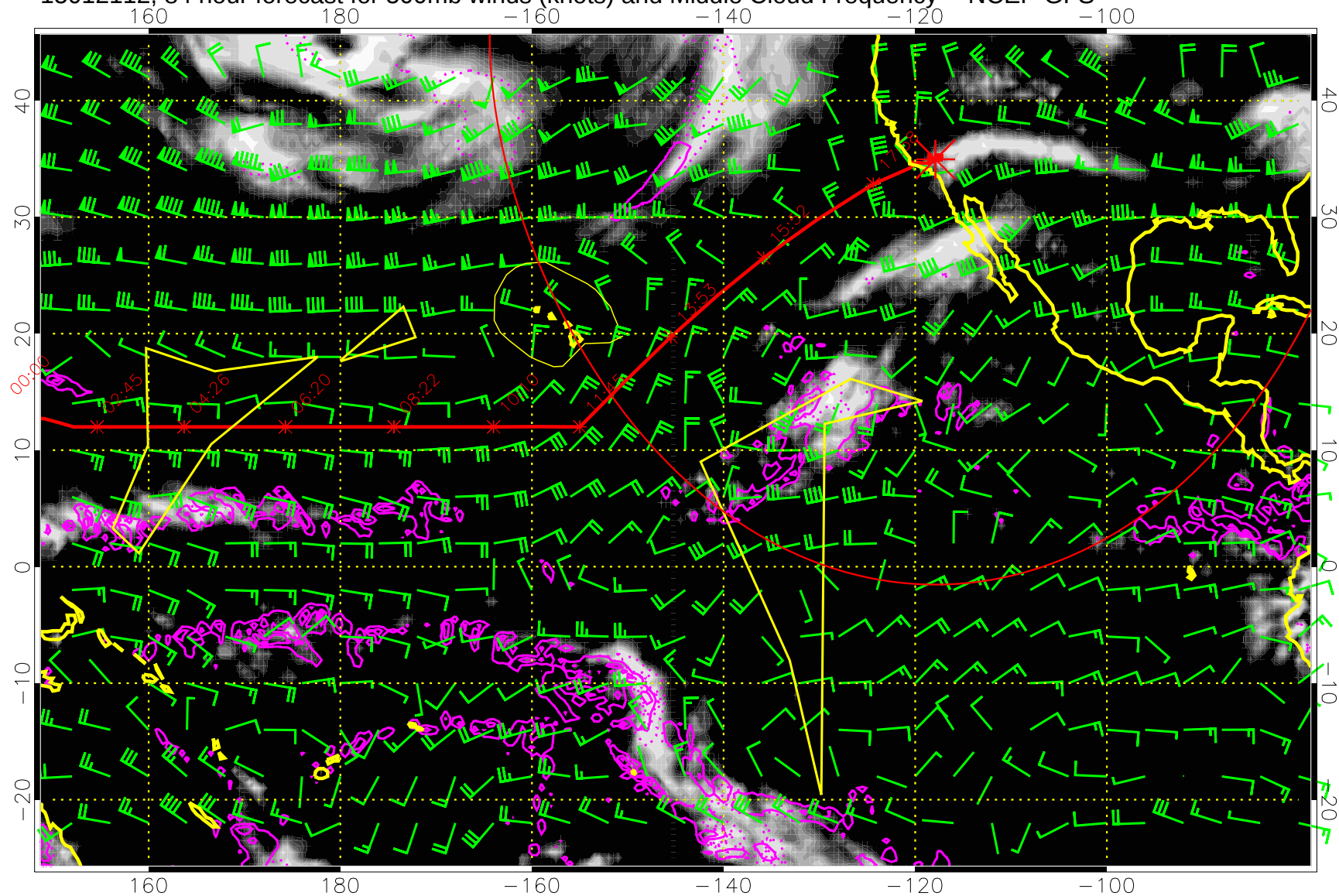
15012112, 84 hour forecast for 500mb winds (knots) and Middle Cloud Frequency -- NCEP GFS
