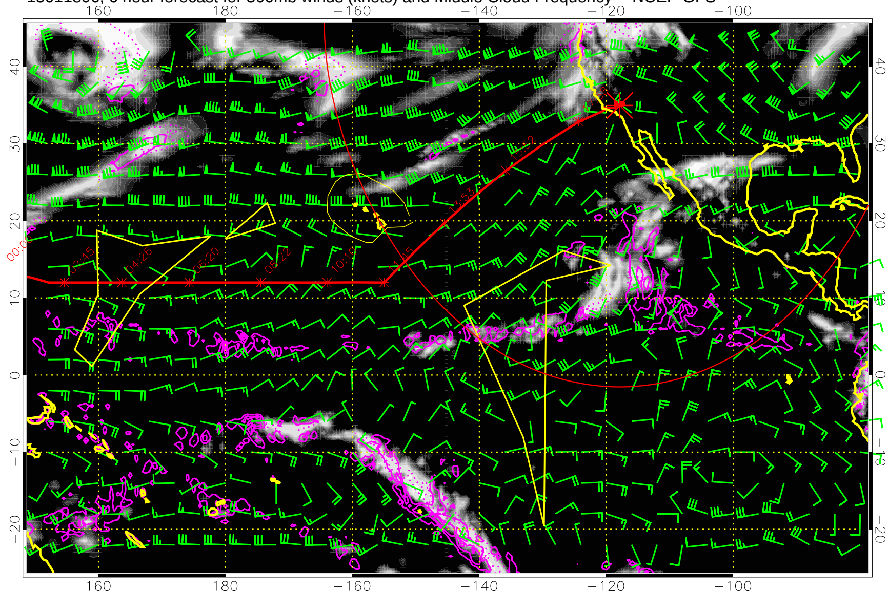
15011806, 6 hour forecast for 500mb winds (knots) and Middle Cloud Frequency -- NCEP GFS
