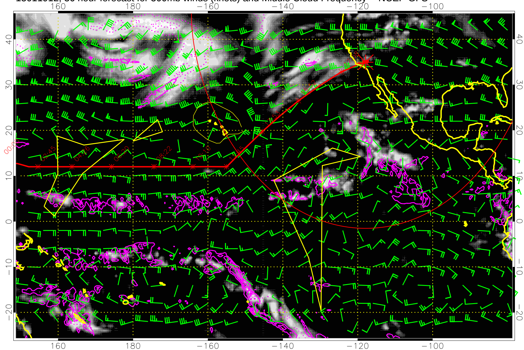
15011912, 36 hour forecast for 500mb winds (knots) and Middle Cloud Frequency -- NCEP GFS
