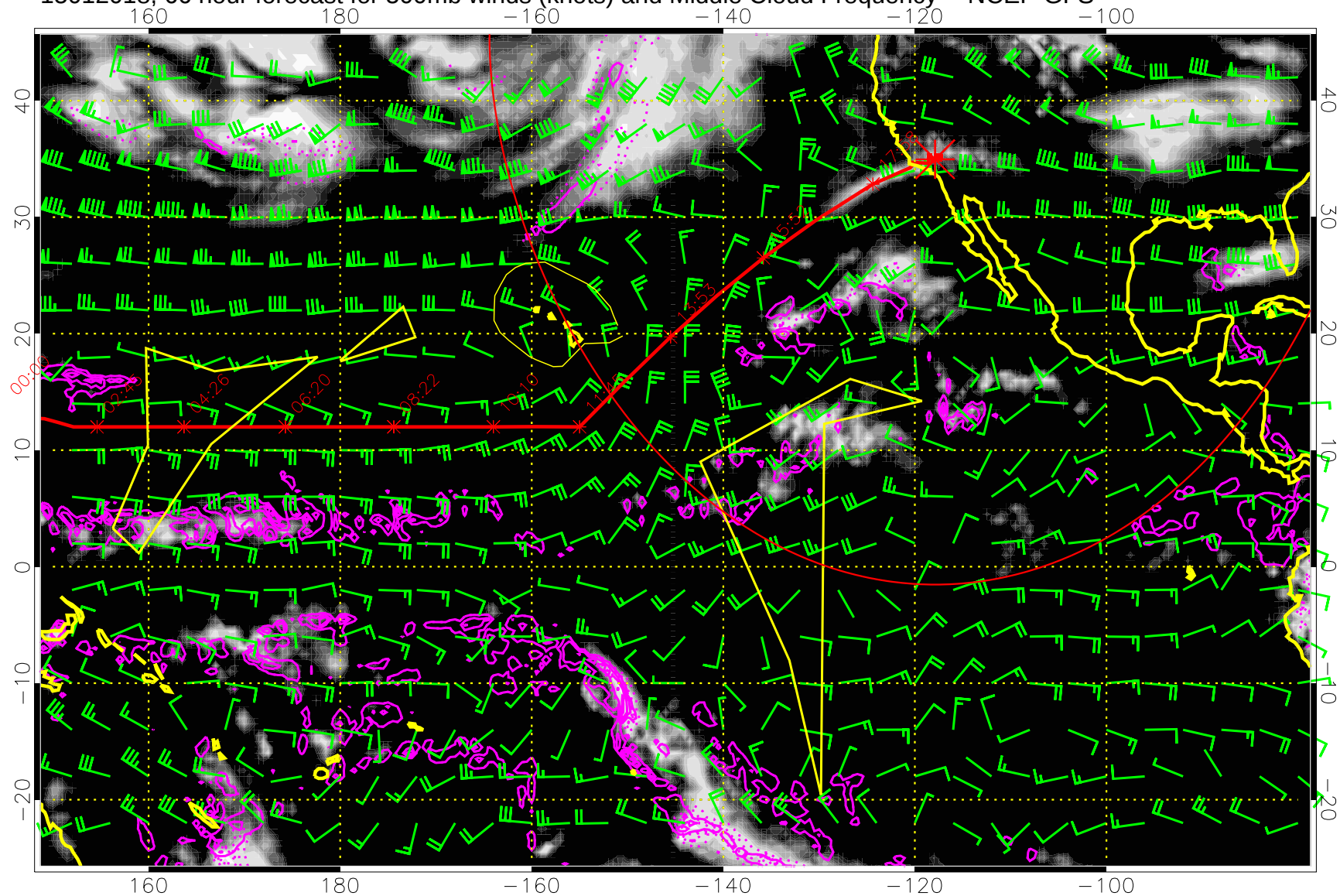
15012018, 66 hour forecast for 500mb winds (knots) and Middle Cloud Frequency -- NCEP GFS
