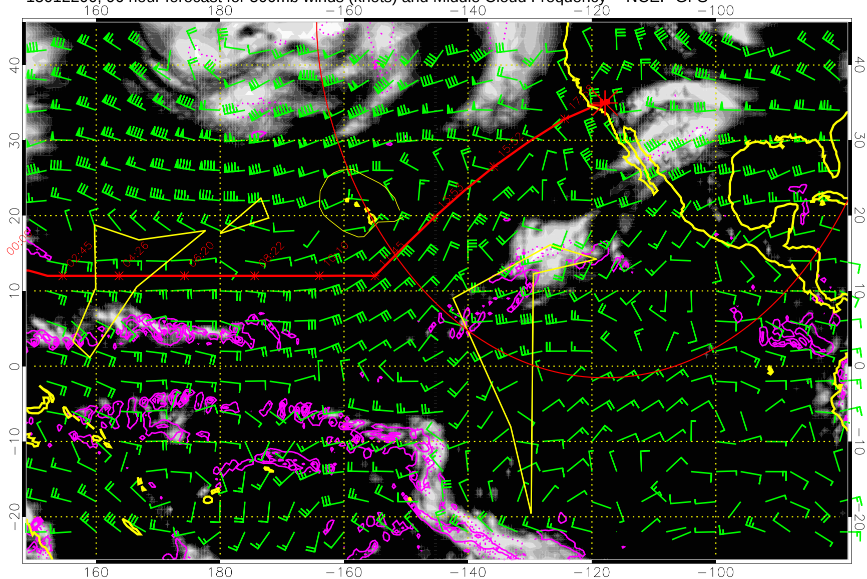
15012200, 96 hour forecast for 500mb winds (knots) and Middle Cloud Frequency -- NCEP GFS
