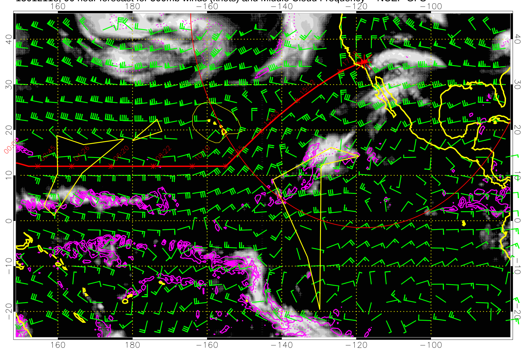
15012118, 90 hour forecast for 500mb winds (knots) and Middle Cloud Frequency -- NCEP GFS
