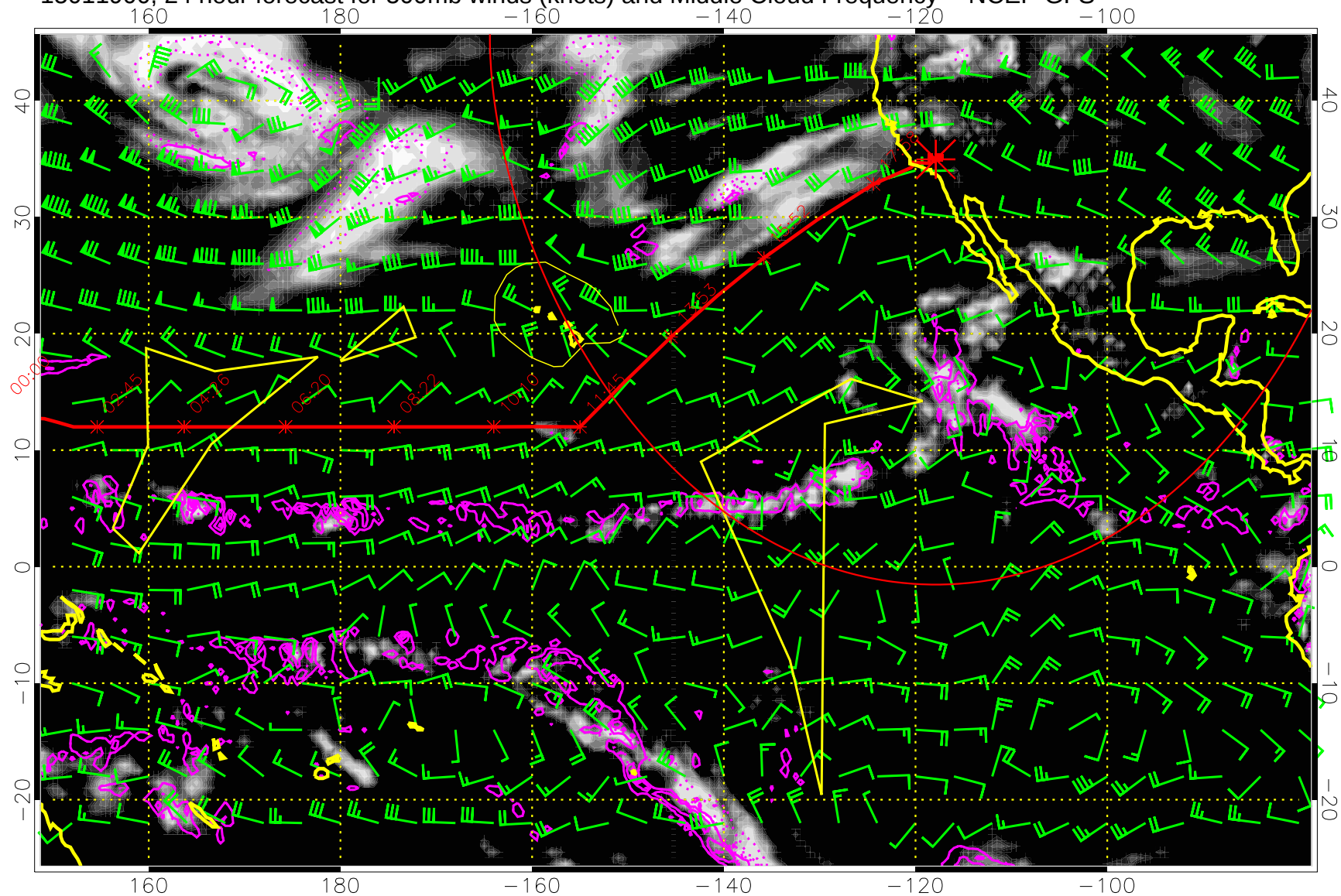
15011900, 24 hour forecast for 500mb winds (knots) and Middle Cloud Frequency -- NCEP GFS
