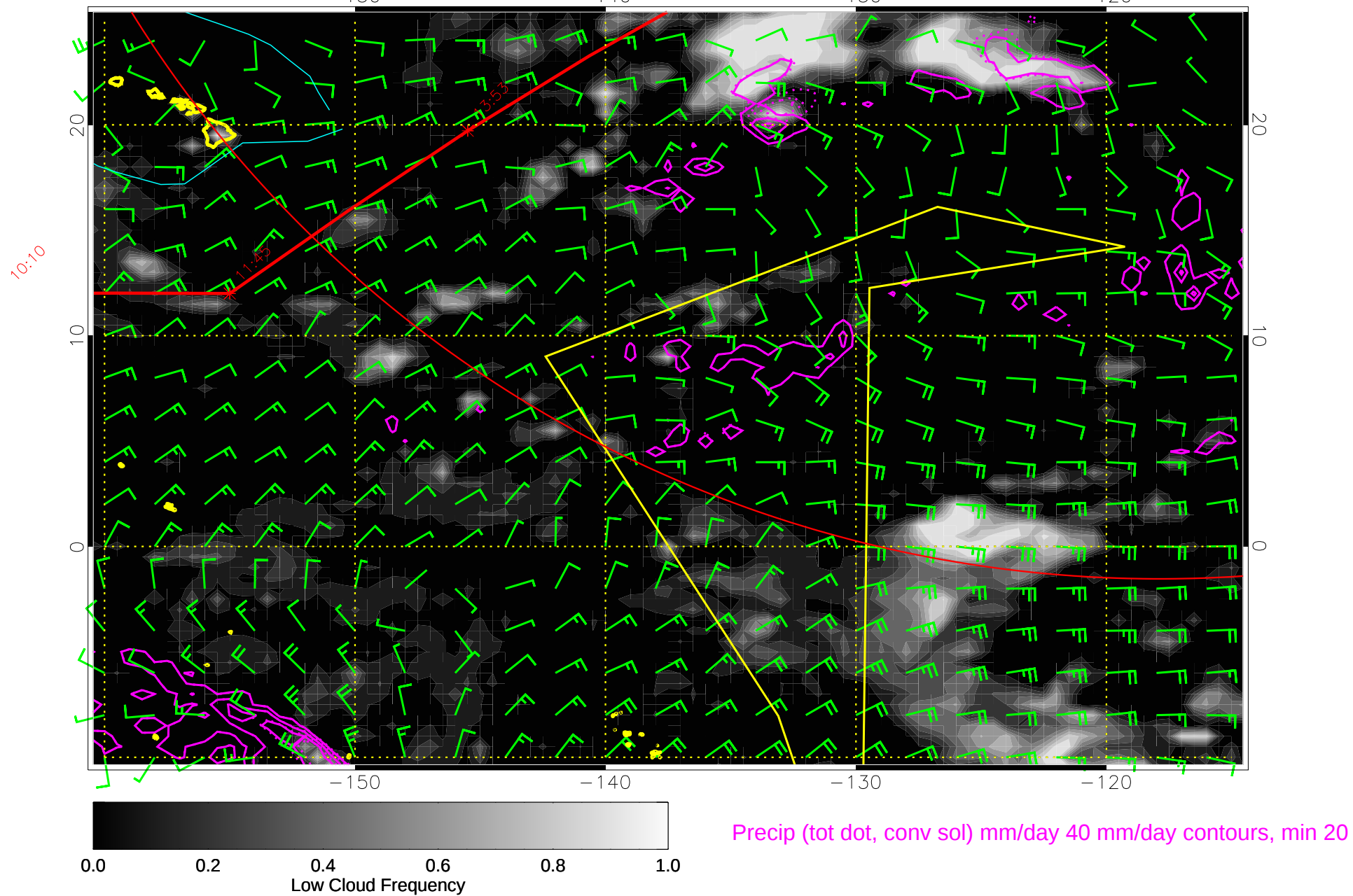
15012012, 60 hour forecast for 850mb winds (knots) and Low Cloud Frequency -- NCEP GFS
