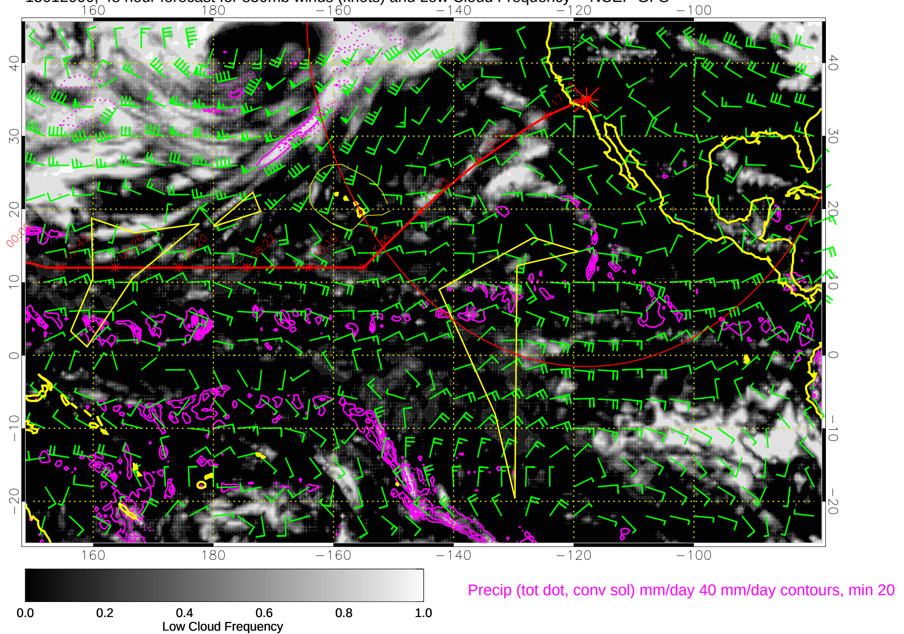
15012000, 48 hour forecast for 850mb winds (knots) and Low Cloud Frequency -- NCEP GFS
