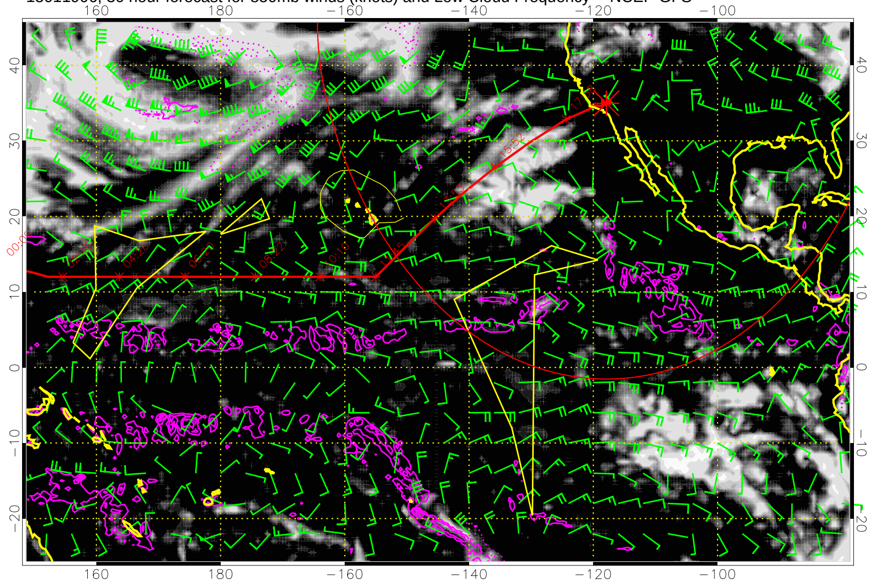
15011906, 30 hour forecast for 850mb winds (knots) and Low Cloud Frequency -- NCEP GFS
