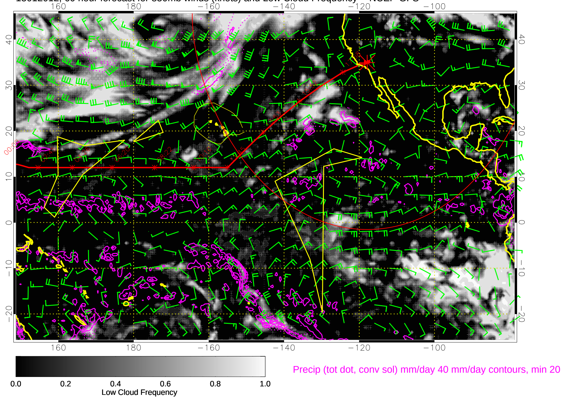
15012012, 60 hour forecast for 850mb winds (knots) and Low Cloud Frequency -- NCEP GFS
