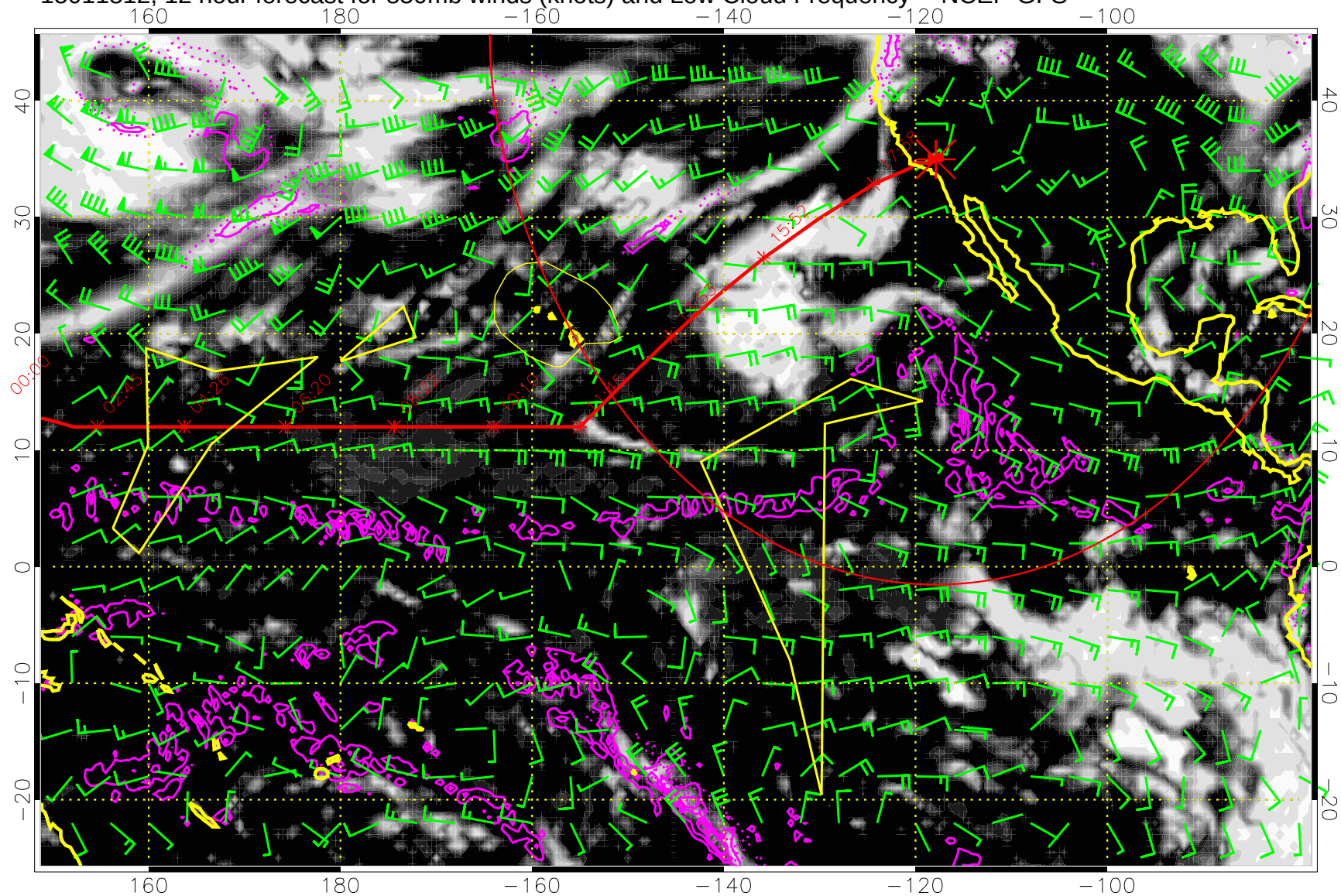
15011812, 12 hour forecast for 850mb winds (knots) and Low Cloud Frequency -- NCEP GFS
