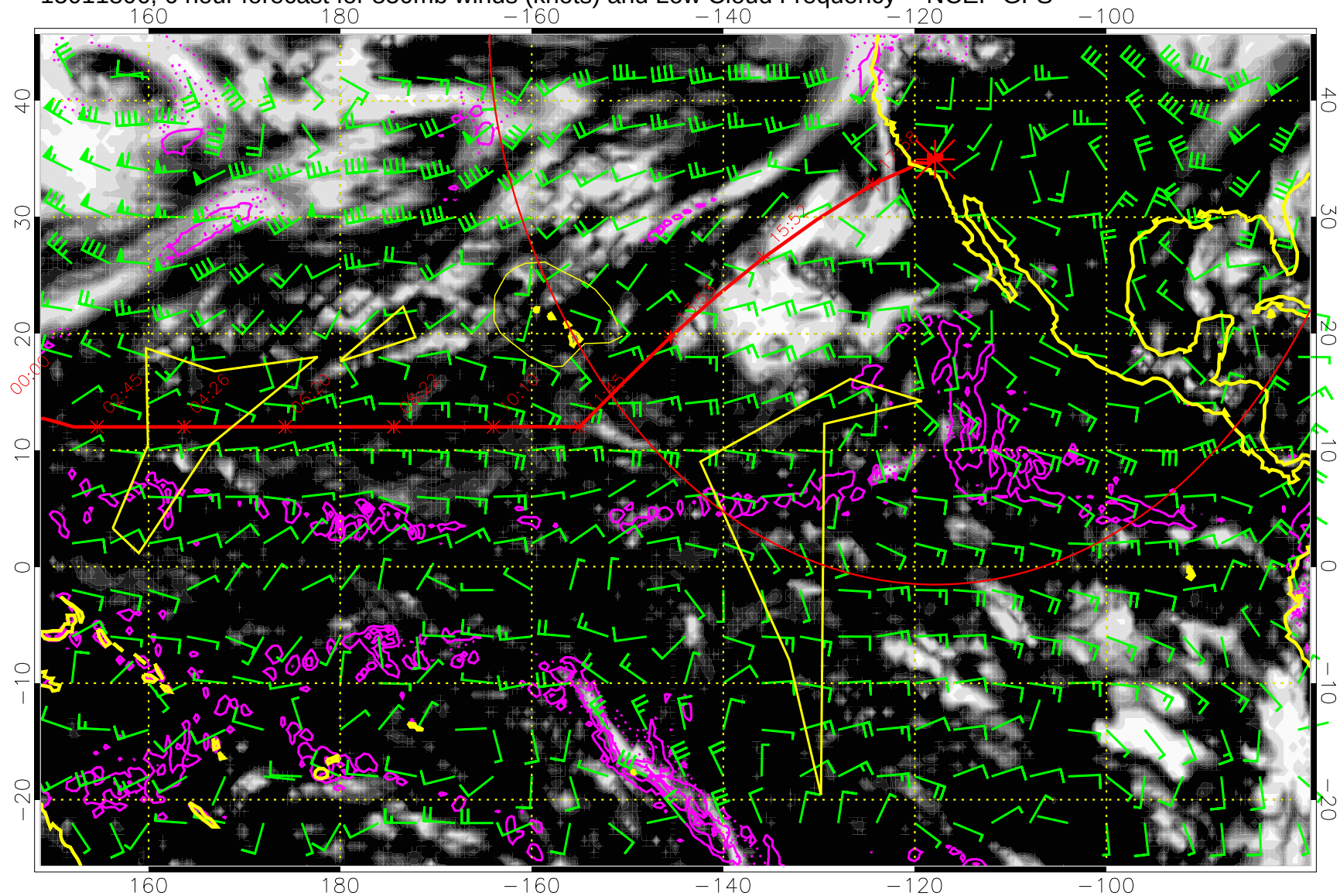
15011806, 6 hour forecast for 850mb winds (knots) and Low Cloud Frequency -- NCEP GFS
