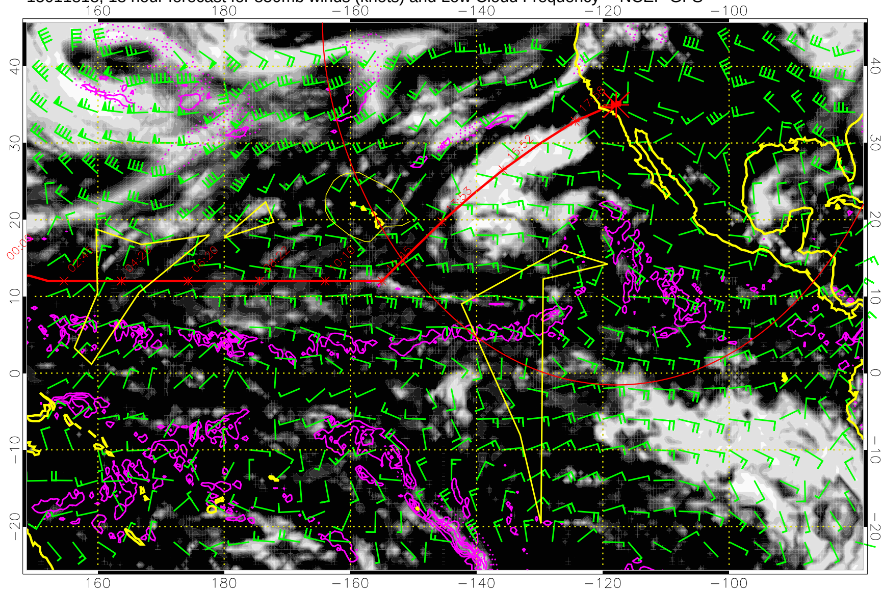
15011818, 18 hour forecast for 850mb winds (knots) and Low Cloud Frequency -- NCEP GFS
