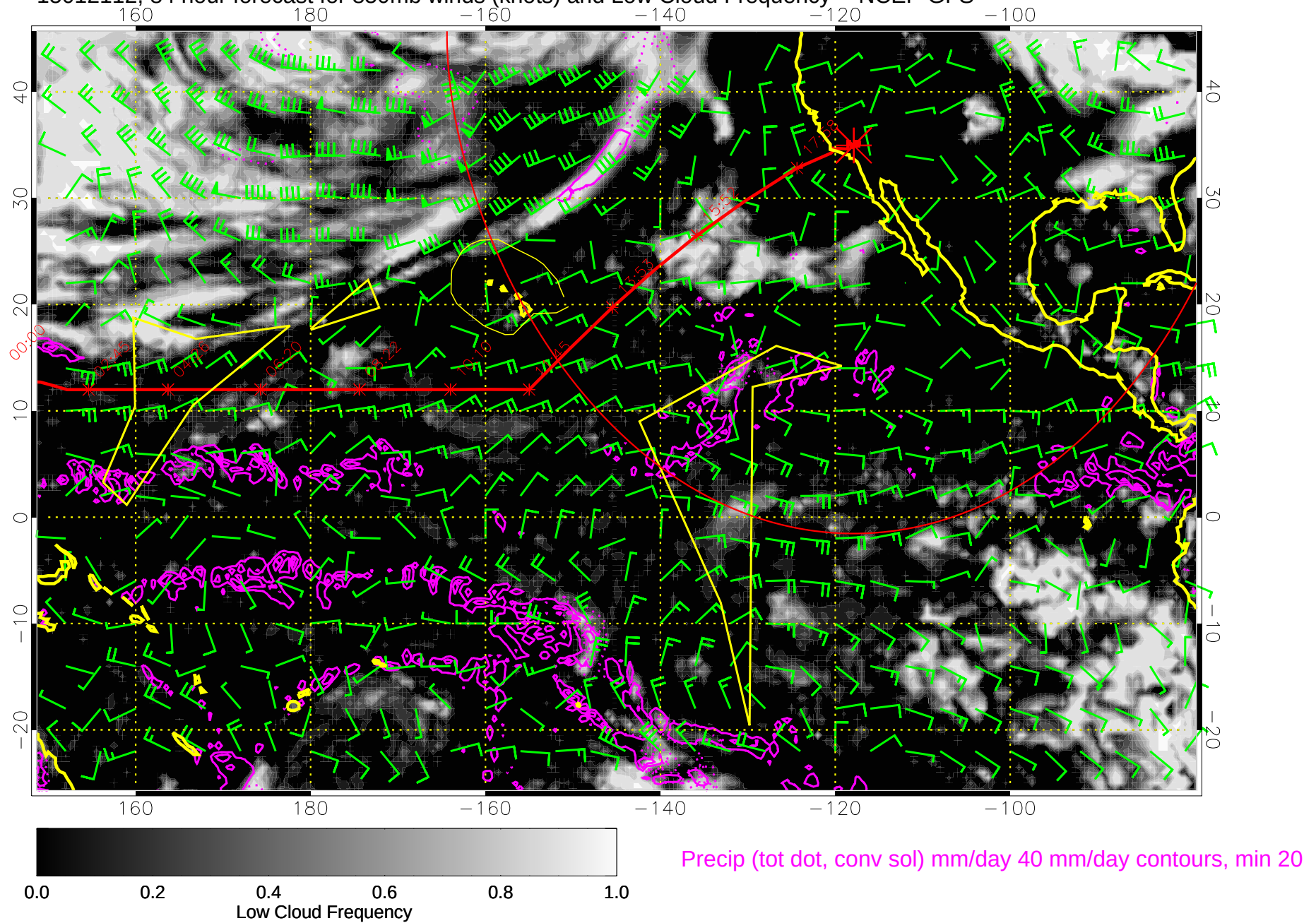
15012112, 84 hour forecast for 850mb winds (knots) and Low Cloud Frequency -- NCEP GFS
