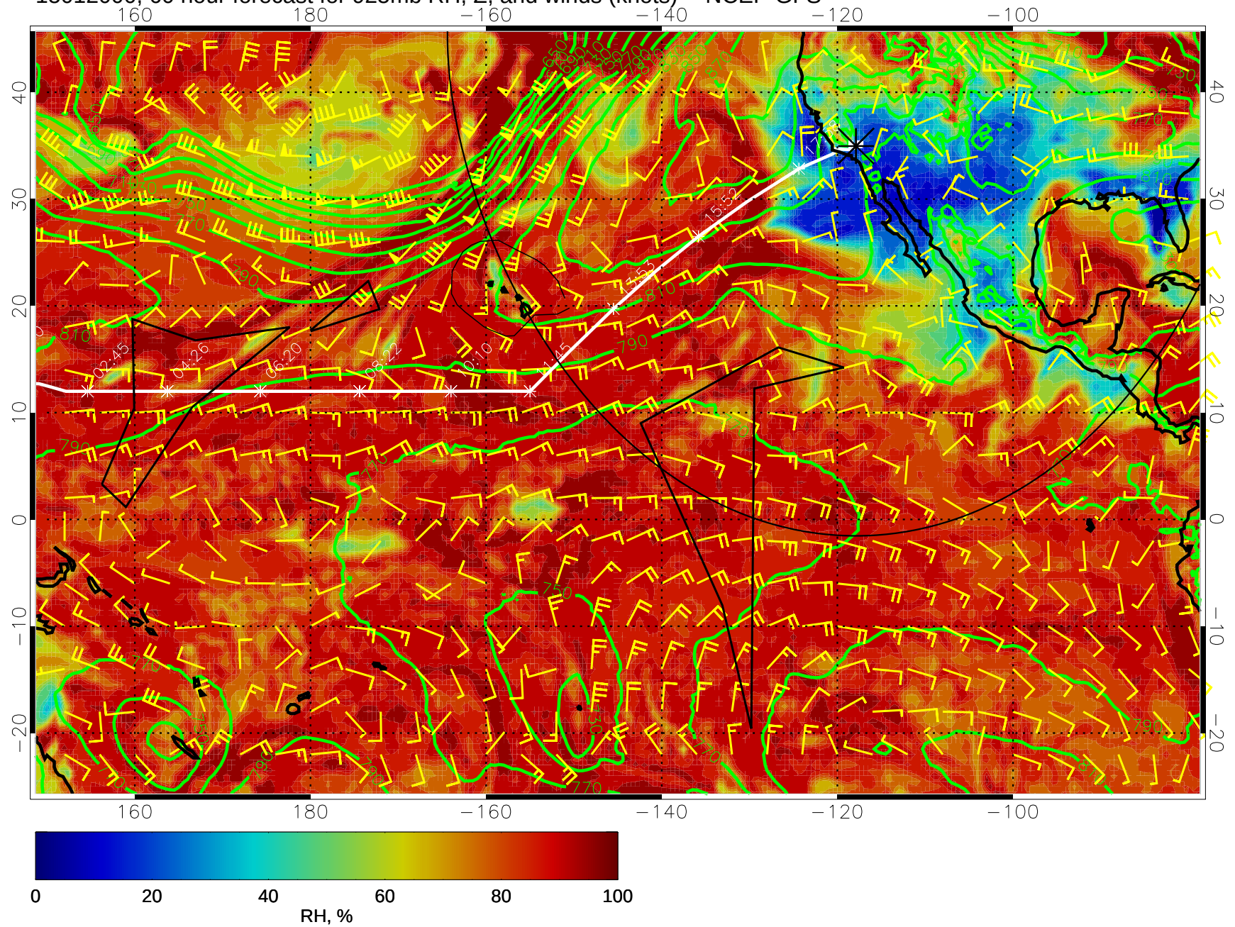
15012000, 60 hour forecast for 925mb RH, Z, and winds (knots) -- NCEP GFS
