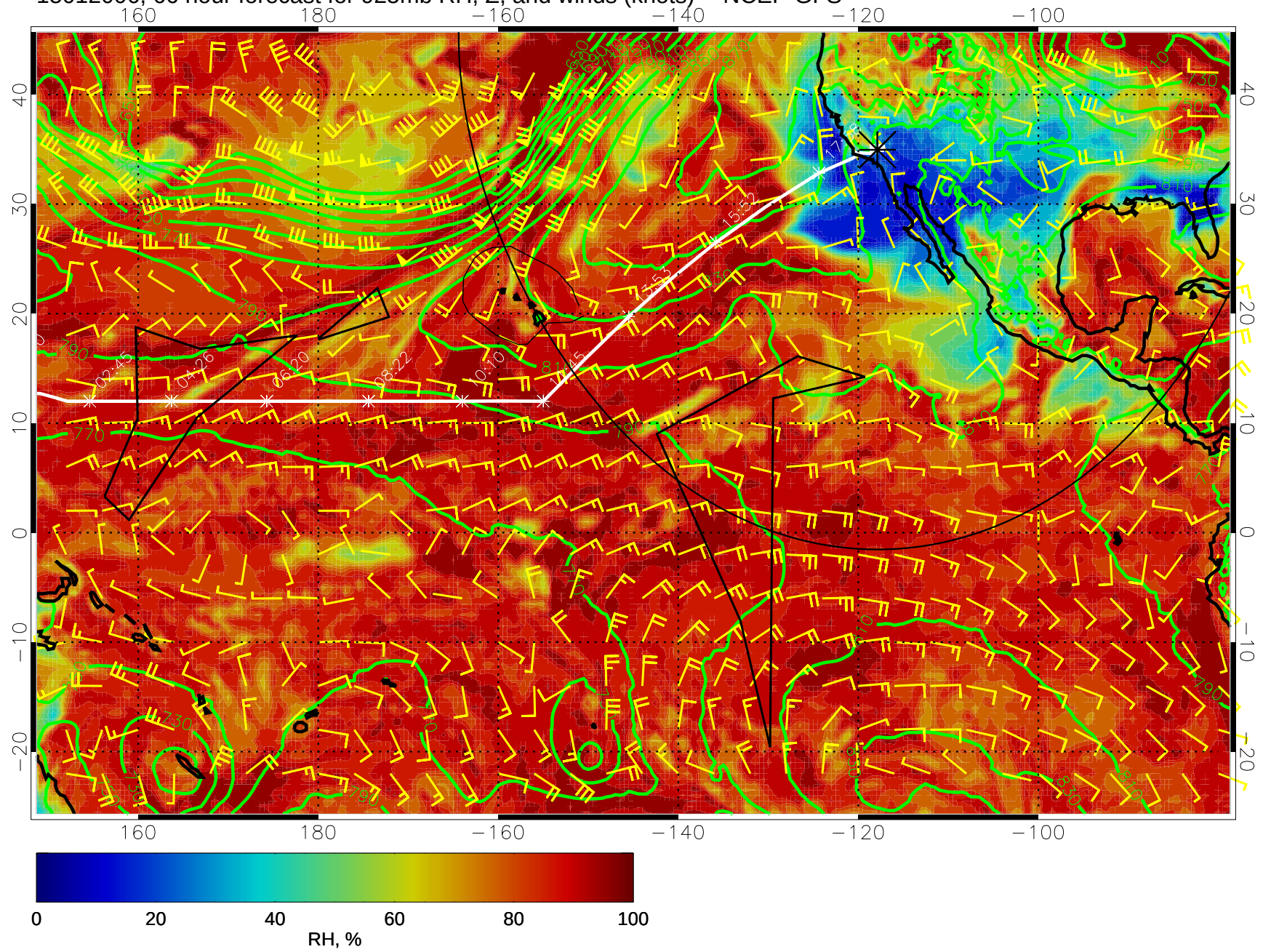
15012006, 66 hour forecast for 925mb RH, Z, and winds (knots) -- NCEP GFS
