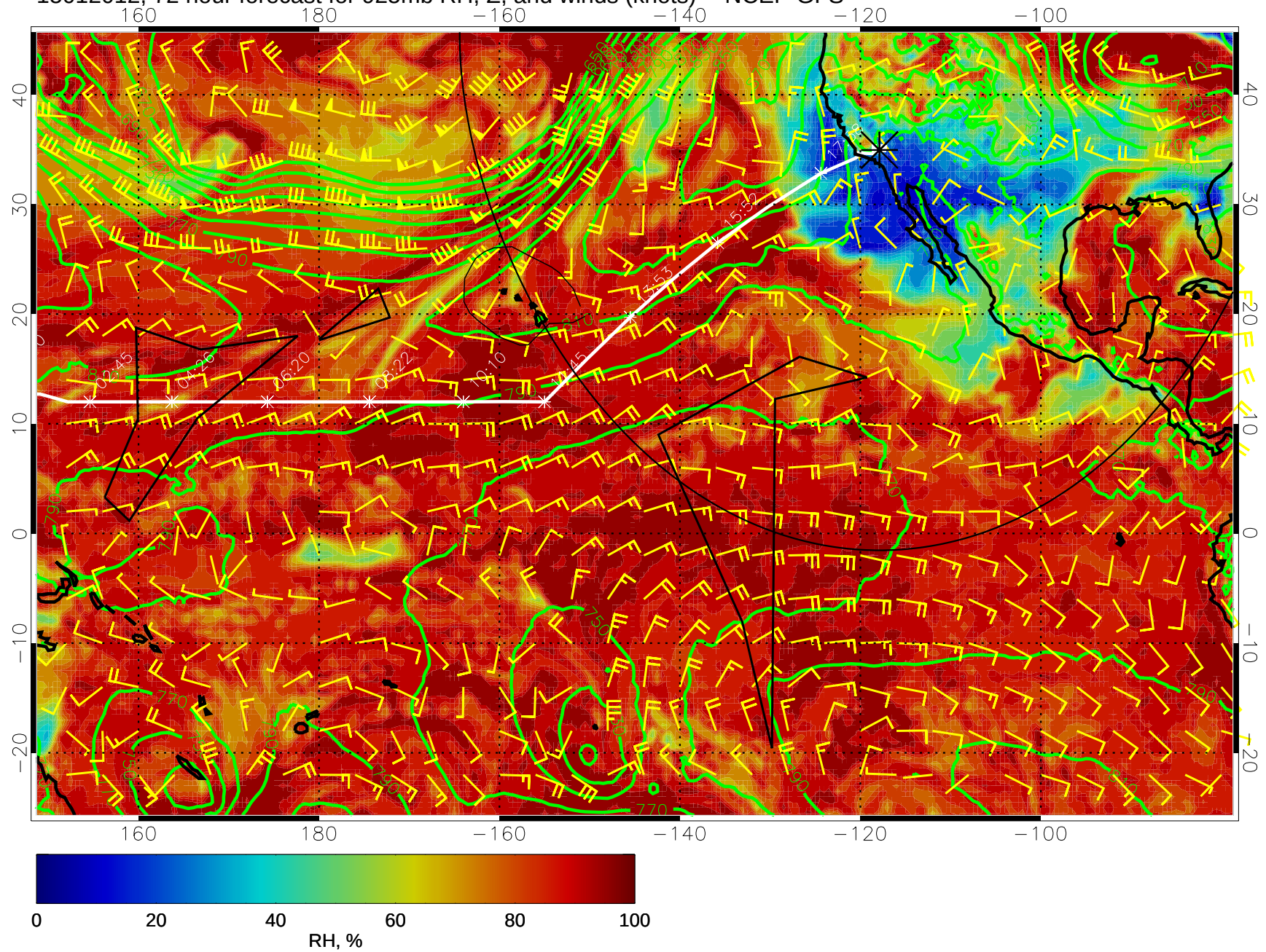
15012012, 72 hour forecast for 925mb RH, Z, and winds (knots) -- NCEP GFS
