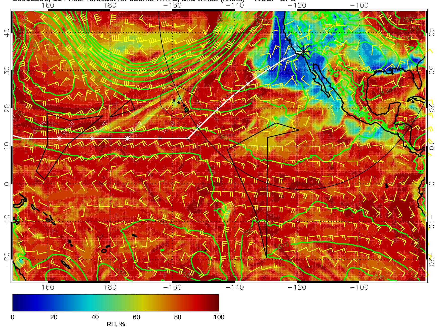
15012206, 114 hour forecast for 925mb RH, Z, and winds (knots) -- NCEP GFS
