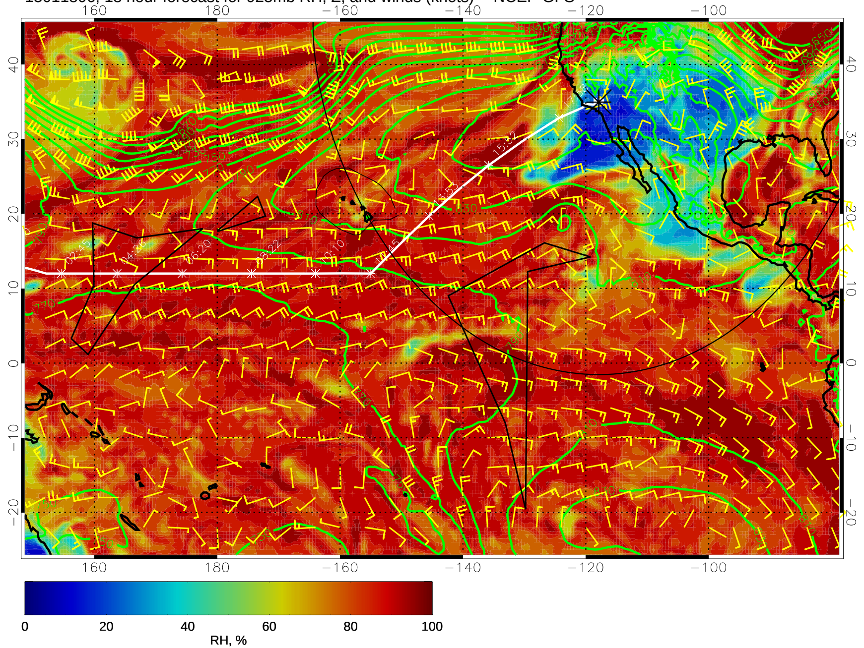
15011806, 18 hour forecast for 925mb RH, Z, and winds (knots) -- NCEP GFS
