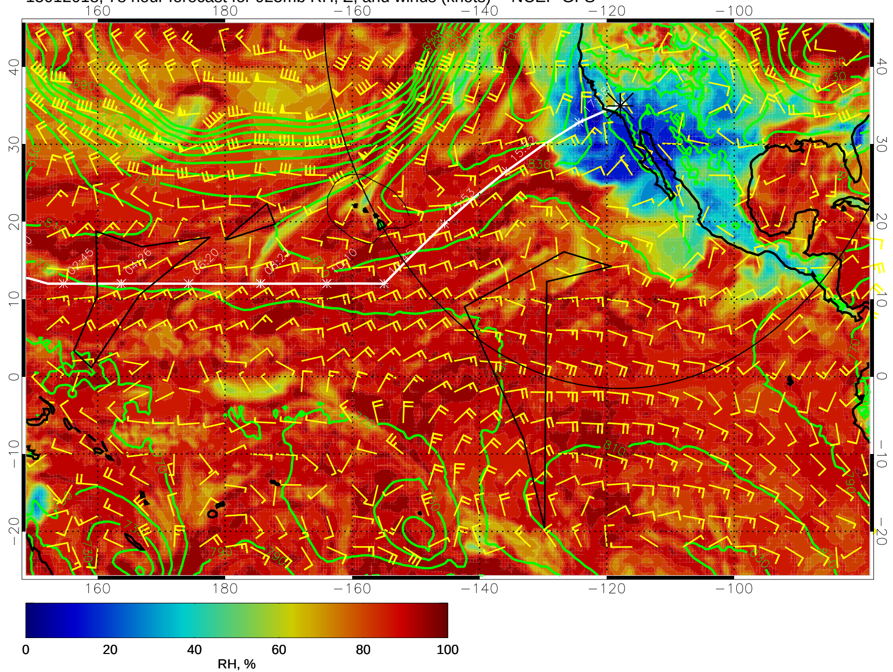
15012018, 78 hour forecast for 925mb RH, Z, and winds (knots) -- NCEP GFS
