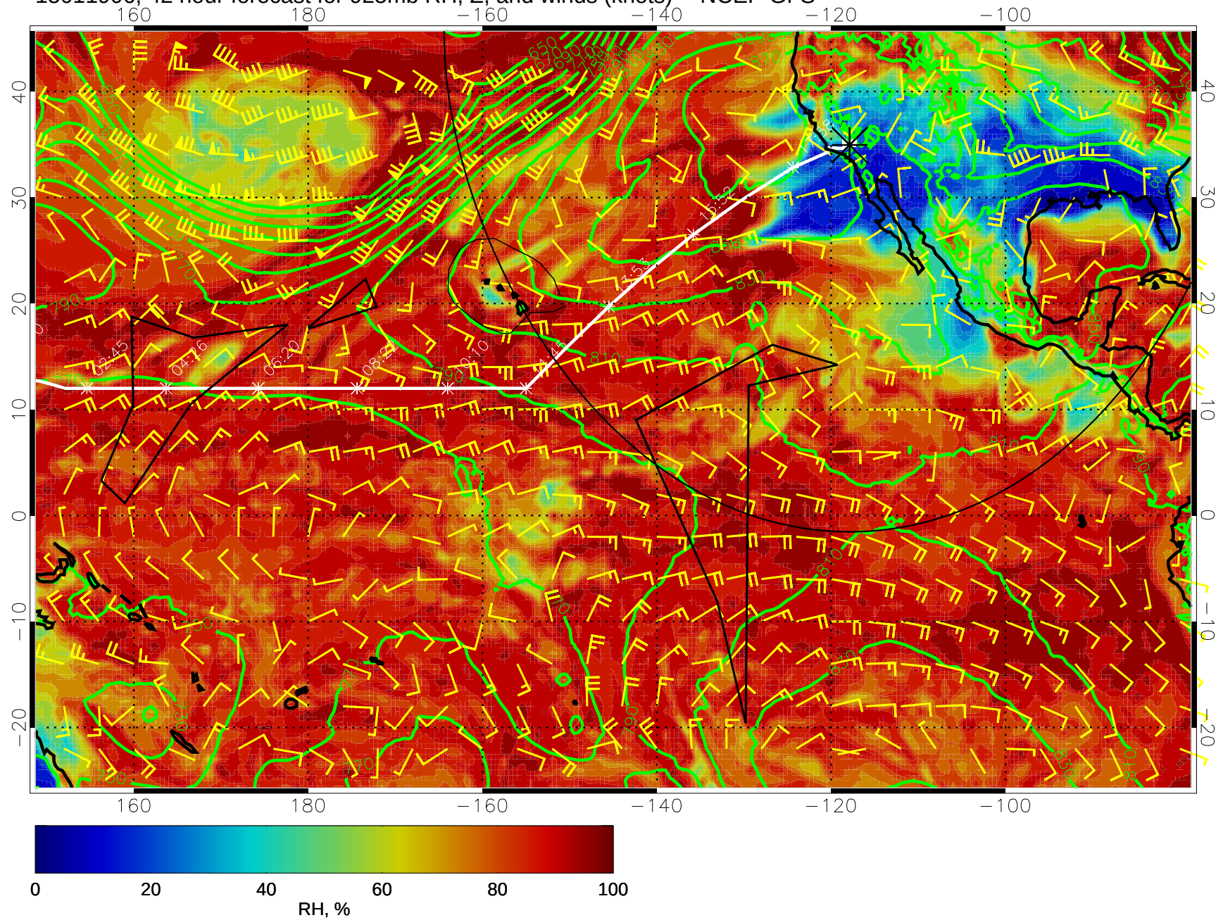
15011906, 42 hour forecast for 925mb RH, Z, and winds (knots) -- NCEP GFS
