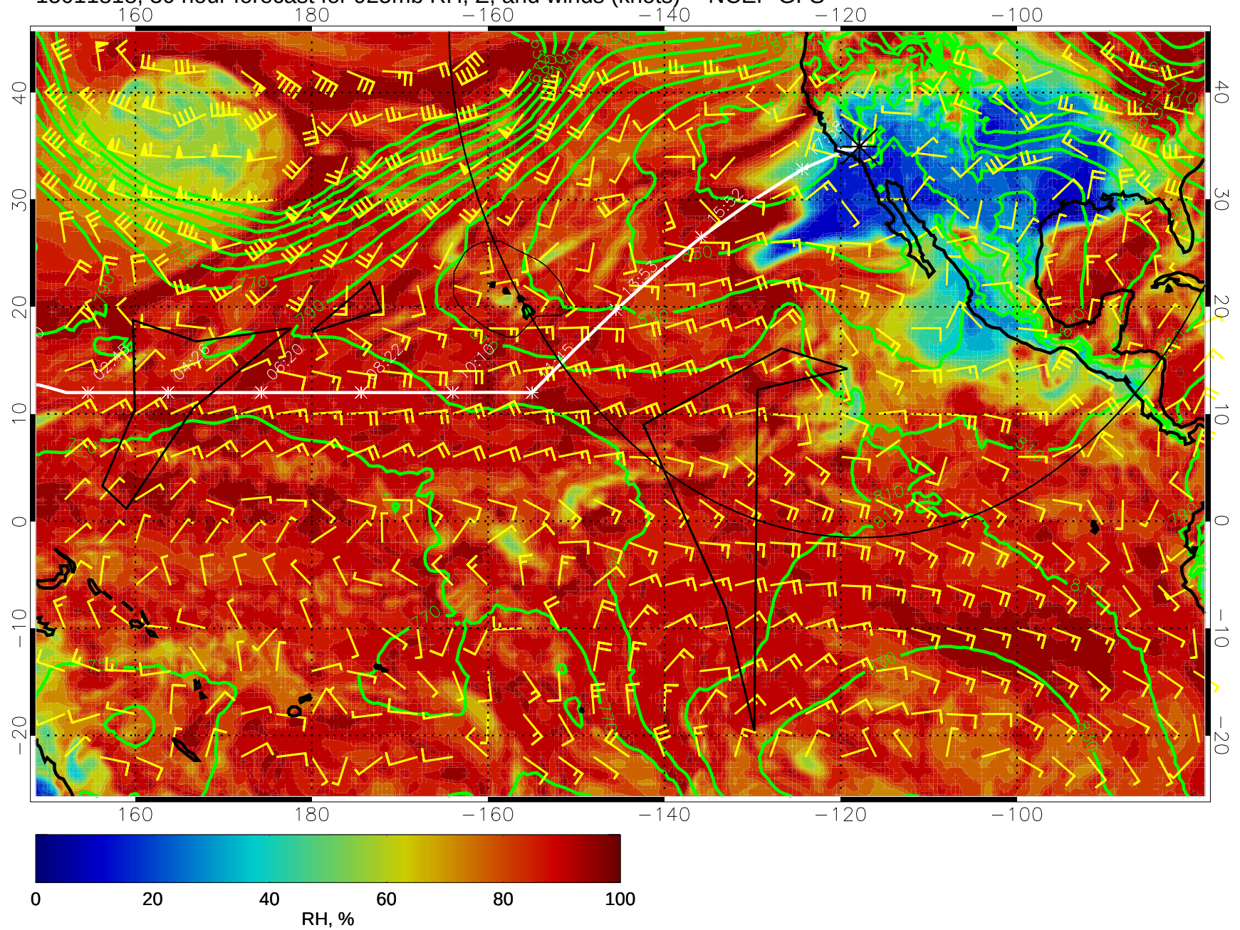
15011818, 30 hour forecast for 925mb RH, Z, and winds (knots) -- NCEP GFS
