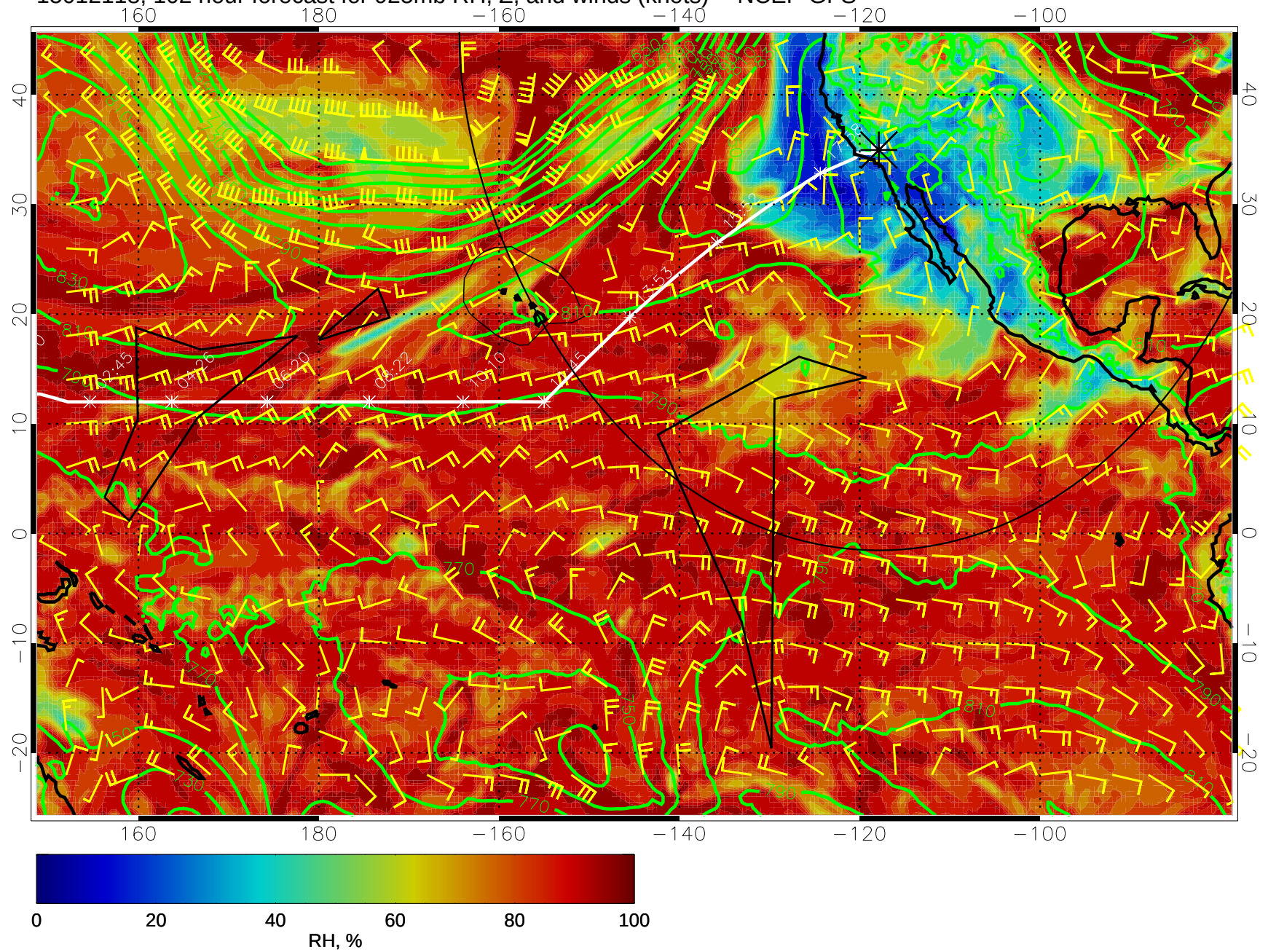
15012118, 102 hour forecast for 925mb RH, Z, and winds (knots) -- NCEP GFS
