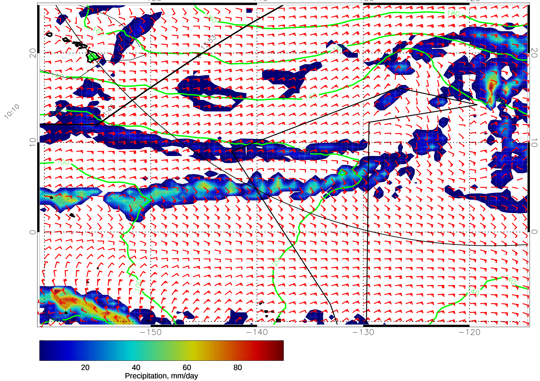
15011818, 30 hour forecast for precip, 1000mb Z, and winds (knots) -- NCEP GFS
