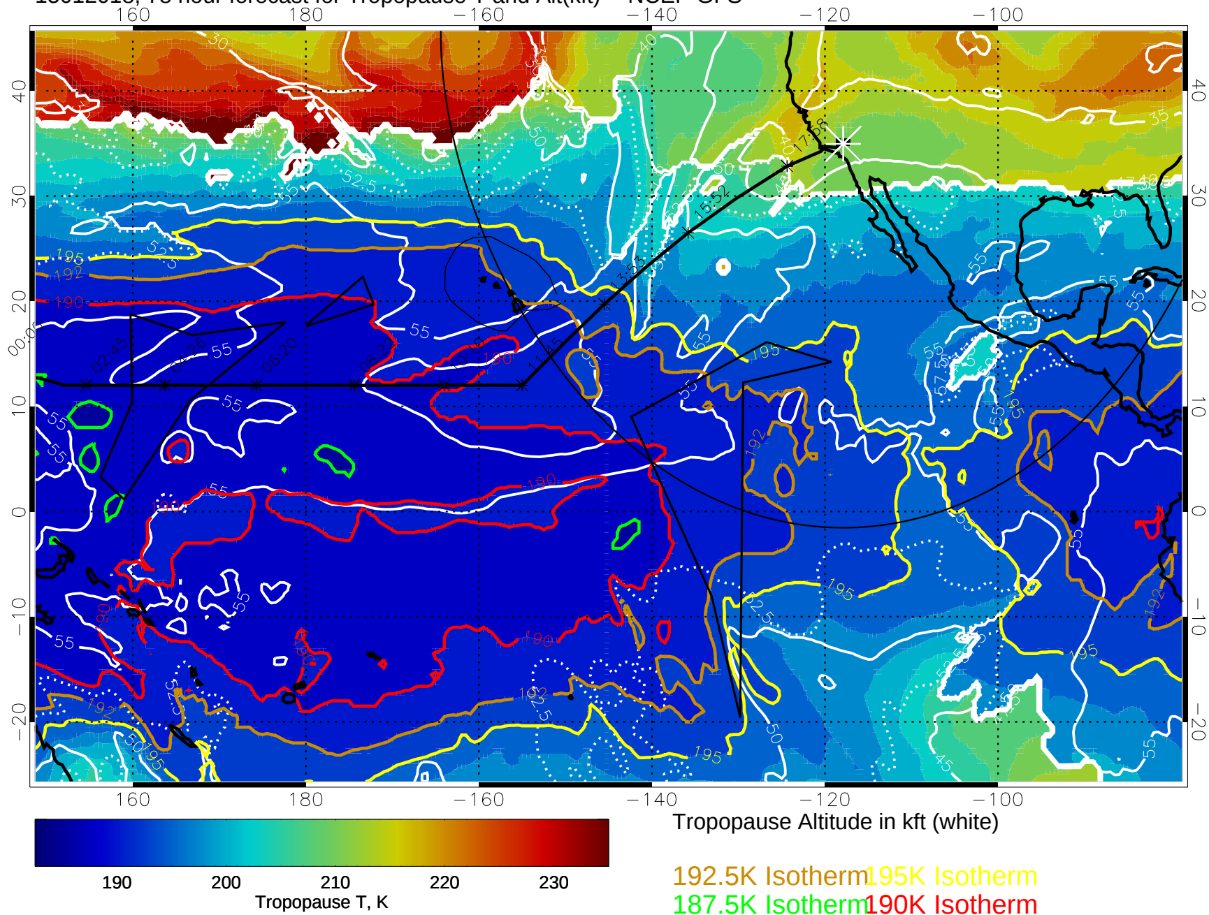
15012018, 78 hour forecast for Tropopause T and Alt(kft) -- NCEP GFS
