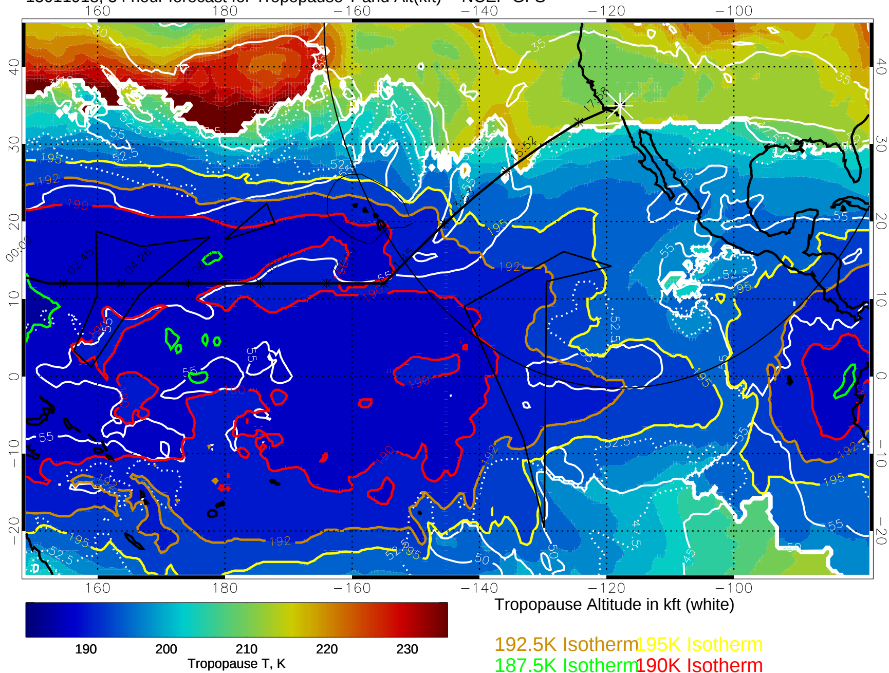
15011918, 54 hour forecast for Tropopause T and Alt(kft) -- NCEP GFS
