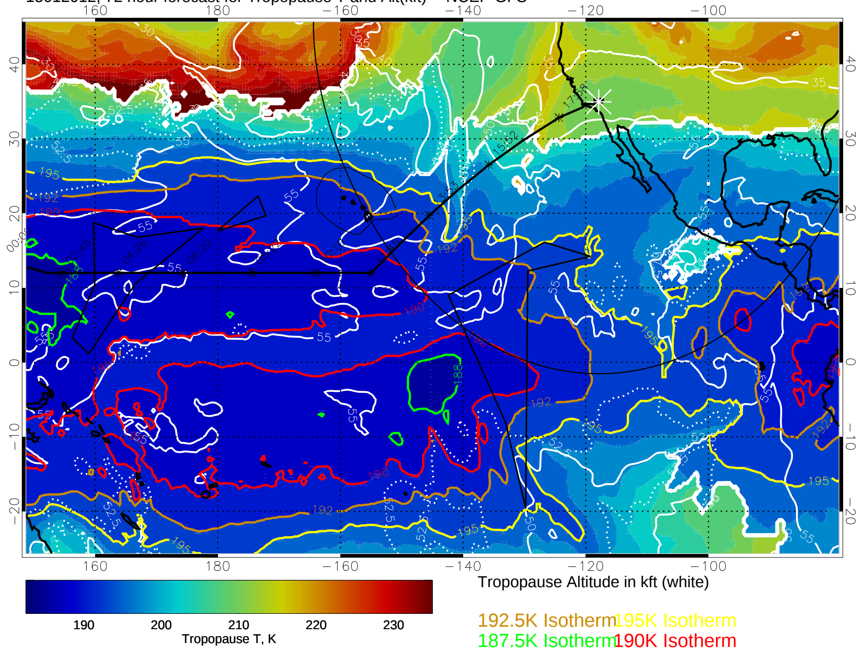
15012012, 72 hour forecast for Tropopause T and Alt(kft) -- NCEP GFS
