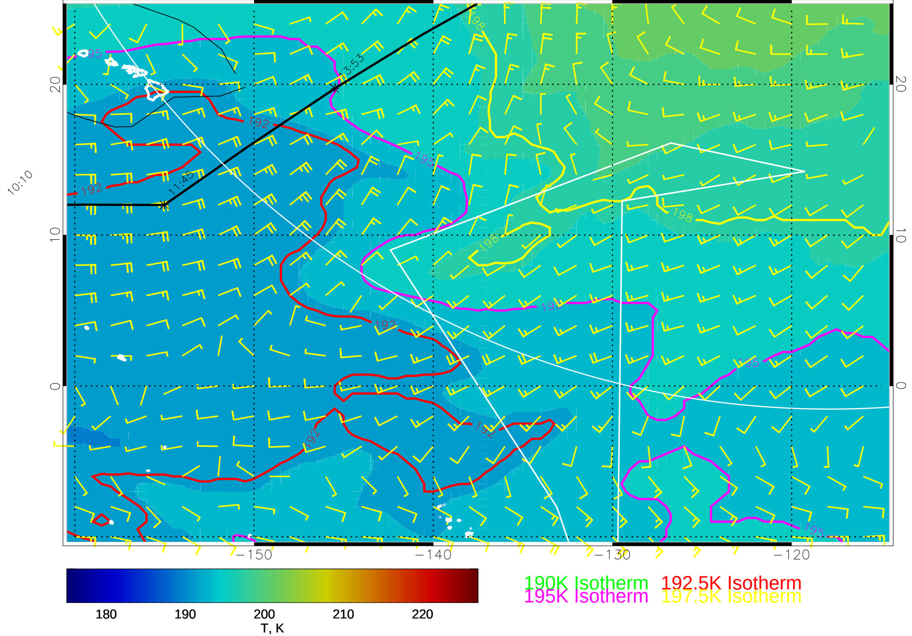
15012212, 120 hour forecast for 70mb T and winds (knots) -- NCEP GFS
