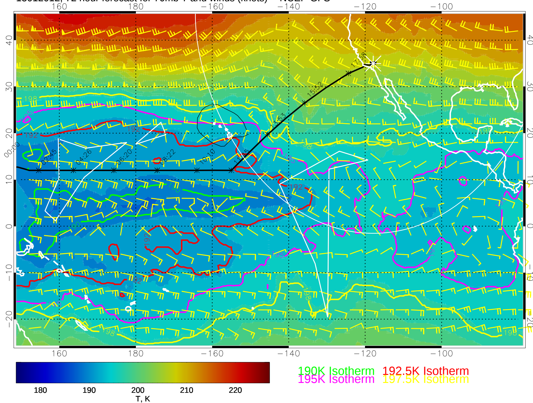
15012012, 72 hour forecast for 70mb T and winds (knots) -- NCEP GFS
