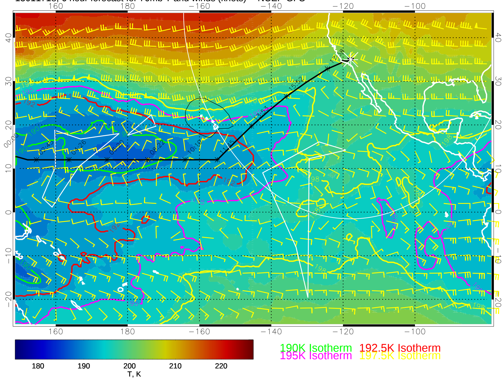
15011718, 6 hour forecast for 70mb T and winds (knots) -- NCEP GFS
