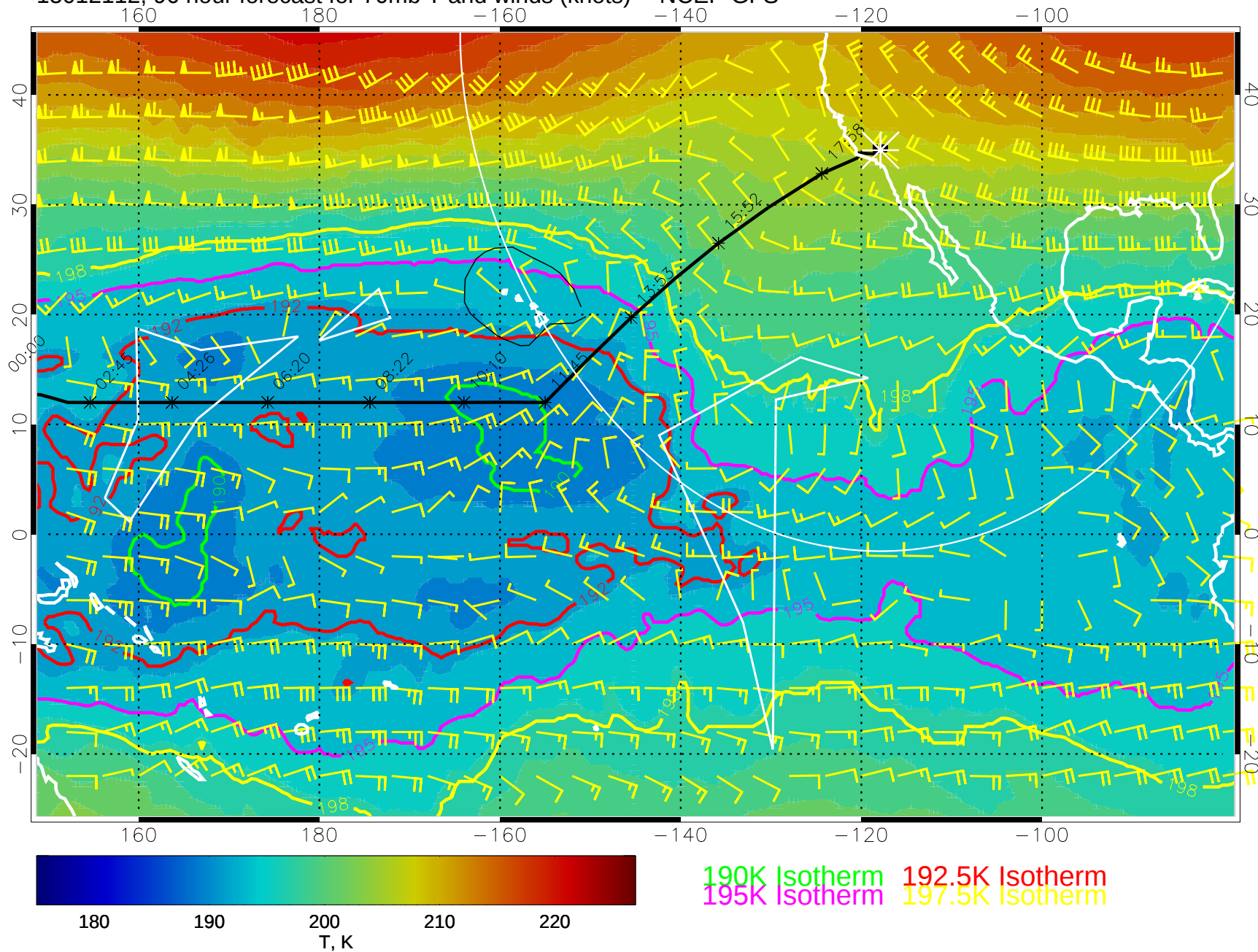
15012112, 96 hour forecast for 70mb T and winds (knots) -- NCEP GFS
