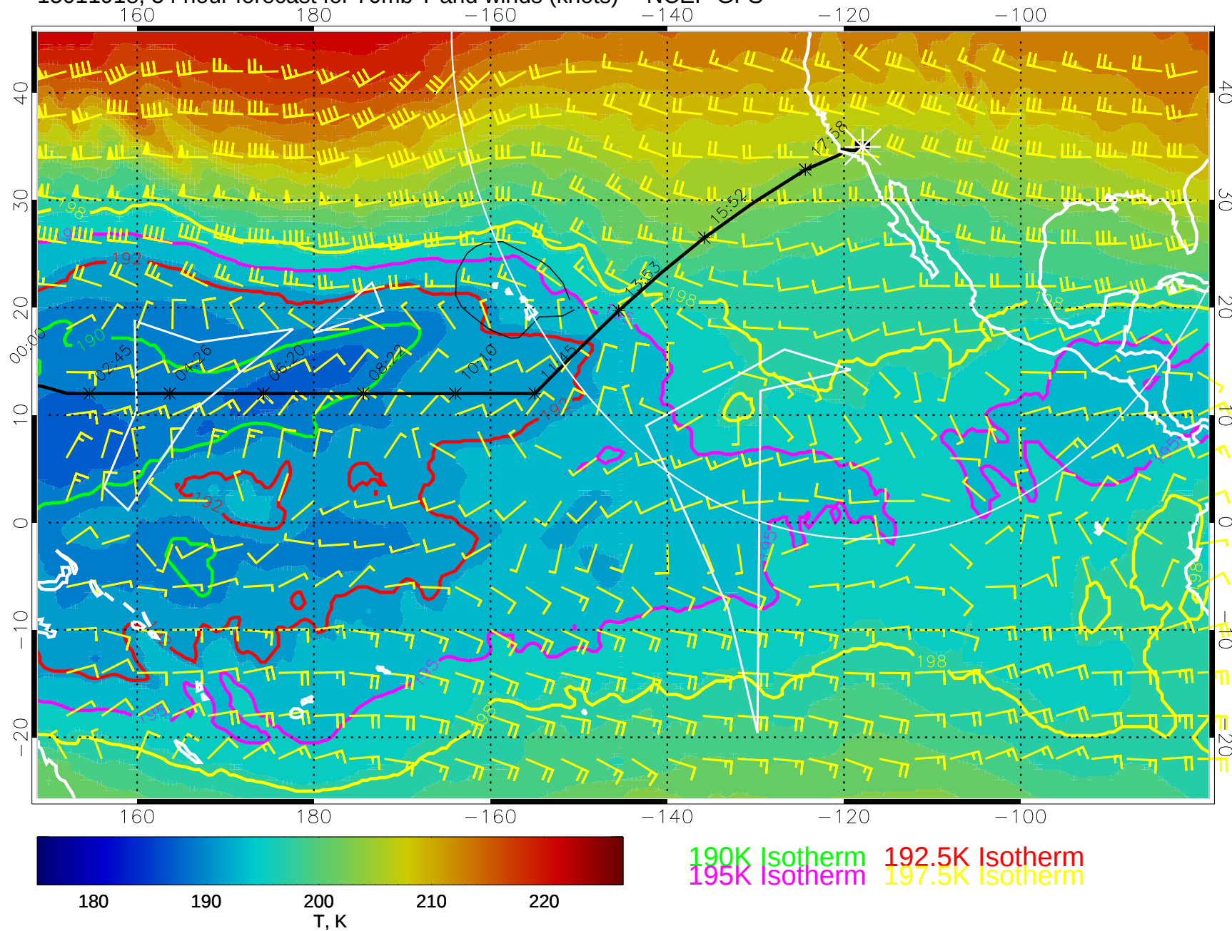
15011918, 54 hour forecast for 70mb T and winds (knots) -- NCEP GFS
