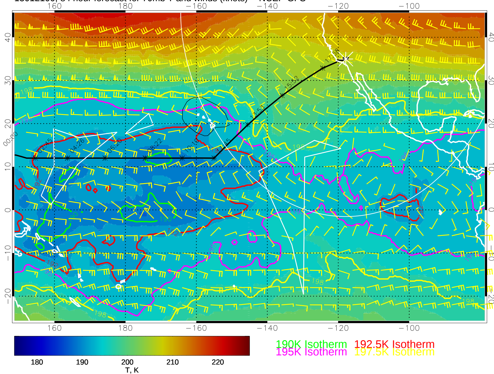
15012100, 84 hour forecast for 70mb T and winds (knots) -- NCEP GFS
