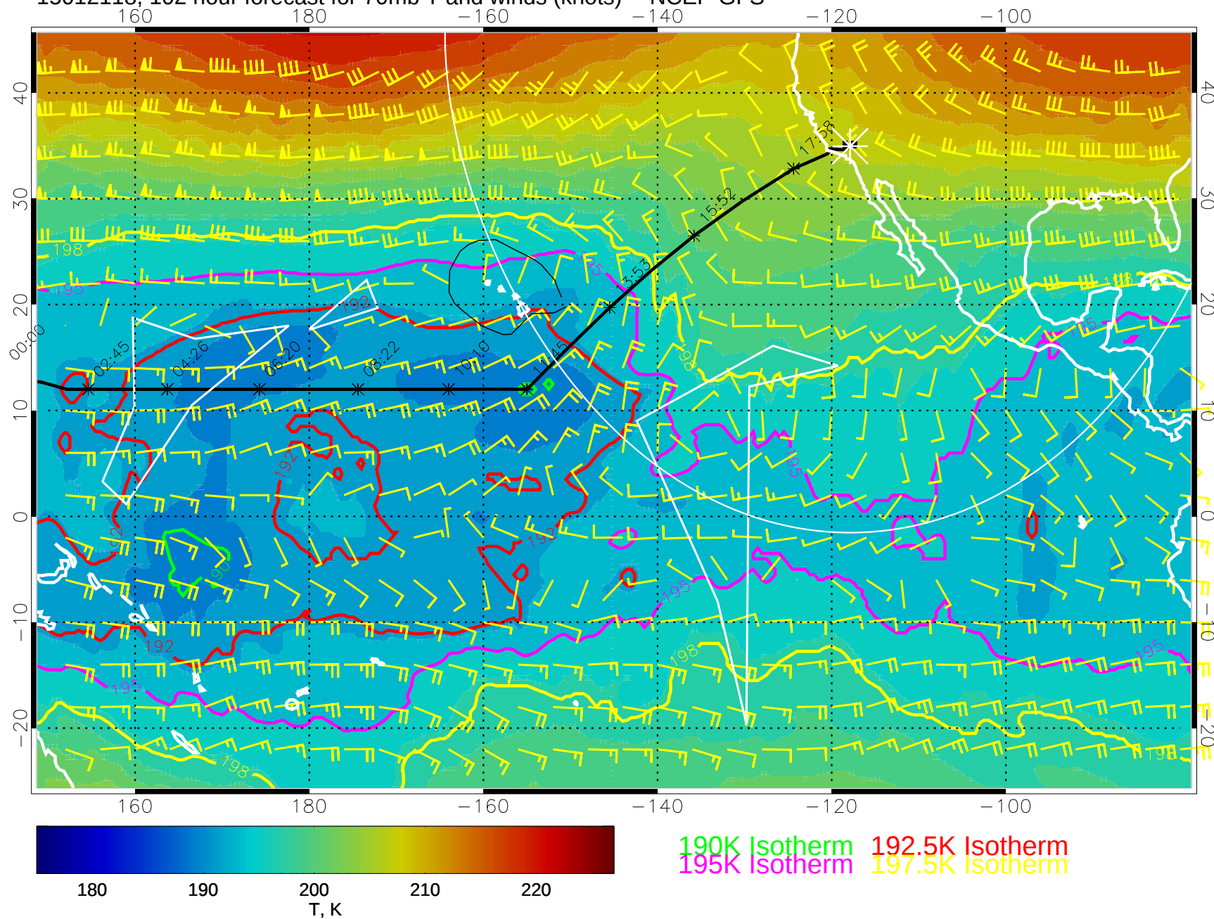
15012118, 102 hour forecast for 70mb T and winds (knots) -- NCEP GFS
