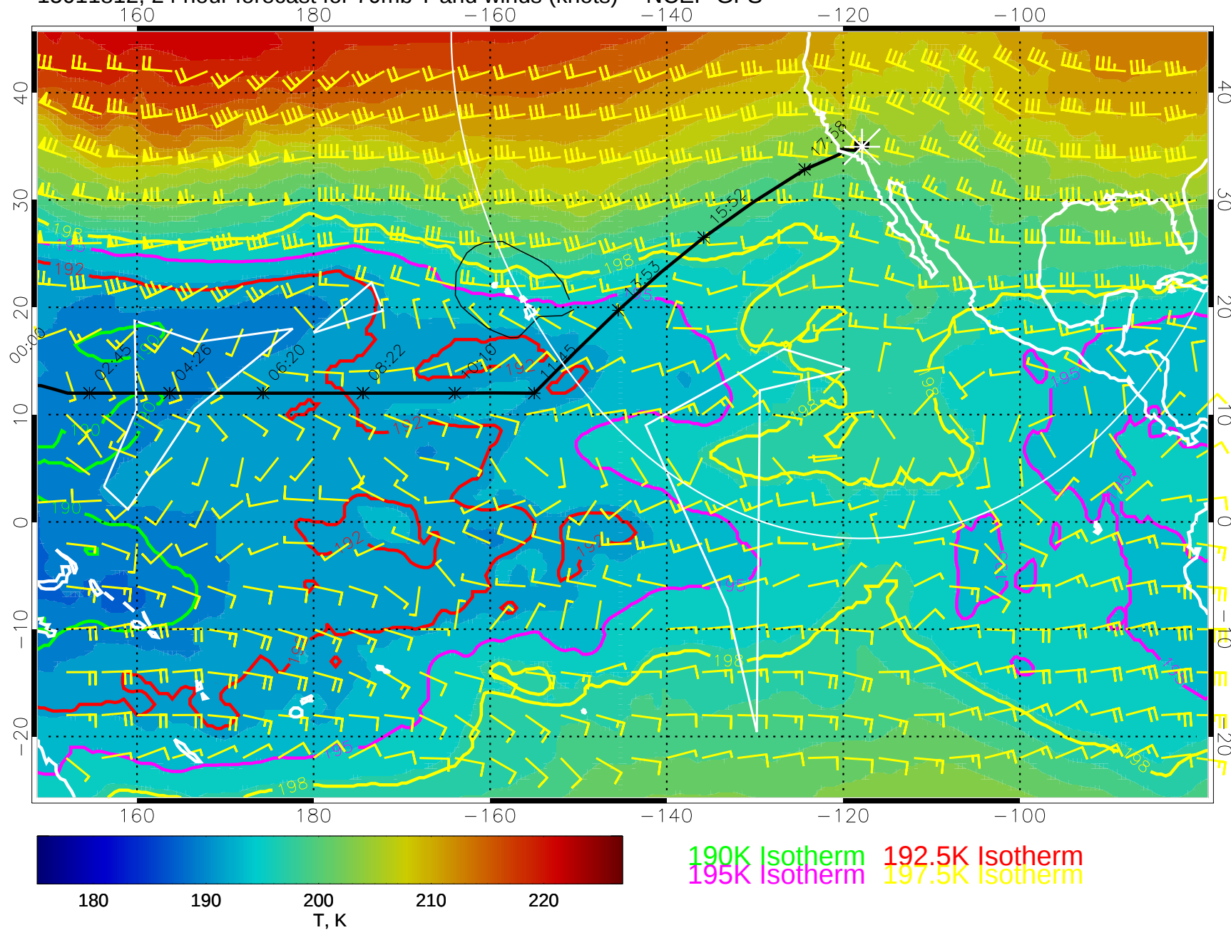
15011812, 24 hour forecast for 70mb T and winds (knots) -- NCEP GFS
