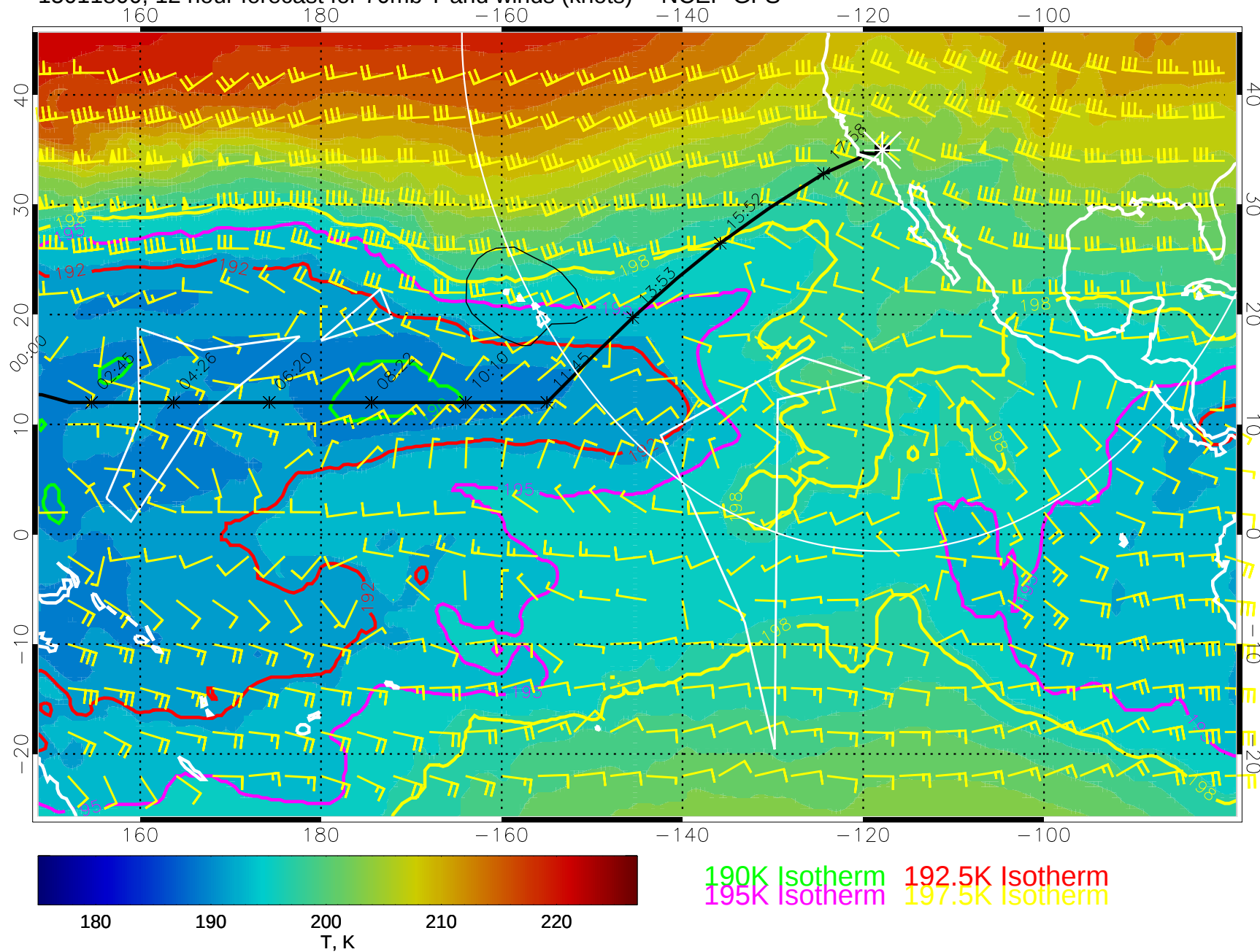
15011800, 12 hour forecast for 70mb T and winds (knots) -- NCEP GFS
