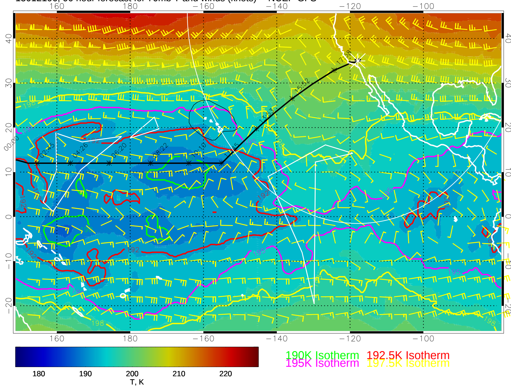
15012106, 90 hour forecast for 70mb T and winds (knots) -- NCEP GFS
