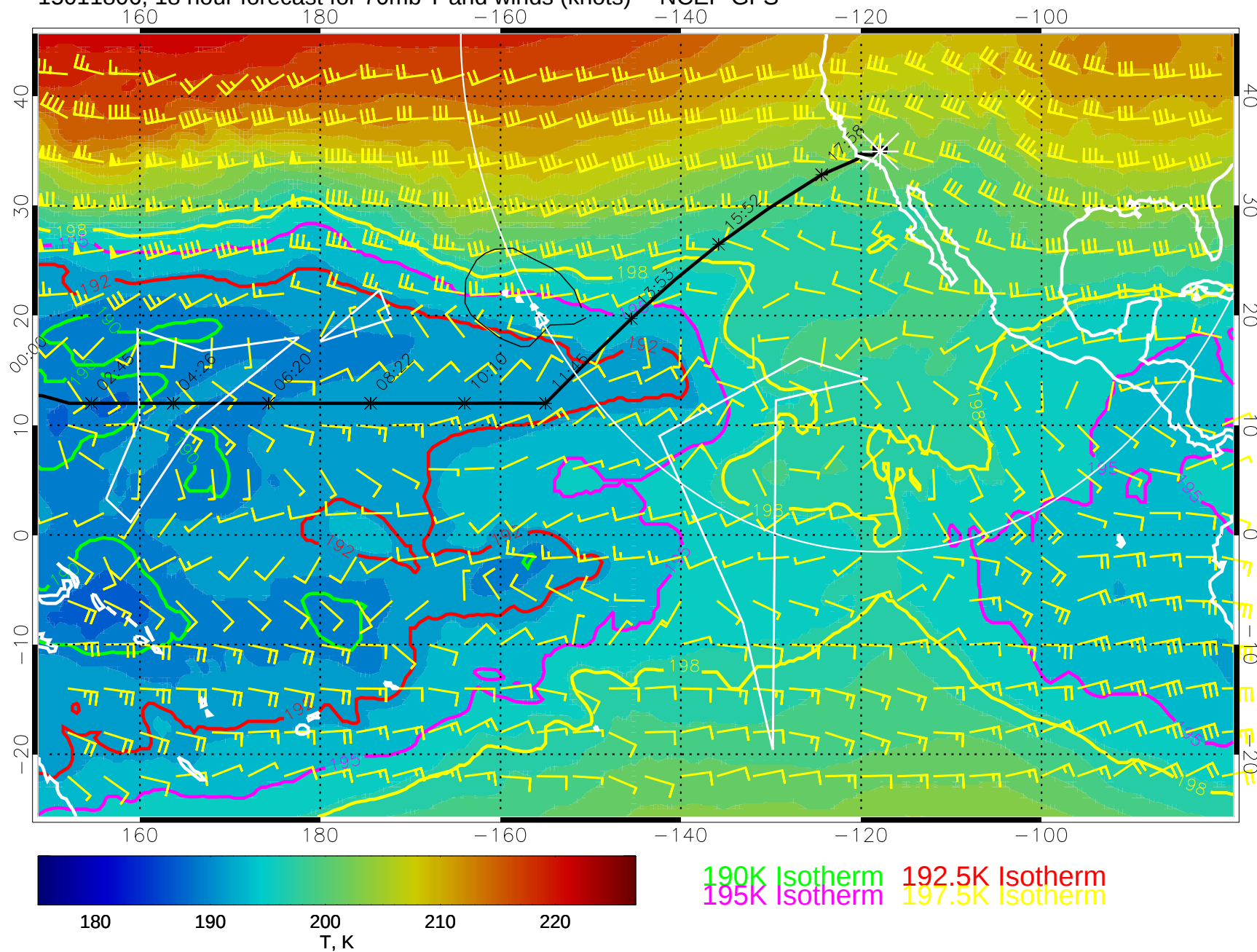
15011806, 18 hour forecast for 70mb T and winds (knots) -- NCEP GFS
