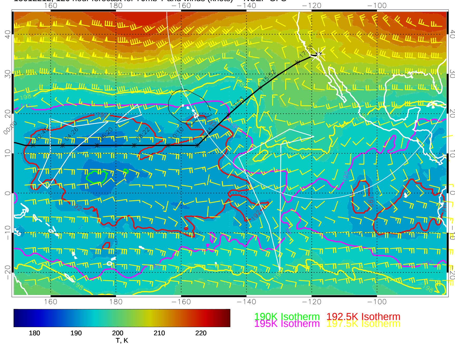
15012212, 120 hour forecast for 70mb T and winds (knots) -- NCEP GFS
