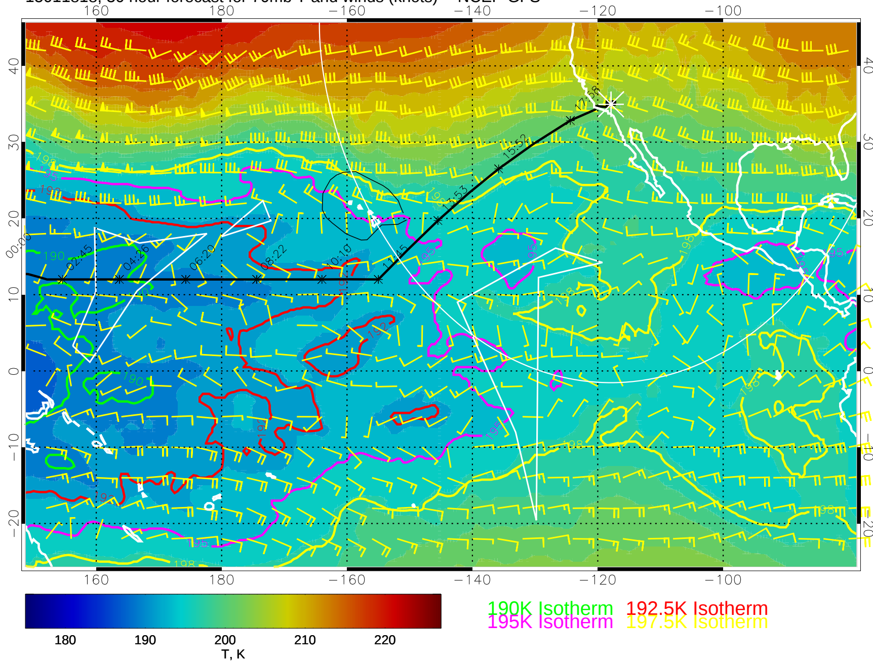
15011818, 30 hour forecast for 70mb T and winds (knots) -- NCEP GFS
