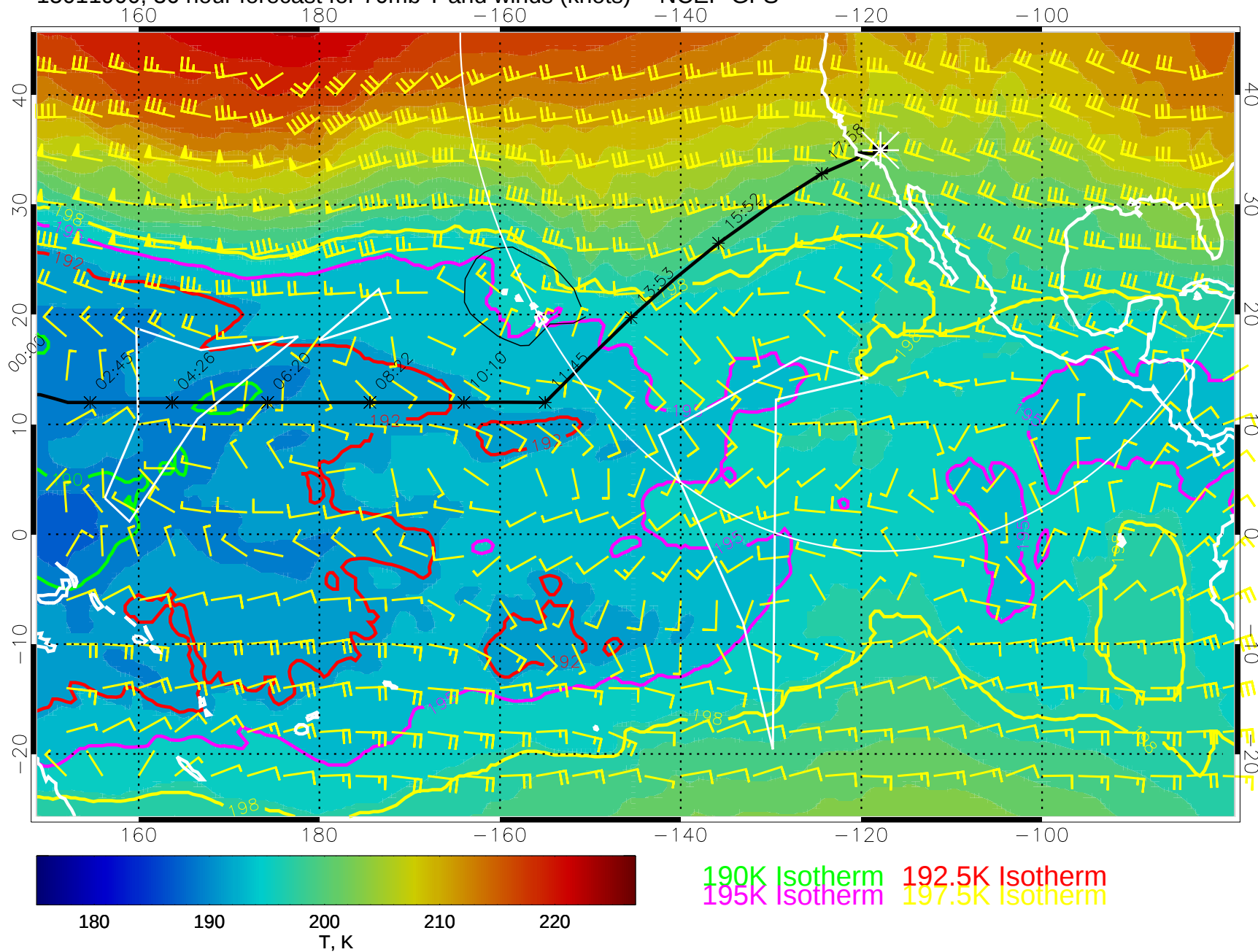
15011900, 36 hour forecast for 70mb T and winds (knots) -- NCEP GFS
