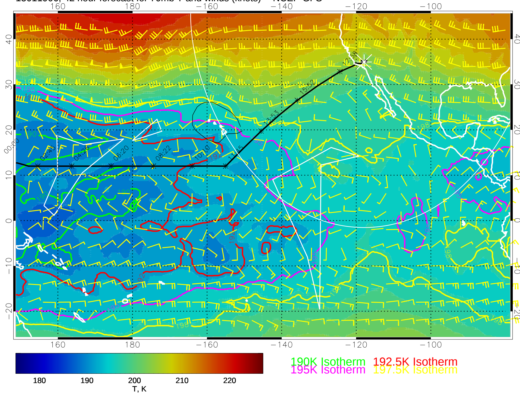
15011906, 42 hour forecast for 70mb T and winds (knots) -- NCEP GFS
