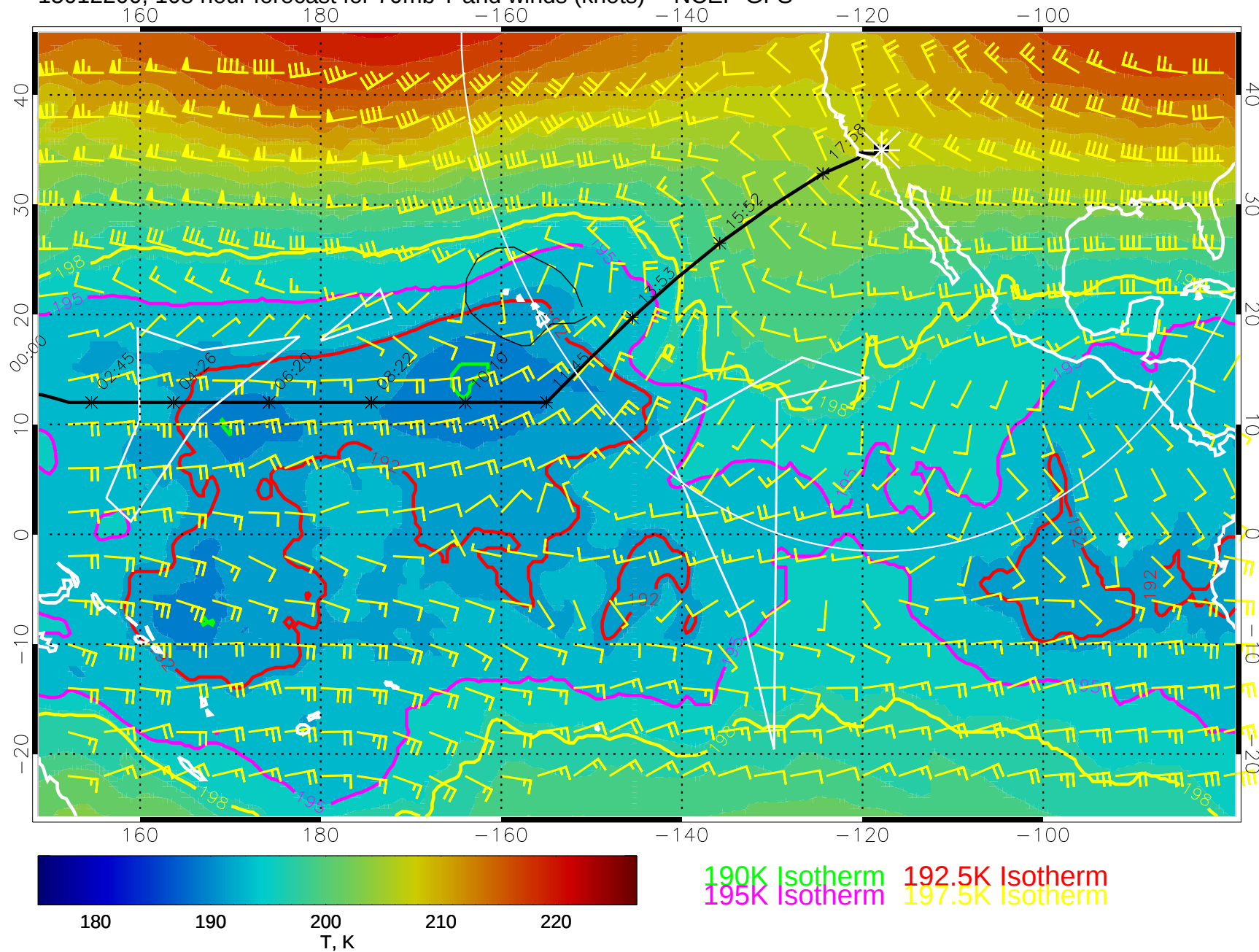
15012200, 108 hour forecast for 70mb T and winds (knots) -- NCEP GFS
