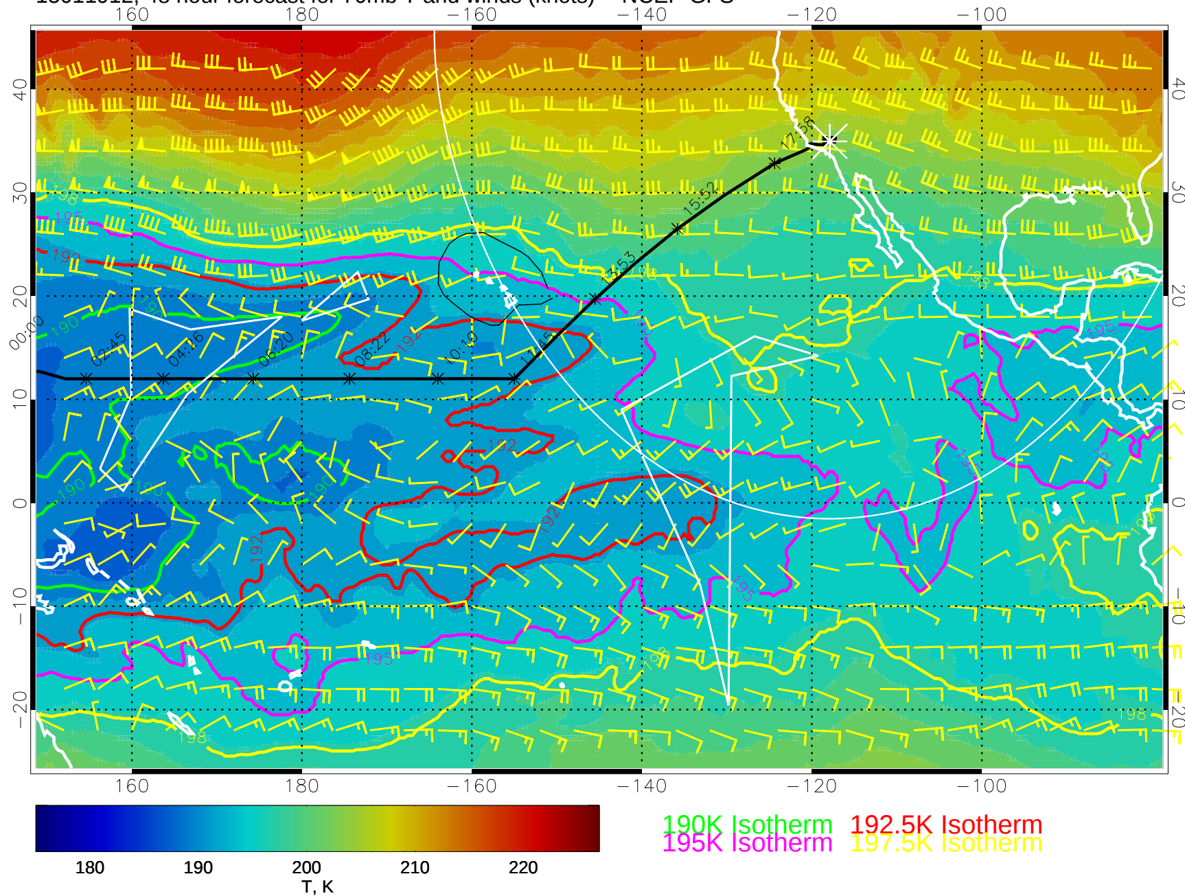
15011912, 48 hour forecast for 70mb T and winds (knots) -- NCEP GFS
