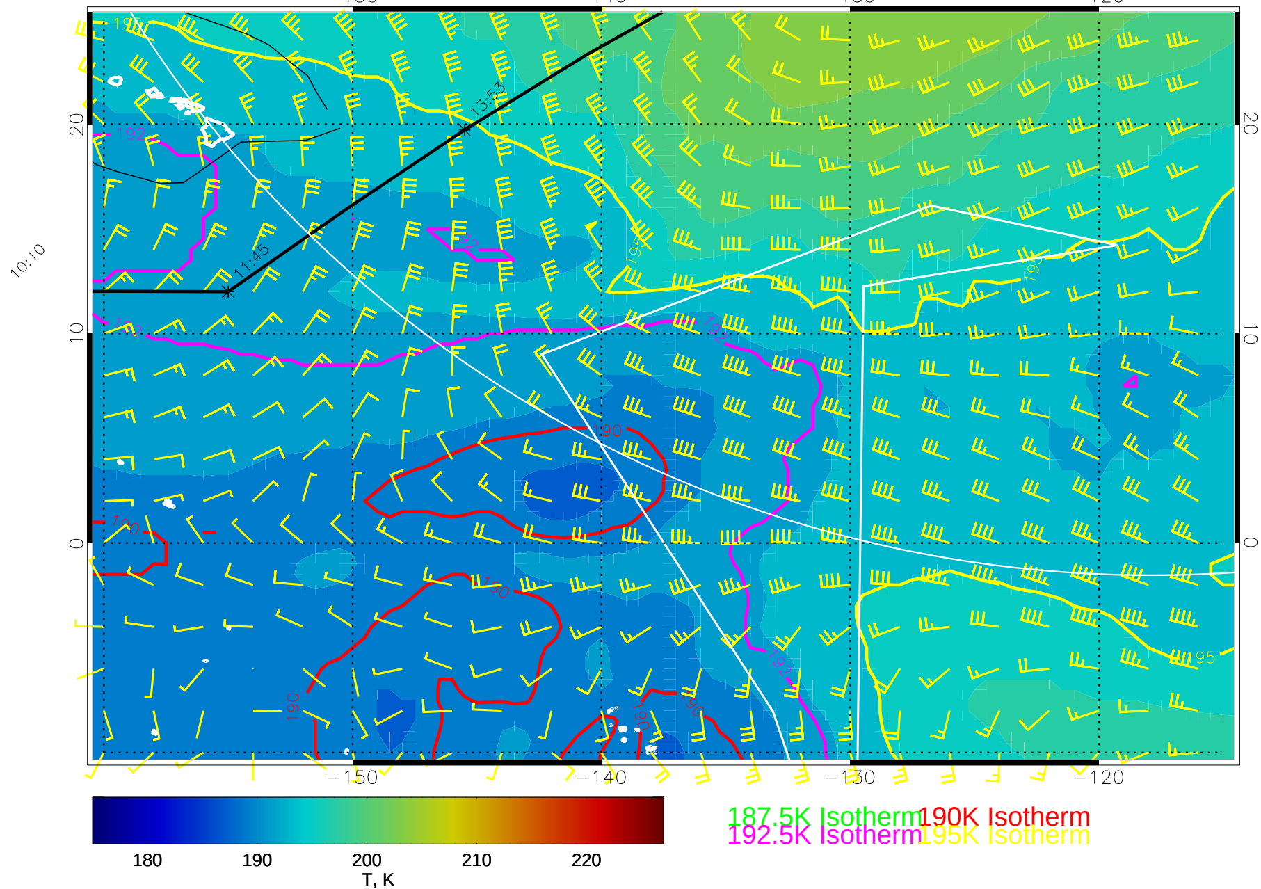
15012112, 96 hour forecast for 100mb T and winds (knots) -- NCEP GFS
